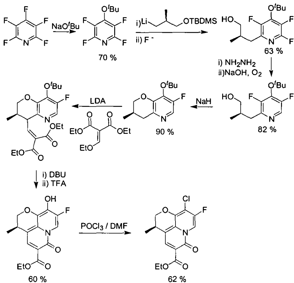
Figure 1.37 2-Pyridone synthesis
