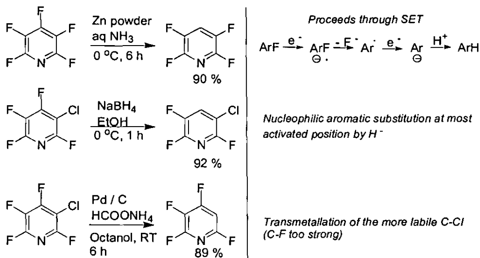
Figure 1.57 Defluorination Strategies
