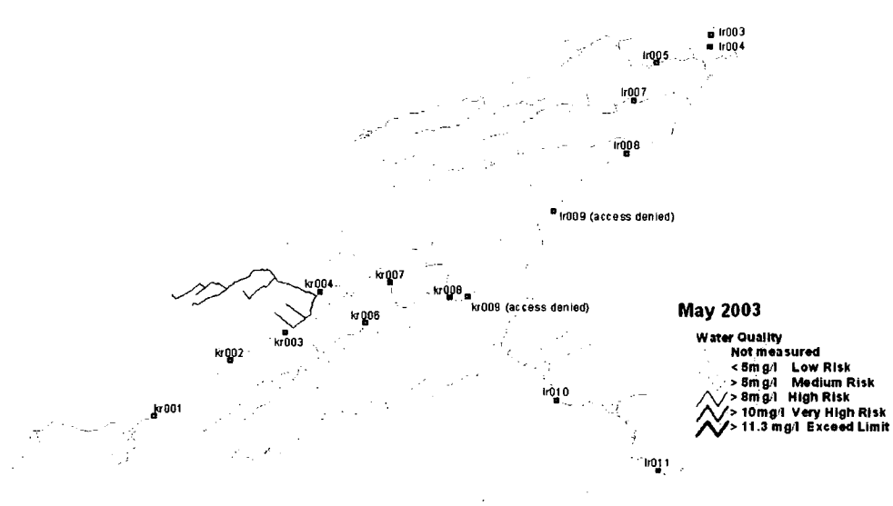
Figure 6.1j NO 3 -N concentrations May 2003
