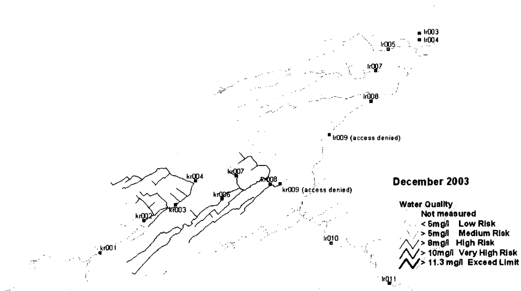
Figure 6.1p NO 3 -N concentrations December 2003
