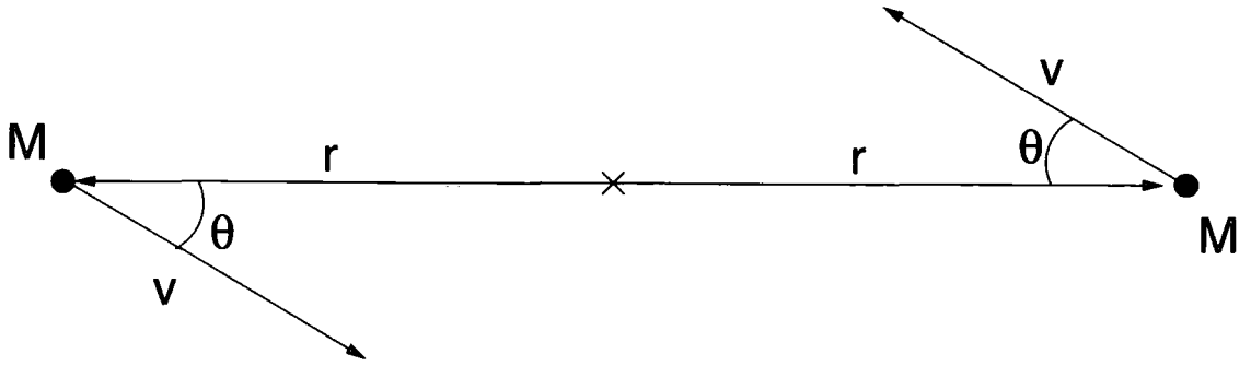
Figure 5.1: Geometry used in the galaxy collision simulations. The circles represent the initial locations of the galaxies. They are separated by an amount 2r , moving with a velocity v and each has mass M .
