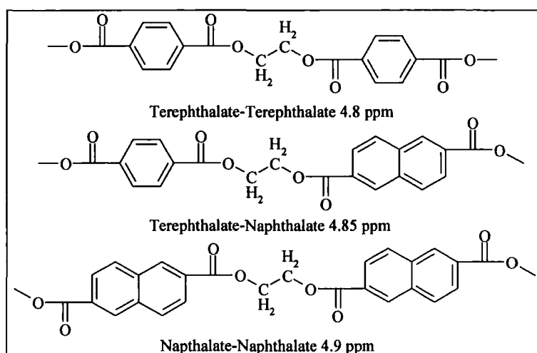
Figure 3.10 Aromatic ^1\text{H} chemical shifts of PET, PEN and PET/PEN copolymer
