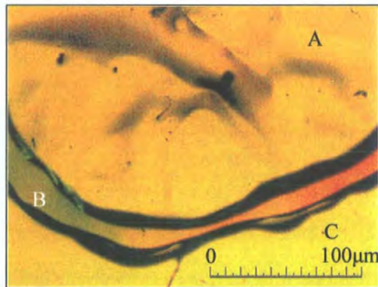
Figure 2.47 A photo of a sample of PET/PC that has been annealed for 60 min at 300^\circ\text{C} and then annealed at 150^\circ\text{C} for 30 min.
