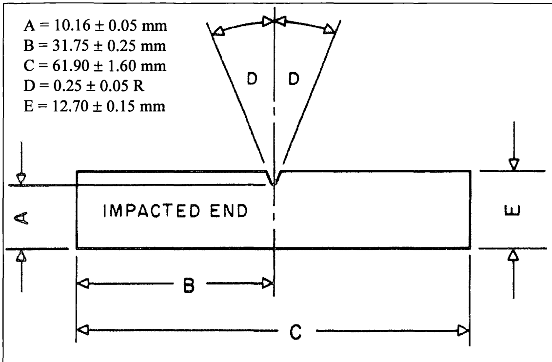
Figure 4.4 Sample shape as dictated by ASTM D256
