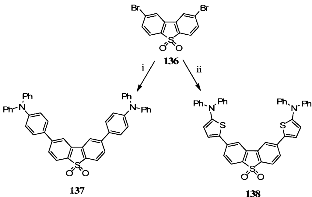
Scheme 1.14 Synthetic route to dibenzothiophene- S,S -dioxide derivatives; i , \text{Bu}_3\text{SnC}_6\text{H}_4\text{NPh}_2 , \text{Pd}(\text{PPh}_3)_2\text{Cl}_2 ; ii , \text{Bu}_3\text{SnC}_4\text{H}_2\text{SNPh}_2 , \text{Pd}(\text{PPh}_3)_2\text{Cl}_2
