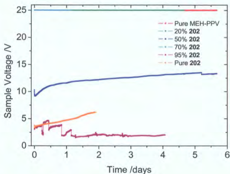
Figure 2.7b Stability data for devices of configuration ITO/PEDOT:PSS/202:MEH-PPV/Al: sample voltage vs time
