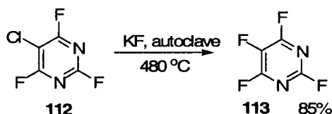
Scheme 1.27
