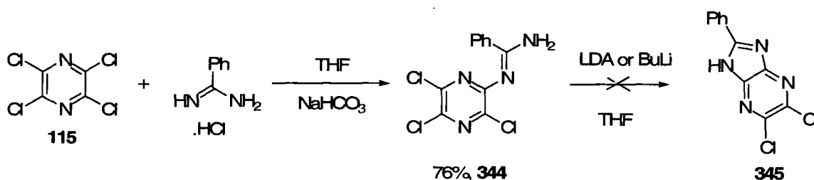
Scheme 5.11
