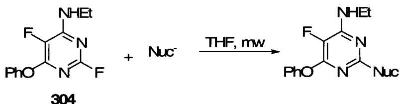
Scheme 3.17
