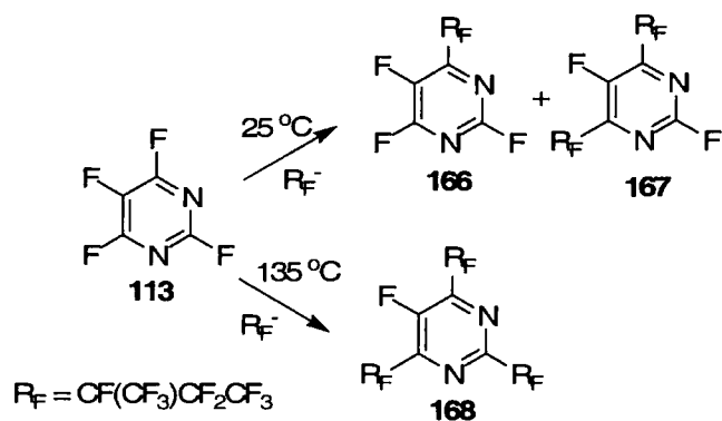
Scheme 1.42
