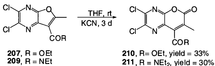
Scheme 1.52
