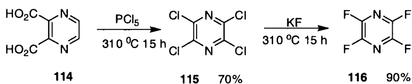
Scheme 1.28
