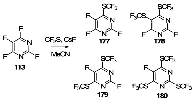
Scheme 1.45
