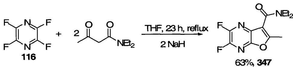
Scheme 5.16
