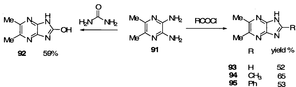
Scheme 1.18
