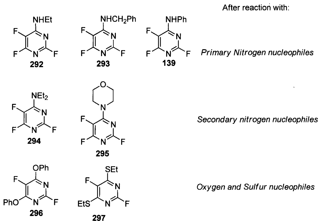
Figure 3.9. Monofunctionalised pyrimidines synthesised from tetrafluoropyrimidine, 113 .
