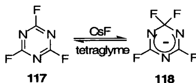
Scheme 1.30
