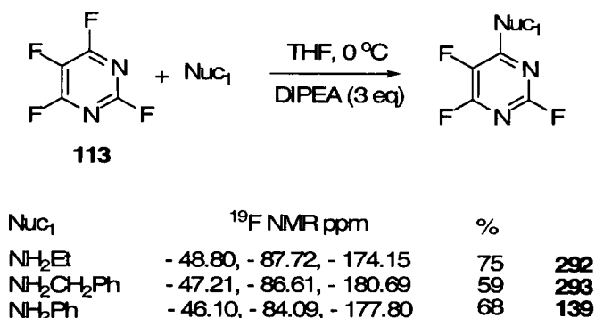
Scheme 3.2
