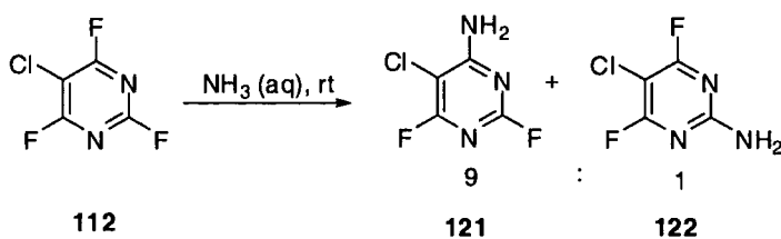
Scheme 2.2
