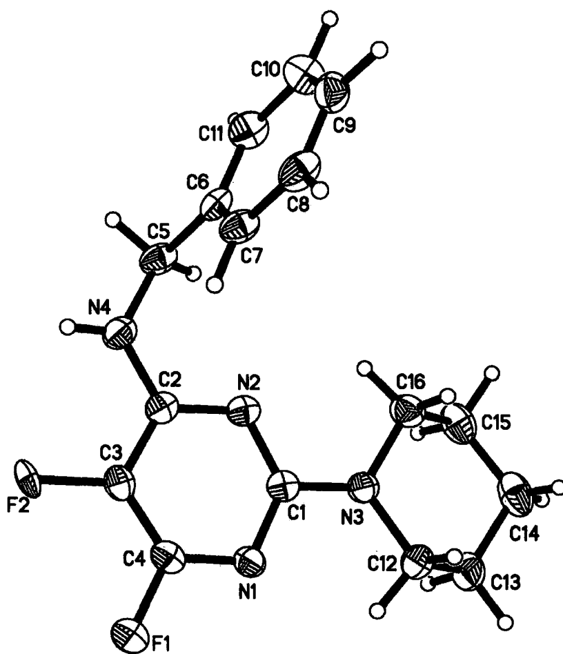
Figure 3.1 The x-ray crystallography structure of compound 303
