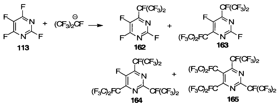
Scheme 1.41
