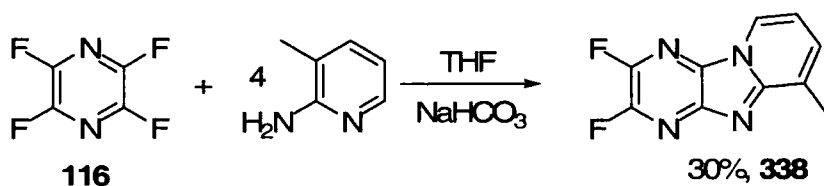
Scheme 5.5
