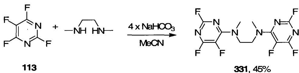
Scheme 4.4
