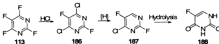
Scheme 1.47
