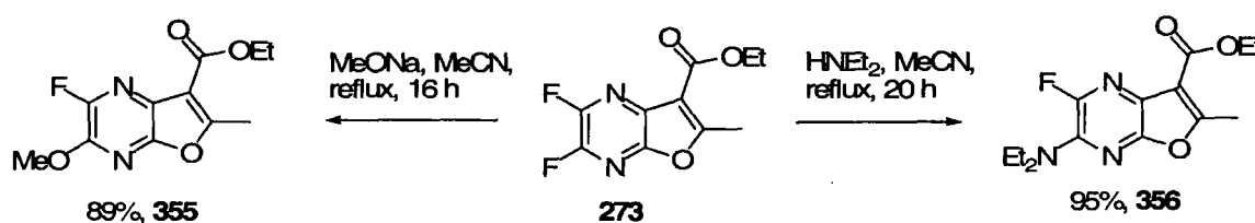
Scheme 5.25
