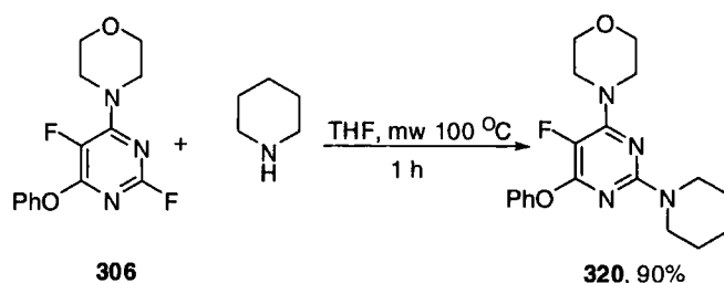
Scheme 3.19
