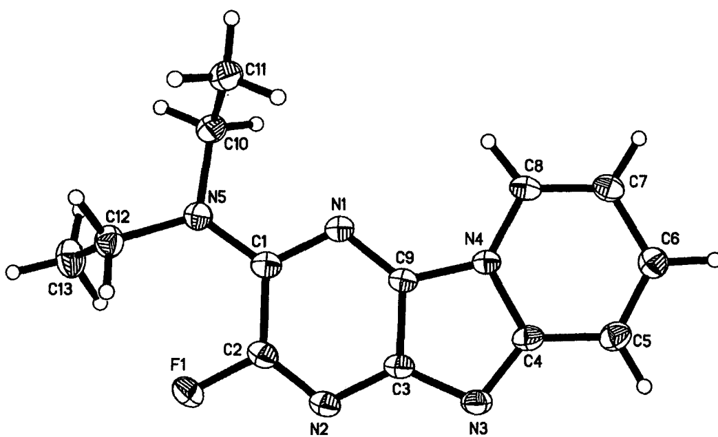
Figure 5.9 The x-ray crystallography structure of compound 352
