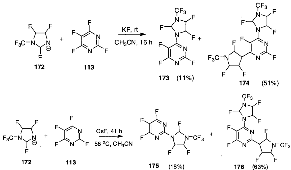
Scheme 1.44
