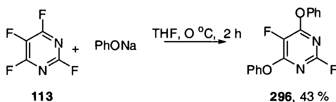
Scheme 3.4
