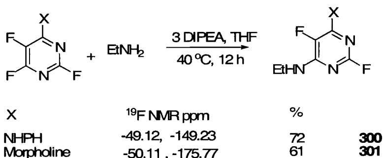
Scheme 3.8
