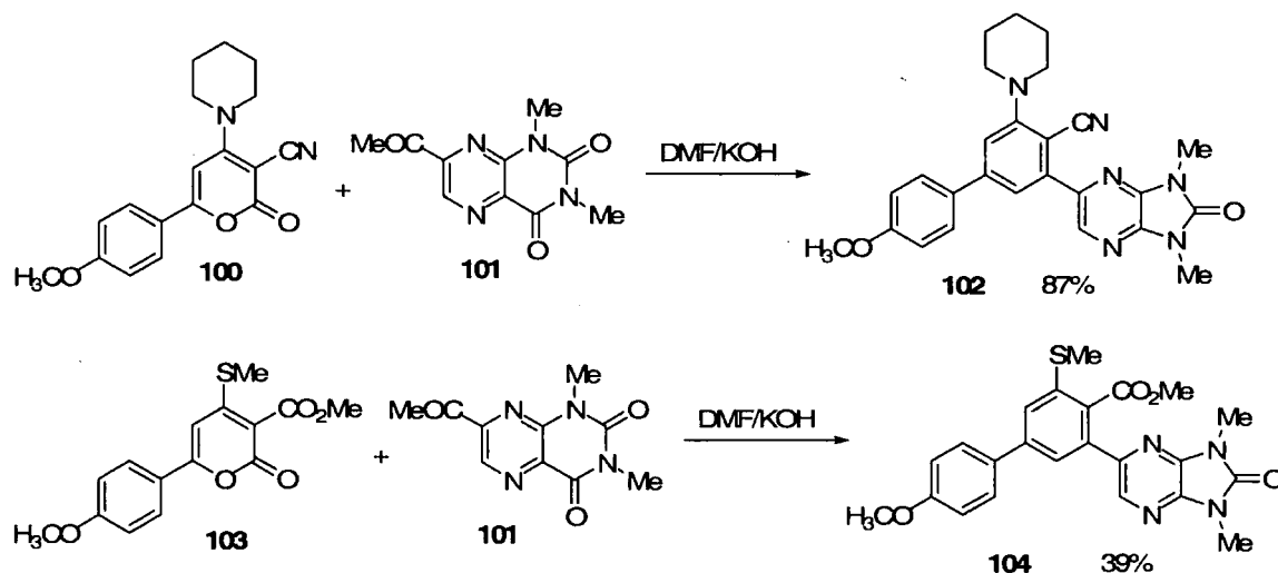
Scheme 1.20
