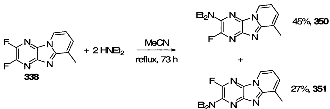
Scheme 5.22
