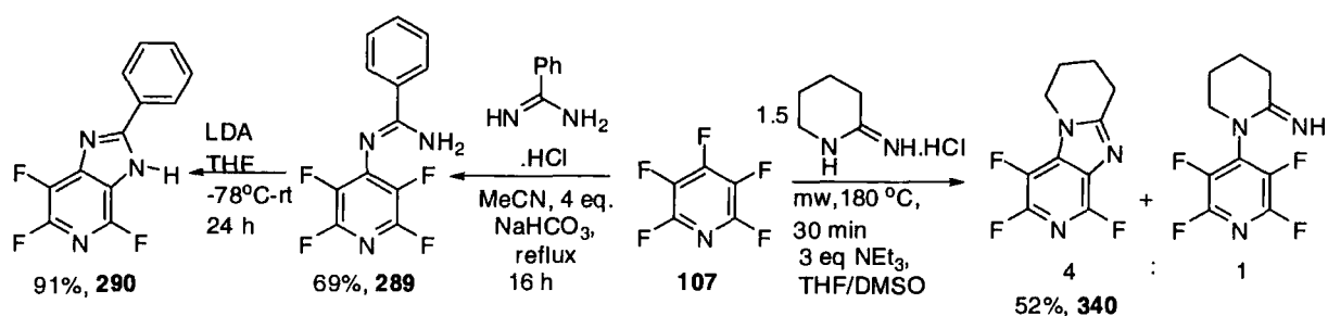
Scheme 5.8
