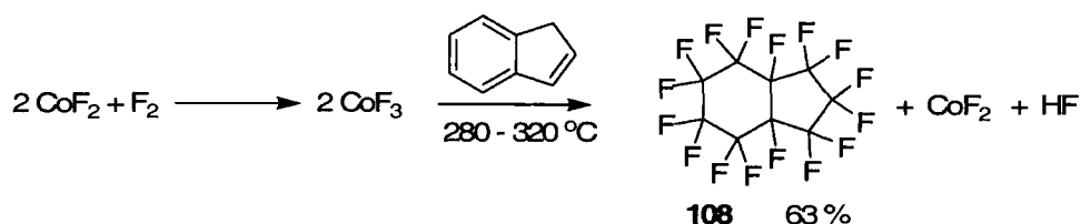
Scheme 1.22
