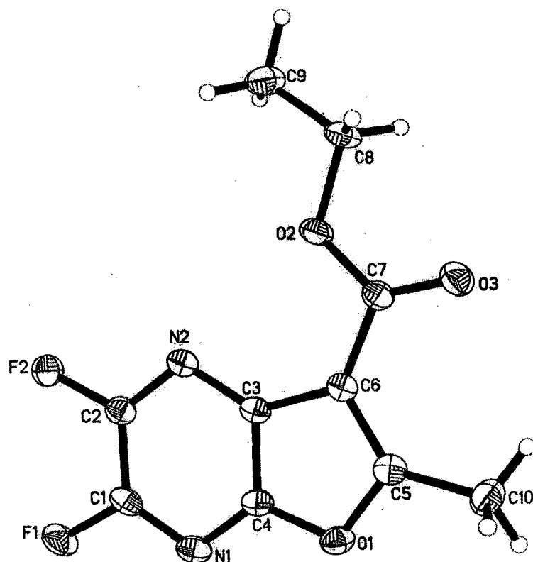
Figure 5.3 The x-ray crystallography structure of compound 273
