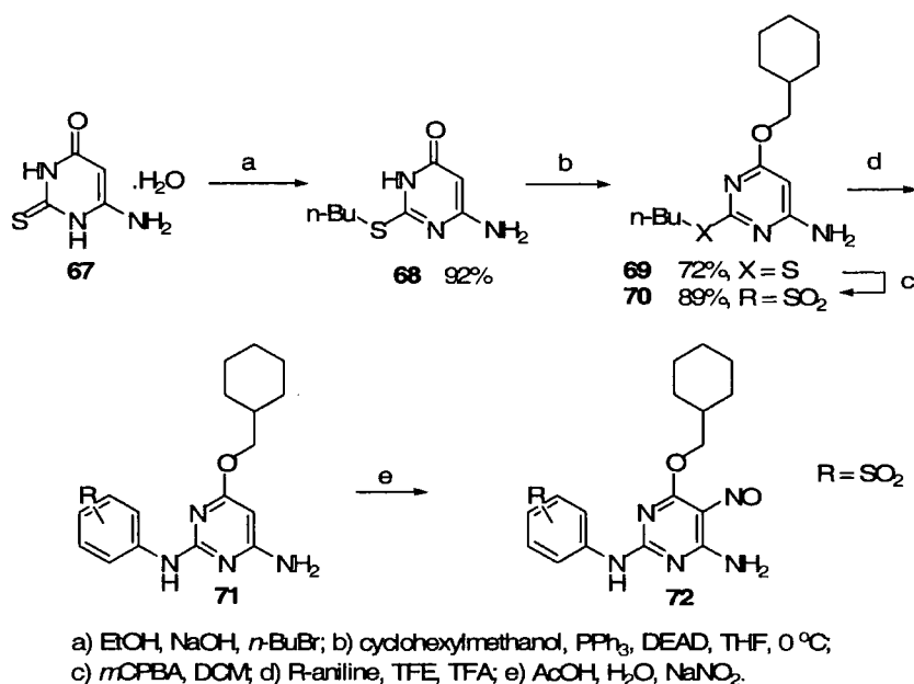
Scheme 1.14
