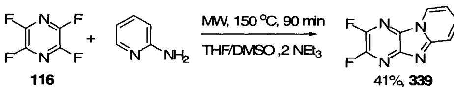
Scheme 5.7
