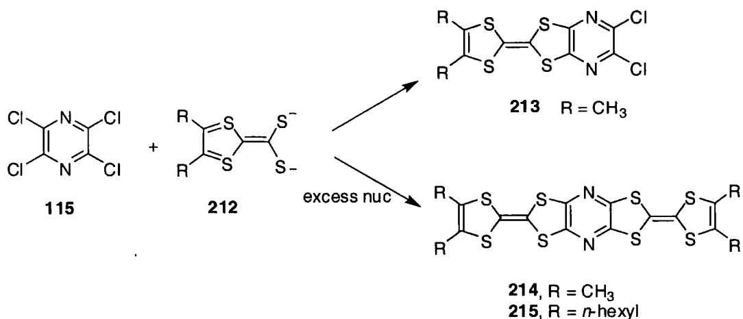
Scheme 1.53
