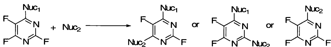
Scheme 3.6
