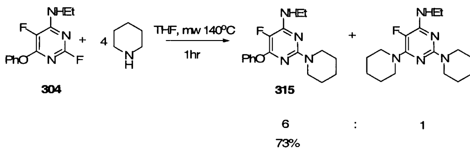
Scheme 3.14
