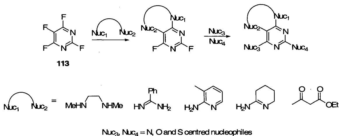
Scheme 4.1
