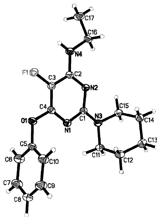
Figure 3.4 The x-ray crystallography structure of compound 315
