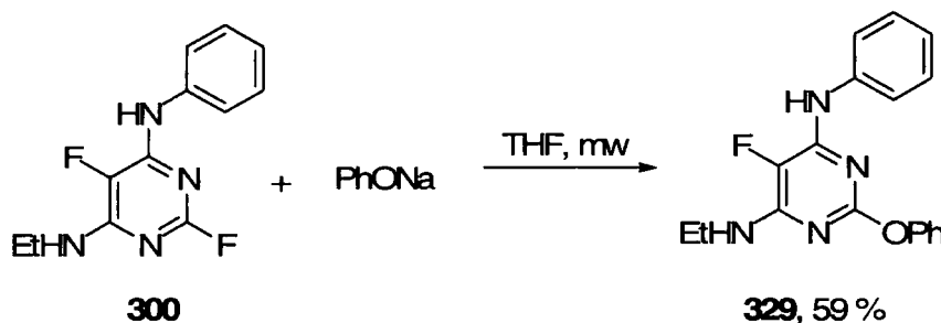
Scheme 3.25
