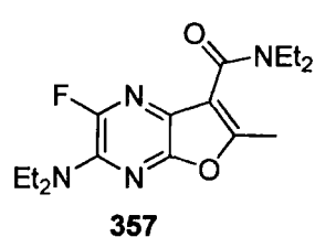
Figure 5.11 The reaction of Imidazo[4,5- b ] and Furo[2,3- b ]pyrazines with mono nucleophiles
