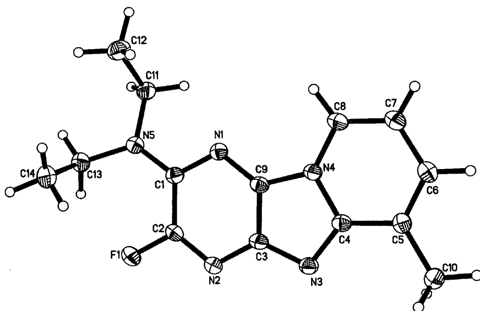
Figure 5.8 The x-ray crystallography structure of compound 350
