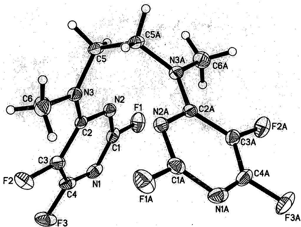
Figure 4.2 The x-ray crystallography structure of compound 331
