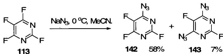
Scheme 1.35
