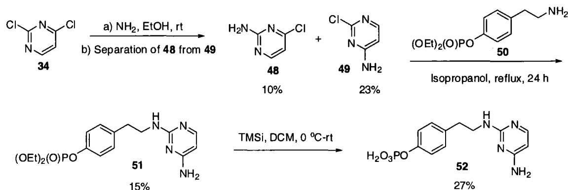
Scheme 1.11
