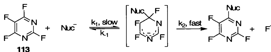
Scheme 1.29
