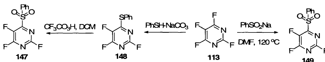
Scheme 1.36
