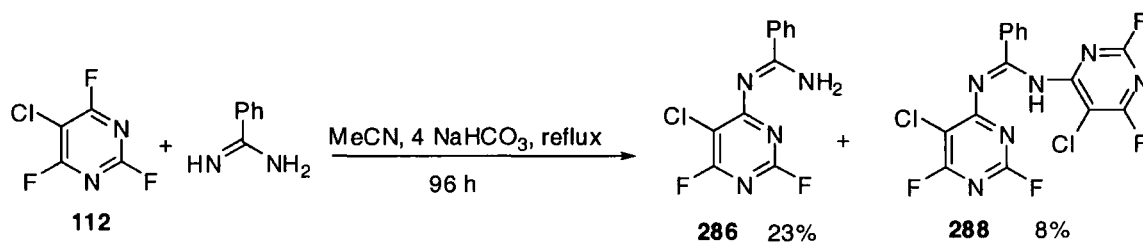
Scheme 2.4
