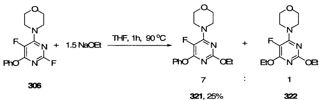
Scheme 3.20
