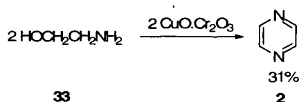
Scheme 1.8
