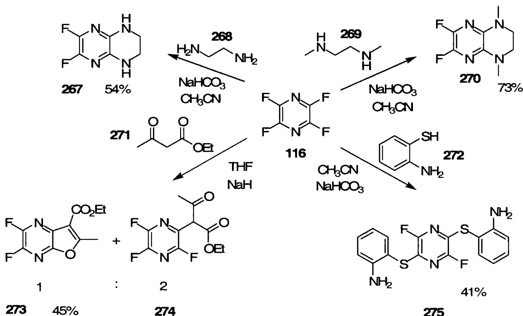
Scheme 1.59
