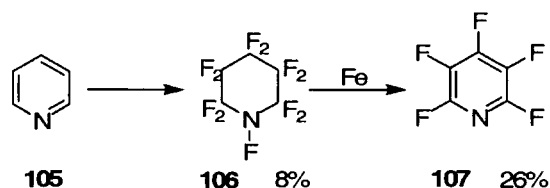
Scheme 1.21
