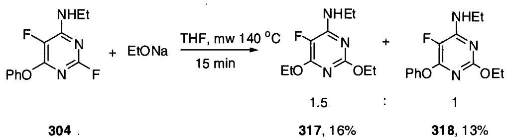
Scheme 3.16
