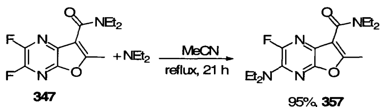
Scheme 5.26
