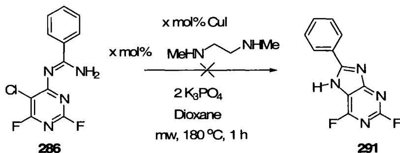
Scheme 2.7
