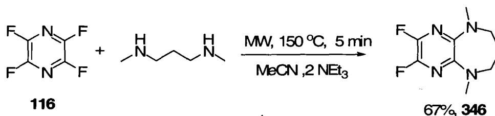
Scheme 5.13
