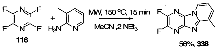
Scheme 5.6
