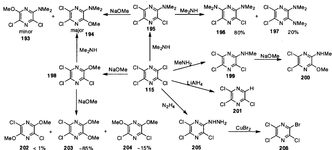
Scheme 1.50
