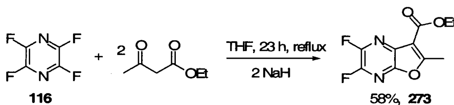
Scheme 5.15
