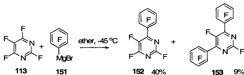
Scheme 1.38
