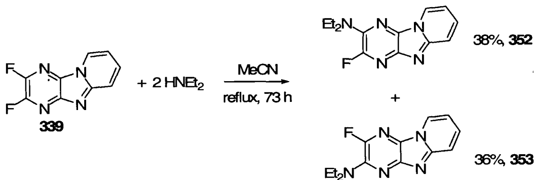
Scheme 5.24
