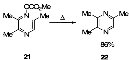
Scheme 1.5
