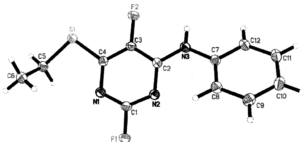
Figure 3.3 The x-ray crystallography structure of compound 312
