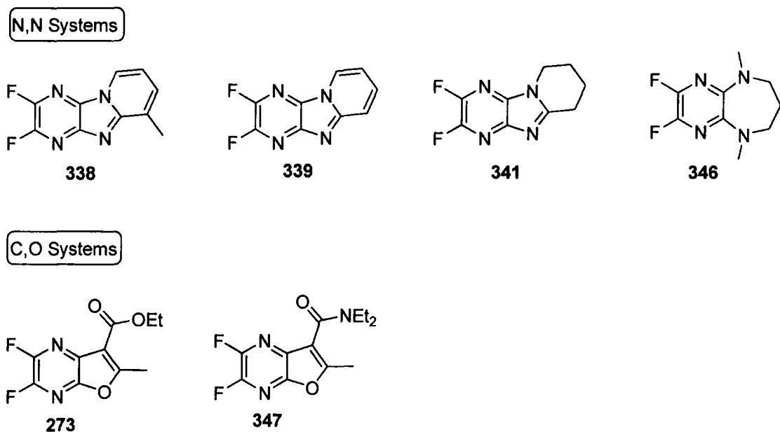
Figure 5.10 A summary of the reaction of tetrafluoropyrazine, 116 , with N,N and C,O dinucleophiles
