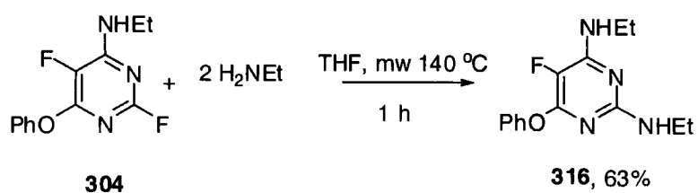
Scheme 3.15
