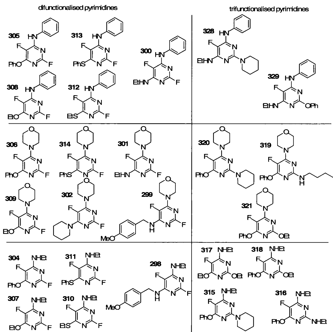
Figure 3.10. Difunctionalised and trifunctionalised pyrimidines synthesised from tetrafluoropyrimidine, 113 .
