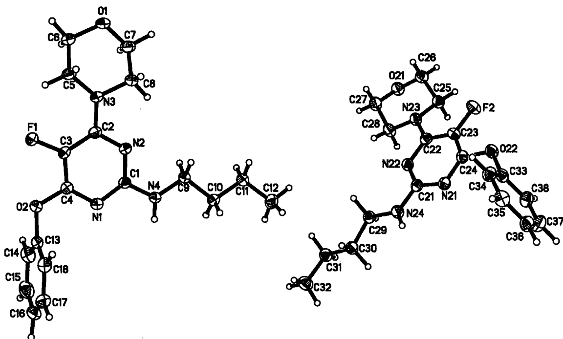
Figure 3.7 The x-ray crystallography structure of compound 319
