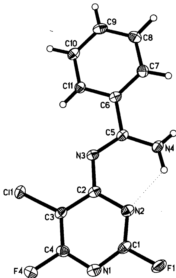
Figure 2.1 The X-ray crystallography structure of compound 286.
