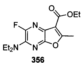
Figure 5.11 The reaction of Imidazo[4,5- b ] and Furo[2,3- b ]pyrazines with mono nucleophiles
