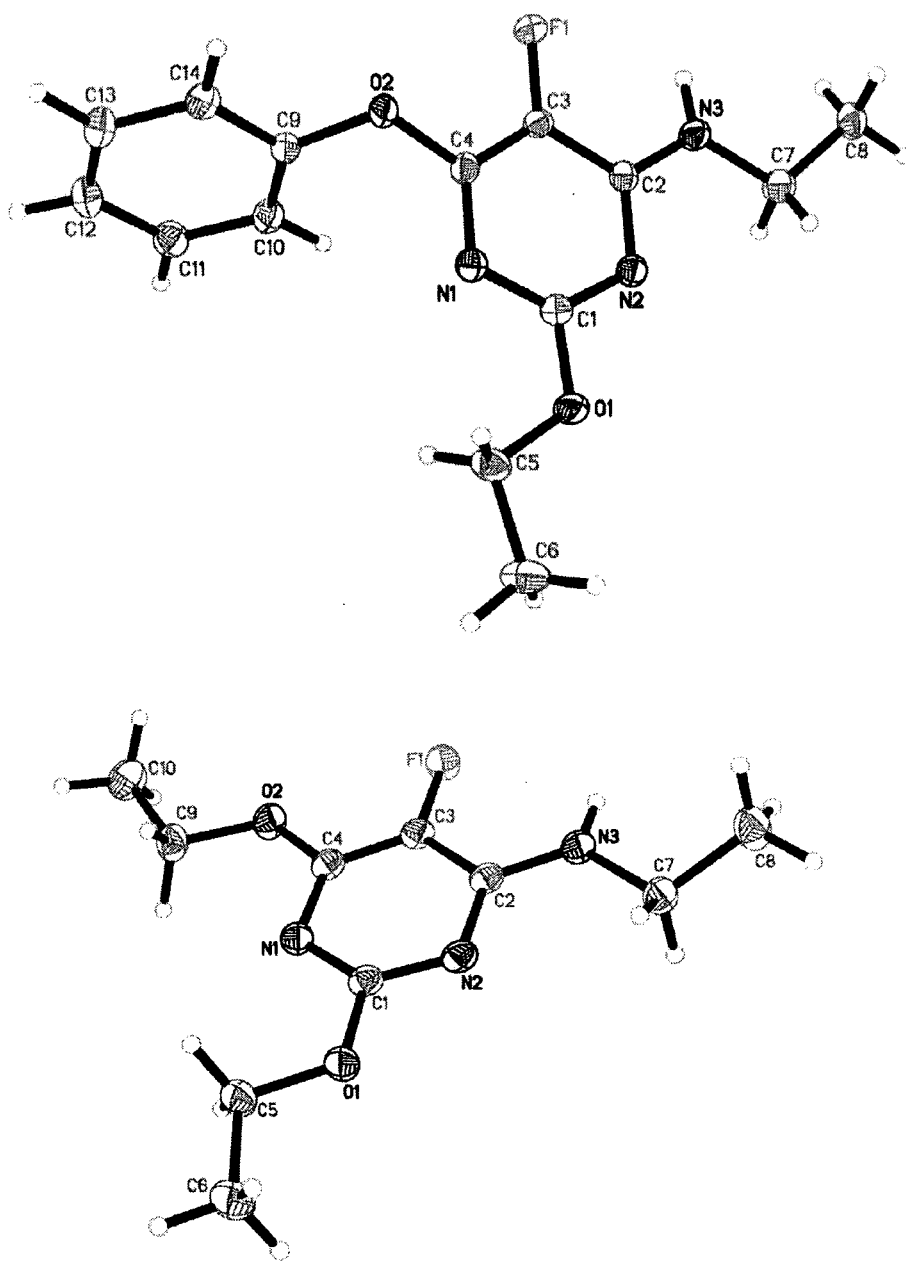
Figure 3.6 The x-ray crystallography structures of compounds 317 and 318
