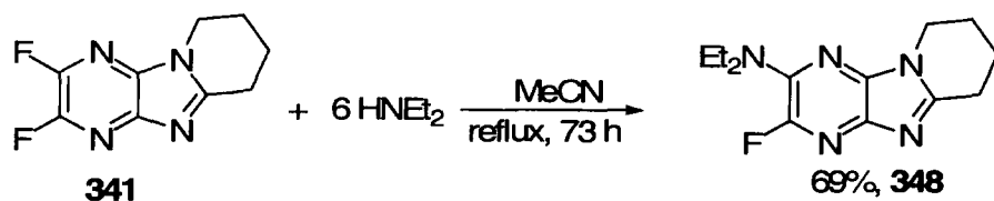
Scheme 5.19
