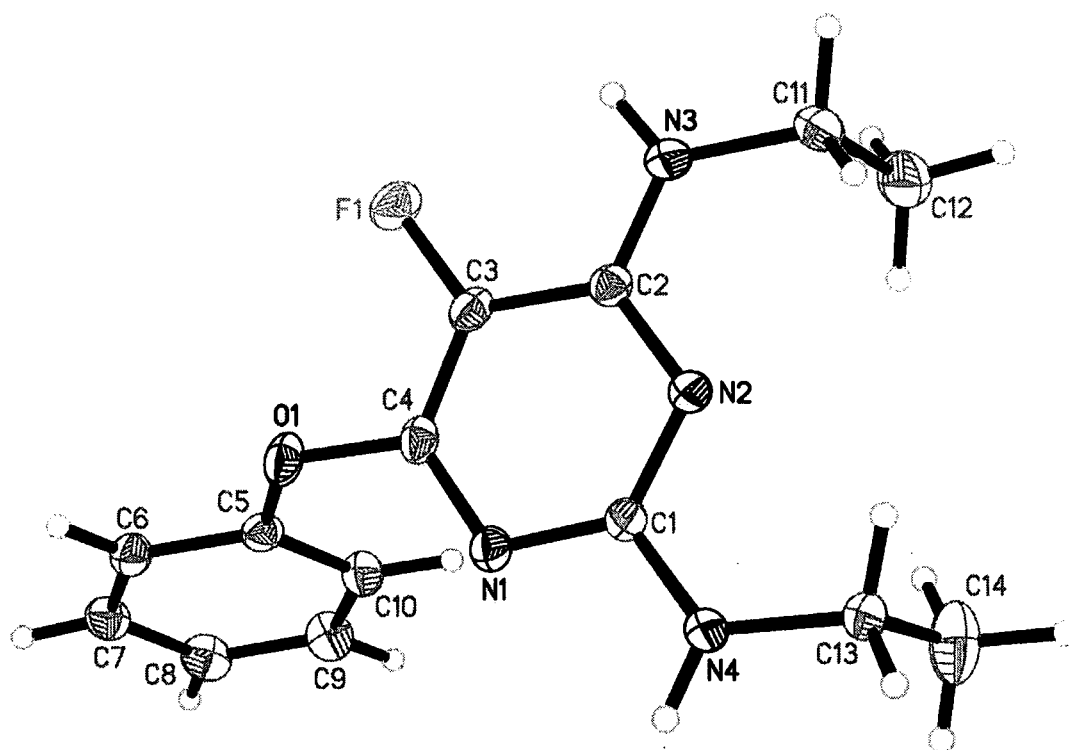
Figure 3.5 The x-ray crystallography structure of compound 316
