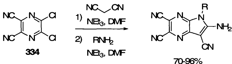
Scheme 5.3
