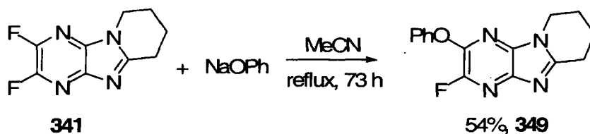
Scheme 5.20
