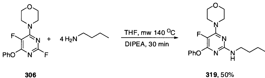
Scheme 3.18
