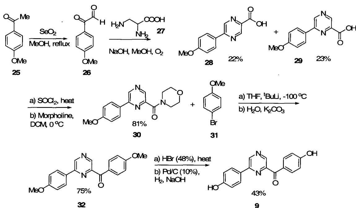
Scheme 1.7
