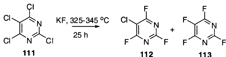
Scheme 1.26
