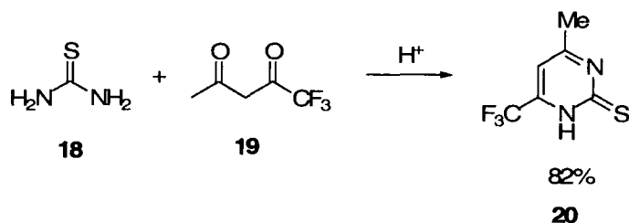
Scheme 1.3
