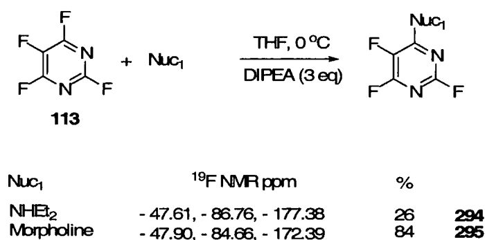
Scheme 3.3
