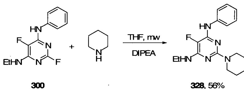
Scheme 3.24
