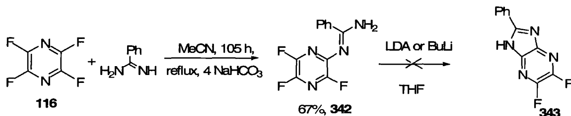
Scheme 5.10
