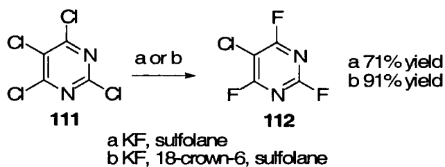
Scheme 1.25
