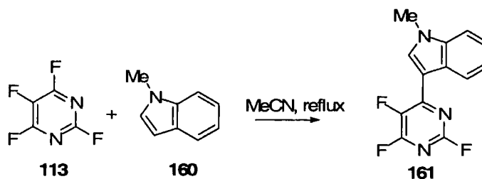
Scheme 1.40
