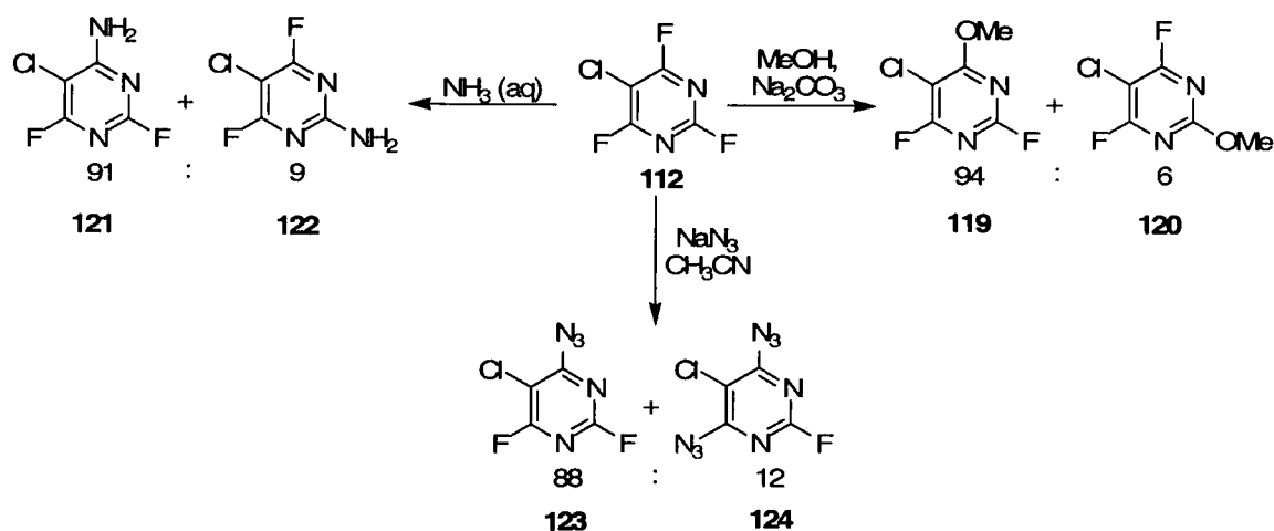
Scheme 1.31
