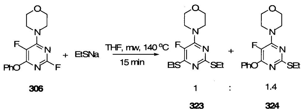
Scheme 3.21
