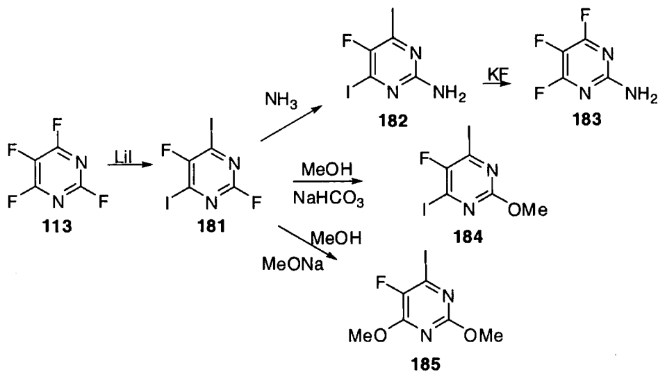
Scheme 1.46
