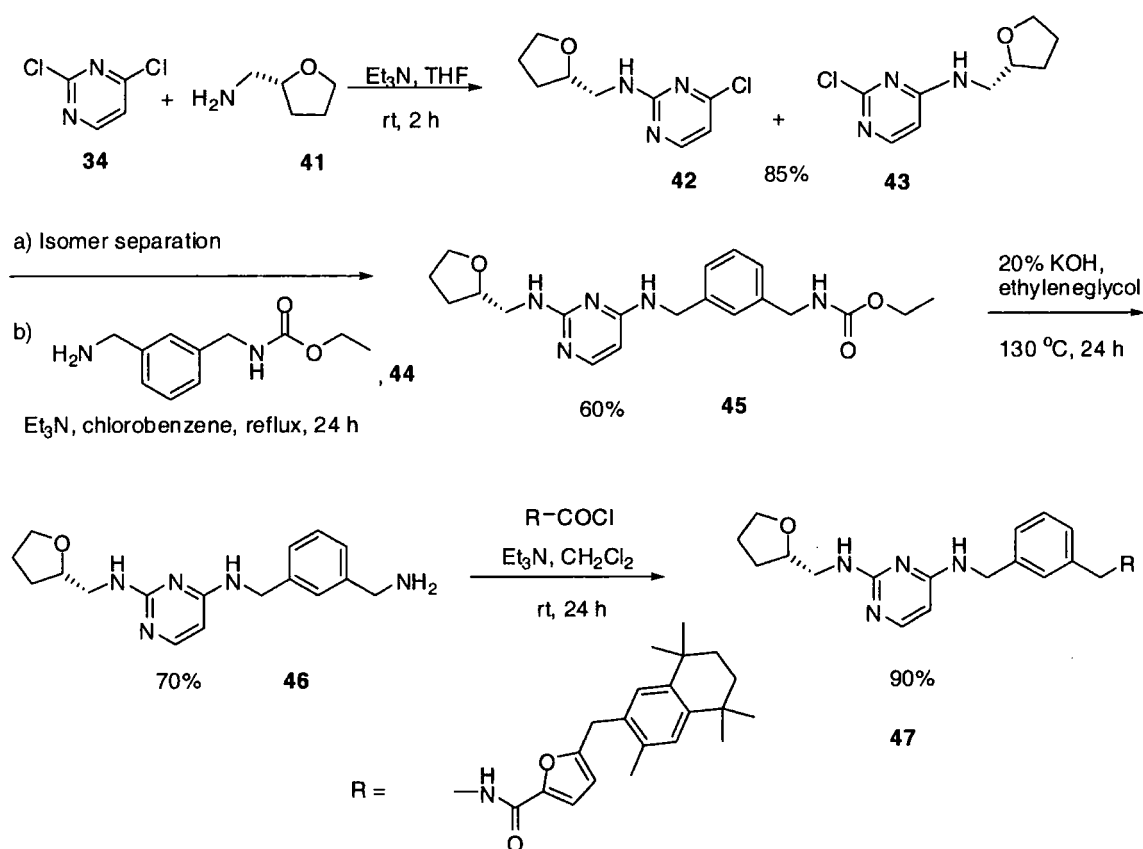
Scheme 1.10
