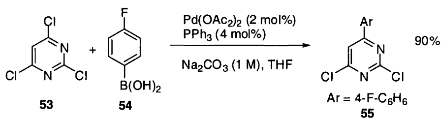
Scheme 1.12
