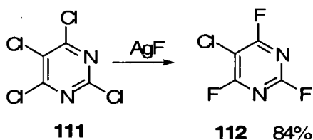
Scheme 1.24
