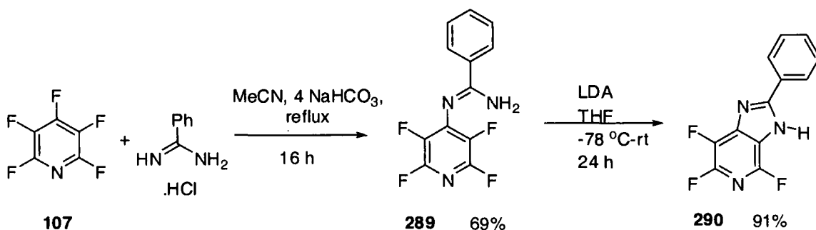
Scheme 2.5
