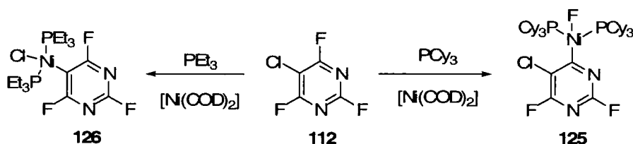
Scheme 1.32
