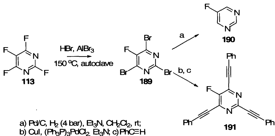
Scheme 1.48
