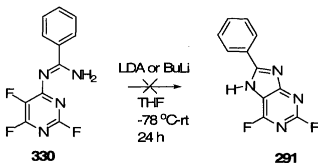
Scheme 4.3
