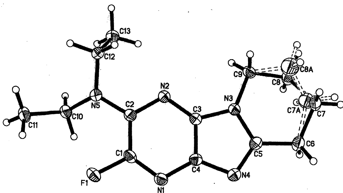
Figure 5.5 The x-ray crystallography structure of compound 348
