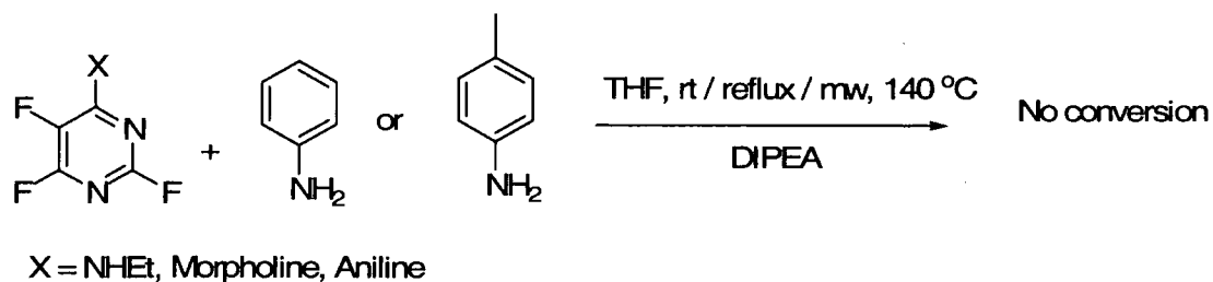
Scheme 3.10
