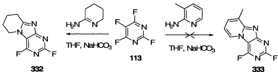
Scheme 4.5
