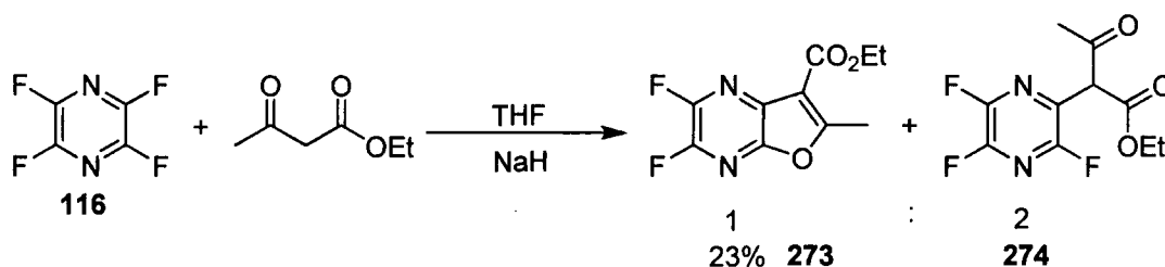
Scheme 5.14
