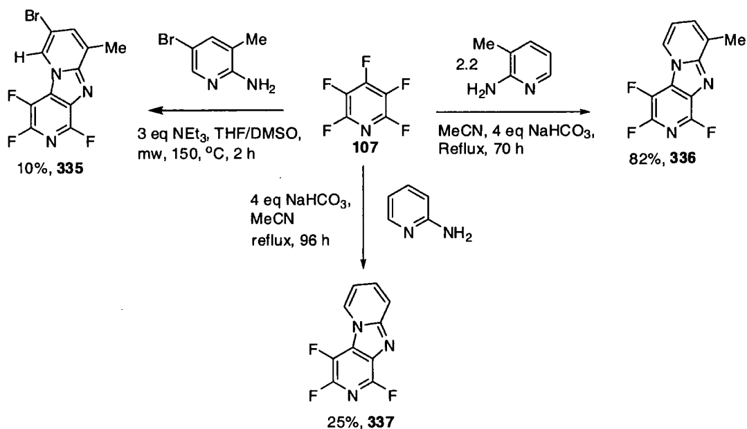
Scheme 5.4
