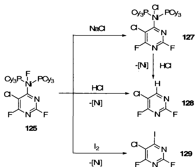
Scheme 1.33
