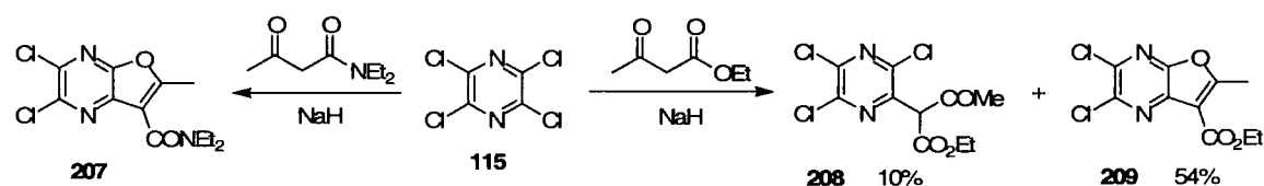
Scheme 1.51
