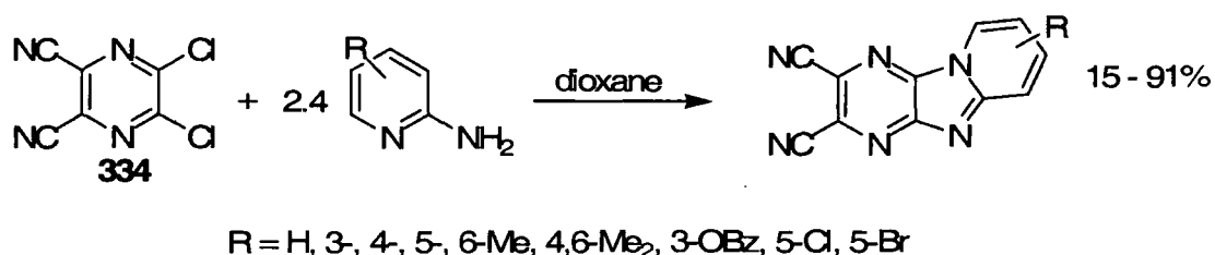
Scheme 5.2
