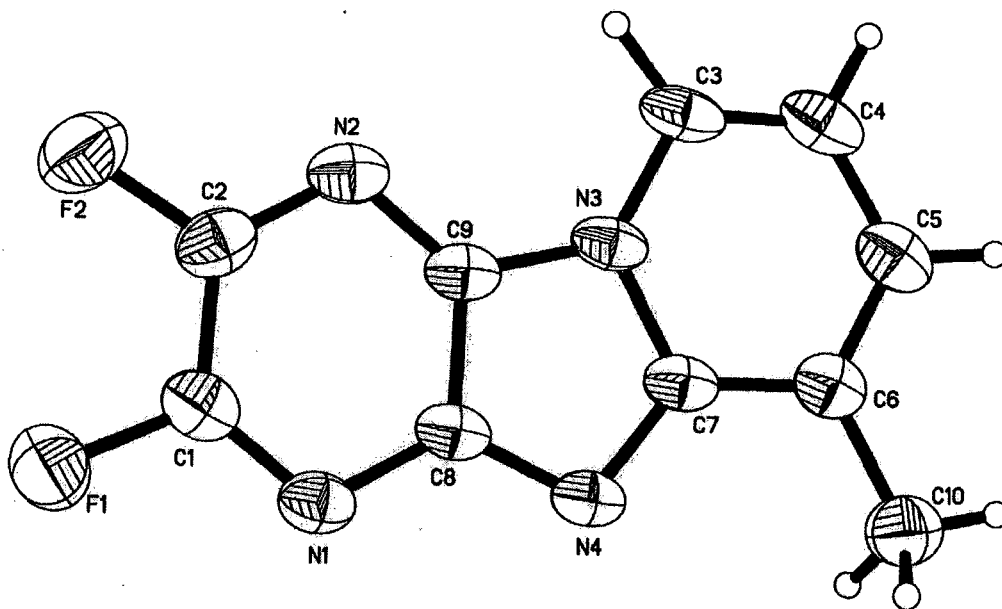
Figure 5.1 The x-ray crystallography structure of compound 338
