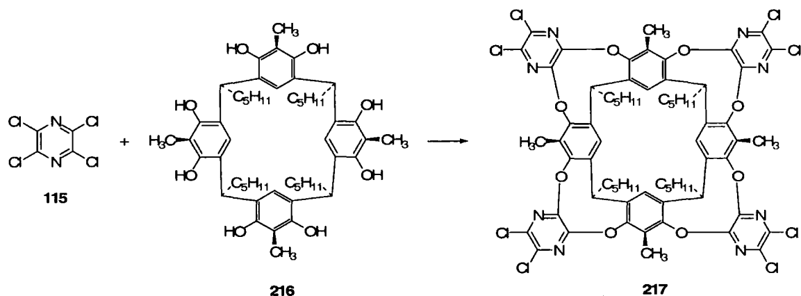
Scheme 1.54
