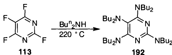
Scheme 1.49
