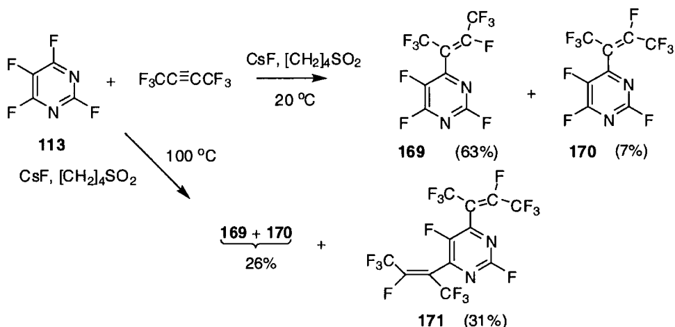
Scheme 1.43
