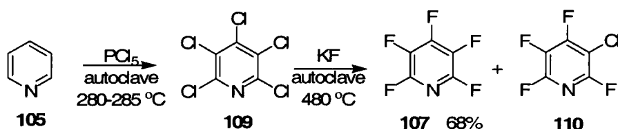
Scheme 1.23
