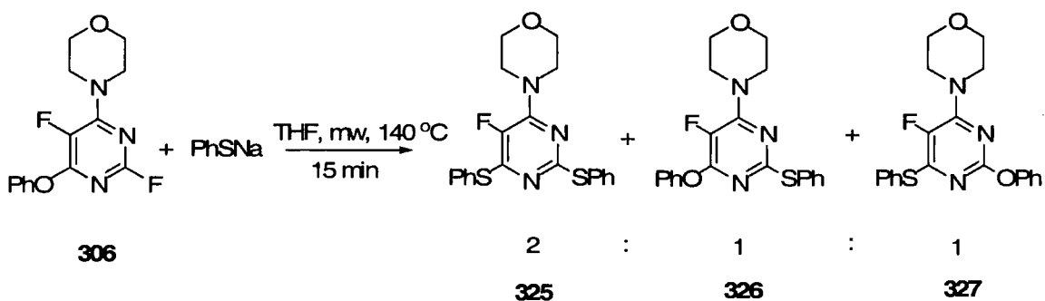
Scheme 3.22
