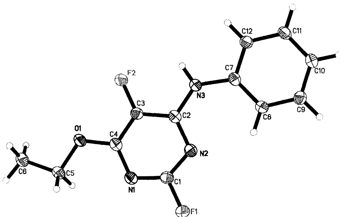
Figure 3.2 The x-ray crystallography structure of compound 308
