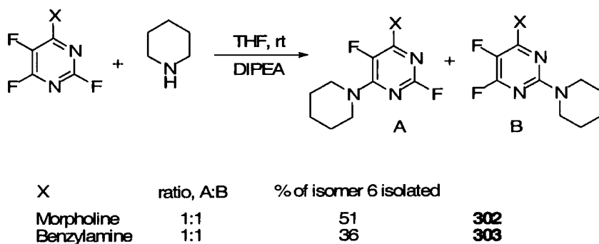
Scheme 3.9
