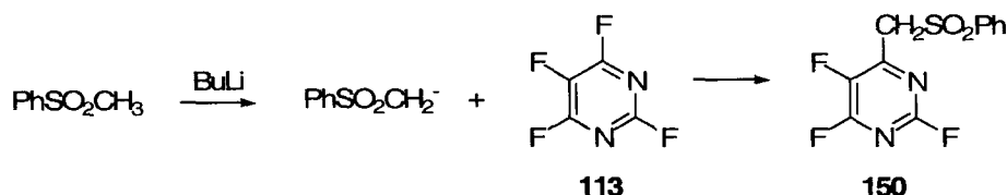
Scheme 1.37
