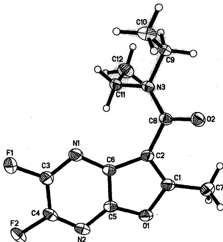
Figure 5.4 The x-ray crystallography structure of compound 347
