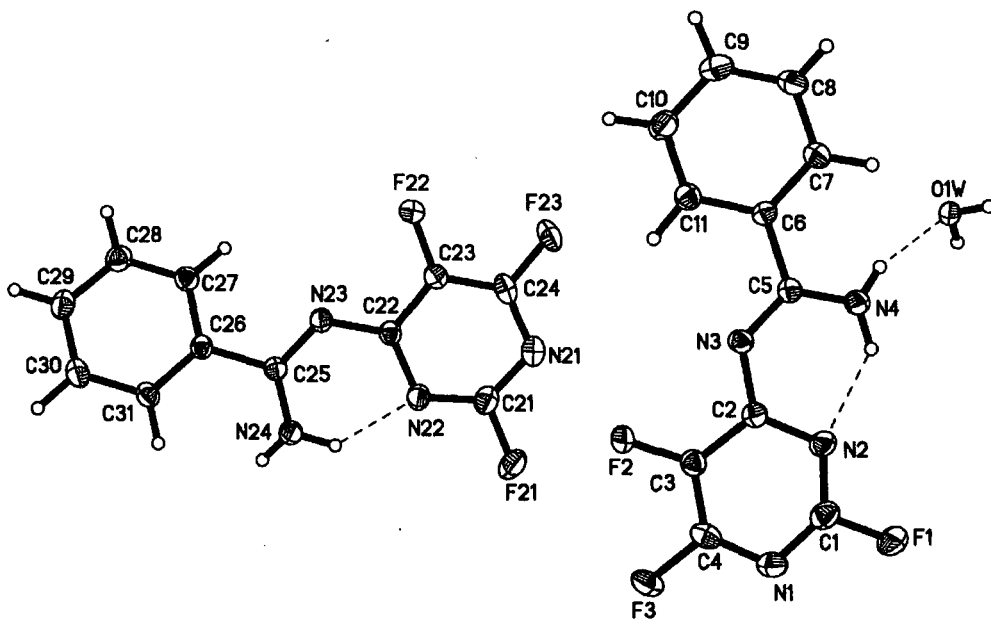
Figure 4.1 The x-ray crystallography structure of compound 330
