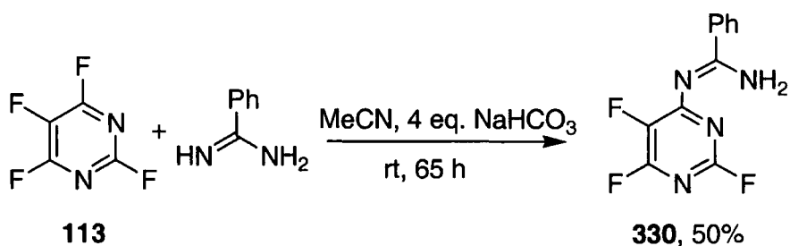
Scheme 4.2
