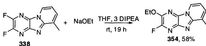
Scheme 5.23
