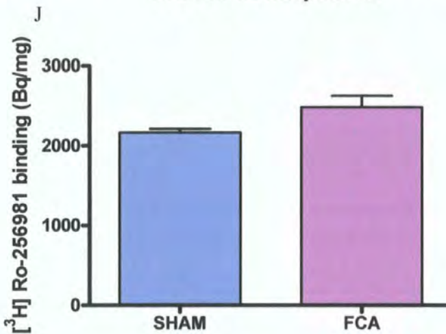
Figure 6.17 Autoradiographical data showing [ ^3\text{H} ] Ro-256981 binding within the whole brains of sham and FCA-treated animals.
