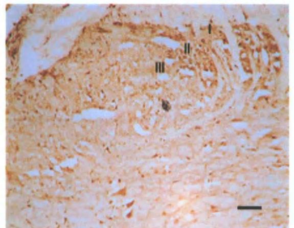
Figure 6.5 Expression of phosphorylated NR2A subunit at tyrosine 1387 in the dorsal horn of sham (A) and FCA (B) lumbar cord tissue. Initial evidence for increased phosphorylation of NR2A at tyrosine 1387 in the outer laminae (I, II and III) during the inflammatory response. Scale bar represents 100 \mu m.
