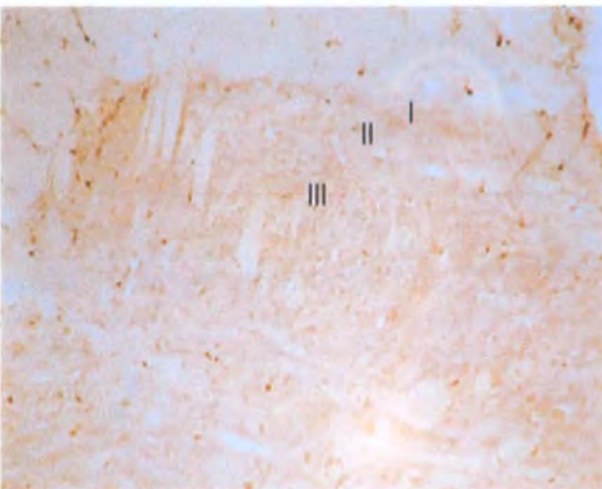
Figure 6.5 Expression of phosphorylated NR2A subunit at tyrosine 1387 in the dorsal horn of sham (A) and FCA (B) lumbar cord tissue. Initial evidence for increased phosphorylation of NR2A at tyrosine 1387 in the outer laminae (I, II and III) during the inflammatory response. Scale bar represents 100 \mu m.
