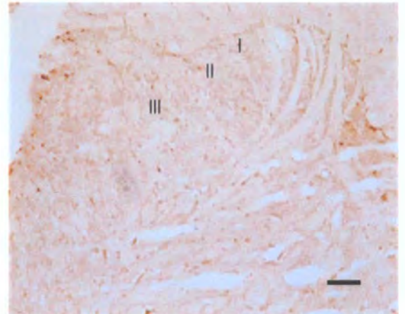
Figure 6.4 Expression of phosphorylated NR2A subunit at tyrosine residue 1325 in the dorsal horn of sham (A) and FCA (B) lumbar cord tissue. Weak immunoreactivity is present particularly in the outer laminae (I, II and III) of the dorsal horn. Scale bar represents 100 \mu m.
