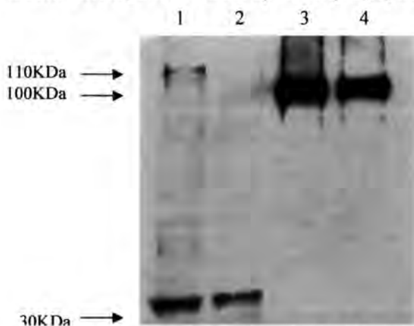
Figure 4.3 Immunoblot showing adult rat forebrain (1) and spinal cord (2) membranes (30µg) and recombinant NR3B expressed in HEK 293 cells (3+4), probed with anti-rodent NR3B (2µg/ml). Representative from n=3 experiments.
