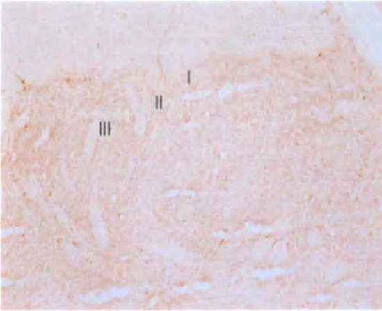
Figure 6.4 Expression of phosphorylated NR2A subunit at tyrosine residue 1325 in the dorsal horn of sham (A) and FCA (B) lumbar cord tissue. Weak immunoreactivity is present particularly in the outer laminae (I, II and III) of the dorsal horn. Scale bar represents 100 \mu m.
