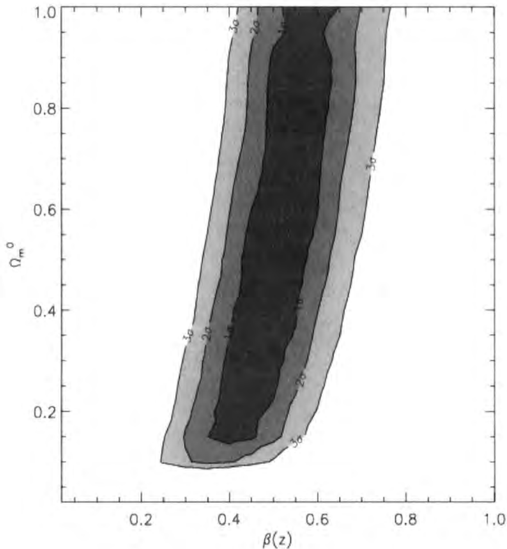
Figure 4.4: Likelihood contours of \Omega_m^0 - \beta(z = 0.55) using the geometric method of Alcock-Paczynski test and modelling the redshift-space distortions, assuming an EdS cosmology. The best-fit values are \Omega_m = 0.40^{+0.60}_{-0.25} and \beta = 0.45^{+0.20}_{-0.10} using a model with \gamma = 1.67 and a (starting) correlation length of r_0 = 5.65 h^{-1} Mpc. A value of \Omega_m \sim 1.0 lies within our 1\sigma contour but again there is a large degeneracy along the \Omega_m direction.
