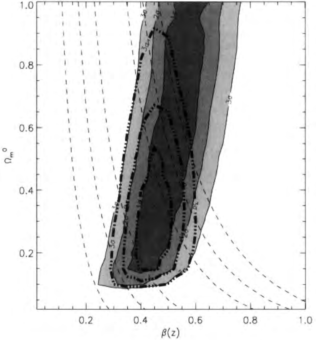
Figure 4.6: Joint likelihood contours for \Omega_m^0 - \beta(z = 0.55) using the geometric method of Alcock-Paczynski test, modelling the redshift-space distortions and including the evolution of clustering constraints, assuming an EdS cosmology. The joint best-fit has \Omega_m = 0.35 \pm 0.15 , \beta = 0.45 \pm 0.05 (marked with the cross) and a \langle w_z^2 \rangle^{1/2} of 330 \text{ km s}^{-1} . When the joint constraints are considered, a value of \Omega_m = 1.0 can be ruled out at the 3\sigma level.
