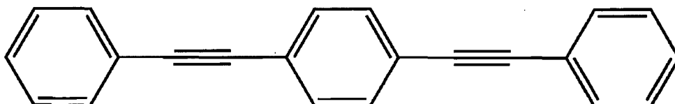
Figure 85: 4-Bis(phenylethynyl)benzene, (BPEB)
