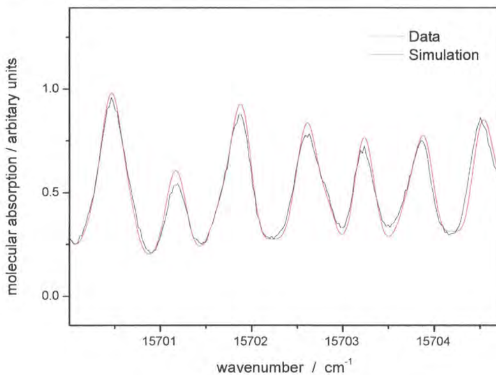
Figure 94: Shows overlap of individual peaks between simulation (red) and experimental (black).
