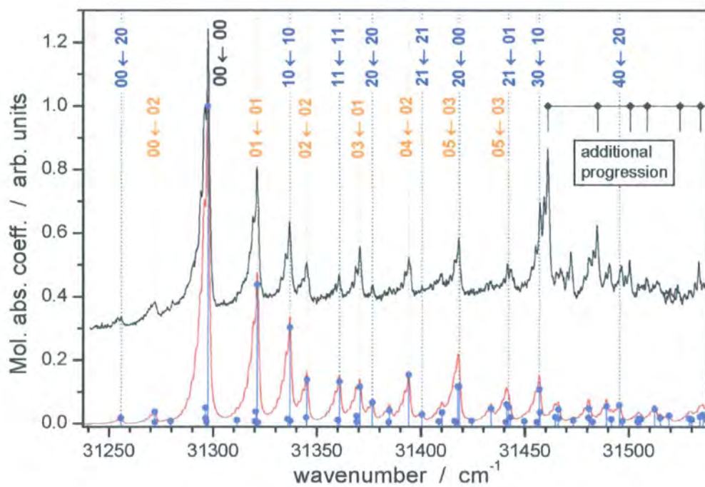
Figure 103: Upper: experimental and simulated spectra of BPEB. Lower: experimental and simulate spectra of DBPEB. The transitions of the main torsional progression are shown as vertical sticks with intensities shown by points. The most intense progressions are labeled in blue and orange ( \nu'_s \nu'_{as} \leftarrow \nu''_s \nu''_{as} ), where orange are pure anti-symmetric transitions and blue are transitions with symmetric contributions. The locations of additional torsional
