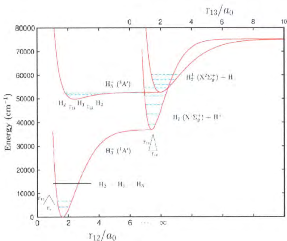
Figure 11: Energy diagram of the electronic energy levels of the H_3^+ system [60].
