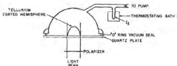
Figure 15: Photolysis Apparatus [96].
