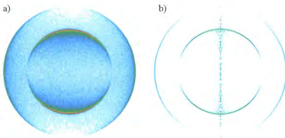
Figure 46: a) Raw ion image, rotated by 8.5^\circ and, b) 2D slice through the reconstructed 3D distribution.
