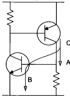
Figure 1.14: The operation of an SCR. If the resistance from point (A) to ground is decreased, less current will flow in to npn transistor base (B). Therefore the collector current from the pnp (C) will have to be increased to keep the SCR triggered.
