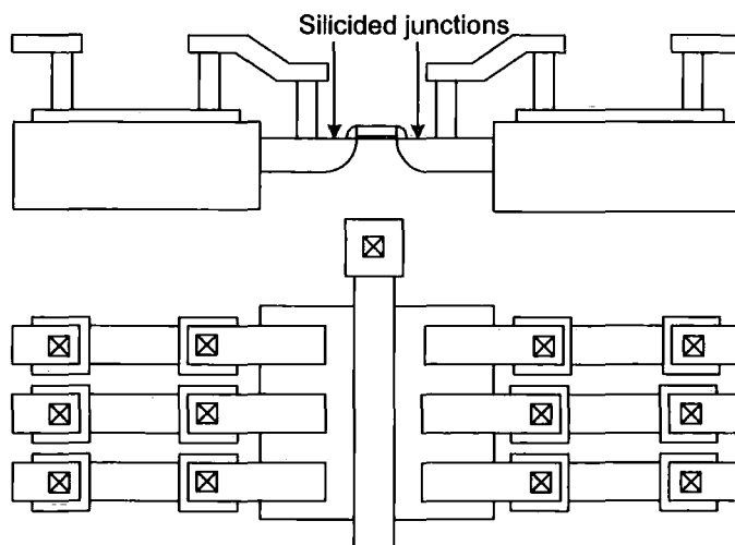
Figure 1.37: A hybrid solution based on the ideas illustrated in Figures 1.35 and 1.36 [3]
