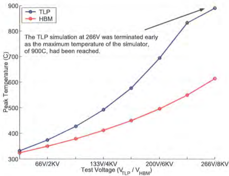
Figure 5.32: T_{MAX} for TLP and HBM simulations over a range of test energies
