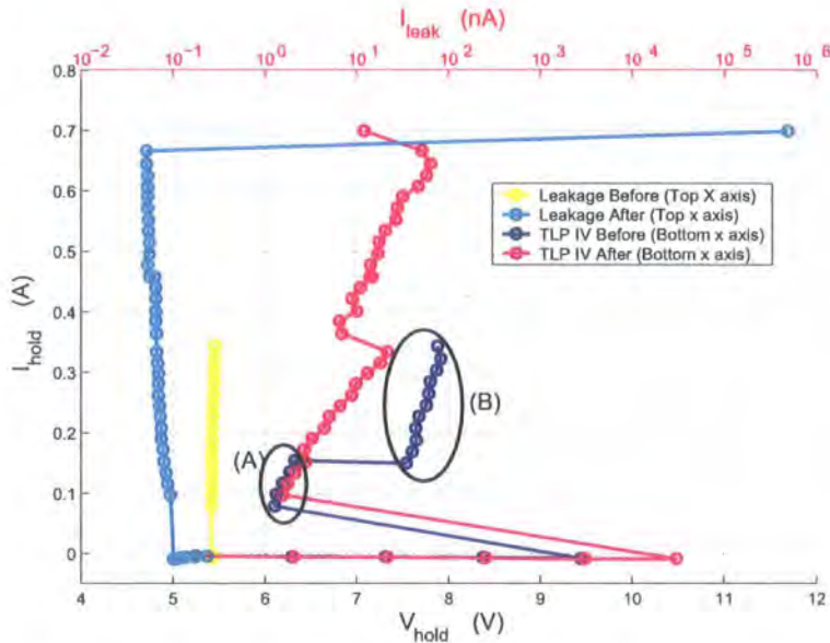
Figure 3.20: First IV curve of ggNMOS2 in parallel with the output drivers
