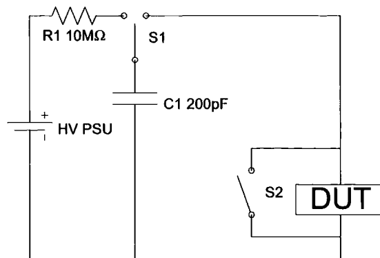
Figure 1.48: MM ESD test circuit
