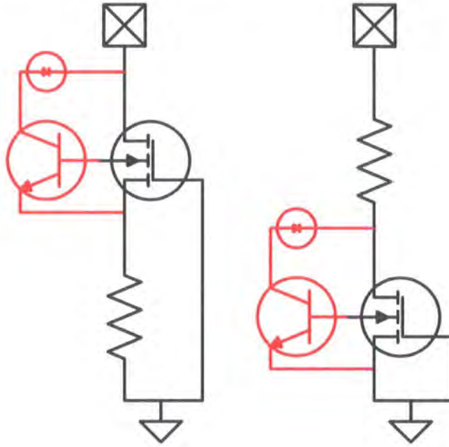
Figure 5.39: Extended source and extended drain ggNMOS schematic
