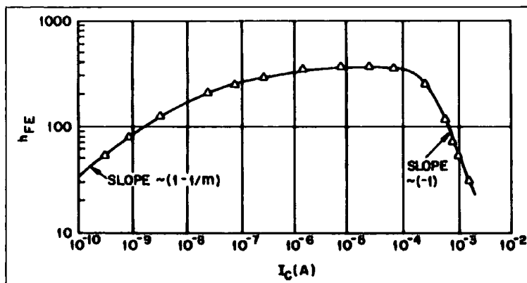
Figure 6.9: Variation in the bipolar current gain ( \beta ) as a function of I_{CE} for a bipolar transistor [5]
