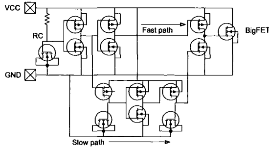
Figure 1.19: BigFET ESD solution with modified RC triggering circuit to minimise area consumption of the MOSCaps and eliminate the requirement for positive feedback
