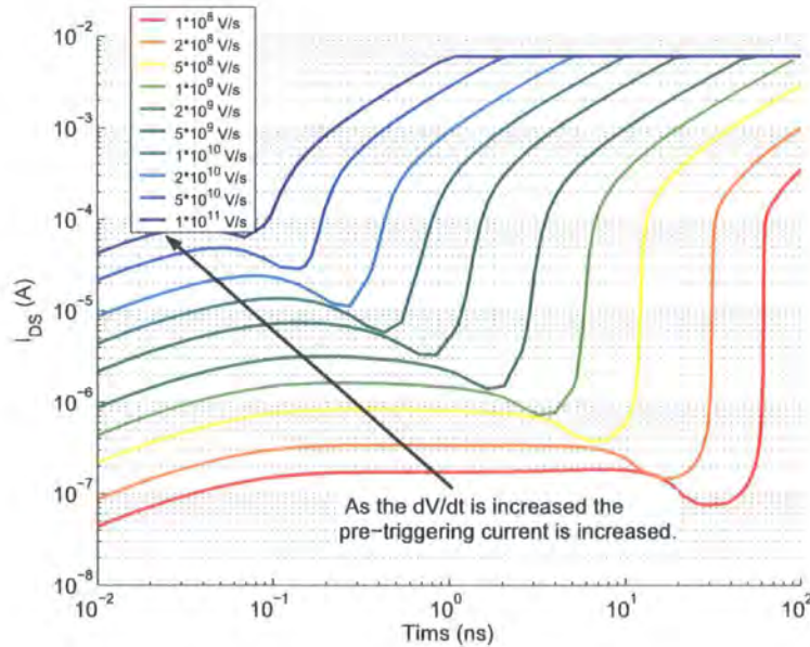
Figure 5.23: I_{DS} vs Time over a range of applied voltage ramps
