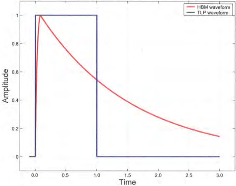
Figure 2.3: Normalised TLP and HBM waveforms
