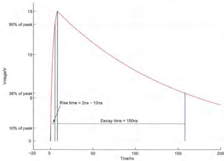
Figure 1.45: Current vs time for an HBM ESD event
