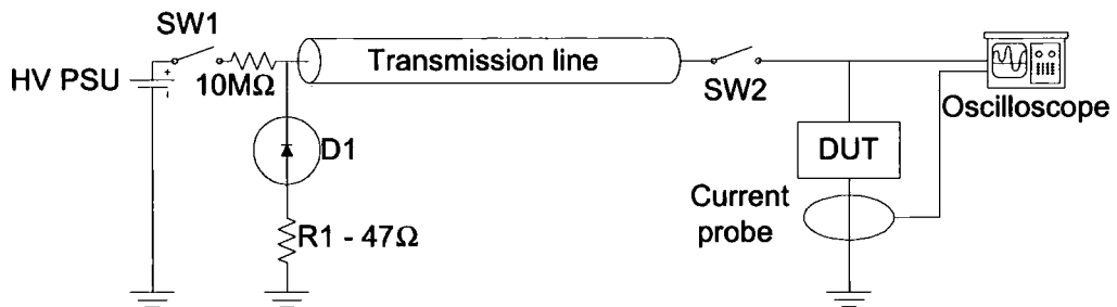
Figure 2.5: Constant impedance TLP tester
