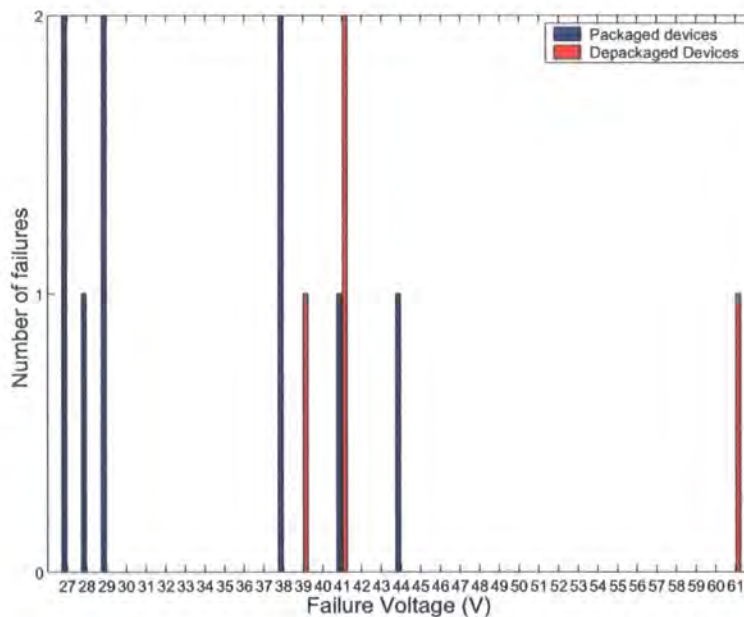
Figure 3.11: Number of failures vs Failure voltage of packaged and depackaged devices
