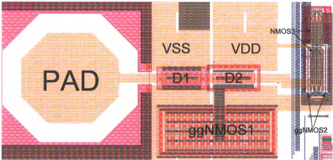
Figure 7.2: Layout of the output stage of the BC01b's TX_A identical to TX_B)
