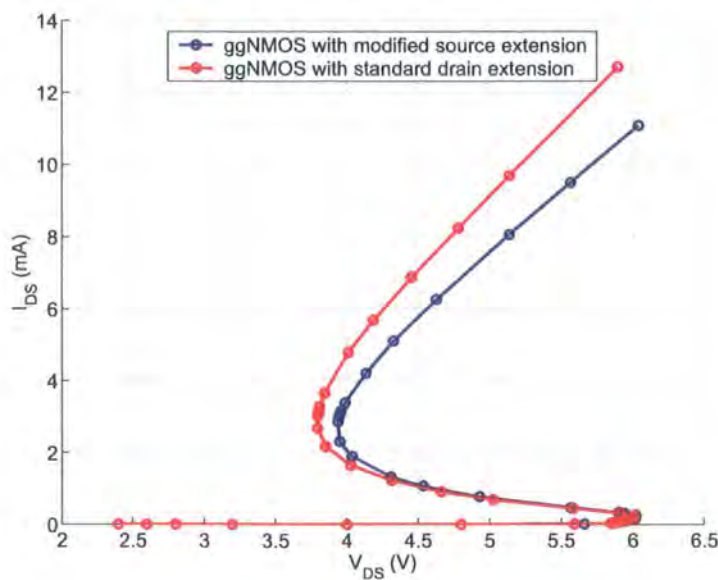
Figure 5.45: Extended source using a poly silicon resistor ggNMOS IV curves
