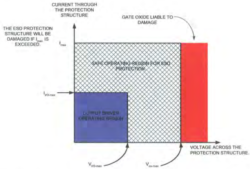
Figure 1.2: The safe operating area for an IO ESD protection circuit
