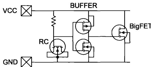
Figure 1.16: The basic concept of a BigFET ESD protection
