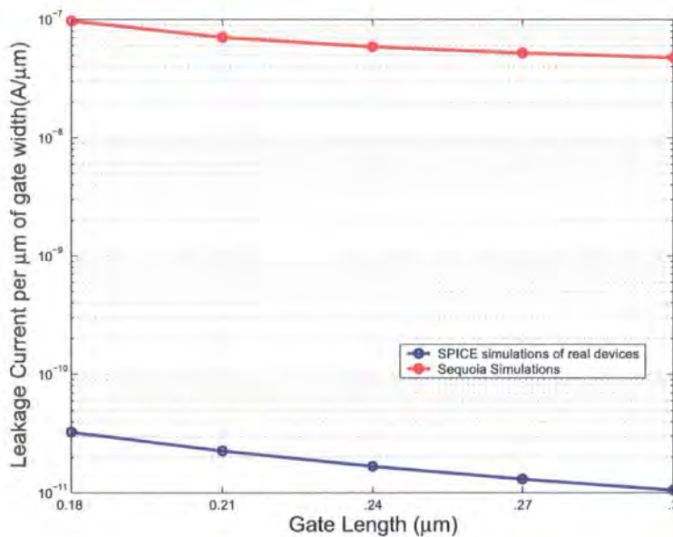
Figure 6.10: Comparison of the leakage current of a ggNMOS calculated using SPICE and Finite Element Simulation
