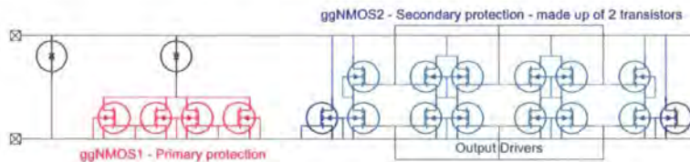
Figure 3.23: Output circuit of the BC01b showing each individual transistor including identical instances of transistors connected in parallel
