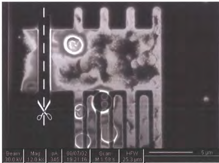
Figure 3.14: An image of the FIB cut to remove ggNMOS2 and the output drivers
