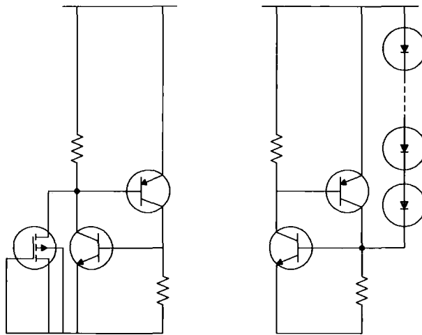
Figure 1.12: Left: This SCR is triggered by a small ggNMOS. Right: This SCR is triggered by the diode string
