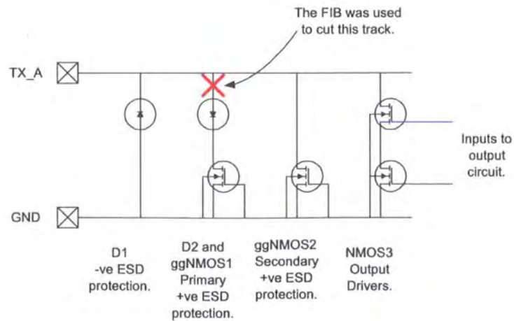
Figure 3.15: The position of the FIB cut to remove ggNMOS1
