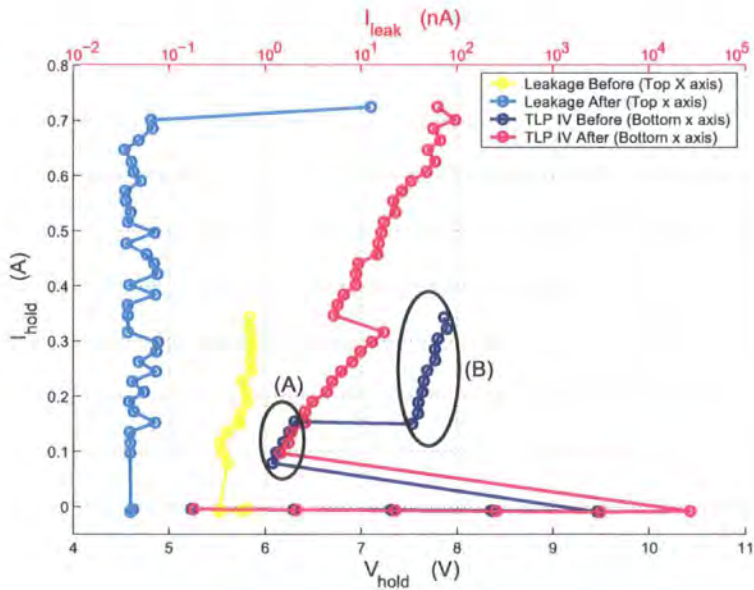
Figure 3.22: Third IV curve of ggNMOS2 in parallel with the output drivers
