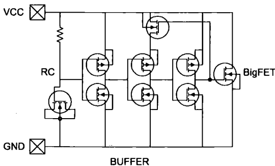
Figure 1.18: BigFET ESD solution with modified positive feedback to assist triggering and prevent power supply latchup
