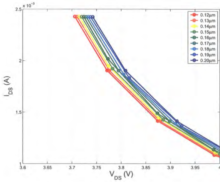
Figure 6.13: Detail from Figure 6.12 (hold voltage) of the IV characteristics of a modified ggNMOS
