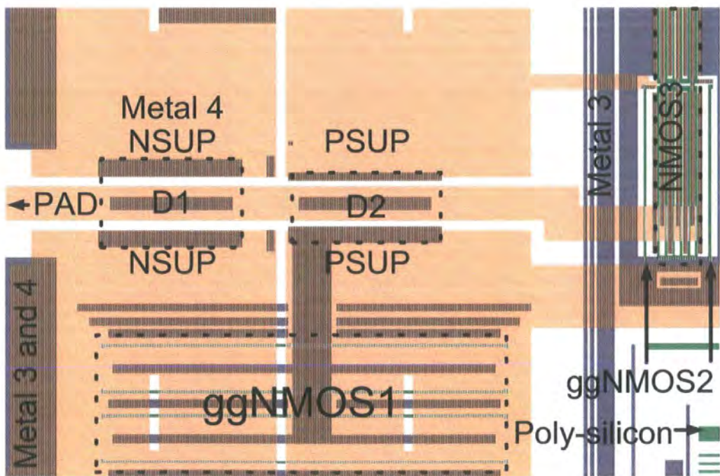
Figure 3.12: The layout of the metal layers in the output driver
