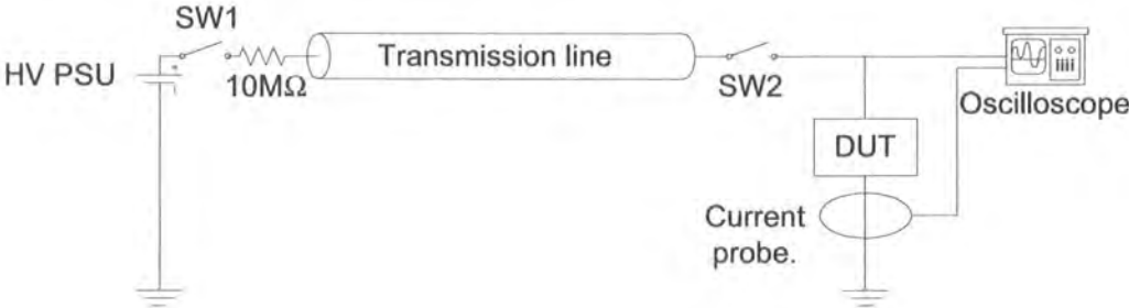
Figure 2.4: The basic set up of a TLP tester
