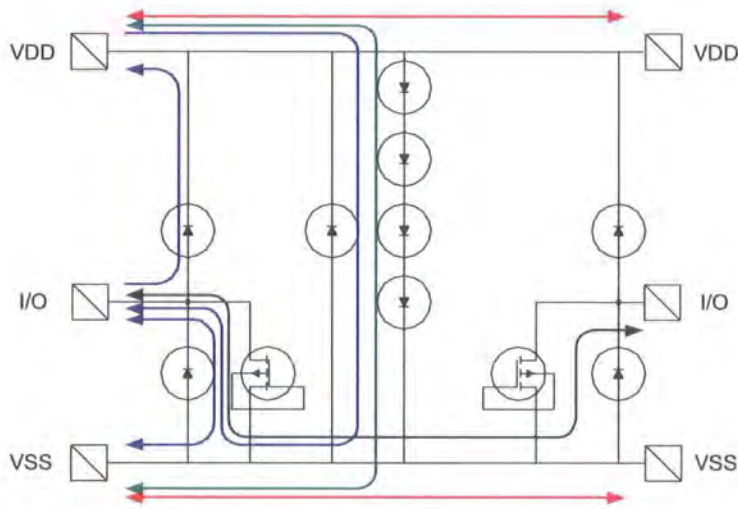
Figure 1.44: Current paths through a chip for all pin discharge combinations
