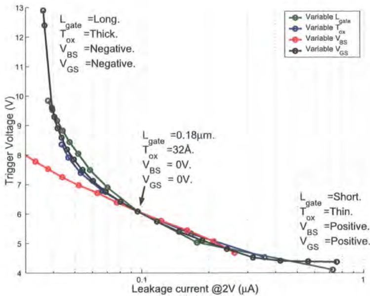
Figure 5.21: V_{t1} vs I_{leak} over a range of gate lengths, oxide thicknesses, gate biases and bulk biases
