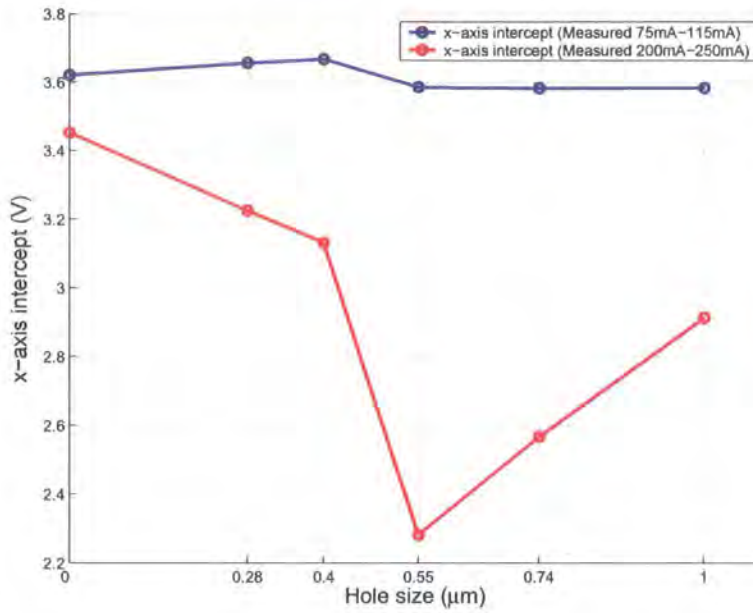
Figure 6.21: The voltage offset vs hole size of the ggNMOSs with holes in the extended drain
