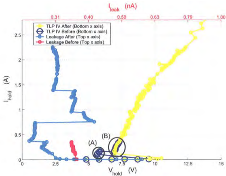
Figure 3.17: TLP IV curve of TX_A before and after ggNMOS2 and the output drivers were removed (first sample)
