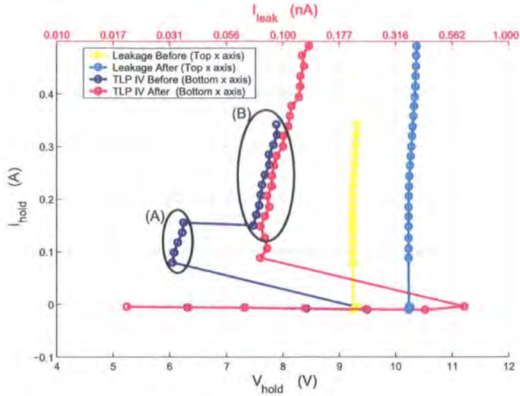
Figure 3.19: TLP IV curve of TX_A before and after ggNMOS2 and the output drivers were removed (second sample)
