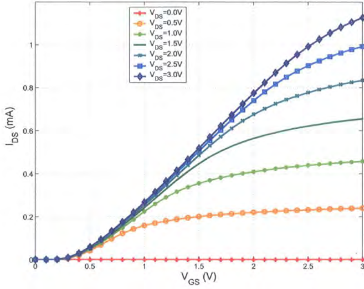
Figure 5.12: V_{GS} vs I_{DS} over a range of V_{DS}
