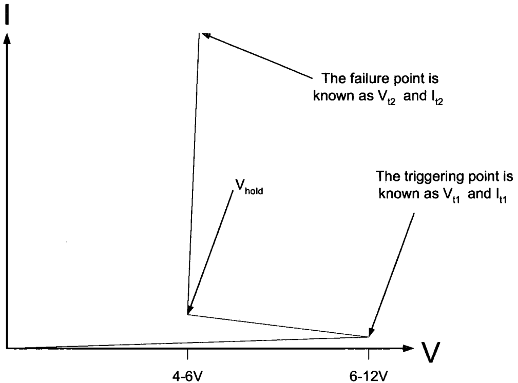
Figure 1.5: IV profile of a ggNMOS under ESD conditions
