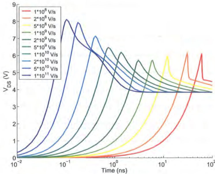
Figure 5.22: V_{DS} vs Time over a range of applied voltage ramps
