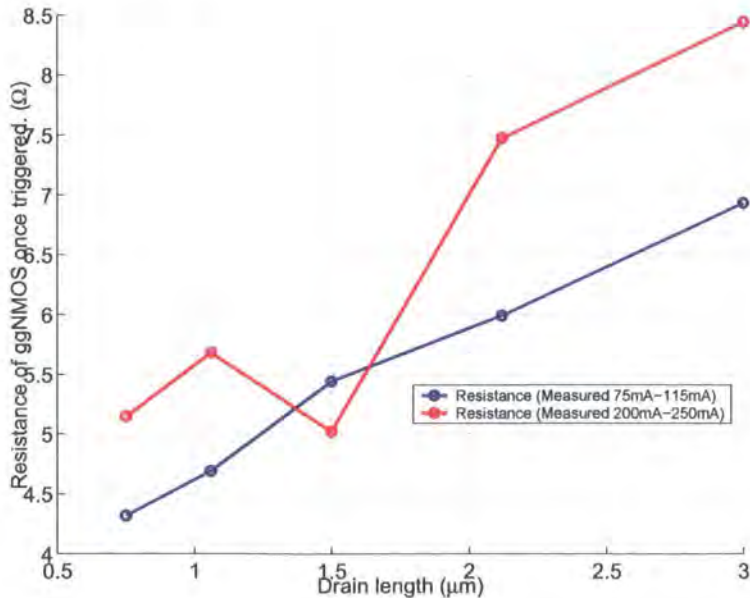
Figure 6.16: The resistance of the ggNMOS once the device is triggered over a range of drain lengths
