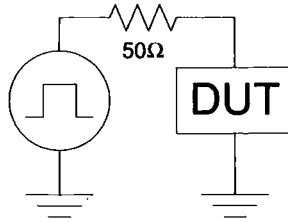
Figure 2.1: The basic concept of a TLP tester
