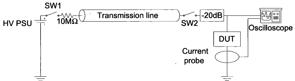
Figure 2.6: Constant impedance TLP tester with a 20db attenuator
