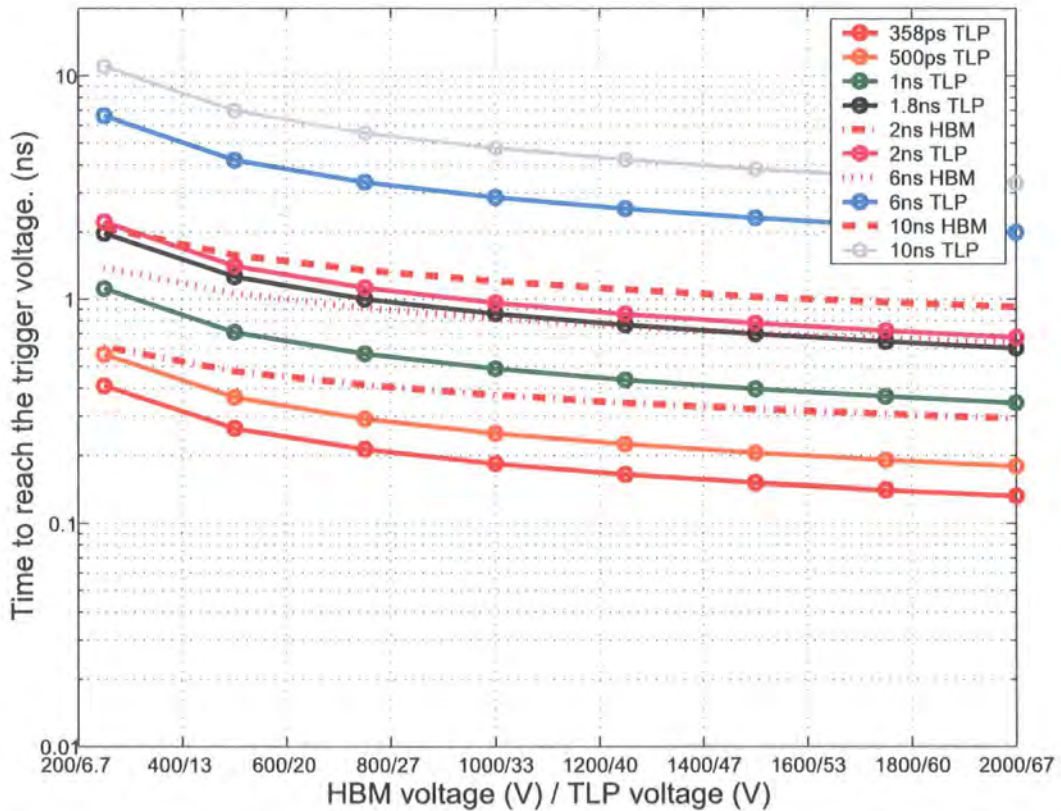
Figure 4.4: The time taken for a ggNMOS V_{DS} to reach 6V under TLP and HBM test conditions for a variety of rise times and amplitudes
