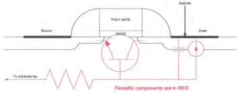
Figure 1.4: Location of the parasitic components in a typical deep sub-micron MOSFET
