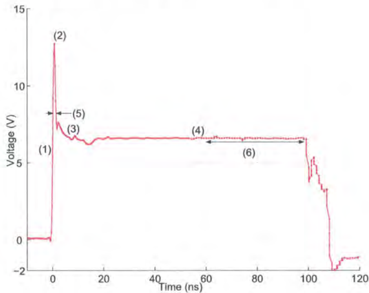
Figure 3.5: The voltage across the DUT vs time for a TLP- 50\Omega tester
