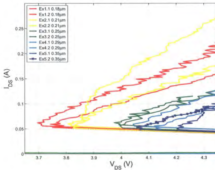
Figure 6.7: Detail of Figure 6.6 showing ggNMOS once triggered
