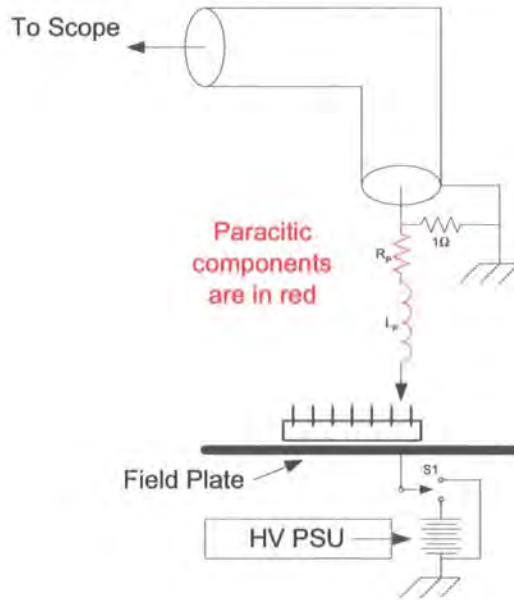
Figure 1.50: CDM ESD test circuit with parasitics
