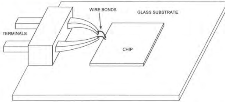
Figure 3.9: Depackaged chip mounted on a glass substrate
