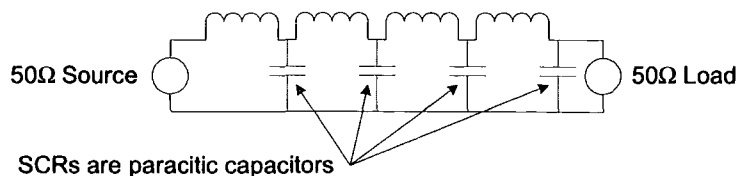
Figure 1.31: The use of inductors to mitigate the capacitive loading effect of a SCR to create a transmission line
