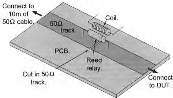
Figure 2.12: The physical construction of the output switch of the TLP tester
