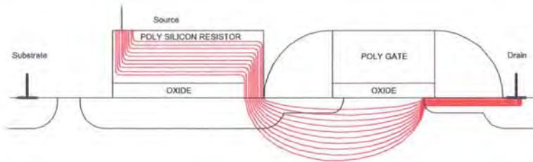
Figure 5.44: Extended source using a poly silicon resistor ggNMOS layout
