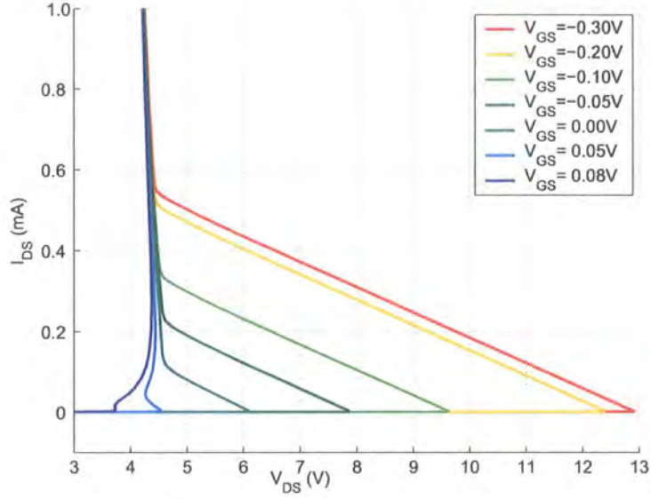
Figure 5.19: Sequoia simulation of V_{DS} vs I_{DS} over a range of V_{GS}
