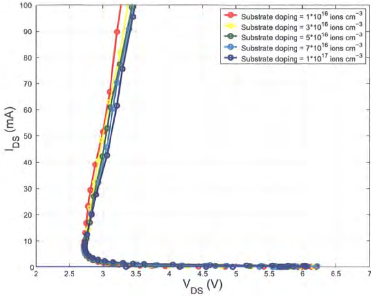
Figure 5.27: The ggNMOS IV profile for different substrate doping
