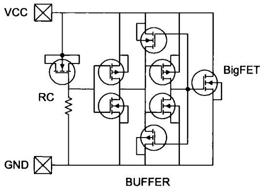
Figure 1.17: BigFET ESD solution with positive feedback to assist triggering
