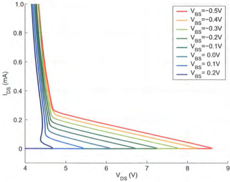
Figure 5.20: Sequoia simulation of V_{DS} vs I_{DS} over a range of V_{BS}
