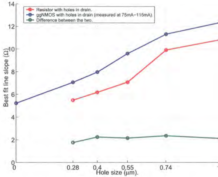
Figure 6.23: Resistance of ggNMOS and standard resistors for different active hole sizes
