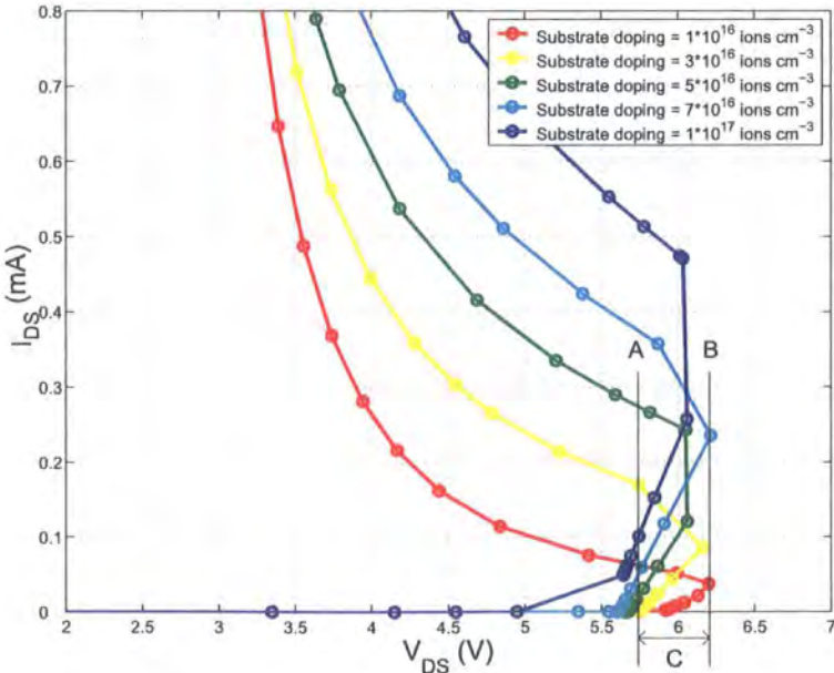
Figure 5.28: Triggering detail from Figure 5.27
