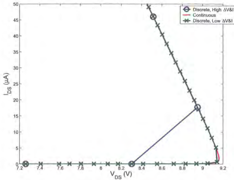
Figure 5.31: Improvement of the simulation accuracy due to the decrease in simulation step size
