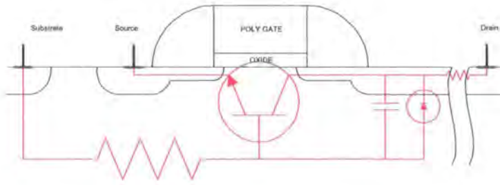
Figure 1.33: The location of parasitics and drain extension design modification
