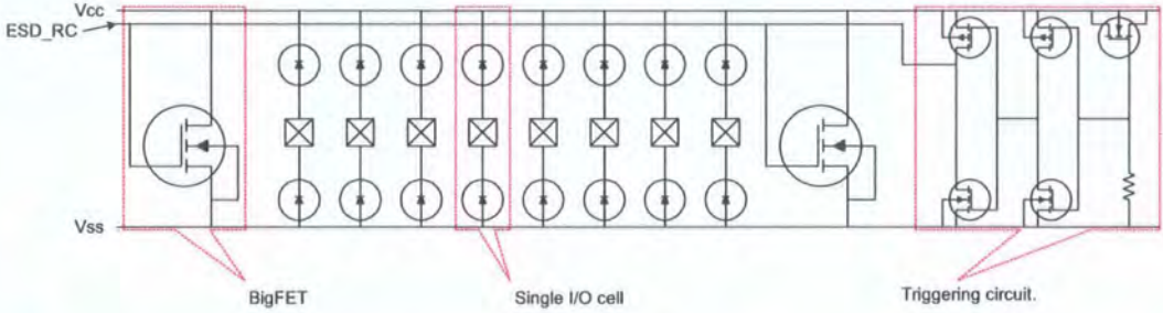
Figure 1.23: The use of a few BigFETs to protect a large number of IOs
