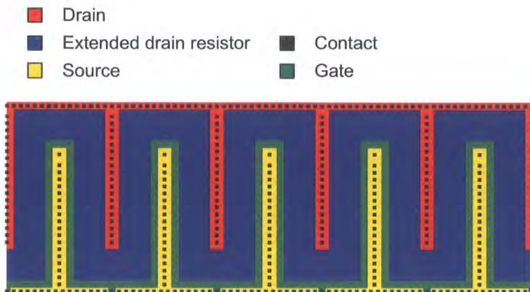
Figure 7.5: Suggested layout for single finger construction ggNMOS with multiple gate taps and efficient silicon area usage
