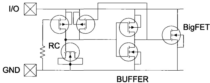
Figure 1.22: Feedback can be used to reduce leakage whilst the protection structure is inactive
