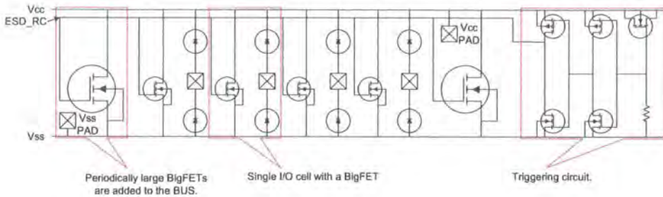
Figure 1.25: The triggering of distributed BigFETs by a single ESD detecting circuit
