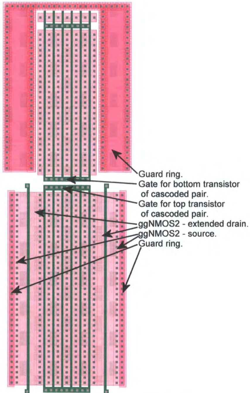
Figure 7.4: Detail from Figure 7.2 showing ggMOS2 ESD protection and ggNMOS3 output drivers
