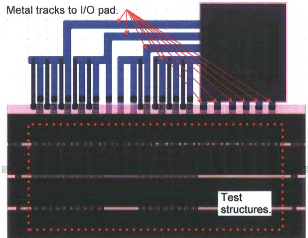
Figure 6.2: A close up of the ggNMOS test structures
