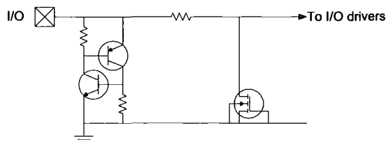
Figure 1.27: The use of an n-well resistor, SCR and a ggNMOS to create a hybrid ESD protection solution
