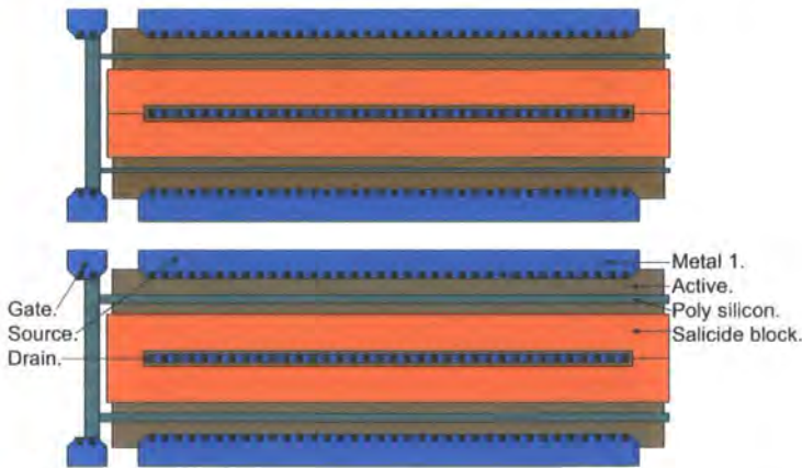
Figure 6.5: The layout of a 0.18\mu\text{m} (top) and 0.35\mu\text{m} (bottom) version of the 1st set of test structures with variable gate length
