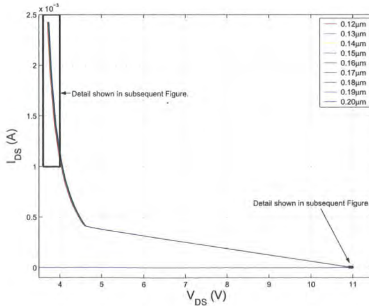
Figure 6.12: IV characteristics of a modified ggNMOS
