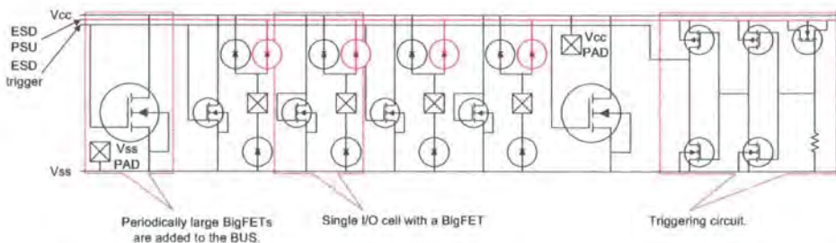
Figure 1.26: The use of a separate ESD detection circuit power supply bus to mitigate the effect of bus resistance
