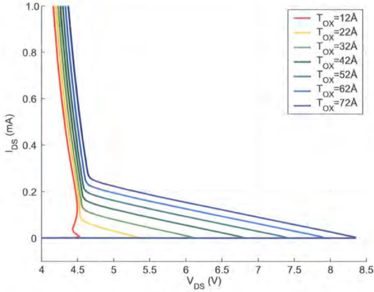
Figure 5.18: Sequoia simulation of V_{DS} vs I_{DS} over a range of T_{ox}
