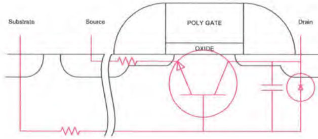
Figure 5.16: The parasitic components in a ggNMOS required to cause snapback
