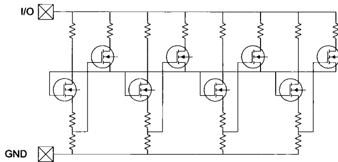
Figure 1.41: The second MFT design. The increase V_{source} in a triggered device is used to reduce the triggering voltage of subsequent devices and therefore propagate triggering.
