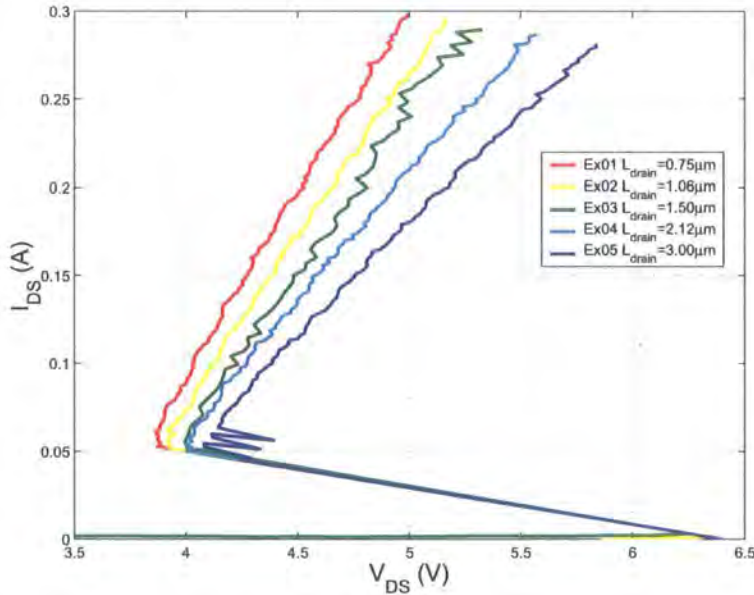
Figure 6.15: IV curves of the test ggNMOS's with variable drain lengths
