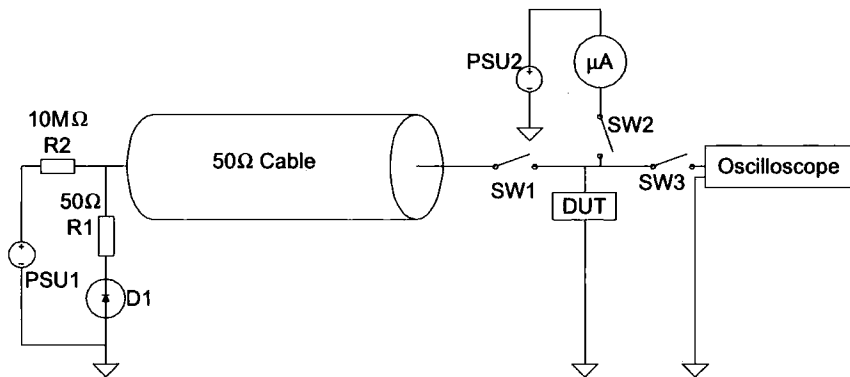
Figure 2.11: TLP tester schematic
