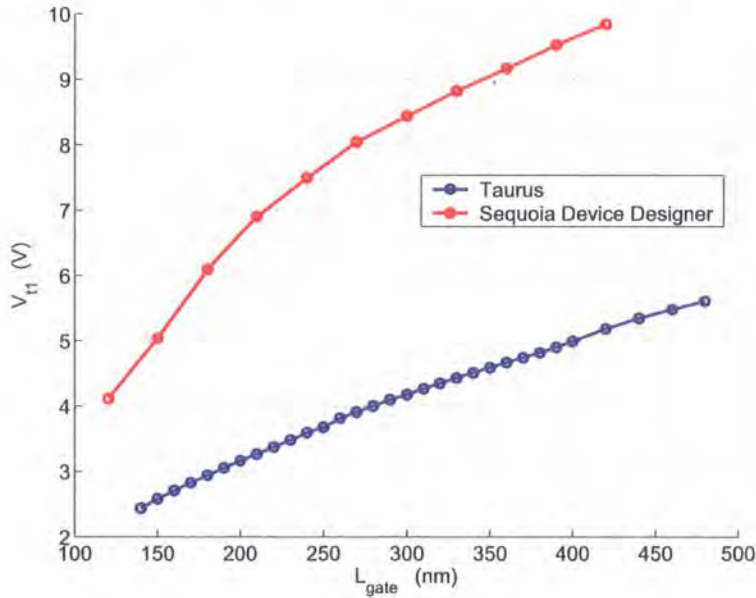
Figure 5.17: The V_{t1} vs L_{gate}
