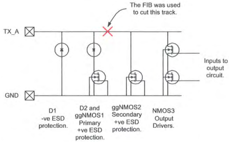
Figure 3.13: The position of the FIB cut to remove ggNMOS2 and the output drivers
