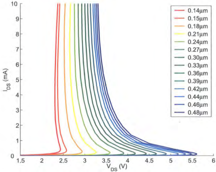
Figure 5.14: Taurus snapback simulation of V_{DS} vs I_{DS} over a range of L_{gate}
