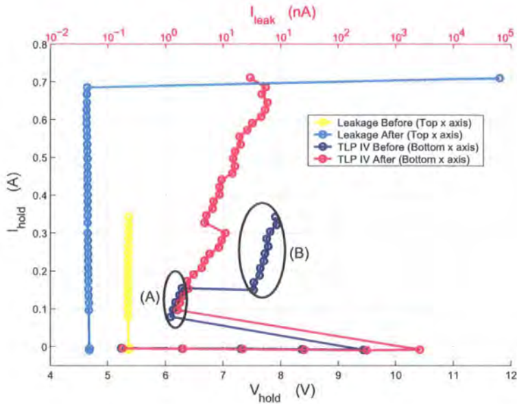
Figure 3.21: Second IV curve of ggNMOS2 in parallel with the output drivers
