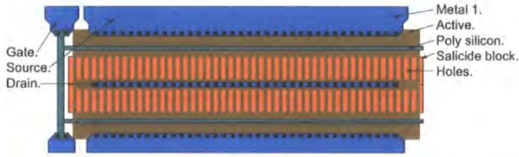
Figure 6.18: The layout of a ggNMOS with holes in the extended drain
