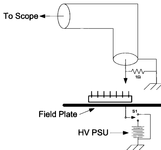
Figure 1.49: CDM ESD test circuit
