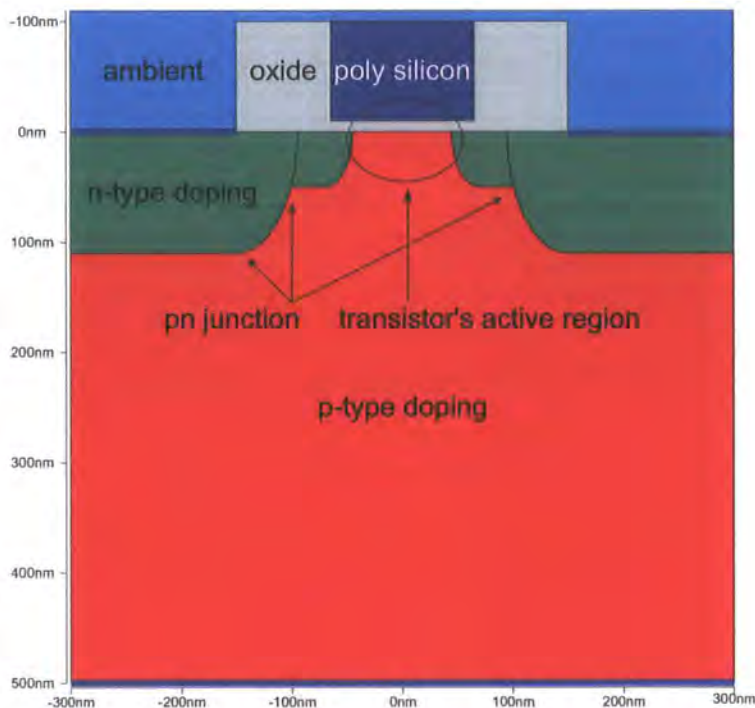
Figure 5.2: The parts of the transistor that require High Grid Density for Finite Element Simulation
