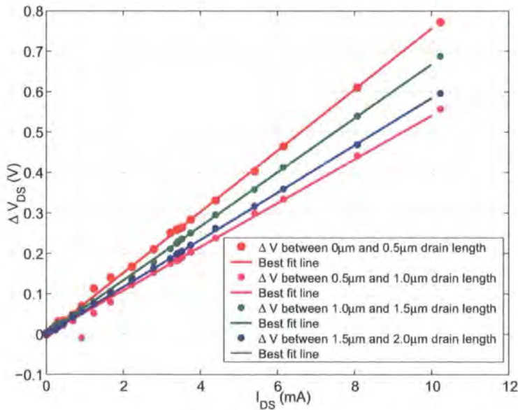
Figure 5.36: Change in V_{DS} for structures with different drain lengths
