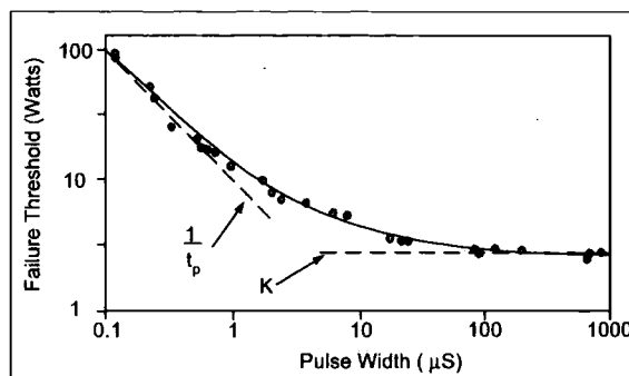
Figure 1.29: Variation of the failure power threshold in relation to the pulse width for a metal track [1]
