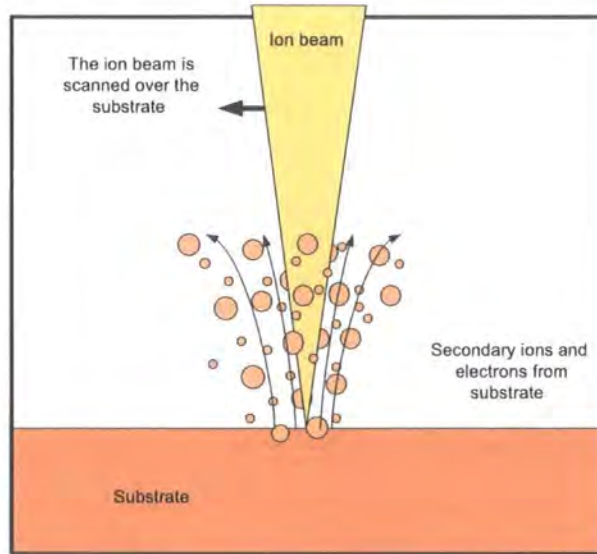
Figure 3.2: The principle of FIB imaging [4]
