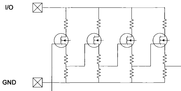
Figure 1.39: The first MFT design where the increased V_{source} is used to increase V_{GS} on the next device and hence propagate triggering
