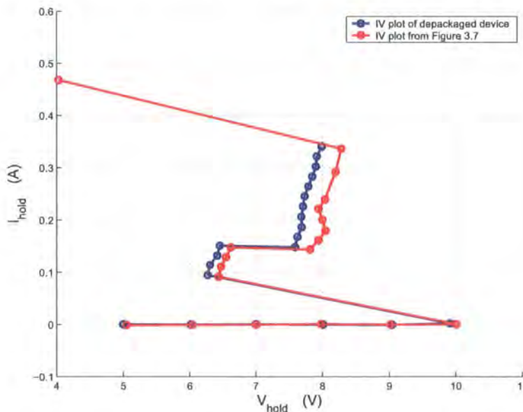
Figure 3.10: IV plot of a depackaged device
