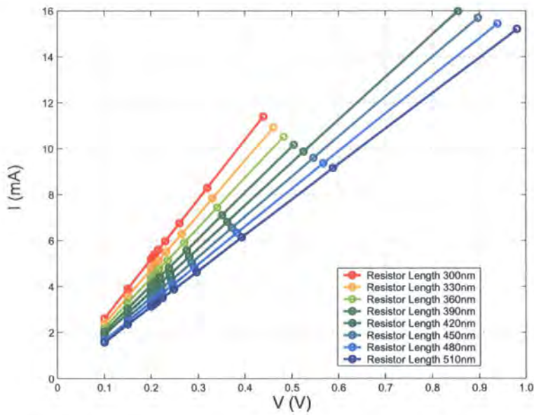
Figure 5.37: IV characteristics of an n-well resistor
