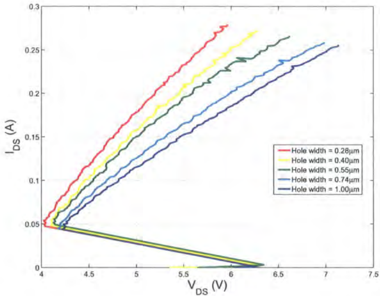
Figure 6.19: The IV characteristics of the ggNMOSs with holes in the extended drain
