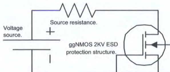
Figure 4.3: The SPICE simulation circuit so that the actual device \frac{dV}{dt} can be derived
