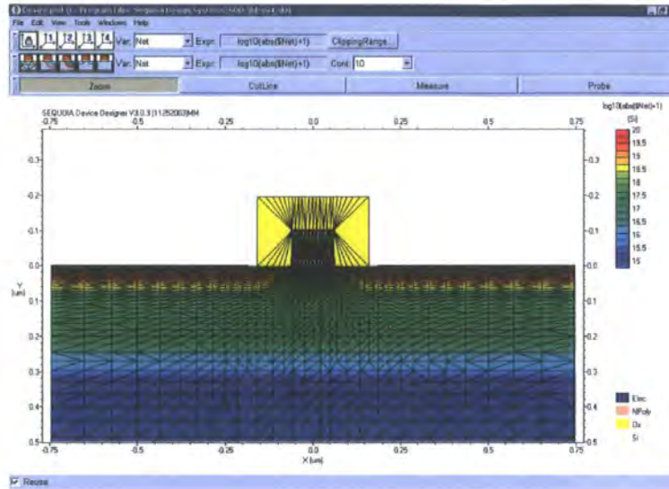
Figure 5.5: A typical MOSFET structure with the finite element grid overlaid
