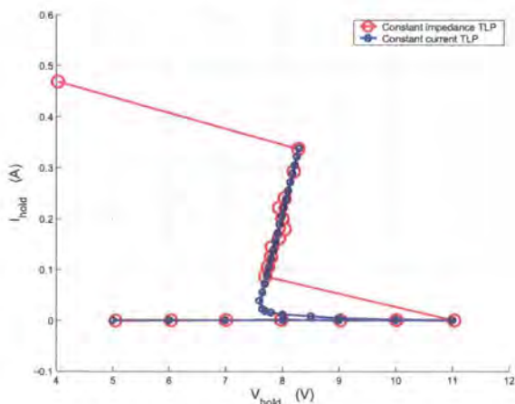
Figure 2.9: Comparison of an IV trace of a ggNMOS using a 50\Omega TLP tester and a constant current TLP tester
