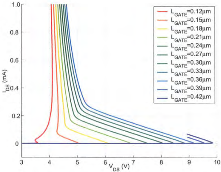
Figure 5.15: Sequoia simulation of V_{DS} vs I_{DS} over a range of L_{gate}
