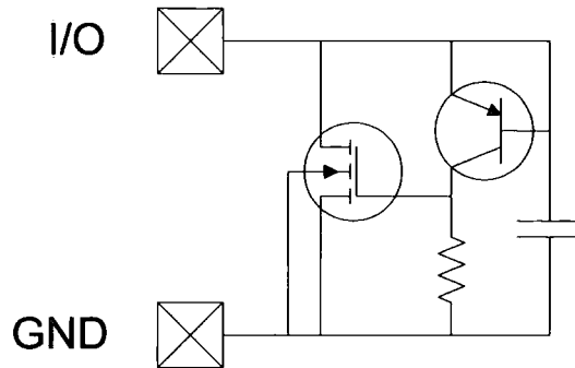
Figure 1.40: The use of an RC based circuit to decrease the triggering voltage of a ggNMOS during an ESD event
