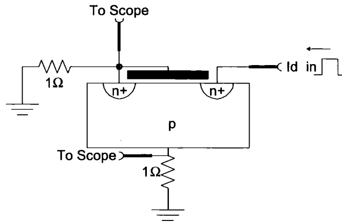
Figure 2.10: The use of a TLP tester to measure the substrate currents during an ESD event
