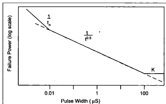
Figure 1.30: The Wunsch-Bell curve for failure due to IR heating [1]
