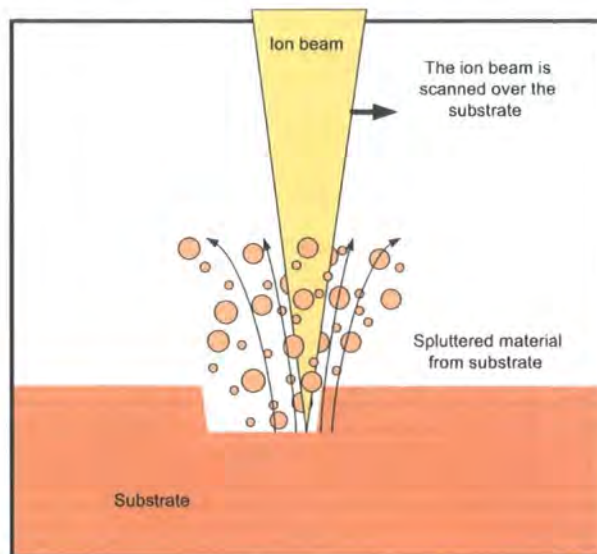
Figure 3.3: The principle of FIB milling [4]
