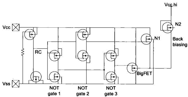
Figure 1.21: Back biasing can be disabled during an ESD event to improve ESD performance
