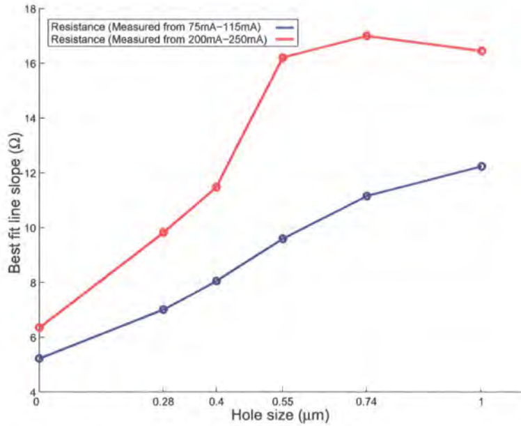
Figure 6.20: The drain resistance vs hole size of the ggNMOSs with holes in the extended drain
