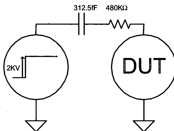
Figure 5.8: Graphical illustration of the application of an HBM pulse in a simulation
