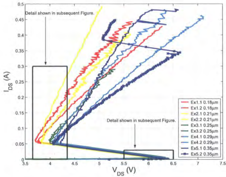
Figure 6.6: IV curves of the test ggNMOS's with variable gate lengths
