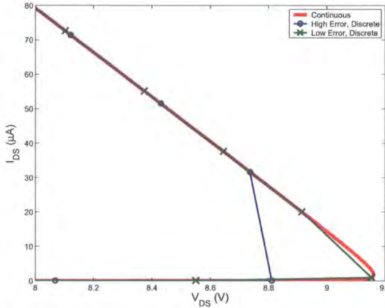
Figure 5.30: Error in peak voltage measurement caused by simulation step size
