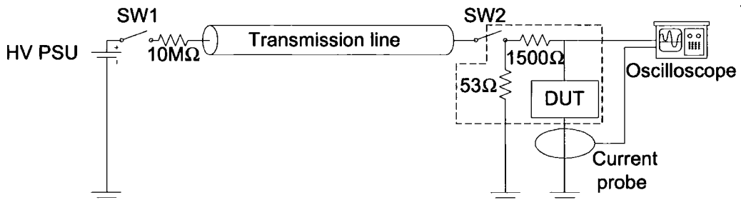
Figure 2.7: Constant current TLP tester
