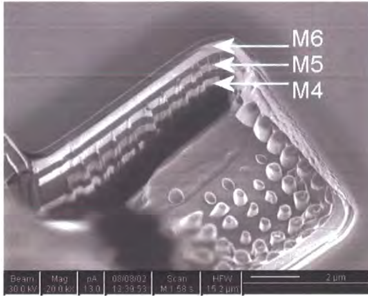
Figure 3.16: An image of the FIB cut to remove ggNMOS1; M4 is used to connect ggNMOS1 to the output
