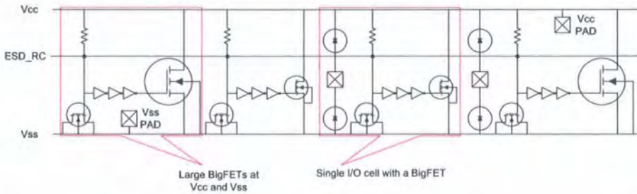
Figure 1.24: The distribution of BigFETs along a chain of IOs to mitigate the effects of bus resistance
