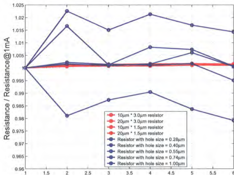
Figure 6.22: Change in measured Resistance vs Current
