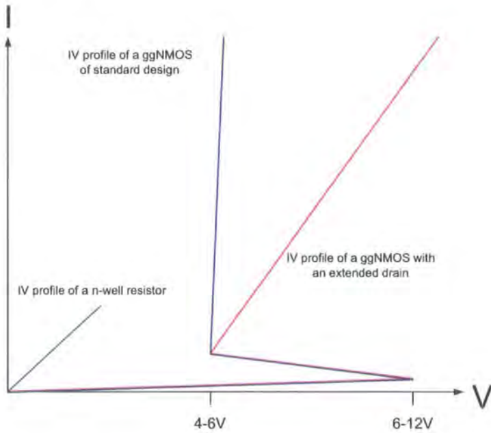
Figure 1.34: The IV profile of an unmodified and modified (drain extended) ggNMOS silicon area consumed by the ggNMOS as well as the parasitic capacitance and alter the triggering voltage of the device whilst maintaining a high I_{t2} .
