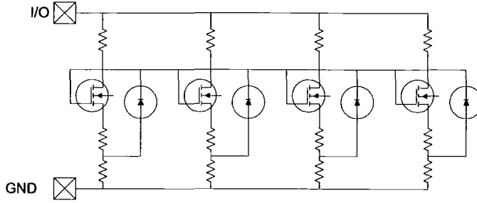
Figure 1.42: The third MFT design. The increase V_{source} in a triggered device is used to reduce the triggering voltage of subsequent devices and therefore propagate triggering.
