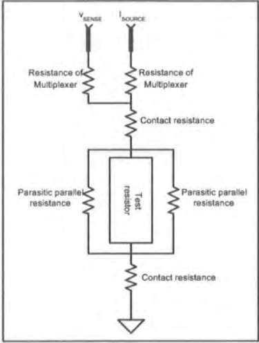
Figure 6.24: The location of the parasitics around the test resistors
