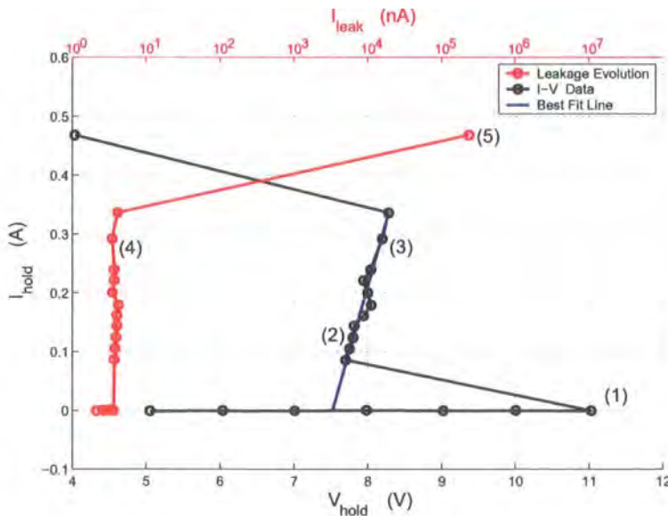
Figure 3.6: Example of a ggNMOS IV plot derived from TLP testing
