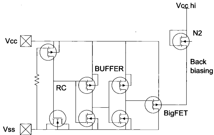
Figure 1.20: The use of back biasing to reduce leakage current in a BigFET
