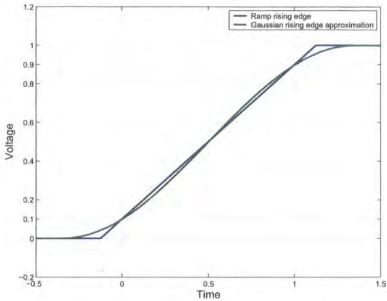
Figure 4.1: Two possible normalised rising edge profiles for a TLP or HBM pulse and an HBM pulse respectively. t_{6V-TLP} and t_{6V-HBM} are the time taken for a 66V TLP pulse and a 2KV HBM pulse respectively to reach 6V. The HBM rise time ( t_{R-HBM} ), as defined by JEDEC [6], ranges between 2ns and 10ns and the TLP rise time ( t_{R-TLP} ) needs to be calculated such that they both reach 6V at the same time (i.e. t_{6V-TLP} = t_{6V-HBM} ).
