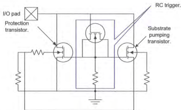
Figure 1.38: RC triggered nMOS switch which pumps the substrate of the protection transistor to assist triggering
