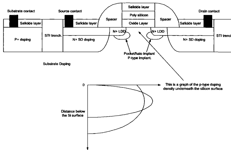
Figure 5.9: The structure of an nMOS transistor
