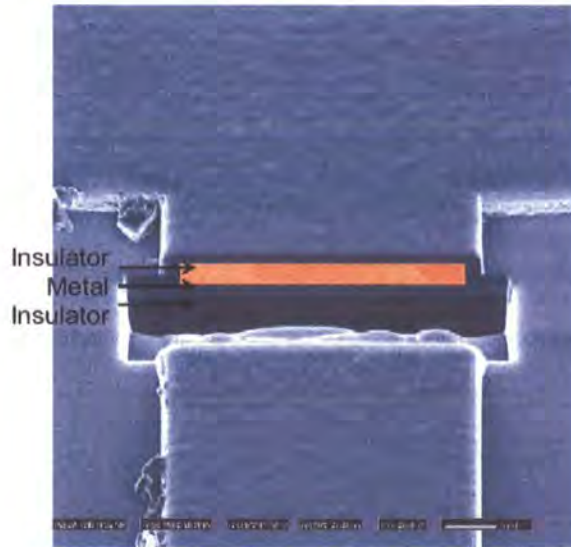
Figure 3.4: An example of milling where a metal track is cut [4]
