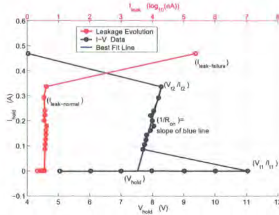
Figure 2.8: Example IV trace of a ggNMOS using a TLP tester
