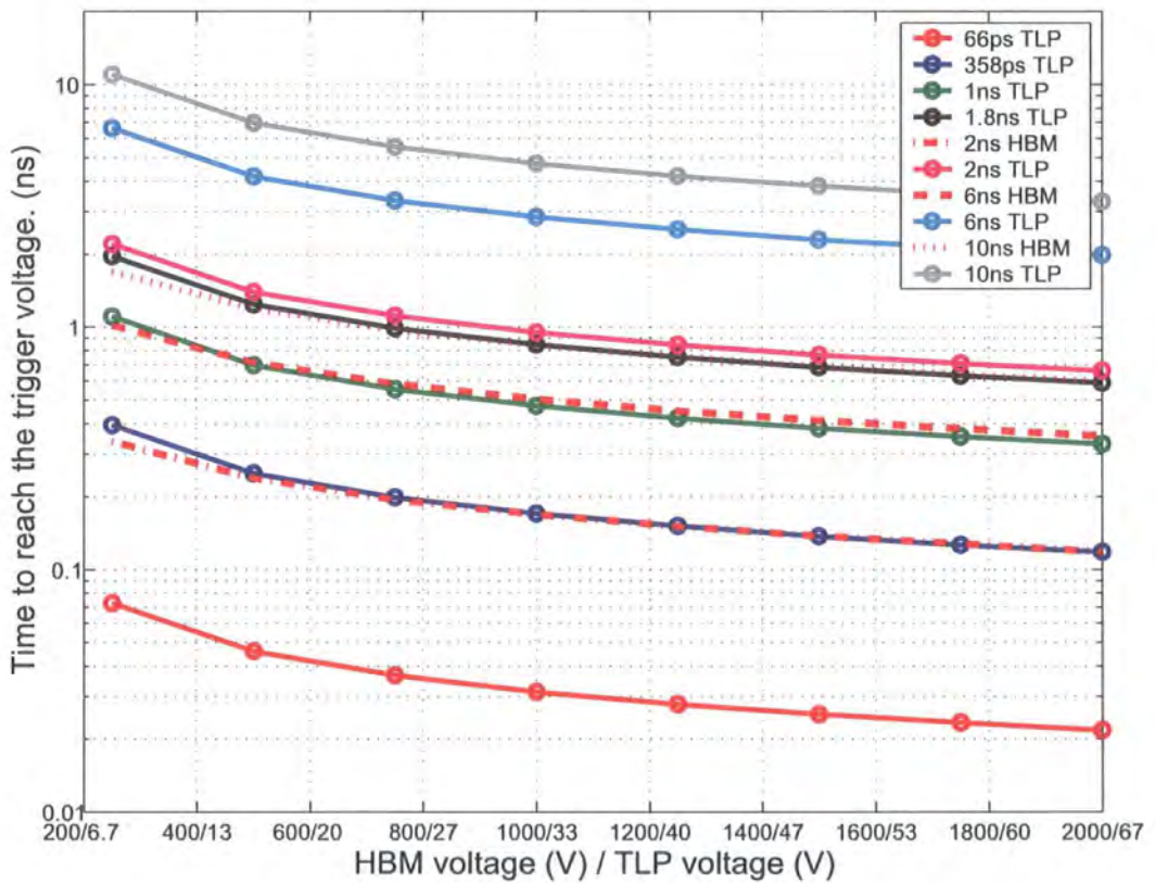
Figure 4.2: The time taken for an HBM or TLP source to reach 6V for a variety of rise times and amplitudes
