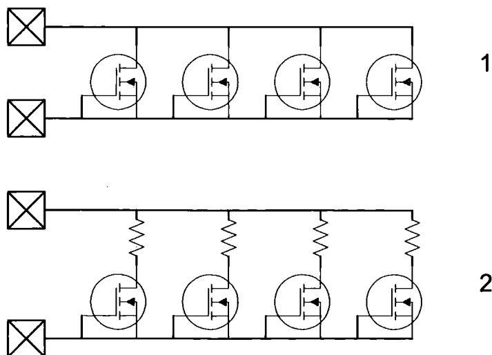
Figure 5.33: The effect an extended drain has on a ggNMOS
