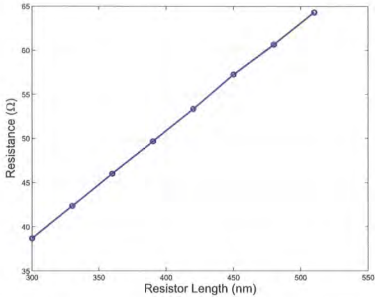
Figure 5.38: Resistance of the n-well resistors vs length
