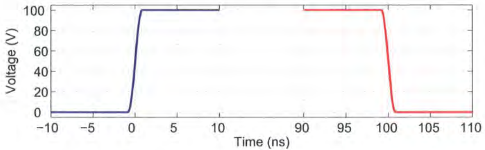
Figure B.1: The voltage characteristics of a TLP waveform with t_R and t_F of 1ns and a duration of 100ns
