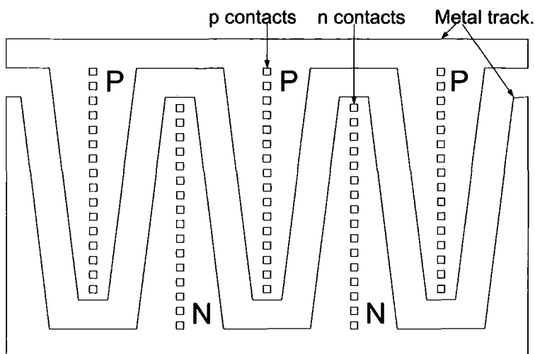
Figure 1.8: Suggested layout of metal tracks to achieve a constant current density and minimise capacitance in a pn junction
