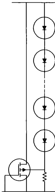
Figure 1.11: The use of diodes to pump the substrate of a ggNMOS to assist triggering
