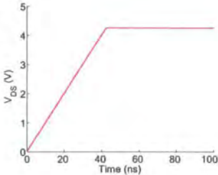
Figure 5.24: 10^8 V/s voltage ramp with a voltage limit of 4.25V
