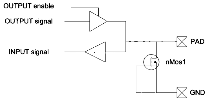
Figure 1.1: An IO circuit with ESD protection
