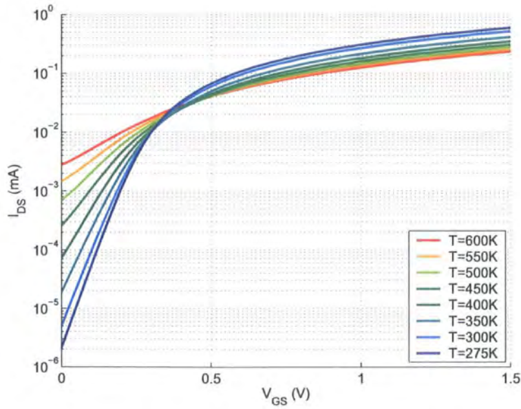
Figure 5.13: V_{GS} vs I_{DS} over Temperature
