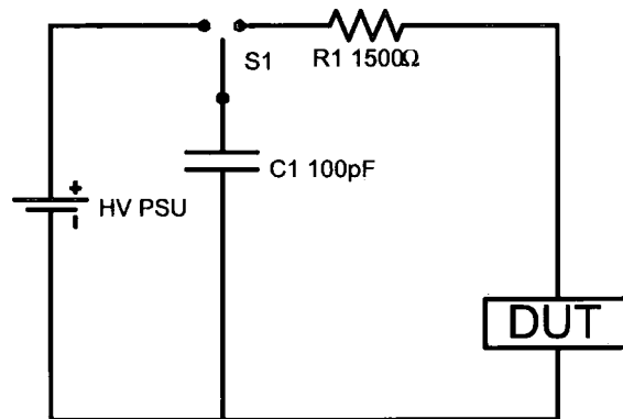
Figure 2.2: HBM ESD tester schematic
