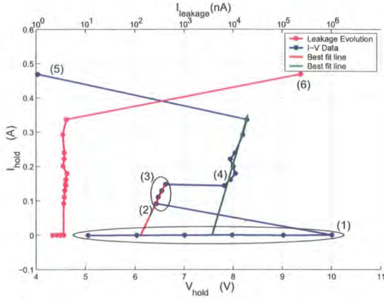
Figure 3.7: IV curve and I_{hold} vs I_{leak} for the BC01b derived from a TLP 50 \Omega tester the current is increased but the hold voltage only rises slightly (3); this increase in V_{hold} is due to the series resistance on the protection device. At (4) the hold voltage rises significantly to 7.81V, which naturally decreases the hold current as the TLP impedance is 50 \Omega . Again, any further increases in TLP energy cause small increases in V_{hold} and the series resistance of the protection structure. The data point at (5) indicates that permanent damage has occurred to the output. This can be confirmed by looking at the leakage current which increased significantly after the last TLP pulse (6).
