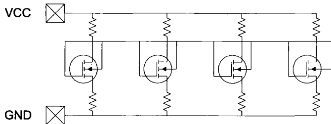
Figure 1.43: The use of substrate pumping principles to propagate triggering between devices
