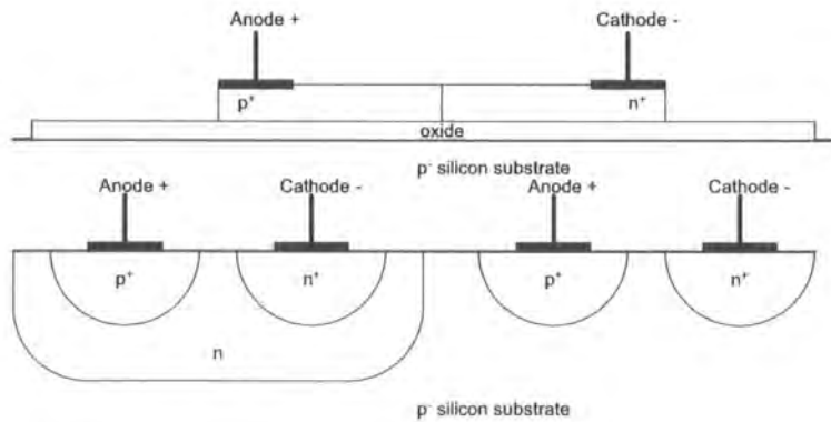
Figure 1.7: Top: Diode made in polysilicon. Bottom: Diodes made using wells in a p^- substrate
