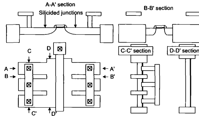
Figure 1.36: Modified drain extension resistor in a ggNMOS used to increase the resistance per unit area [3]
