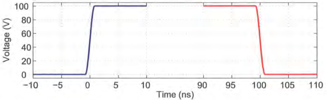
Figure 5.6: The voltage characteristics of a TLP waveform with t_R and t_F of 1ns and a duration of 100ns
