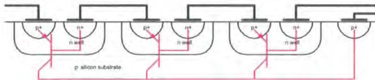
Figure 1.10: The location of the parasitic bipolar transistors found in a series of well diodes. These parasitic structures amplify any leakage current produced by the diodes.
