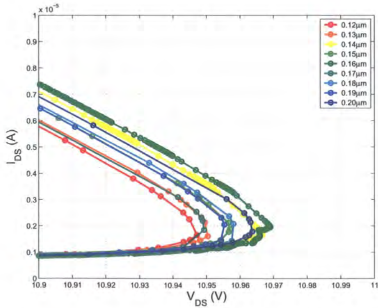
Figure 6.14: Detail from Figure 6.12 (triggering voltage) of the IV characteristics of a modified ggNMOS
