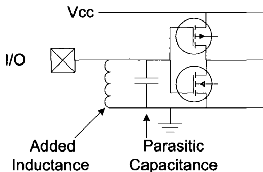
Figure 1.28: The use of an inductor as an ESD protection device
