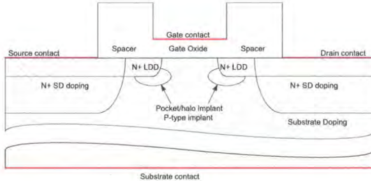
Figure 5.10: The structure of an nMOS transistor as defined by the Finite Element Simulation
