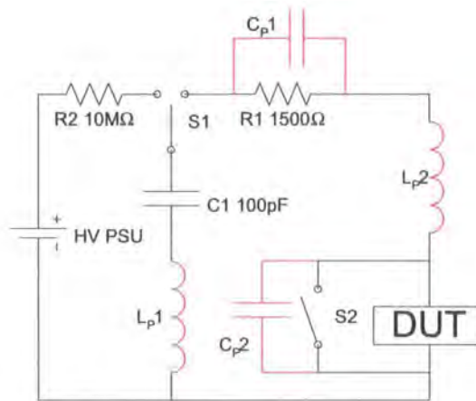
Figure 1.47: HBM ESD test circuit with parasitics
