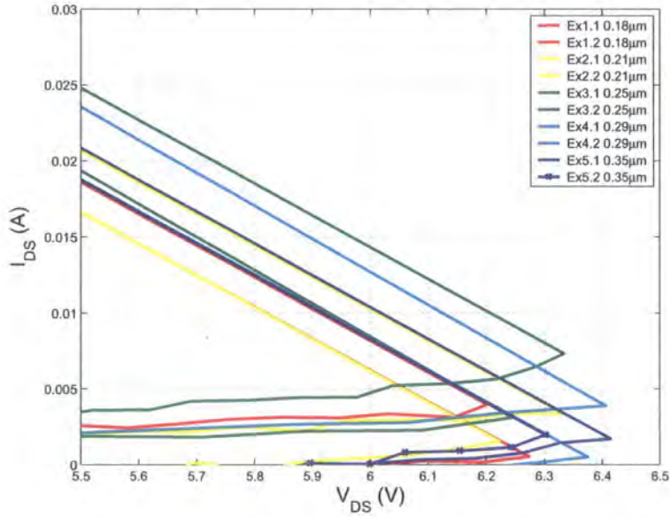
Figure 6.8: Detail of Figure 6.6 showing the triggering of the ggNMOS
