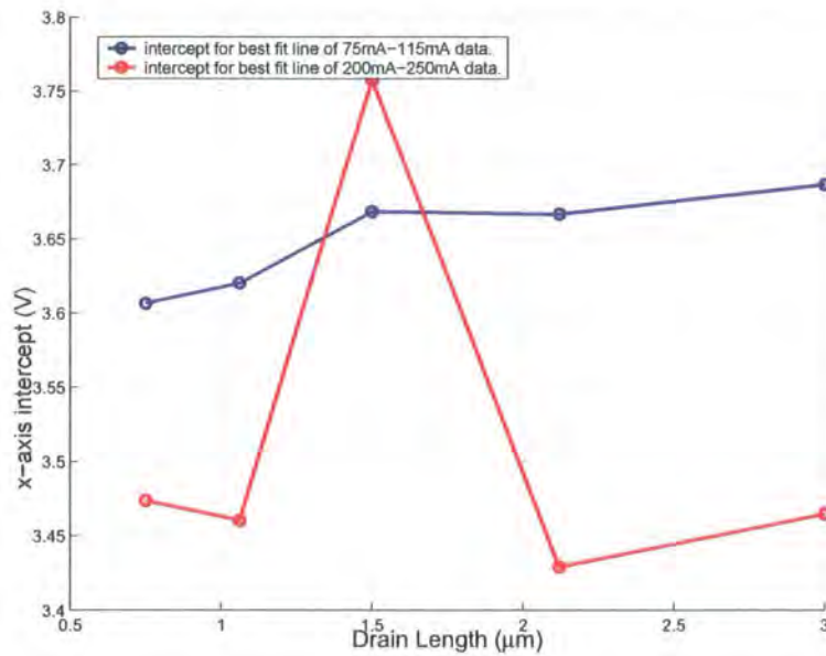
Figure 6.17: The offset voltage of the ggNMOS once the device is triggered over a range of drain lengths
