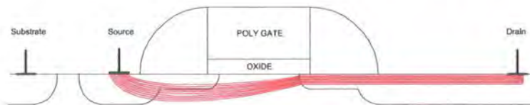
Figure 5.42: The current flow lines in a long drain ggNMOS
