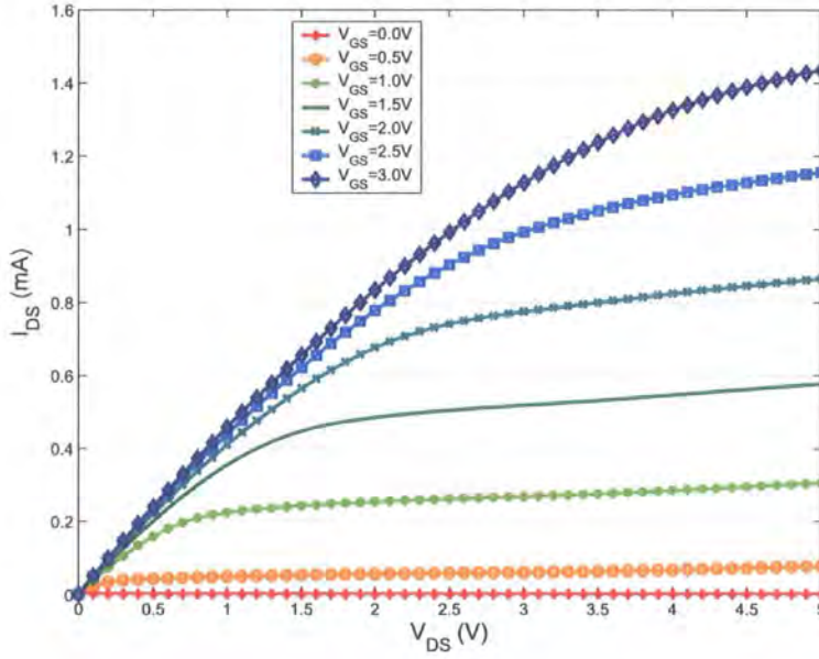
Figure 5.11: V_{DS} vs I_{DS} over a range of V_{GS}
