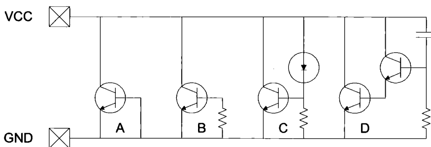
Figure 1.15: Three ESD protection solutions using bipolar transistors
