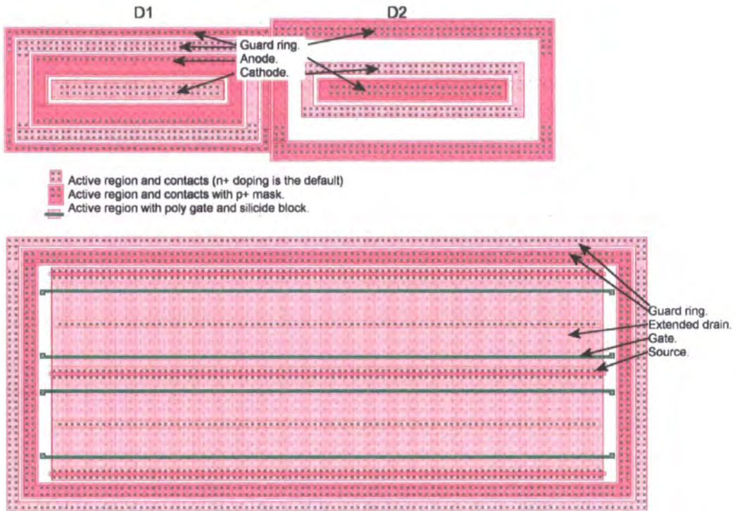
Figure 7.3: Detail from Figure 7.2 showing D1, D2 and ggNMOS1
