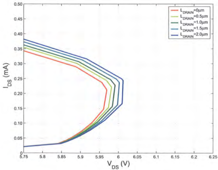
Figure 5.35: Detail from Figure 5.34
