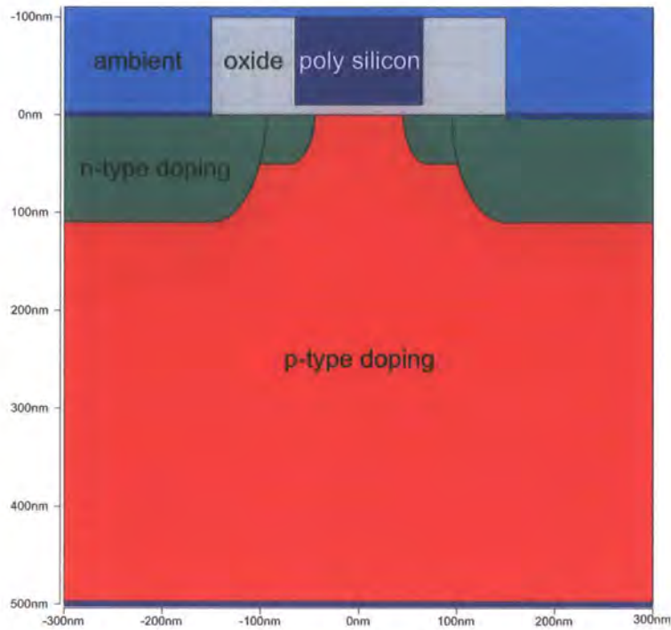
Figure A.1: An un-simulated transistor structure
