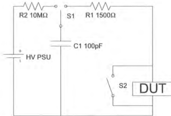
Figure 1.46: HBM ESD test circuit
