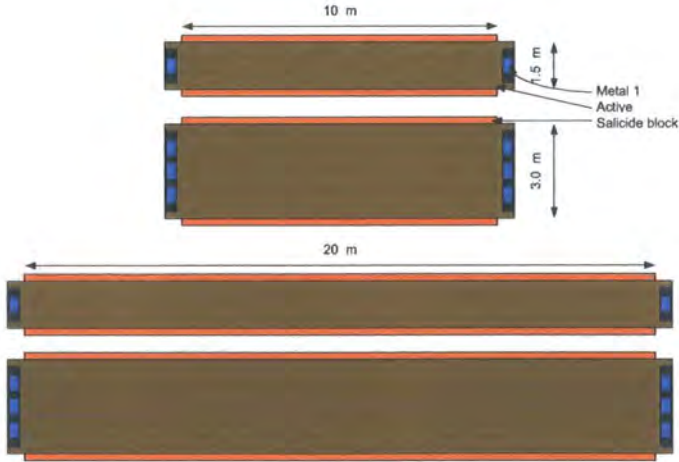
Figure 6.25: Layout of the test resistors
