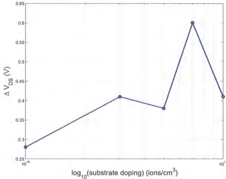
Figure 5.29: Doping density induced changes between the avalanching point and the triggering voltage
