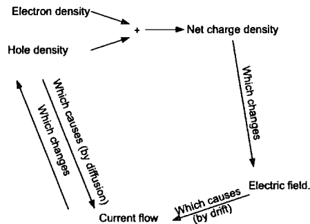
Figure 5.1: The calculations that the Finite Element Simulation software has to satisfy in order for the simulation to converge
