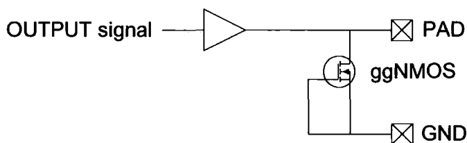
Figure 1.32: Basic ggNMOS design using a standard nMOS
