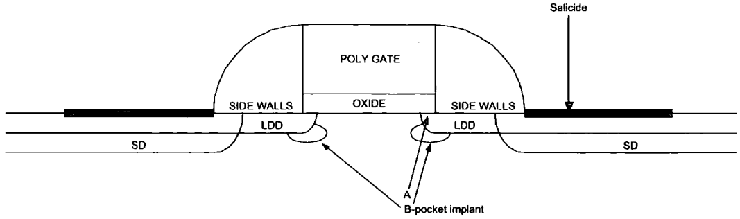
Figure 1.3: Doping profiles in a typical deep sub-micron MOSFET
