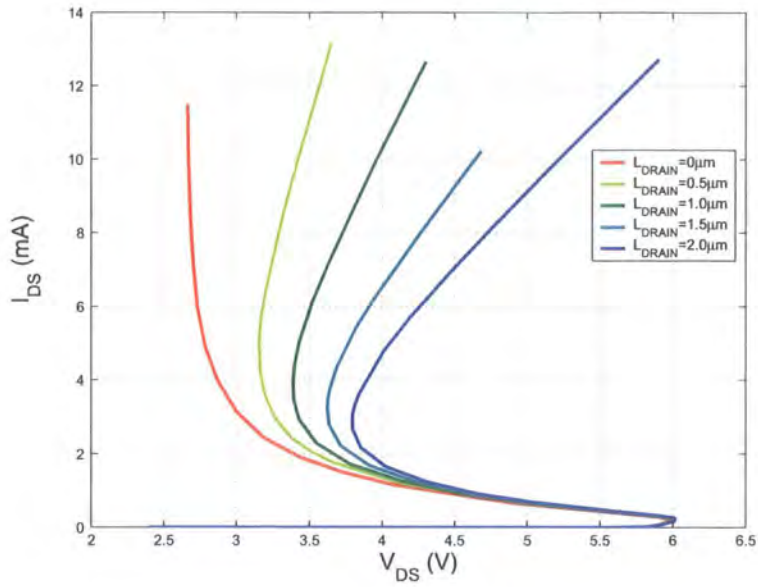
Figure 5.34: The IV characteristics of a ggNMOS for various lengths of extended drain
