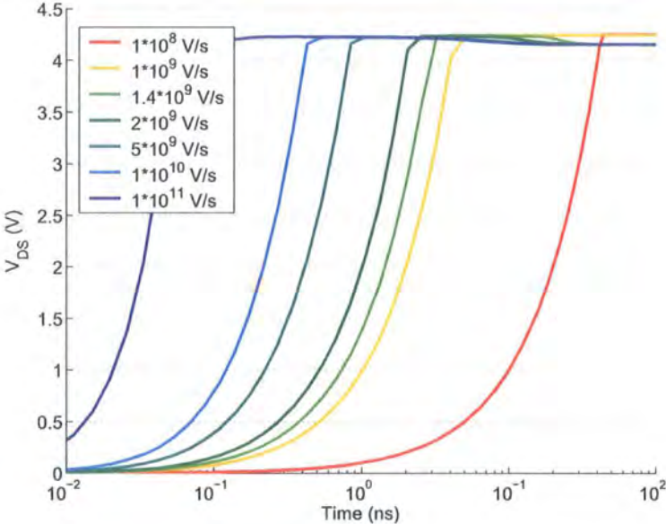
Figure 5.25: V_{DS} vs time over a range of voltage limited ramps
