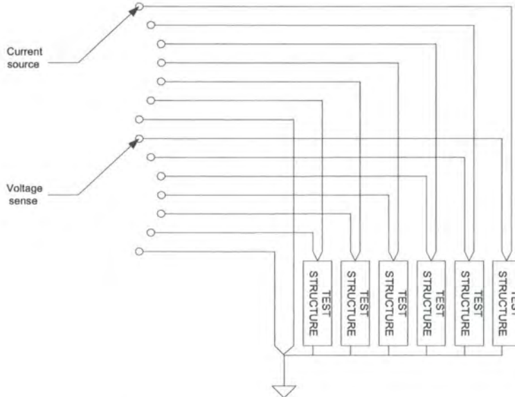
Figure 6.4: The circuit used to characterise the low current test structures
