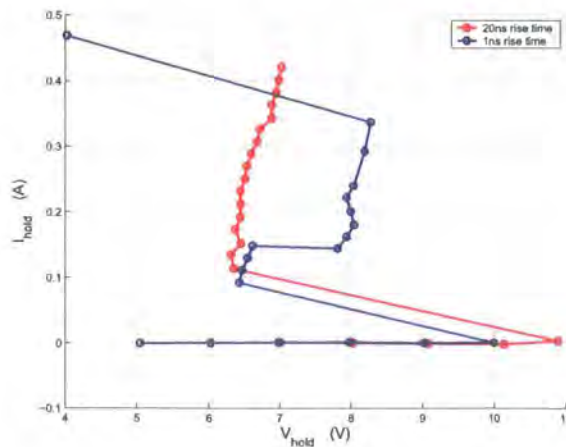
Figure 3.8: IV characteristics of the BC01b for 1ns and 20ns rise times
