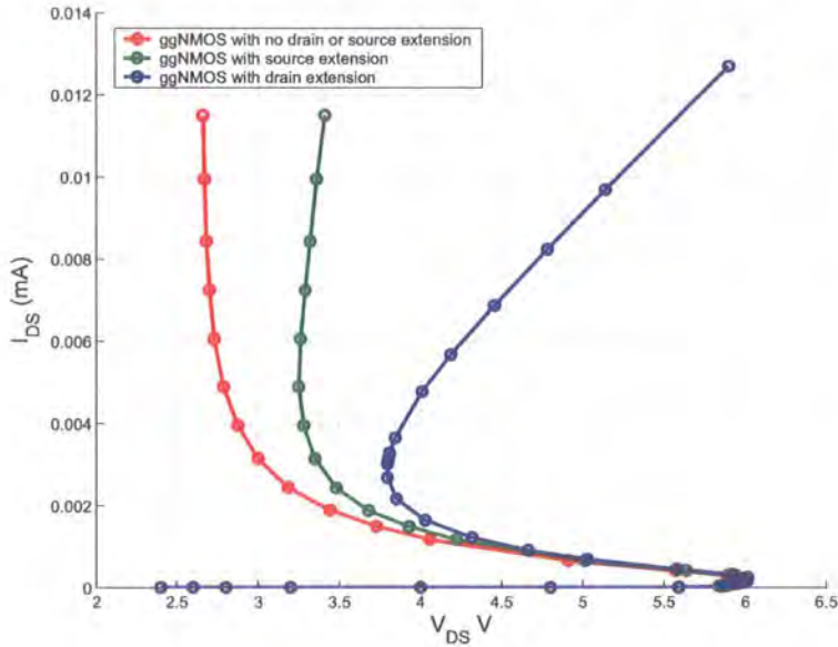
Figure 5.41: Extended source, extended drain and standard ggNMOS IV curves
