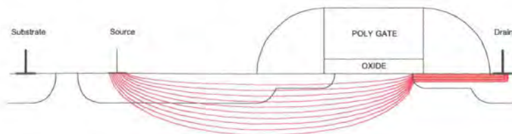
Figure 5.43: The current flow lines in a long source ggNMOS
