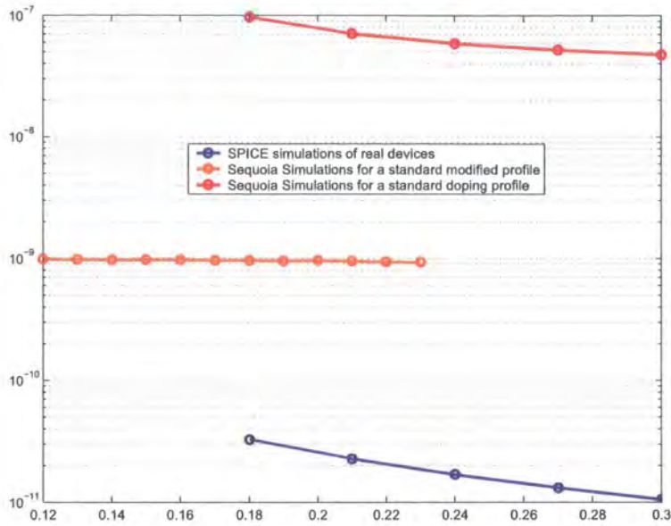
Figure 6.11: Change in I_{leak} when the V_T doping profile is changed
