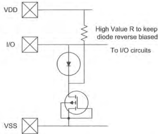
Figure 1.9: The use of the diode to reduce the capacitive load on an IO due to an ESD protection structure
