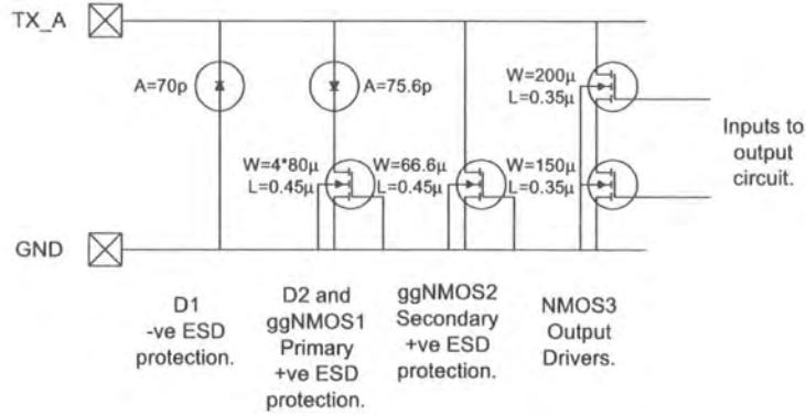
Figure 7.1: Output stage of the BC01b's TX_A identical to TX_B
