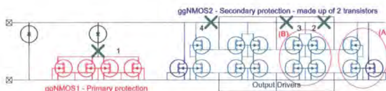
Figure 3.25: Circuit of the BC01b output. The circles indicate the location of circuit failure
