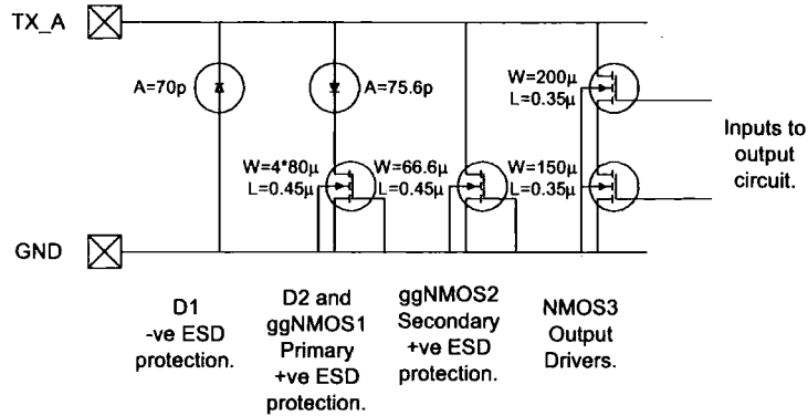
Figure 3.1: Output stage of the BC01b's TX_A which is identical to TX_B
