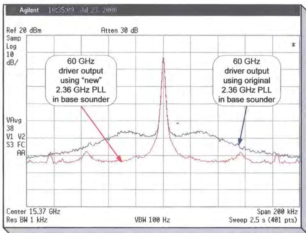
Figure 4.59 Comparison of phase noise at 15 GHz (60 GHz driver) for different PLLs
