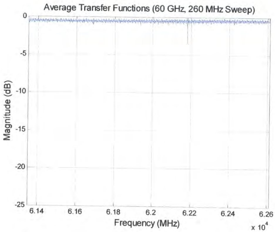
Figure 5.60 60 GHz sounder, 260 MHz sweep width
