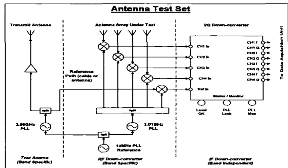
Figure 5. Block diagram of the antenna test set
