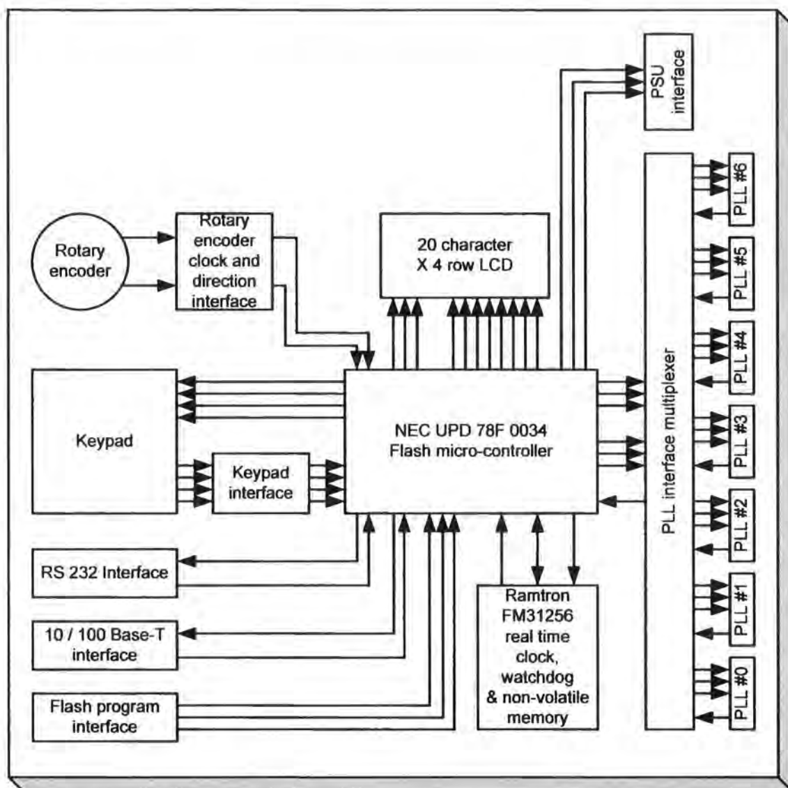
Figure 4.4 Micro-controller
