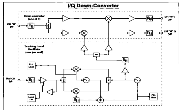
Figure 2. Block diagram of I/Q down-converter module
