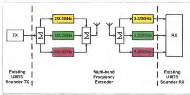
Figure 2. Block diagram for the multi-band sounder
