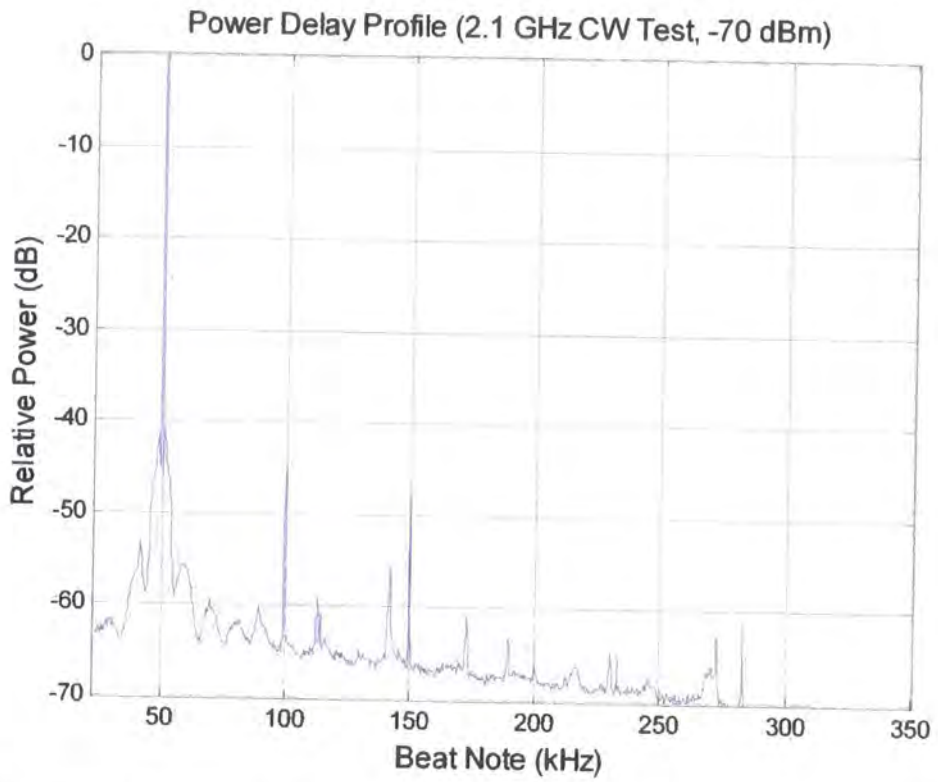
Figure 5.22a 2.1 GHz base sounder CW test (wide)
