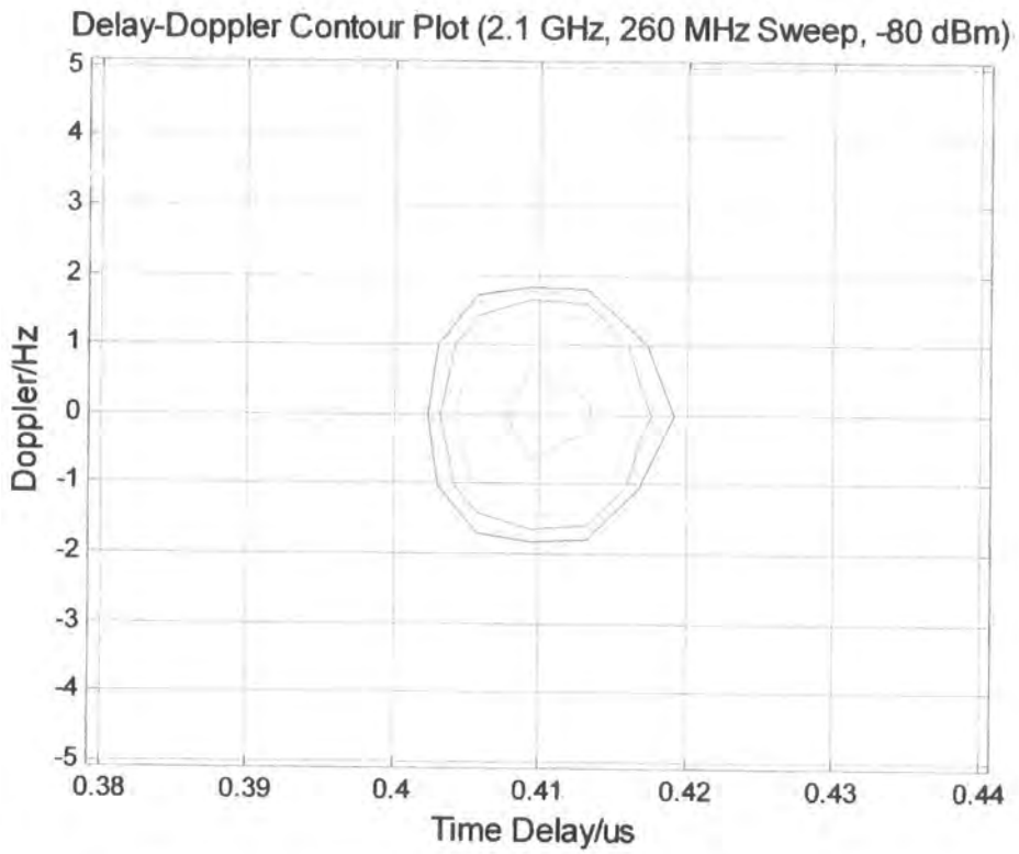
Figure 5.42a Base sounder Doppler ambiguity function, -80 dBm input, 260 MHz
