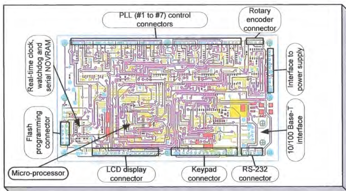
Figure 4.32 Micro-controller PCB
