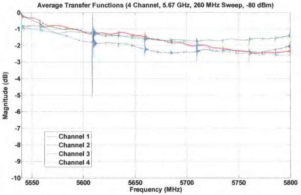
Figure 5.76 5.7 GHz four channel frequency transfer function, -80 dBm, 260 MHz
