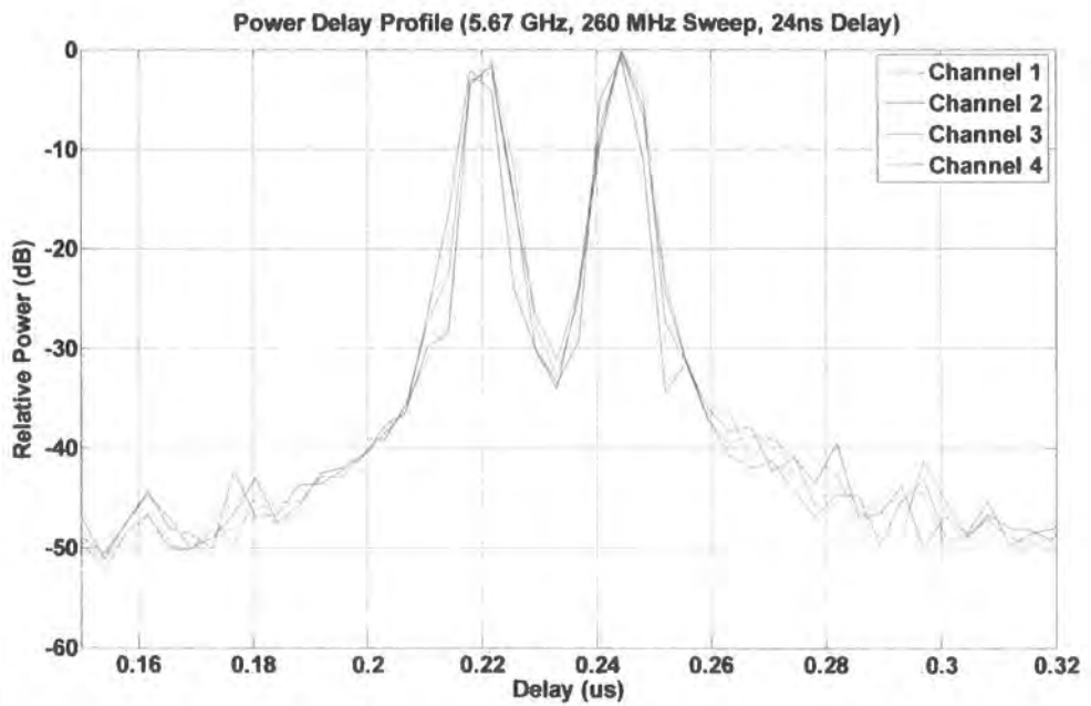
Figure 5.78a 5.7 GHz four channel dual delay profile, -80 dBm, 260 MHz
