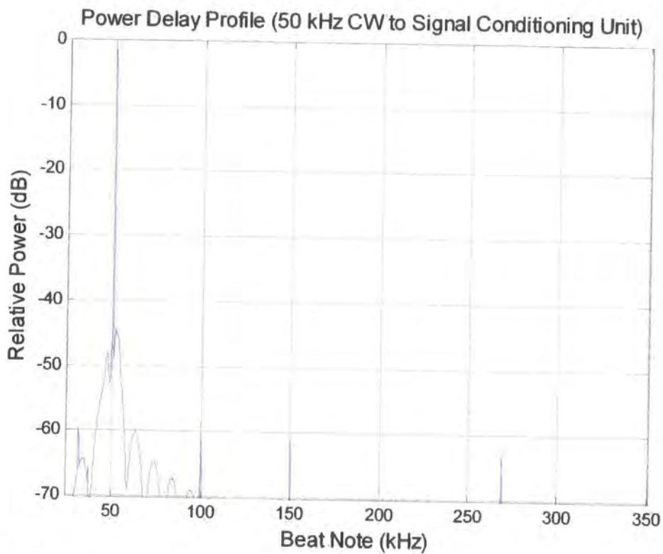
Figure 5.21a Data acquisition CW test (wide)
