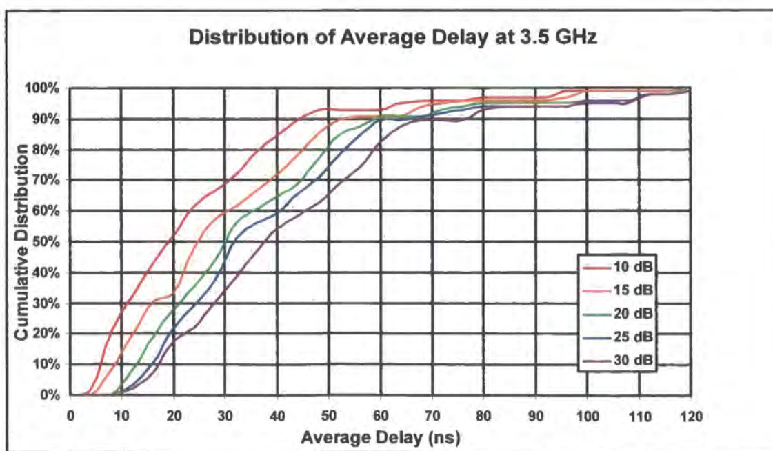
Figure 6.27 Distribution of average delay (indoors) at 3.5 GHz
