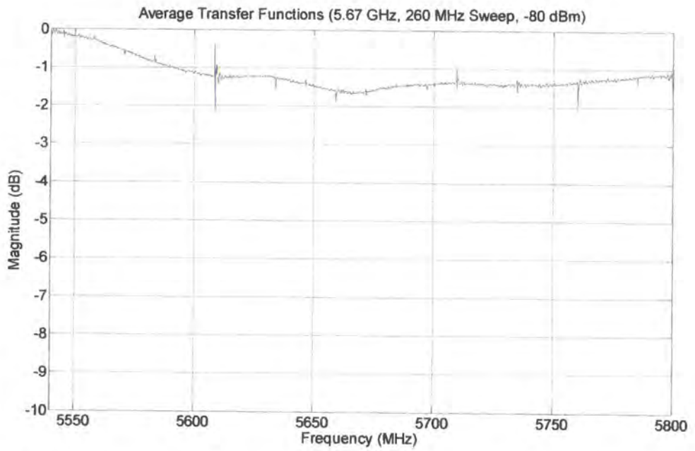
Figure 5.52a 5.7 GHz sounder frequency-transfer function, -80 dBm input, 260 MHz
