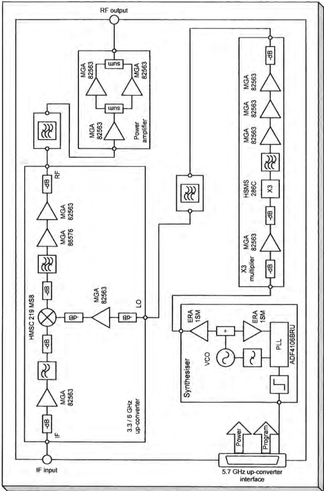
Figure 4.7 Up-converter assembly for 5.7 GHz 4-14
