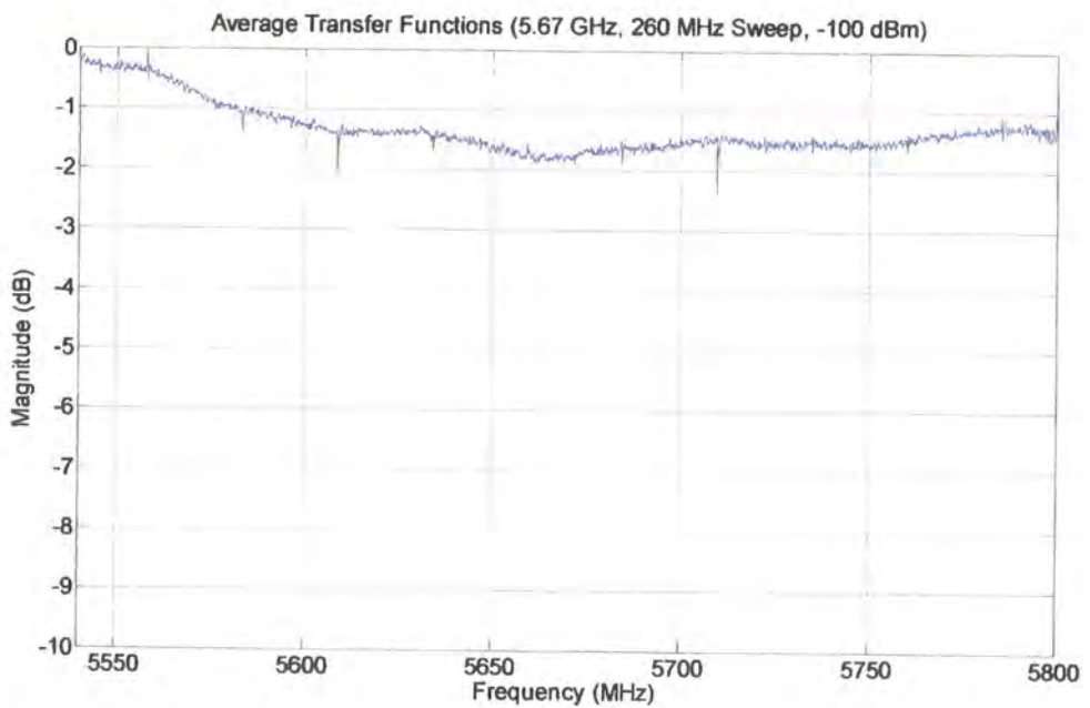
Figure 5.52b 5.7 GHz sounder frequency-transfer function, -100 dBm input, 260 MHz
