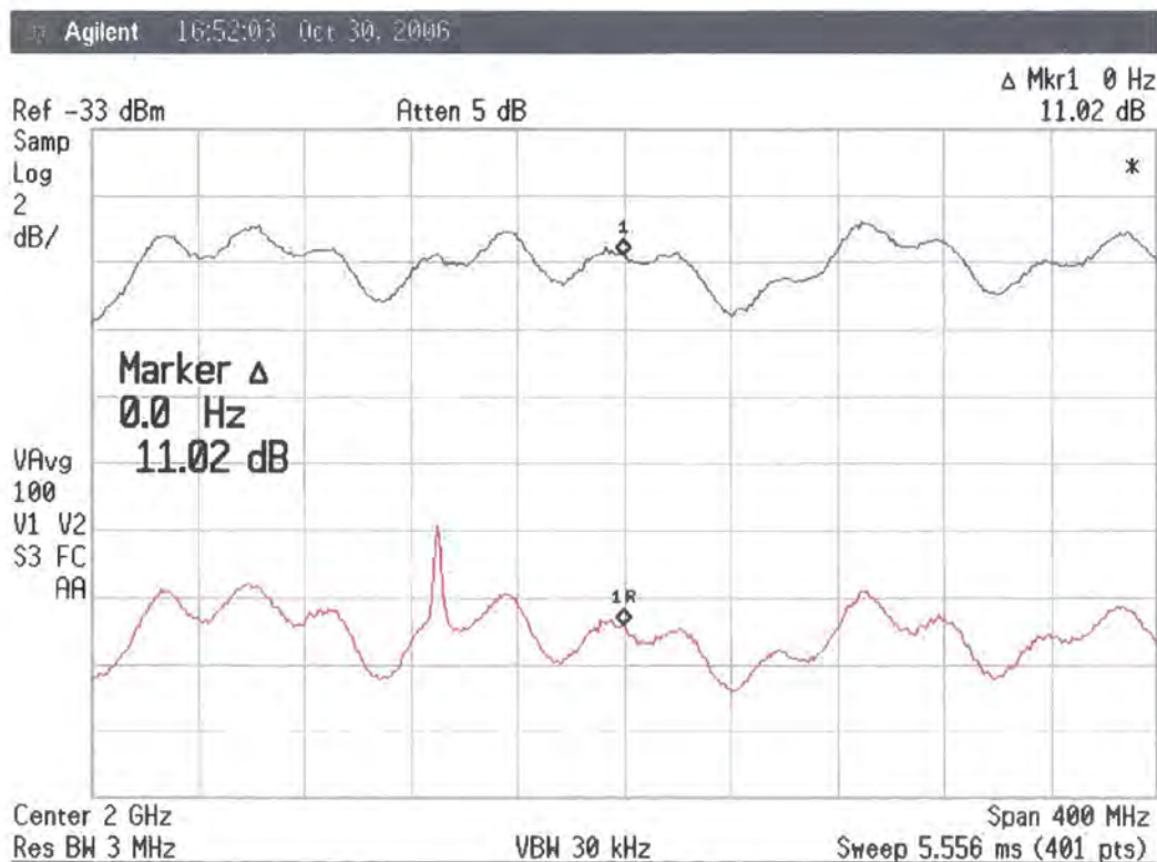
Figure 5.14 “y-factor” measurement of the 2.5 GHz down-converter
