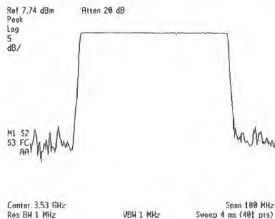
Figure 6. Output at 3.53GHz from the 3.3/4.5GHz converter
