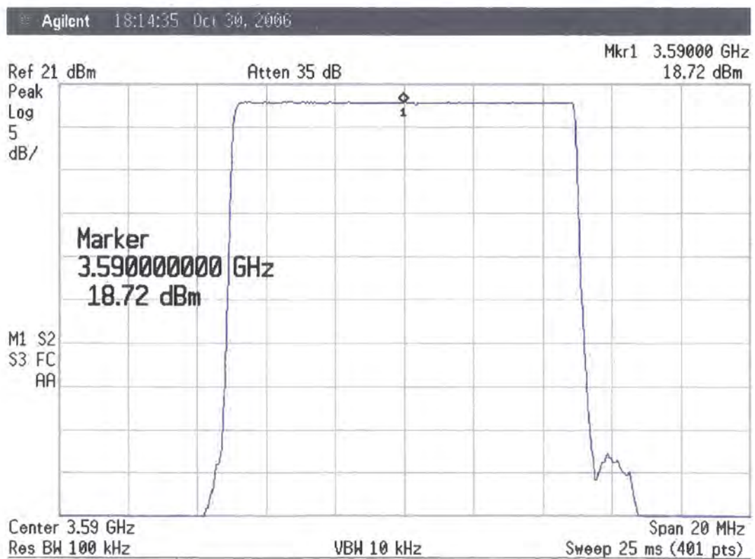
Figure 5.4 3.59 GHz TX Flatness for 10 MHz sweep width
