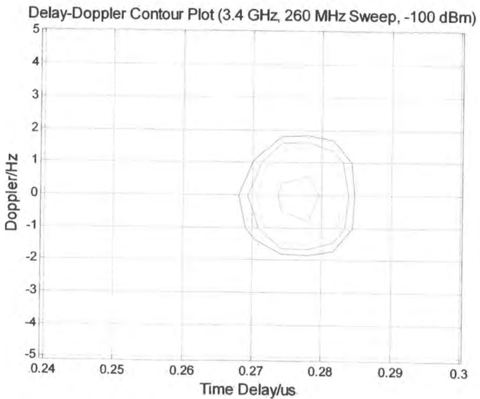
Figure 5.48b 3.5 GHz sounder Doppler ambiguity function, -100 dBm input, 260 MHz
