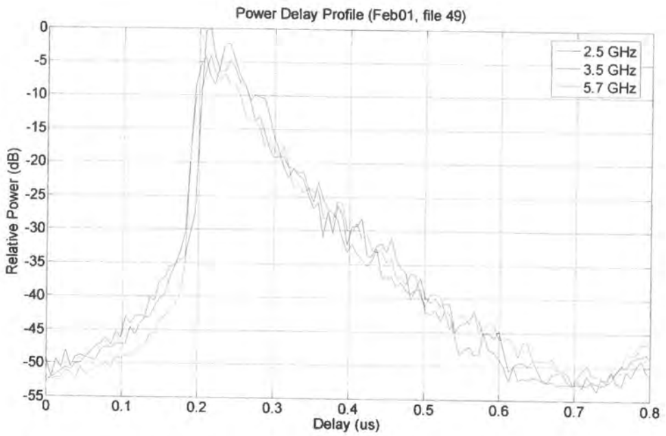
Figure 6.46 Power delay profile for receiver moving away from transmitter
