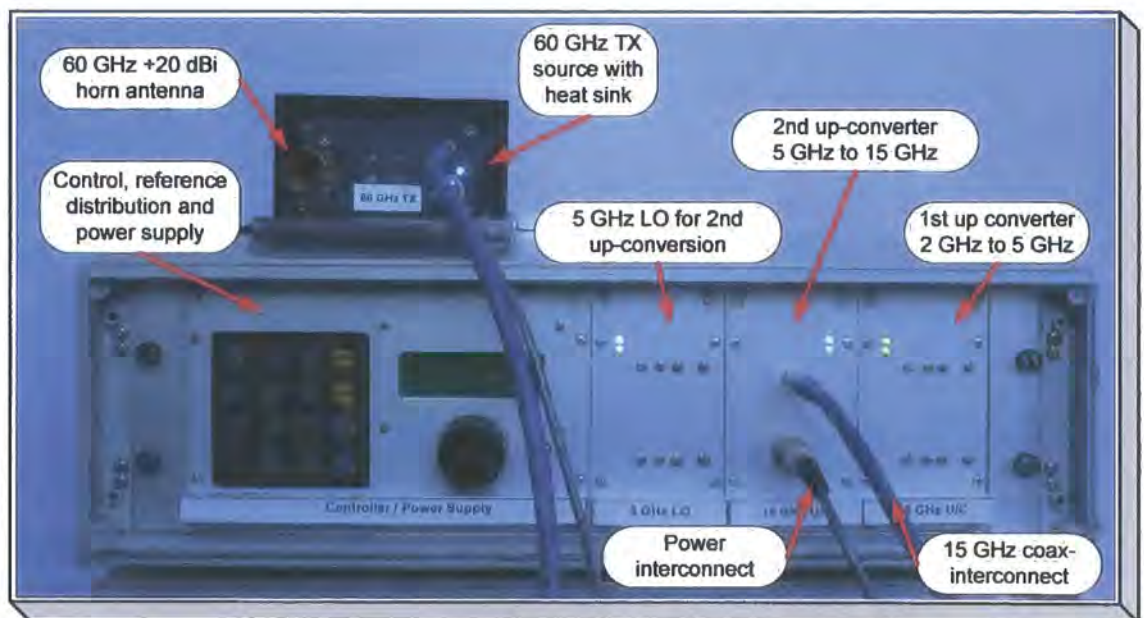
Figure 4.24 60 GHz transmitter driver rack and output multiplier
