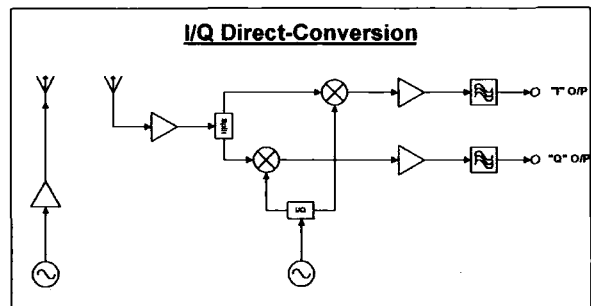
Figure 1. Block diagram of direct conversion architecture
