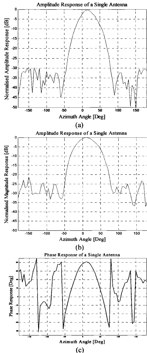
Figure 6. Experimental results for a single antenna (a) amplitude with log-amplifier, (b) amplitude with I/Q down-converter, (c) phase with I/Q down-converter
