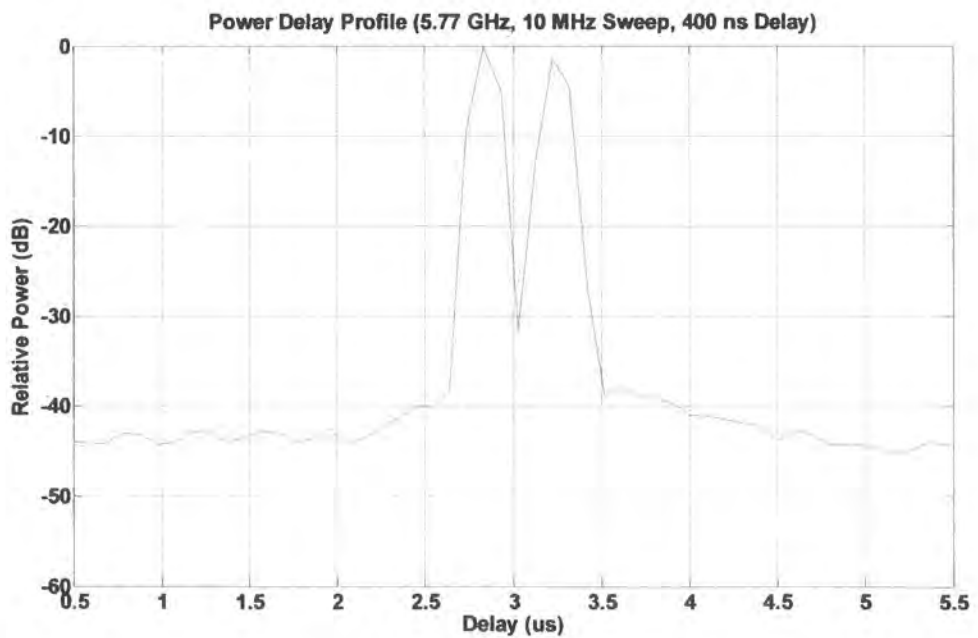
Figure 5.66a Two delay profile for 5.7 GHz sounder, -90 dBm, 10 MHz
