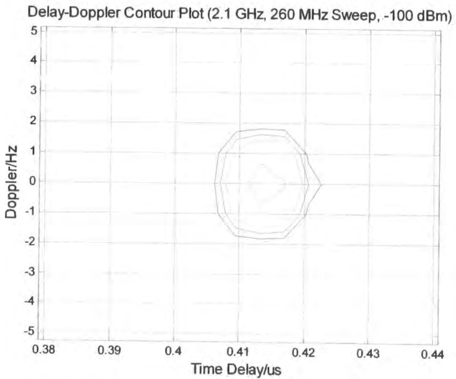
Figure 5.42b Base sounder Doppler ambiguity function, -100 dBm input, 260 MHz
