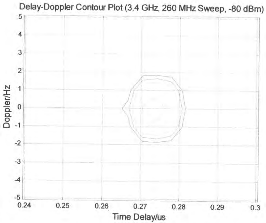
Figure 5.48a 3.5 GHz sounder Doppler ambiguity function, -80 dBm input, 260 MHz
