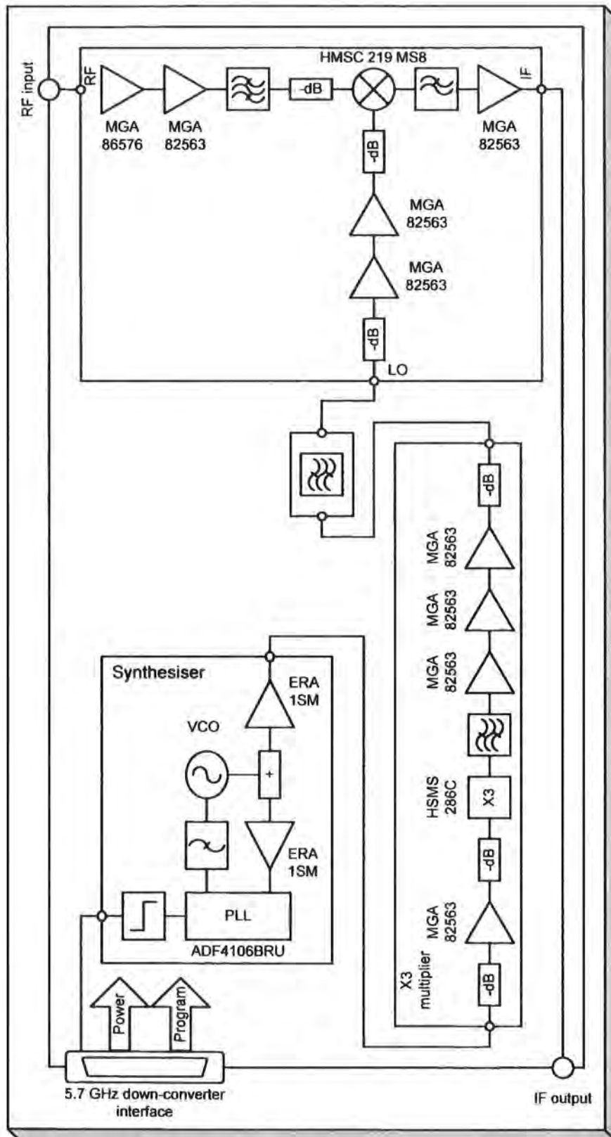
Figure 4.10 Down-converter assembly for 5.7 GHz 4-20
