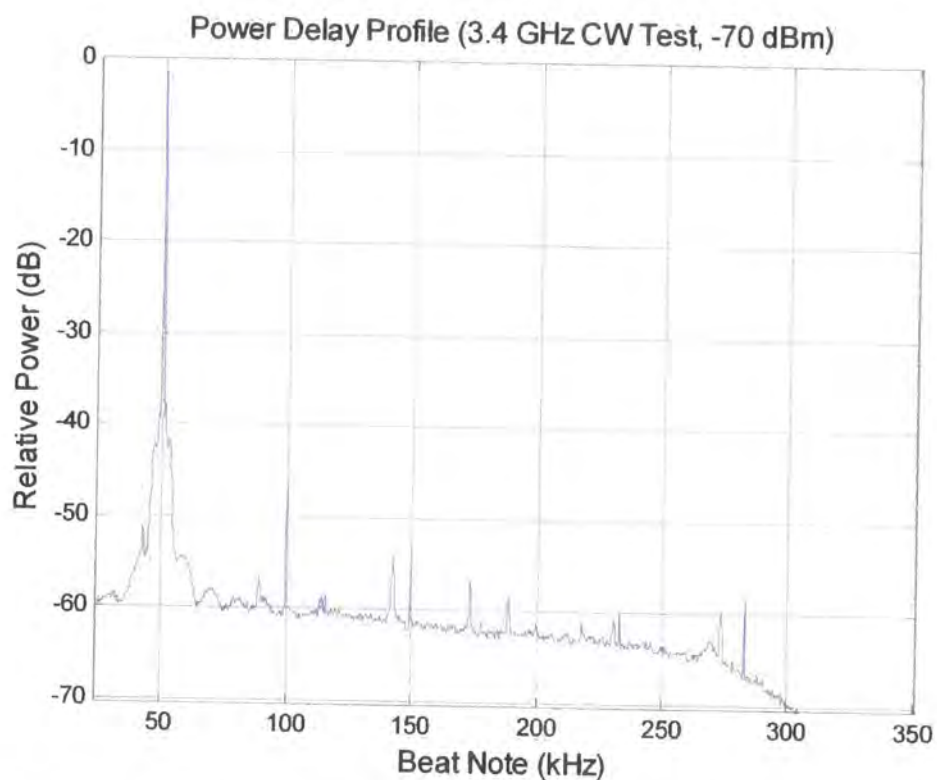
Figure 5.24a 3.4 GHz converter and sounder CW test (wide)
