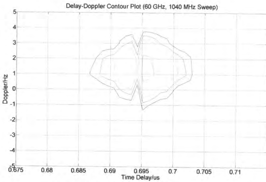
Figure 5.55 60 GHz sounder, 1040 MHz sweep width
