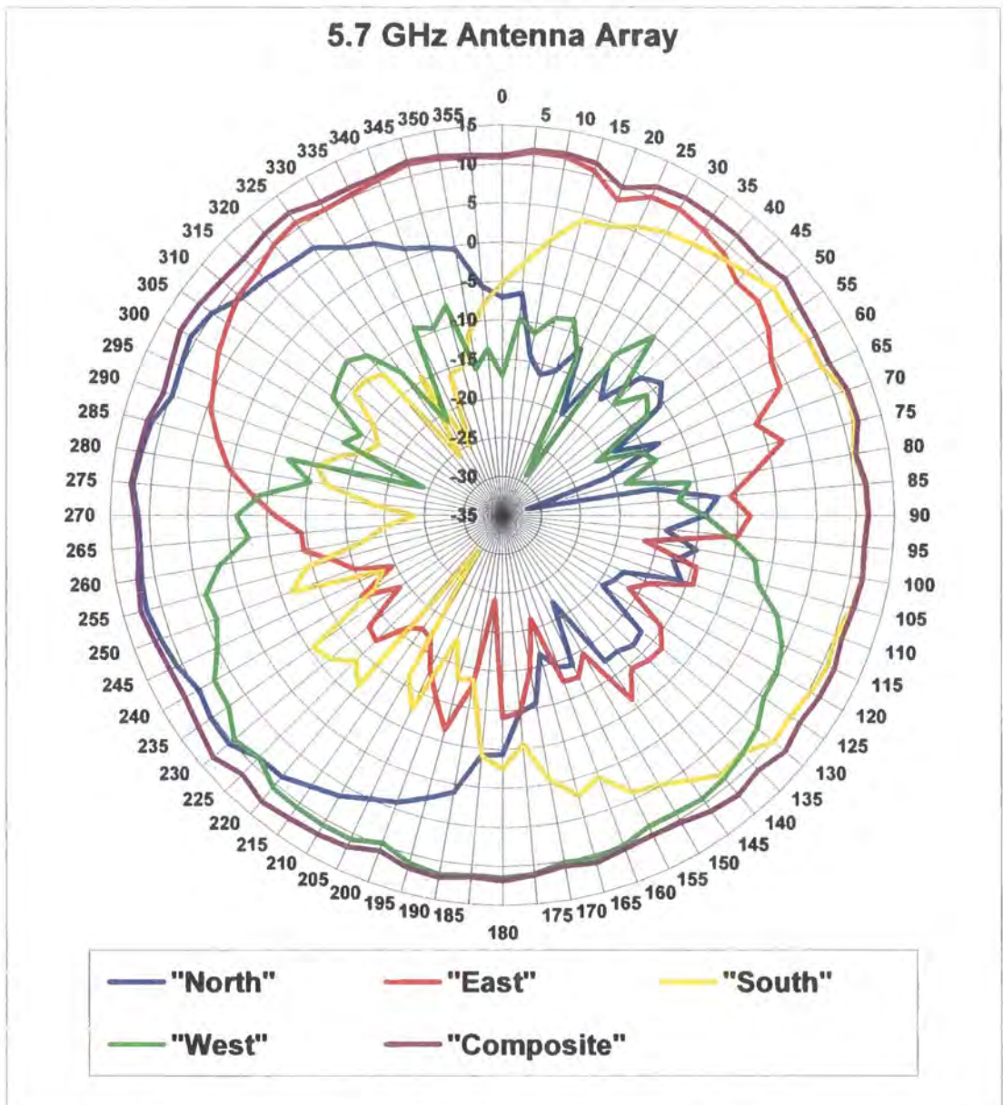
Figure 5.81 Polar response of the 5.7 GHz antenna array
