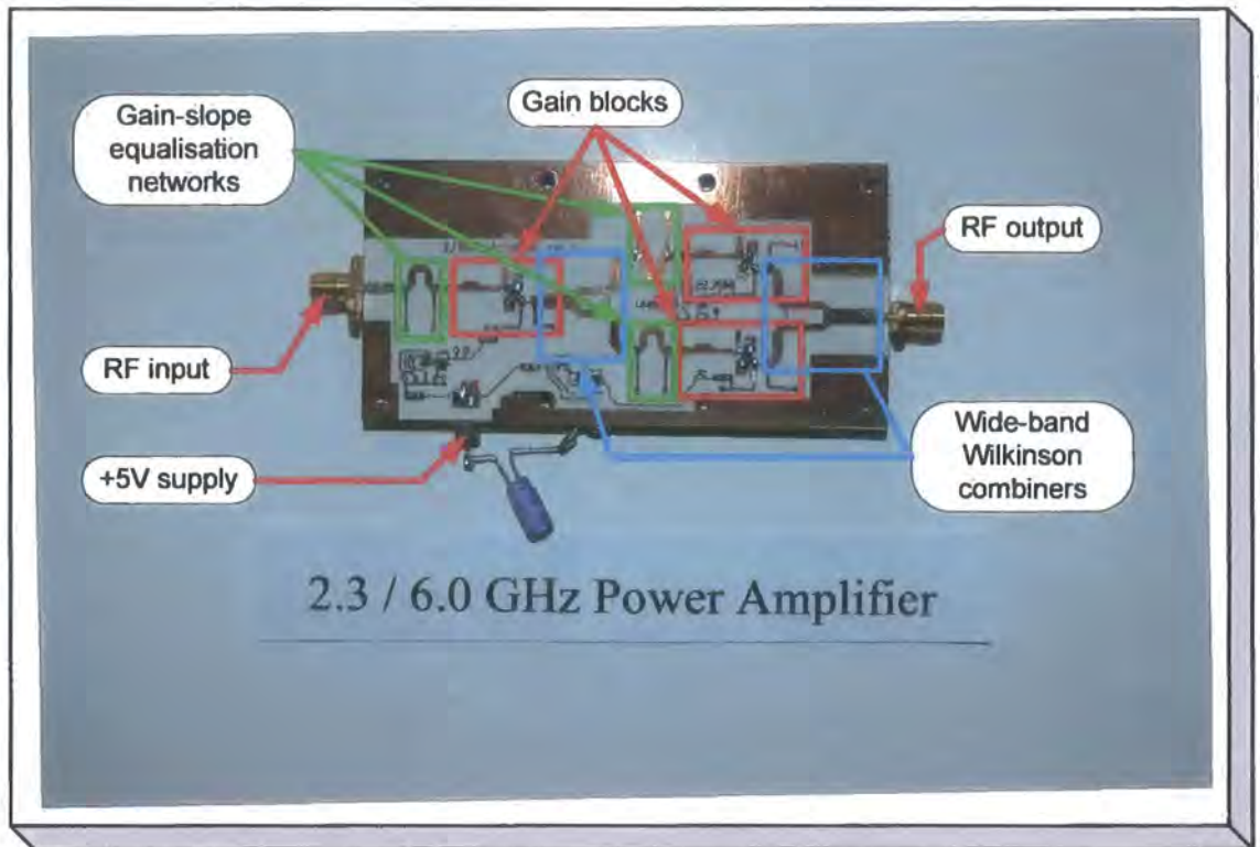
Figure 4.51 Power amplifier
