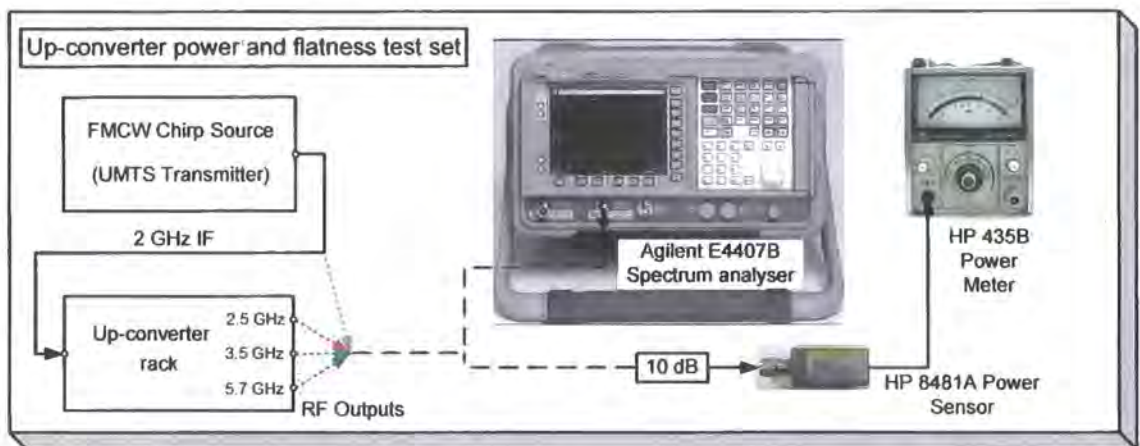
Figure 5.1 Equipment configuration for transmitter power and flatness measurement
