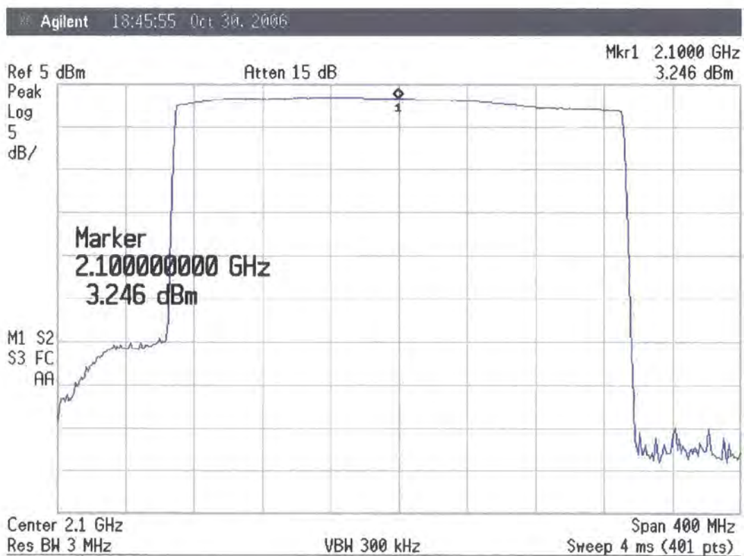
Figure 5.6 2.1 GHz IF flatness for 260 MHz sweep width
