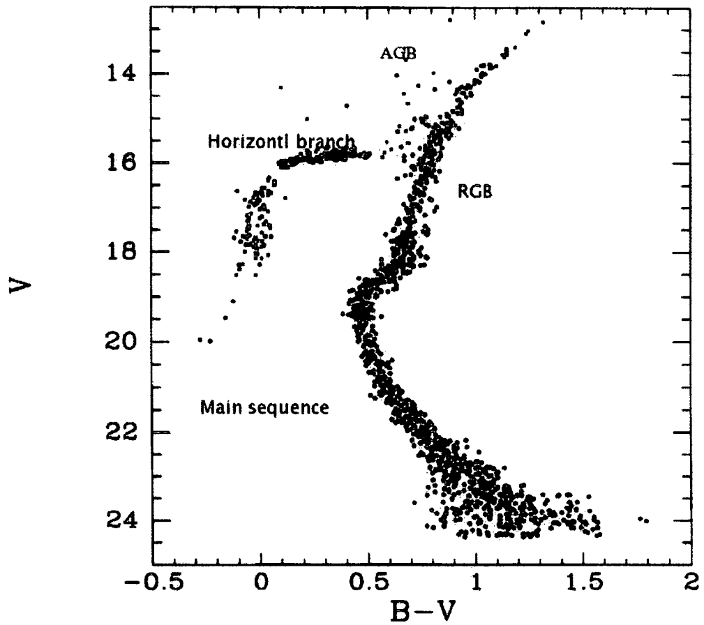
Figure 1.2: Colour-Magnitude diagram of M15 taken from Durrell & Harris (1993). Major evolutionary stages are labelled: main sequence, red giant branch star (RGB), horizontal branch stars, and asymptotic giant branch stars (AGB).
