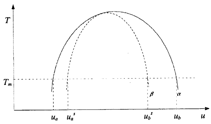
Figure 1.2: Phase diagram of binary alloy.
