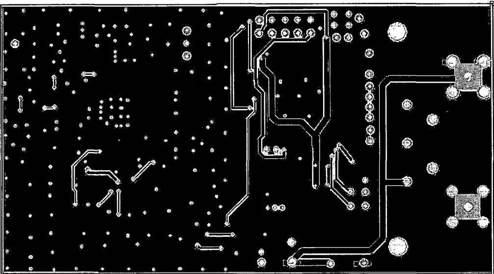
Figure 33 – Pre-production PCB Layout (Bottom Layer)
