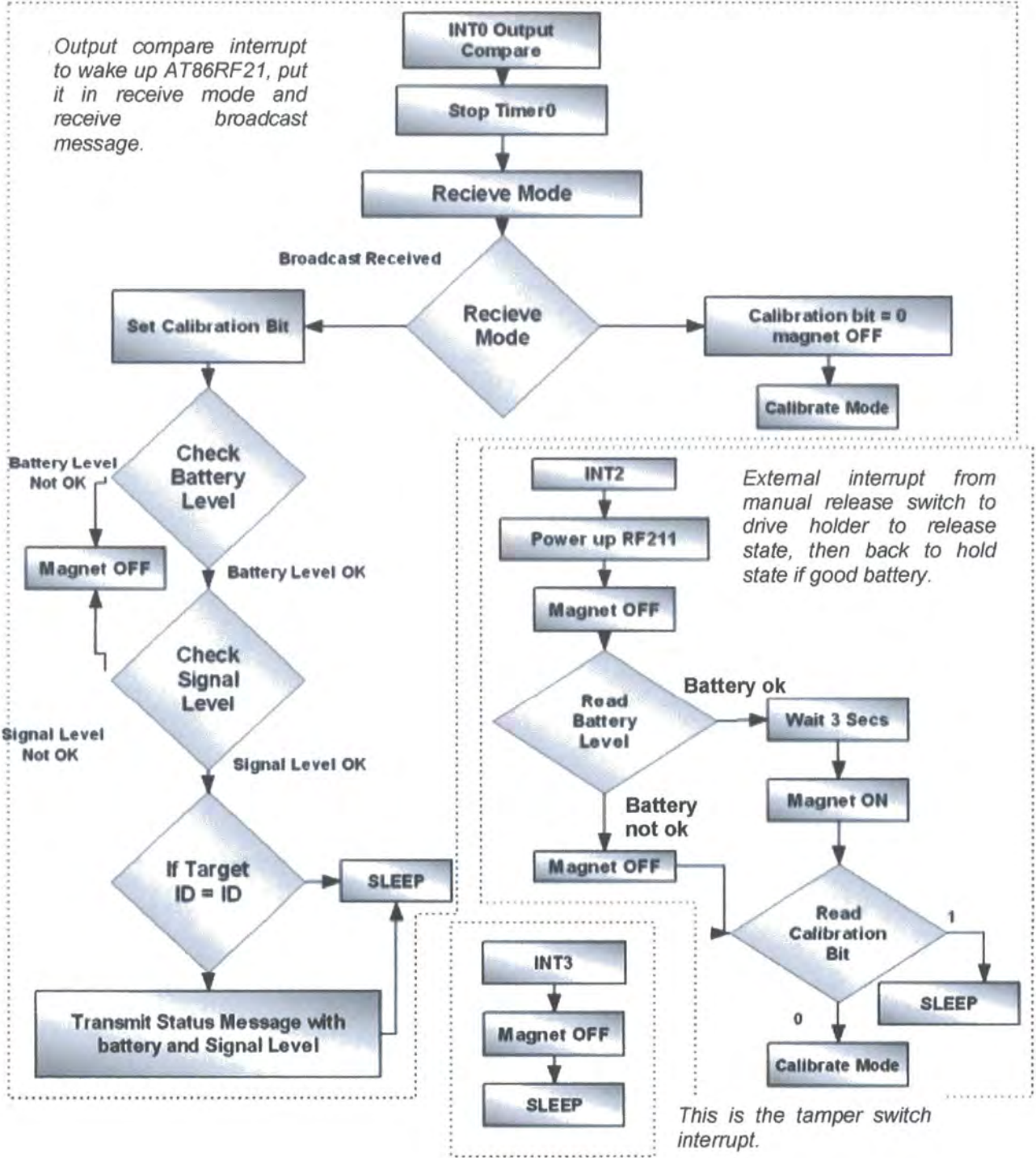
Figure 56 – Slave Software Flowchart(ii)
