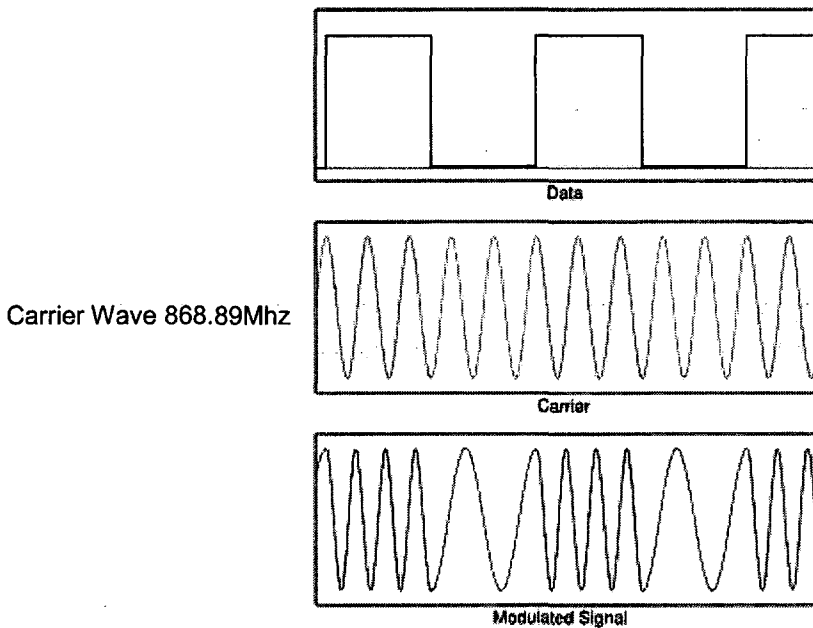
Figure 9 – FSK Modulation
