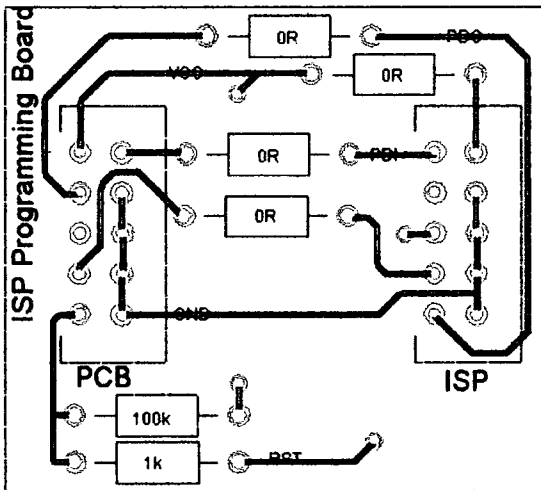
Figure 14 – AVRISP PCB Layout (Top Layer)
