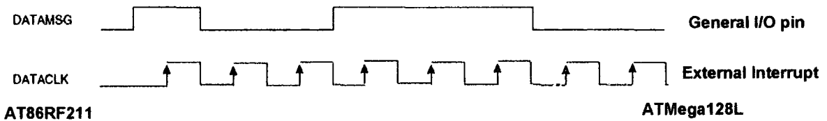
Figure 48 – Dataclk recovery
