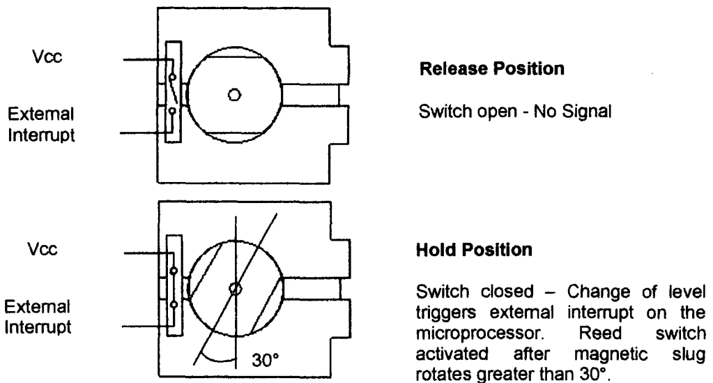
Figure 30 - Release & Hold Positions for Reed Switch
