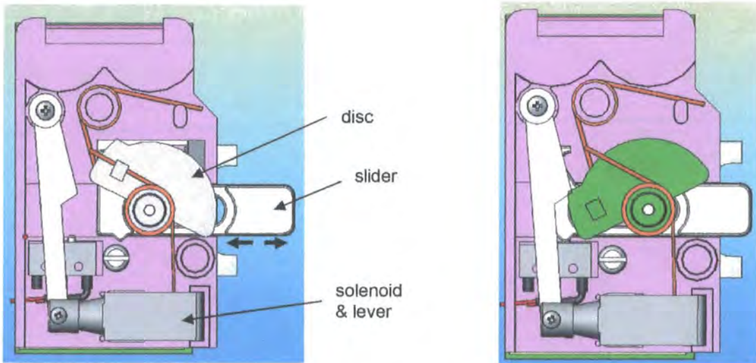
Figure 26 – Solenoid latching Design (Engaged/Disengaged)
