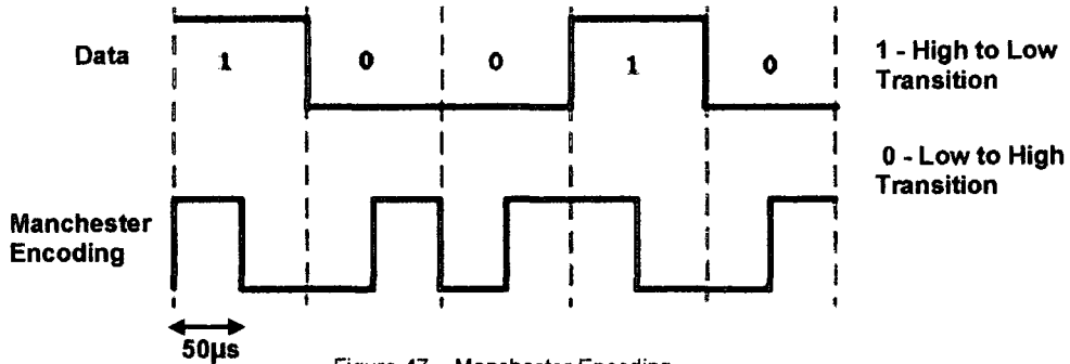
Figure 47 – Manchester Encoding
