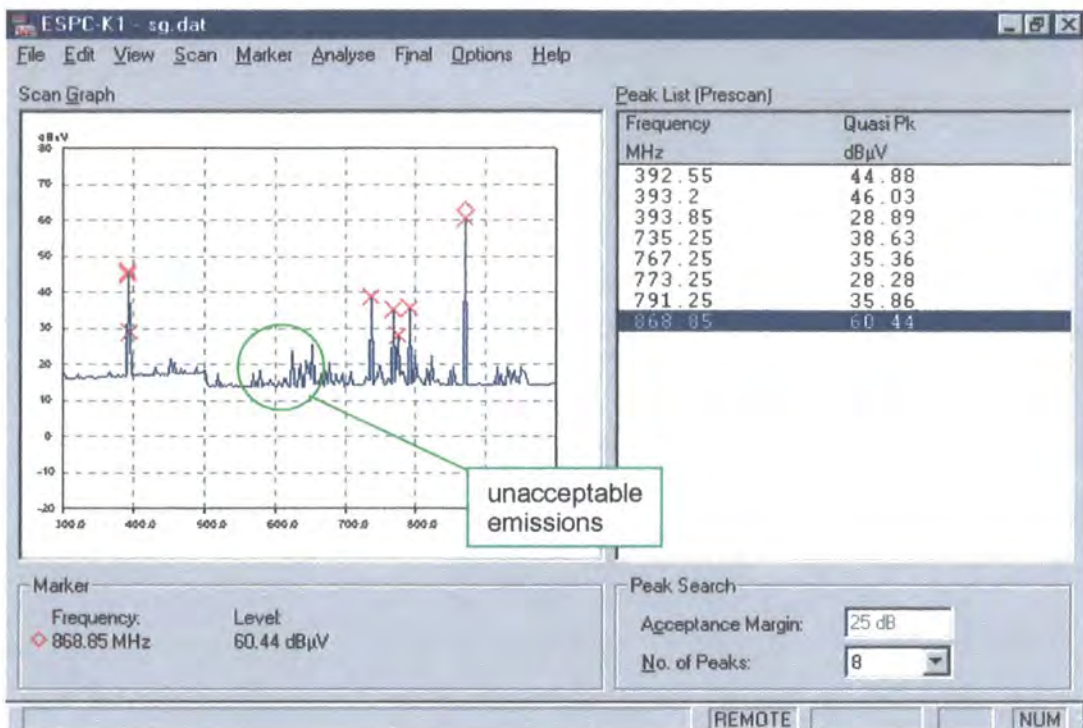
Figure 20 - Screen Image of scan from 300 – 1000MHz, measuring quasi peak (dBuV), 2ms dwell time, 50kHz resolution with no capacitor.
