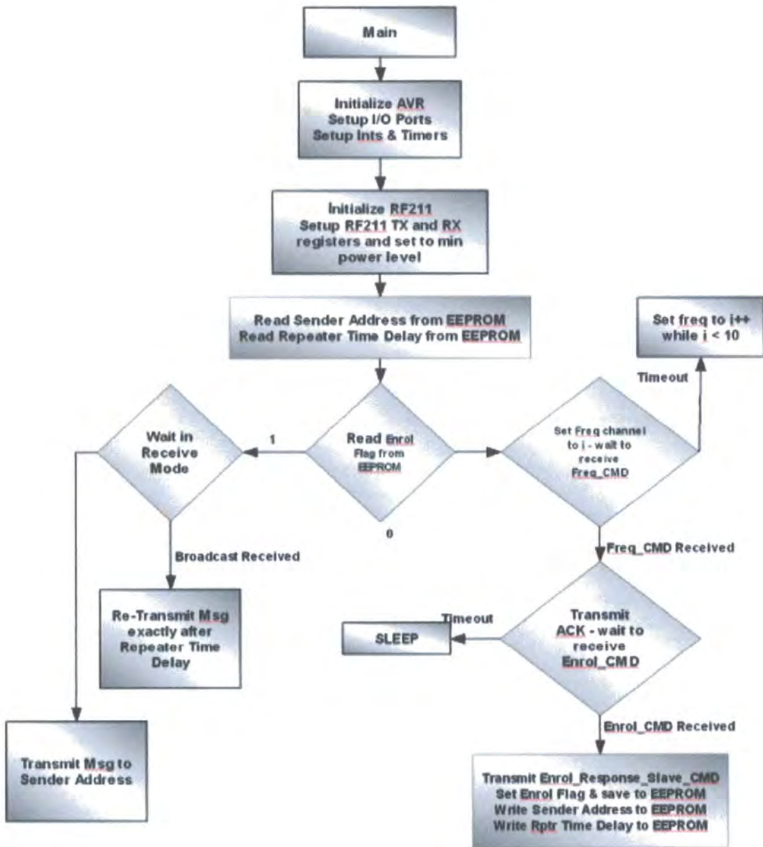
Figure 58 – Repeater Software Flowchart
