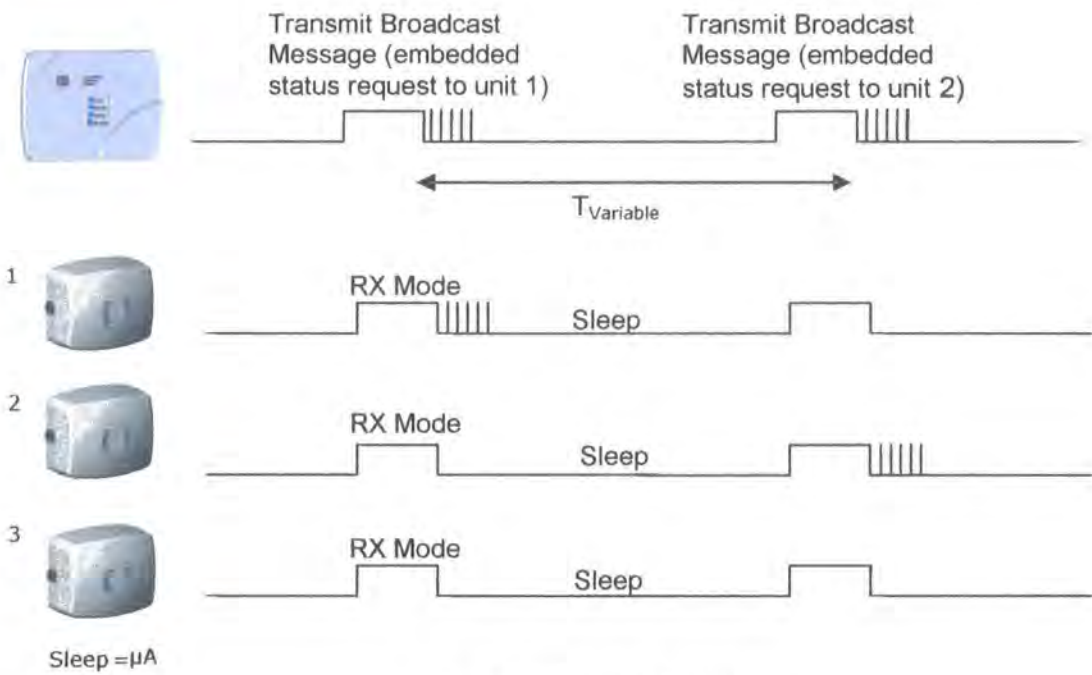
Figure 42 - Hibernation Protocol
