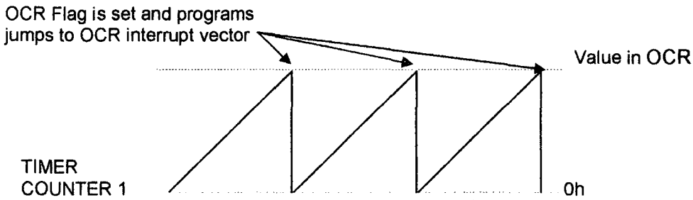
Figure 46 – Output Compare Interrupt Diagram
