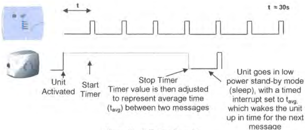
Figure 41 – Calibration Procedure
