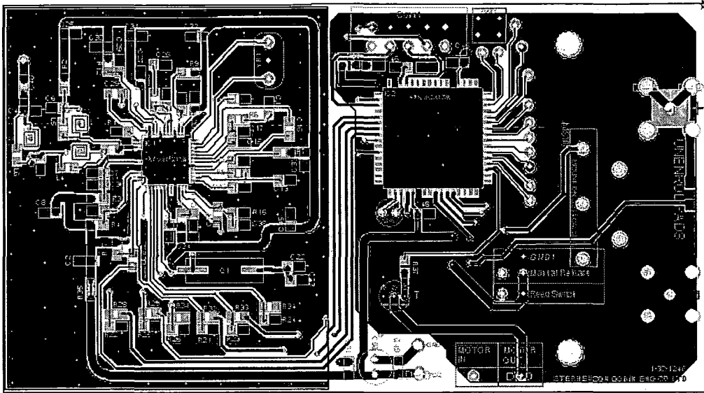
Figure 32 – Pre-production PCB Layout (Top Layer)
