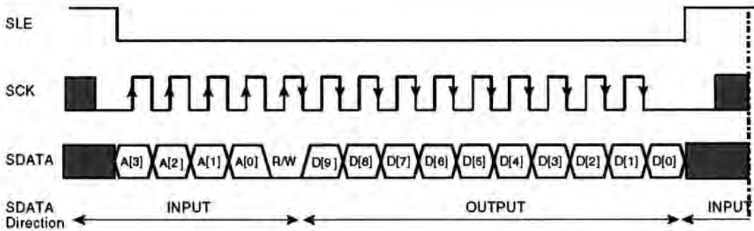
Figure 8 – SPI Read Cycle from a 10 Bit Register
