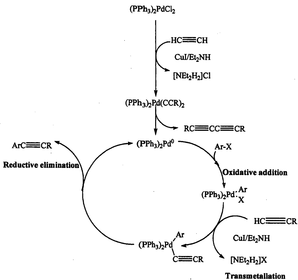
Scheme 1.8: Catalytic cycle for the Sonogashira coupling reaction 1,2
