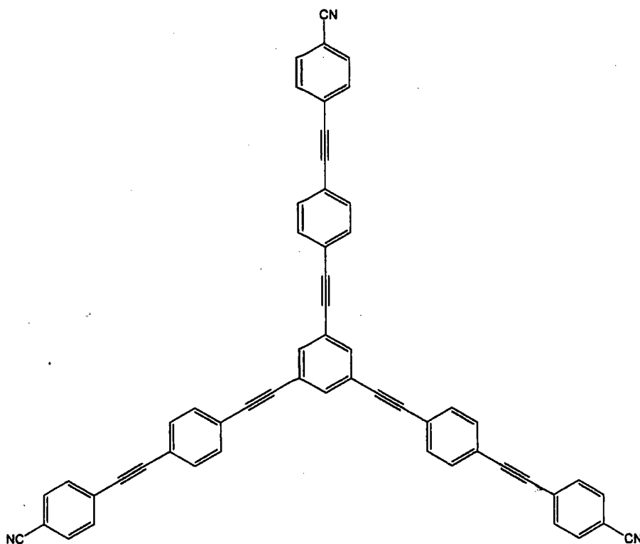
Fig 2.3: Synthesis of a trigonal conjugated compound for use in the preparation of pseudo-hexagonal porous material containing Ag
