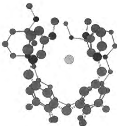
Figure 22 3D model of possible encapsulation of chloride anion within cavity of Tetra[3-(methylamino)pyridinium-methyl] tetrahydroxylcalixarene.
