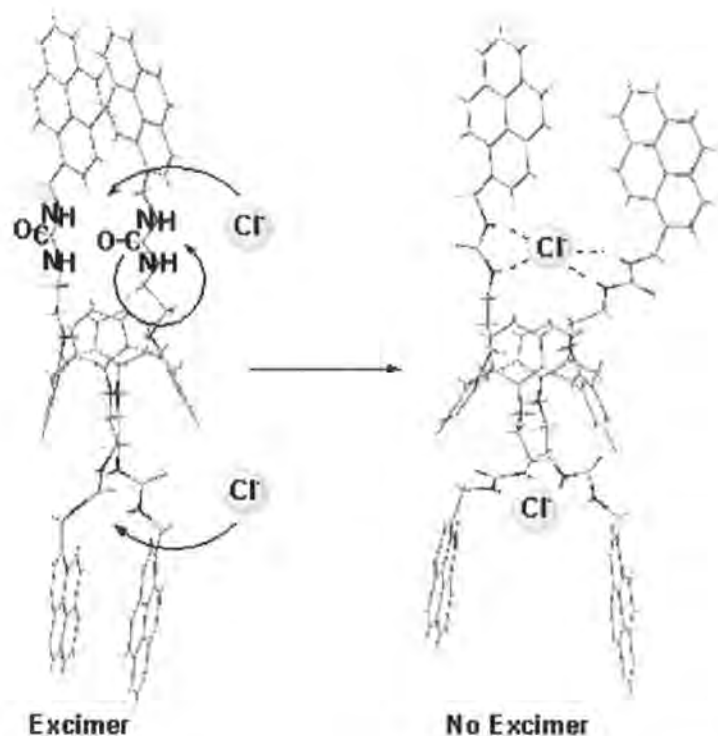
Scheme 5 Binding of chloride ions by 2.11 . Quenching of Excimer Emission (452 nm) caused by a perturbation of the pyrene \pi - \pi interaction by the change in conformation of the pyrene moieties (reproduced from ref 115).
