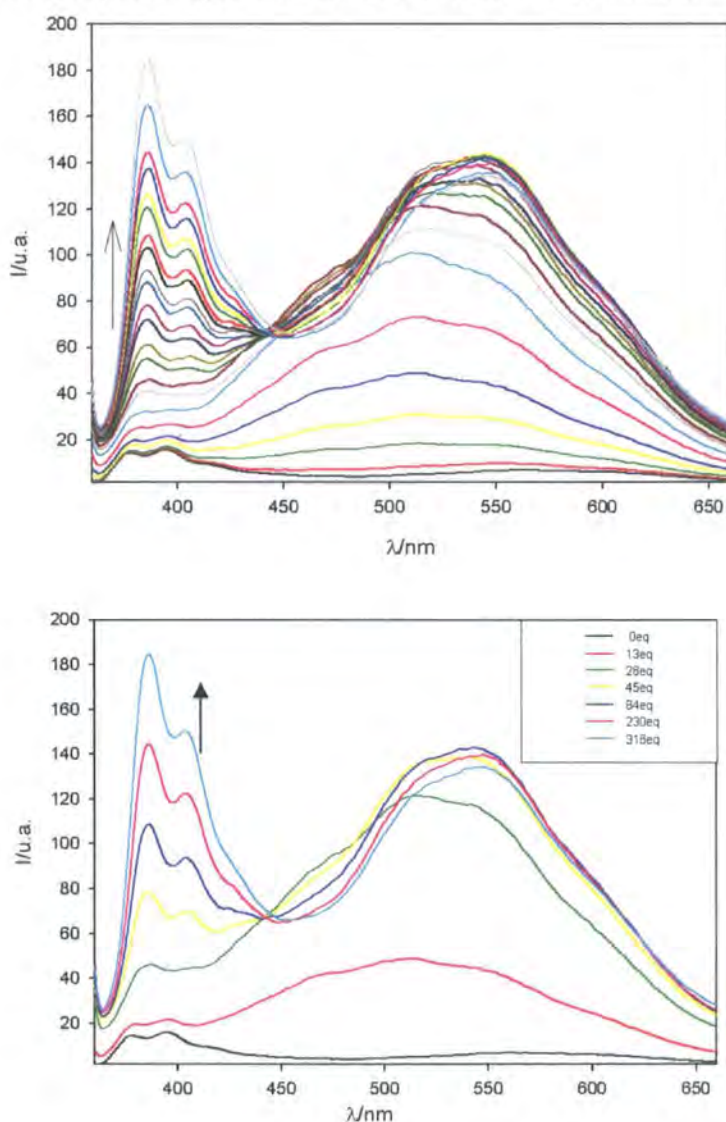
Figure 47 Fluorescence spectra ( \lambda_{\text{exc}} = 343 \text{ nm} ) of 2.20\text{e}\cdot 4\text{PF}_6^- [ 1.27 \times 10^{-5} \text{ M} ] in \text{CH}_3\text{CN} upon addition of increasing amount of tba Cl (lower graph: selected spectra).
