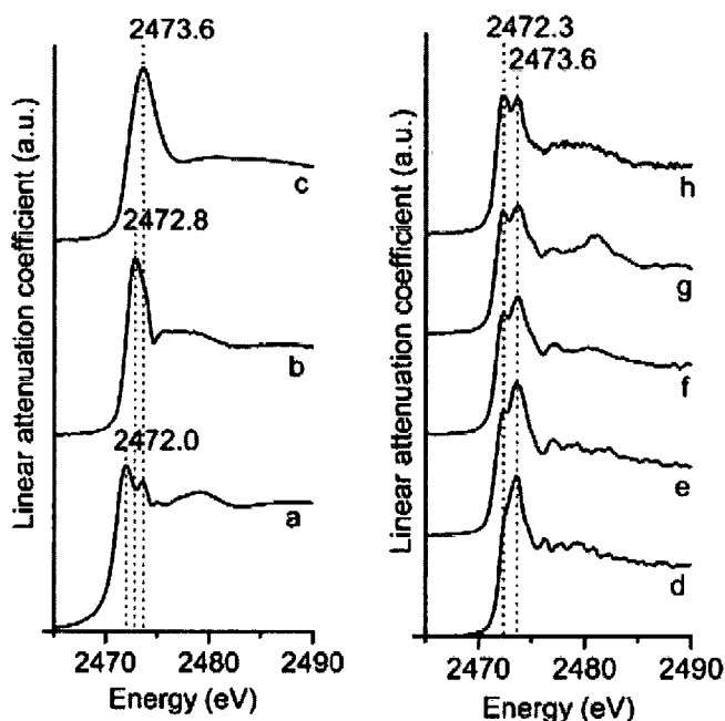
Figure 60 Sulfur K-edge XANES spectra of (a) thioctic acid, (b) dihydroliipoic acid, (c) Au@DHLA (solid state), (d) Au@DHLA (liquid state) in the presence of (e) r=5\% , (f) 13\% , (g) 33\% and (h) 50\% of free DHLA (with r=[\text{DHLA}]_{\text{free}}/([\text{DHLA}]_{\text{free}}+[\text{DHLA}]_{\text{grafted}}) ) (reproduced from ref 141).
