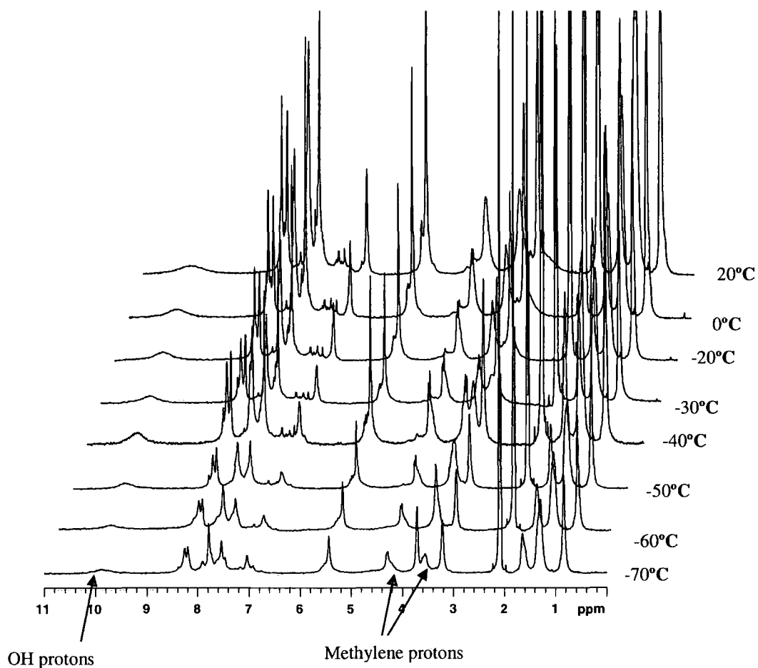
Figure 28 ^1\text{H} NMR VT experiment of 2.17\text{c}\cdot 4\text{PF}_6^- in d_6 -Acetone.
