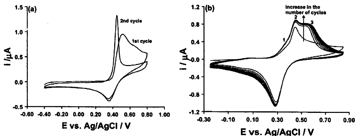
Figure 5 (a) Cyclic voltammetry of solid \text{1.13}\cdot\text{3PF}_6^- adhered to a 1 mm diameter GC electrode in the presence of 0.01 M \text{NaCl} . (b) Cyclic voltammetry (20 cycles) of solid \text{1.13}\cdot\text{3PF}_6^- adhered to a 1 mm diameter GC electrode in the presence of 0.4 M aqueous \text{KPF}_6 . (Scan rates 0.1 \text{ V s}^{-1} ) (reproduced from ref 18).
