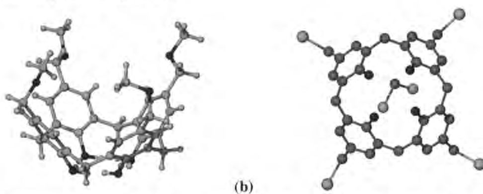
Figure 20 X-ray crystal structures of the methoxy ethyl calix[4]arene a) and bromomethylated calix[4]arene 2.15 with a dichloromethane molecule included in the cavity. The position of protons could not be resolved due to poor quality of the crystal b).
