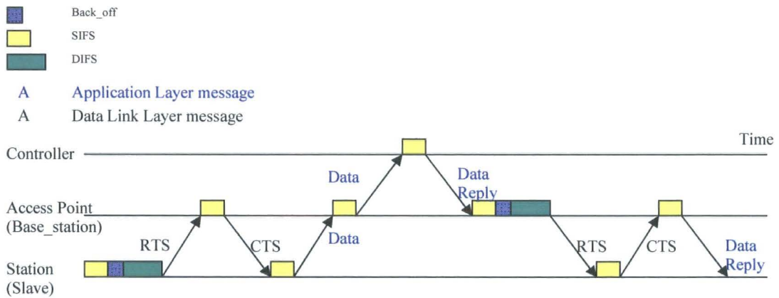
Figure 6.15 Data Transmission
