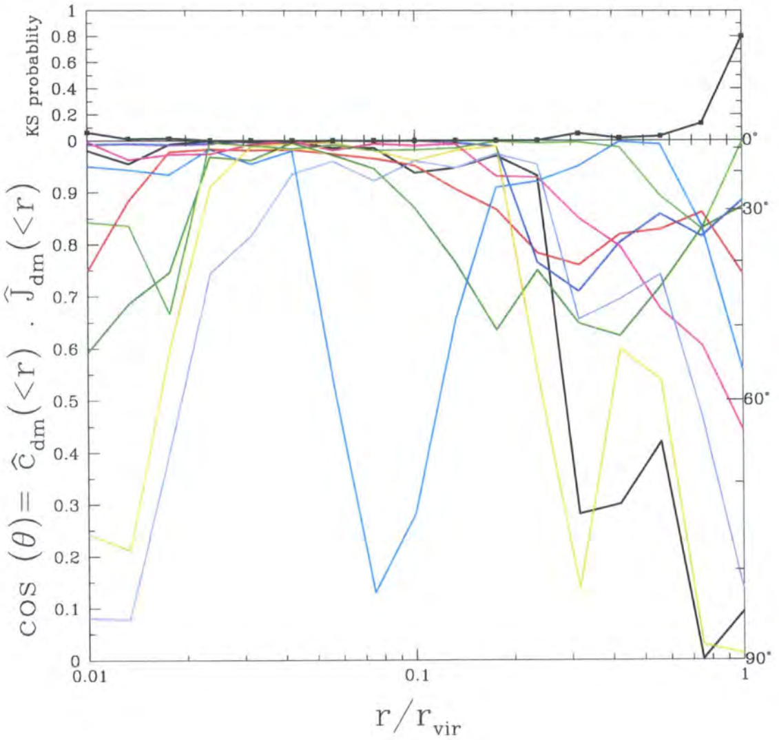
Figure 3.11: The angle between \hat{\mathbf{J}}_{\text{dm}} and \hat{\mathbf{c}}_{\text{dm}} for material within a given radius. Each of the nine galactic haloes is plotted using a different colour, according to the same code used in Fig. 8.
