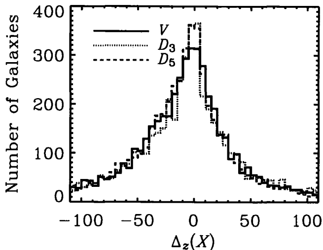
Figure 3.3: The effects of redshift space distortion on each of the Voronoi method and the 3-dimensional n^{\text{th}} nearest neighbour method for n=3, 5 . \Delta_z(X) is defined in equation 3.28 and is plotted here for 5,031 galaxies in the DEEP2-selected simulation within 0.7 < z < 1.4 and more than 4 h^{-1} comoving Mpc from any survey edge [29]
