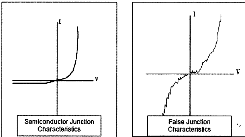
Fig. 2.3 IV- graphs for non-linear junctions [17]
