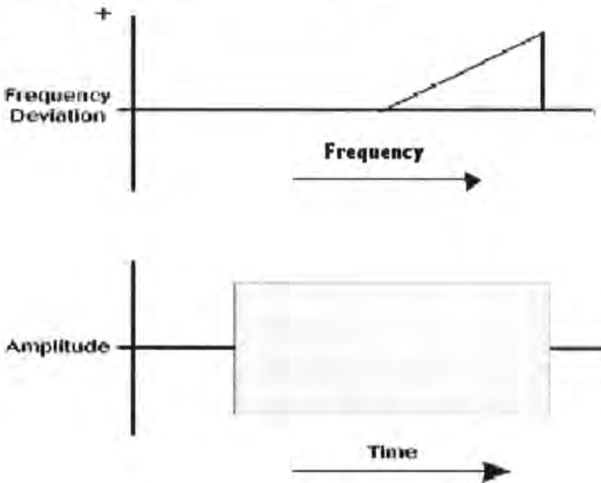
Fig 2.1 A Chirp Signal
