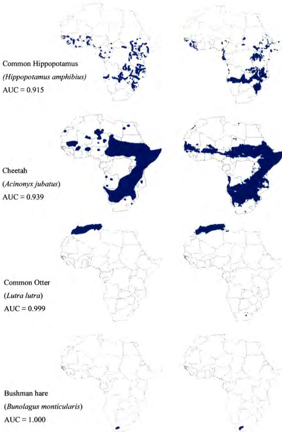
Figure 2.2. Observed (left hand maps) and simulated (right hand maps) current distributions of a sample of 4 species (names on the left of each map) along with their corresponding AUC value. Blue indicates the observed/simulated distribution of each species.
