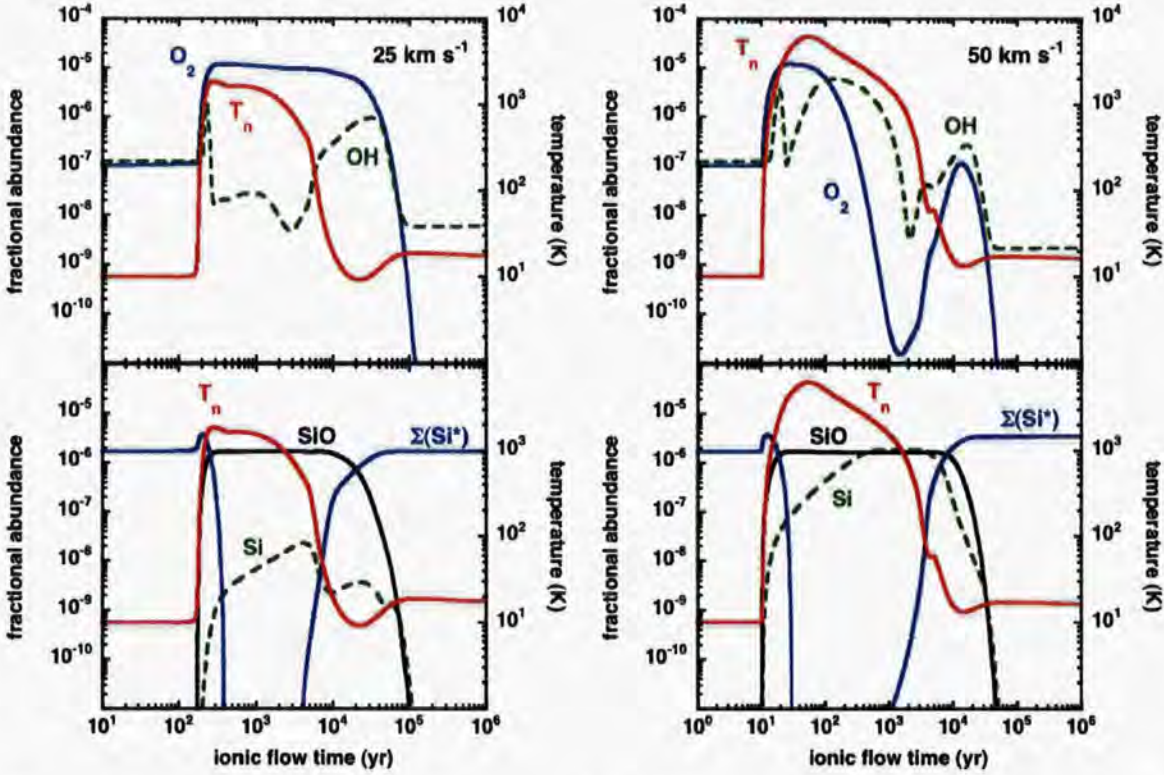
Figure 9.1 – The temperature of the neutral fluid, T_n , and the fractional abundances of \text{OH} and \text{O}_2 (top panels) and of \text{Si} , \text{SiO} , and total amount of silicon in the grain mantles, \Sigma \text{Si}^* (bottom panels), as functions of the flow time of the charged fluid, for two reference C-type shock models : n_{\text{H}} = 10^4 \text{ cm}^{-3} , b = 1 , v_s = 25 \text{ km s}^{-1} (left-hand panels) and 50 \text{ km s}^{-1} (right-hand panels). In both models, it is assumed that 5% of the elemental silicon is initially in the mantles, in the form of \text{SiO} .
