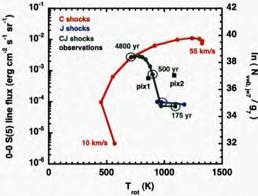
Figure 4.5 – Comparative compact excitation diagrams of C-, J-, and CJ-type shock models. The C-type shock models (red) are displayed for n_H = 10^4 \text{ cm}^{-3} , b = 1 , and shock velocities from 10 to 55 \text{km s}^{-1} , with 5 \text{km s}^{-1} increments, and J-type shock models (blue) with n_H = 10^4 \text{ cm}^{-3} , b = 0.1 , and shock velocities 20, 25, and 30 \text{km s}^{-1} . Also shown are the results for an evolutionary sequence (various ages) of non-stationary CJ-type shock models (green) for n_H = 10^4 \text{ cm}^{-3} , b = 1 , and shock velocity of 25 \text{km s}^{-1} . The observed data are the black pixels.
