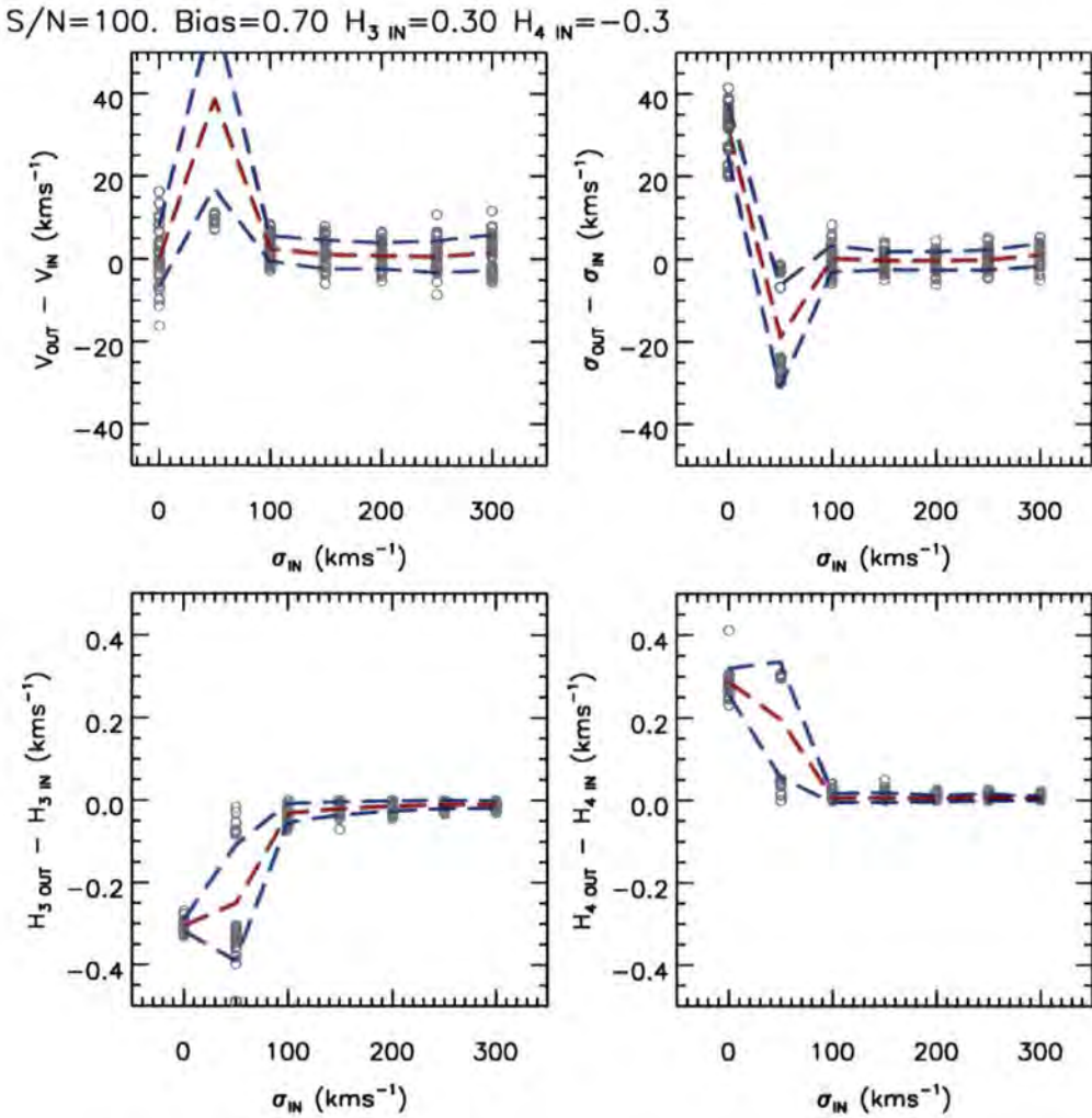
Figure 3.4: As in Figure 3.3, except that in this simulation the vel-scale parameter has been changed to 100kms -1 , in this case matching our earlier epoch data which was binned by 4 in the spectral dimension.
