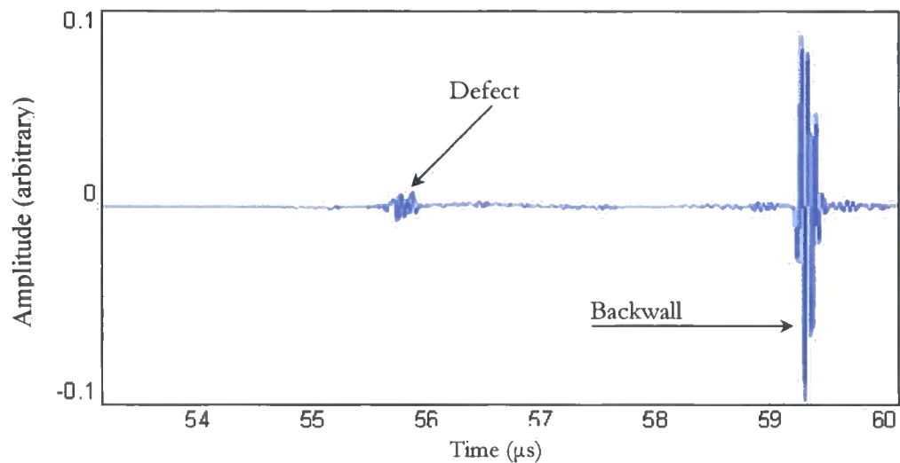
Figure 9.8. Filtered A-scan from Probe D
