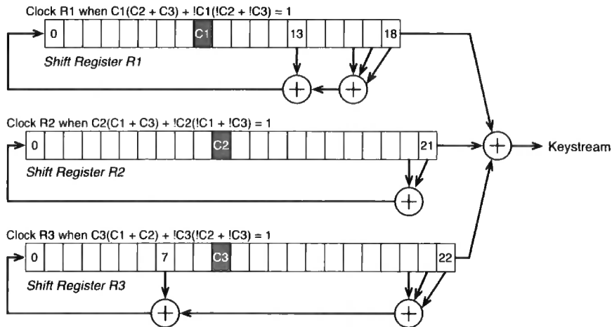
Figure 4.5: Schematic description of the A5/1 keystream generator
