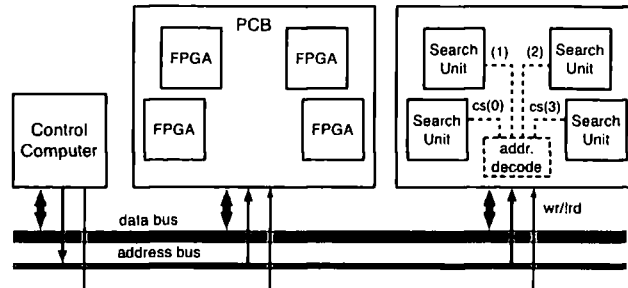
Fig. 3. Inter-unit buses and possible chip layout for DELUGE.
