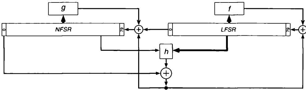
Figure 4.11: Schematic diagram of Grain v0 at initialisation
