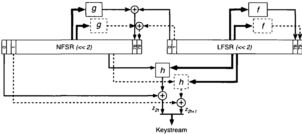
Figure 4.12: Schematic diagram showing Grain v0 with the throughput doubled, this acceleration of Grain v0 can further extended through use of additional feedback loops
