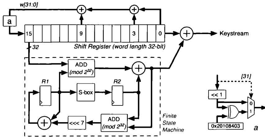
Figure 4.7: Schematic description of the SNOW keystream generator
