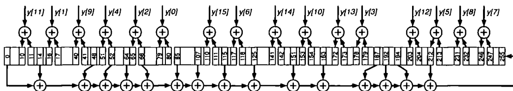
Figure 4.20: SFINKS' LFSR during initialisation
