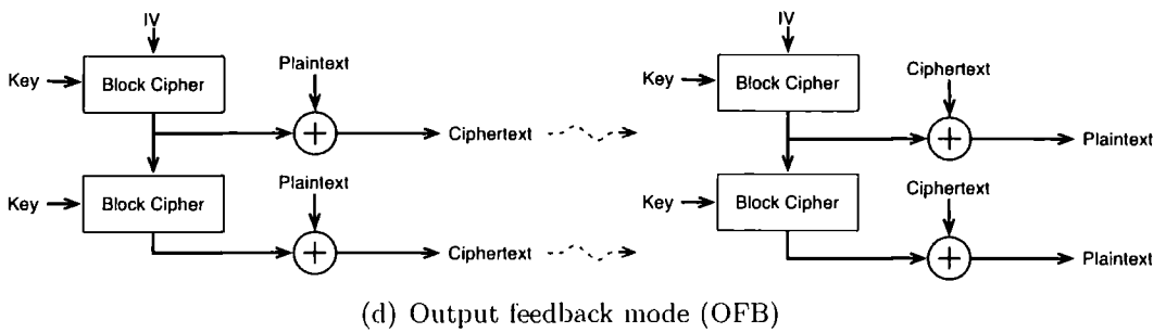
Figure 4.3: Block cipher additional modes of operation
