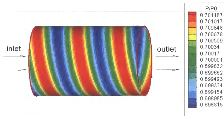
Figure 4.12 Cut-on Simulation 2
