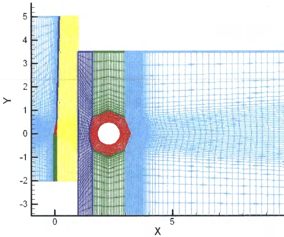
Figure 5.2 One Blade and Tower 2D Mesh
