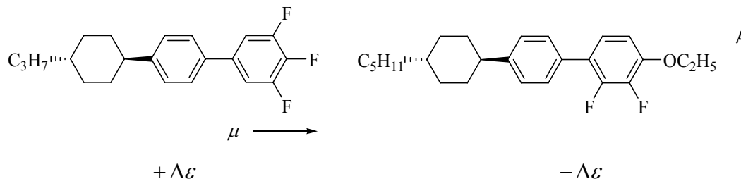
Figure 1. Dielectrically positive and dielectrically negative LCs
