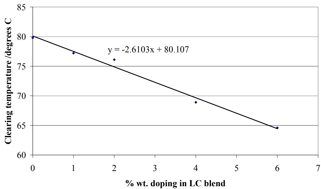
Graph 2. T_{NI} versus percentage doping of a dielectrically negative LC blend with 32 .
