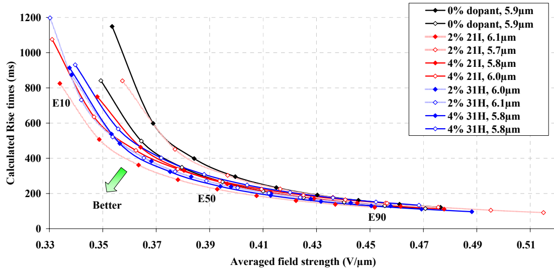
Figure 61. Comparison of materials 86 (21I) and 88 (31H)
