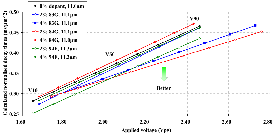
Figure 69. Comparison of materials 92 (94E), 93 (83G) and 94 (84G)
