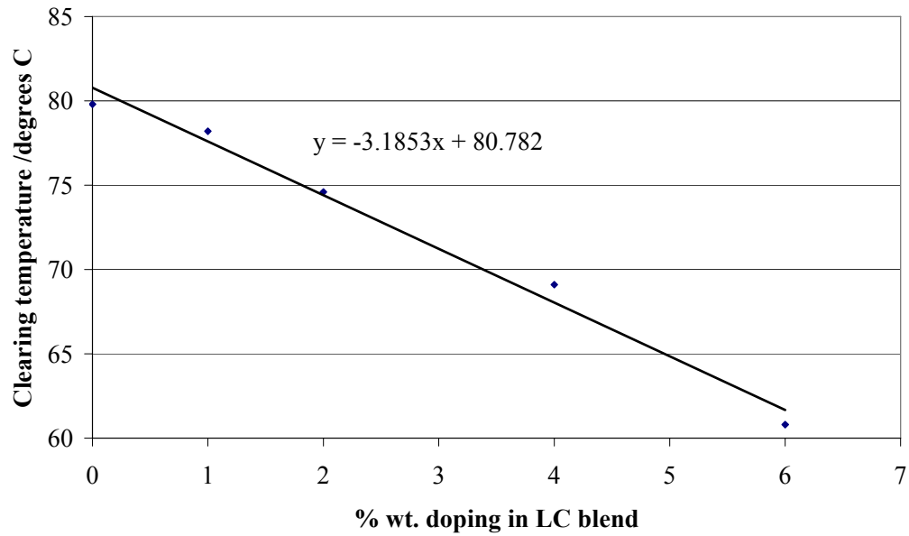
Graph 5. T_{NI} versus percentage doping of a dielectrically negative LC blend with 47 .
