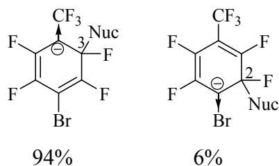
Figure 9. Meisenheimer intermediates following nucleophilic attack on 1-bromo-2,3,5,6-tetrafluoro-4-(trifluoromethyl)benzene at positions 3 and 2 respectively.
