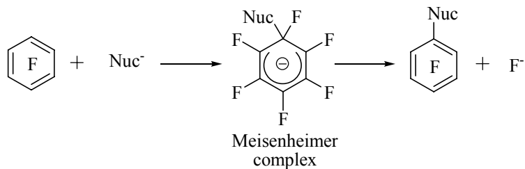
Scheme 3. Nucleophilic substitution in hexafluorobenzene
