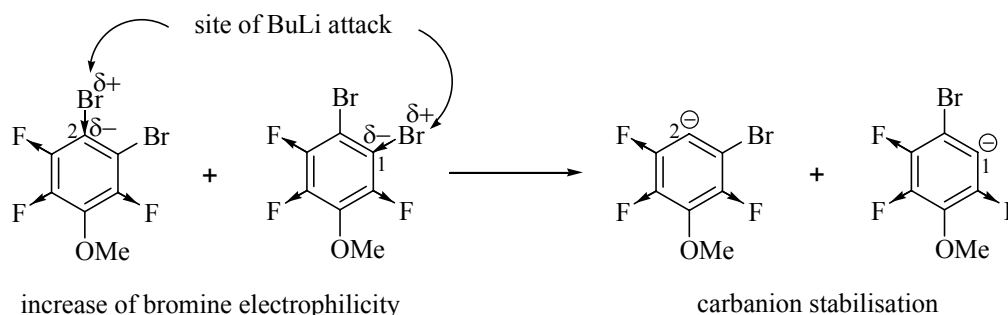
Figure 14. Starting material showing the activating and stabilisation effects of fluorine for the formation of isomers 56 and 57
