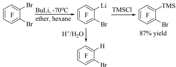
Scheme 10. 54 Functionalisation of 1,2-dibromotetrafluorobenzene
