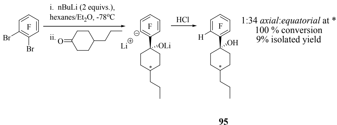
Scheme 35. Alternative alcohol synthesis using two equivalents of butyllithium
