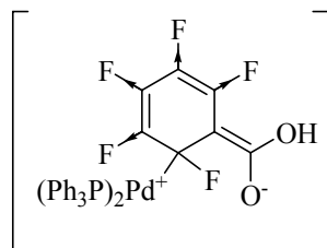
Figure 24. Proposed fluorine lone pair, oxyanion and fluorine electron withdrawing stabilisation effects following addition of palladium catalyst to perfluorobenzoic acid
