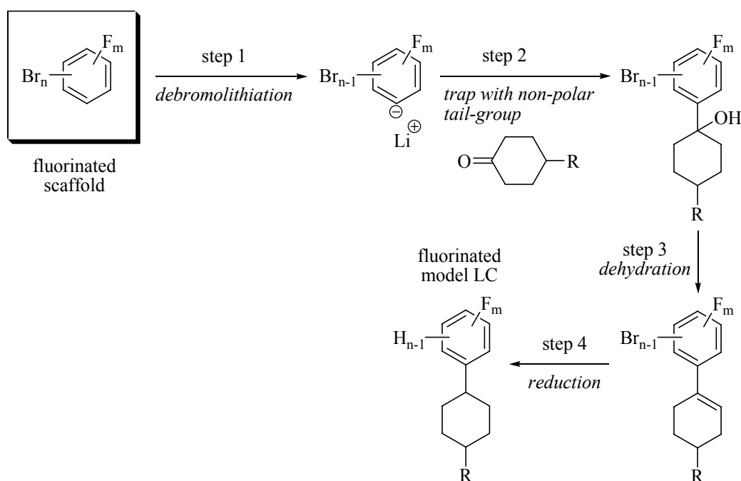
Scheme 23. Synthetic route to fluorinated cyclohexylphenyl structures via debromolithiation
