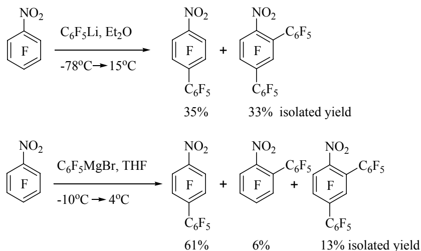
Scheme 37. 27, 110 Synthesis of fluorinated biphenyls via carbon nucleophiles
