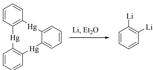
Scheme 27. 96 Synthesis of o -phenylenedilithium
