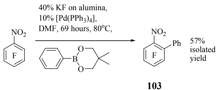
Scheme 45. Scale up of Suzuki-Miyaura cross coupling using optimised conditions.
