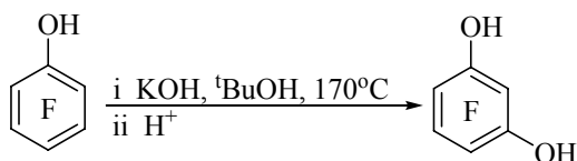
Scheme 5. 12 meta substitution in pentafluorophenol
