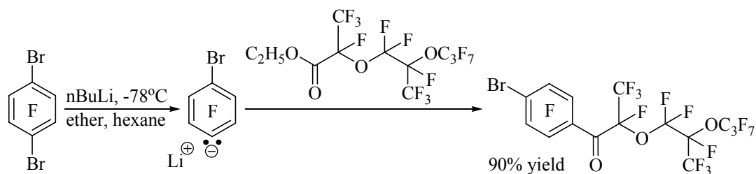
Scheme 11. 55 Functionalisation of 1,4-dibromotetrafluorobenzene
