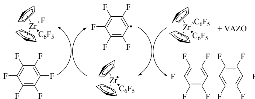
Scheme 17. 85 Zirconium-activated homocoupling of perfluorobenzene
