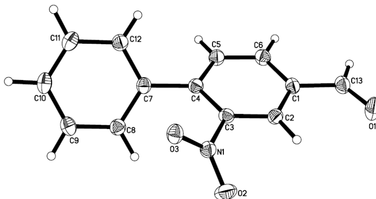
Figure 21. X-Ray crystal structure of nitrophenylbenzaldehyde 96
