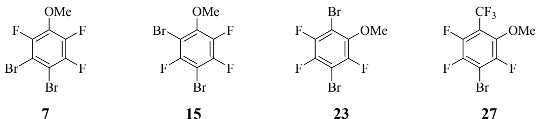
Figure 8. Potential LC head-group scaffolds
