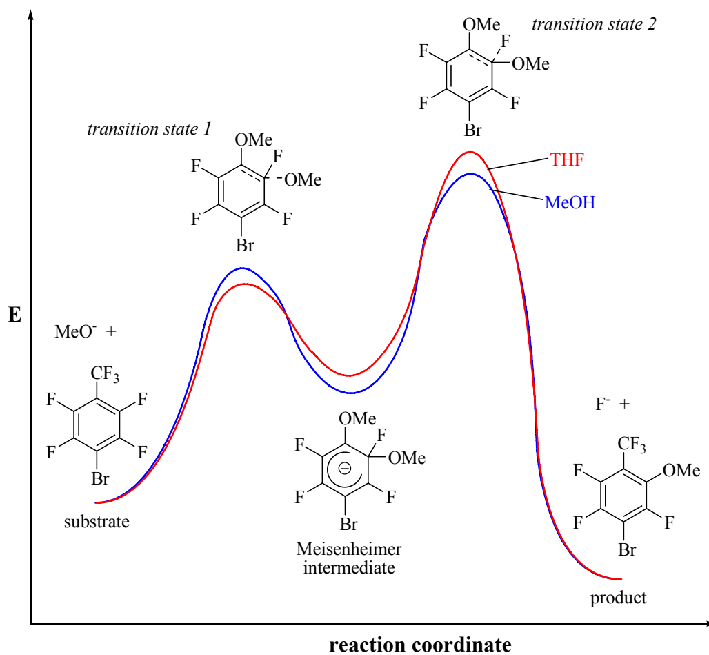
Figure 10. Solvent effects in the reaction of an alkoxide with a fluoroaryl
