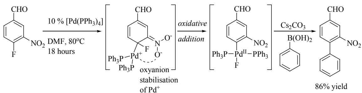
Scheme 14. 68 Suzuki-Miyaura-type C–C coupling through C–F bond activation.
