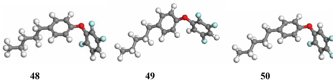
Figure 27. 114 Molecular modelling of three trifluoro(4-pentyl-phenoxy)-benzenes
