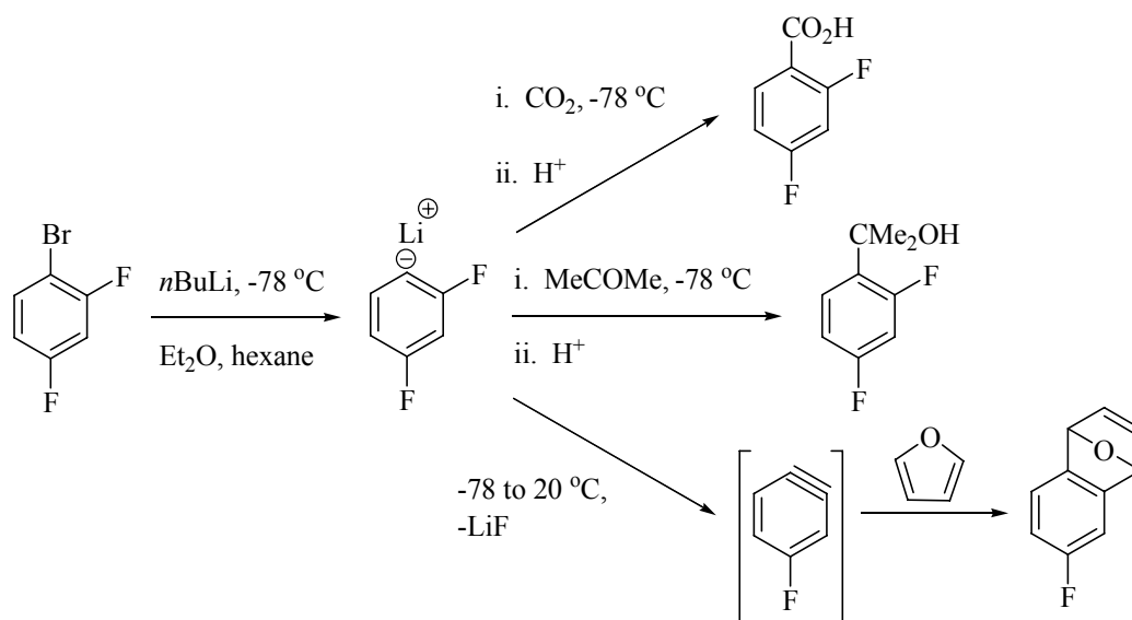
Scheme 7. 49, 50 Reactions of fluoroaryllithium species with electrophiles
