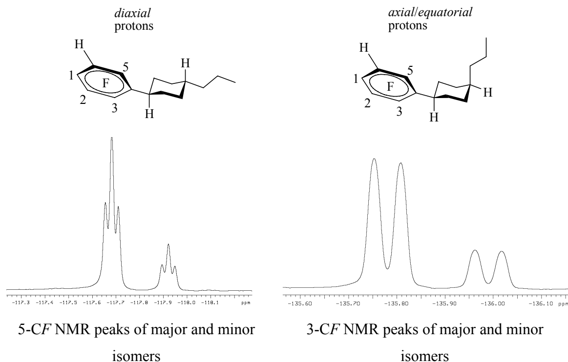
Figure 18. The configurational isomers of 85 which arise following the reduction of alkene 74 and the additional fluorine NMR signals observed
