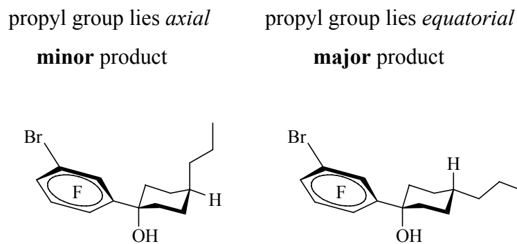
Figure 15. Two possible configurational isomers of 63
