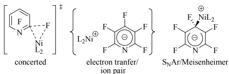
Figure 7. 73 Possible intermediates and transition state for the C–F activation of pentafluoropyridine at nickel
