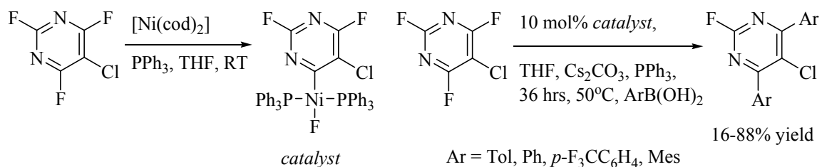
Scheme 19. 87 Coupling of a fluoropyrimidine to arylboronic acids via C–F bond activation
