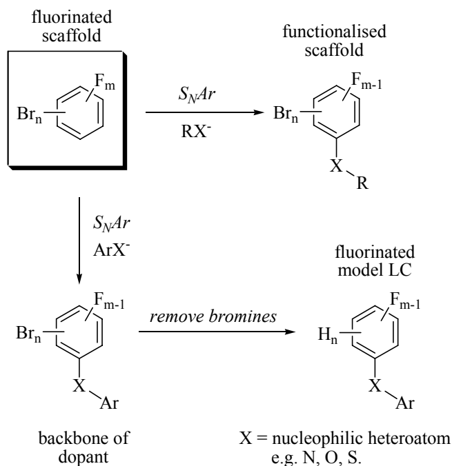
Scheme 22. Synthetic route to heteroatom bridged fluorinated biphenyl structures via nucleophilic aromatic substitution
