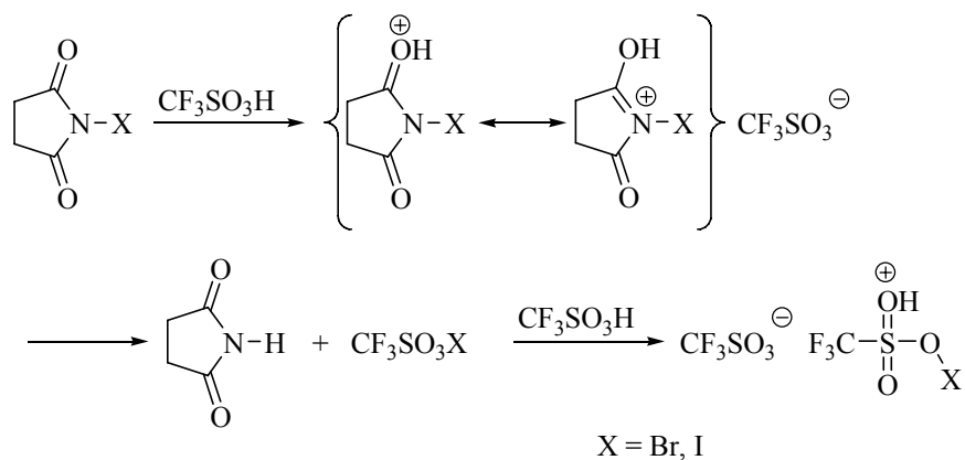
Scheme 25. 91 Proposed mechanism for generation of active species in the halogenation of fluorobenzenes
