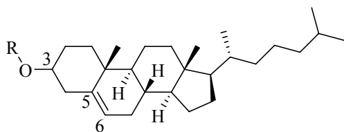
Numbering of carbons in cholesteric molecules
