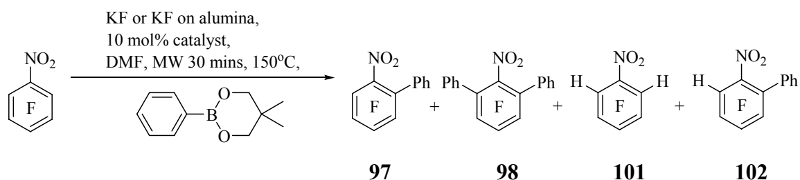
Scheme 44. C–C coupling with perfluoronitrobenzene using alternative base and source of phenyl nucleophile
