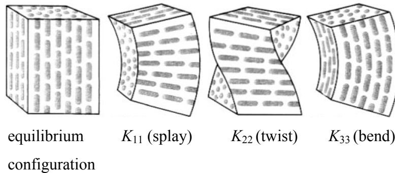
Figure 25. 6 Elastic deformations of calamitic, rod-like LCs in the nematic phase.
