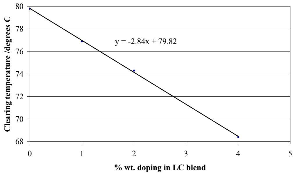
Graph 6. T_{NI} versus percentage doping of a dielectrically negative LC blend with 48 .
