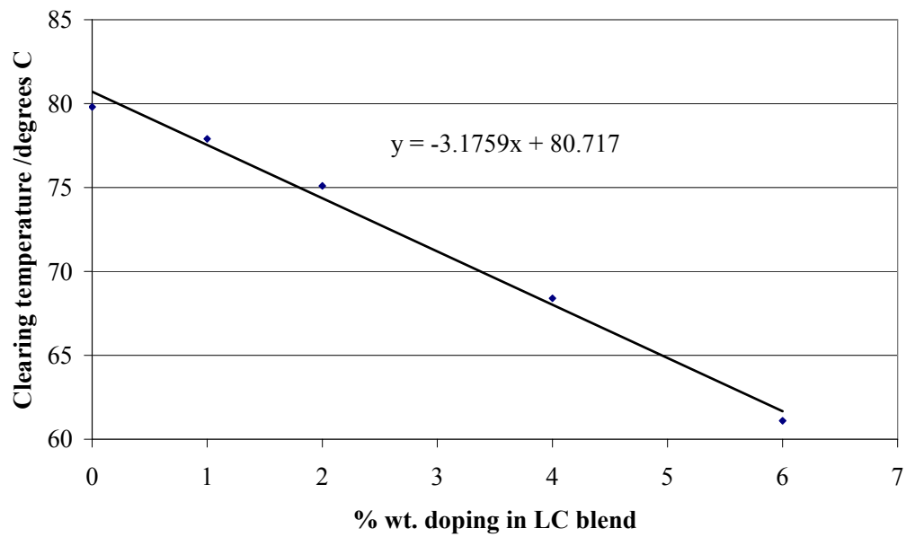
Graph 4. T_{NI} versus percentage doping of a dielectrically negative LC blend with 45 .
