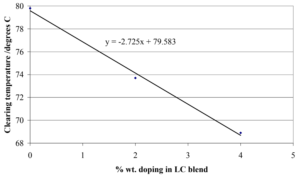
Graph 7. T_{NI} versus percentage doping of a dielectrically negative LC blend with 49 .
