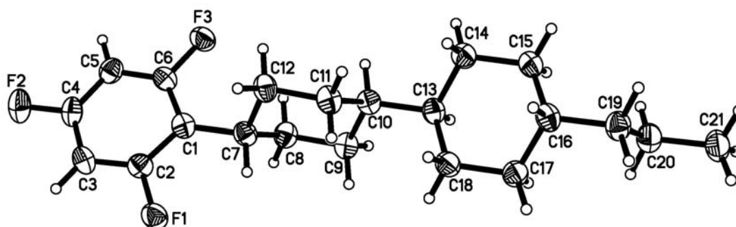
Figure 20. X-Ray crystal structure of bicyclohexylaryl 94
