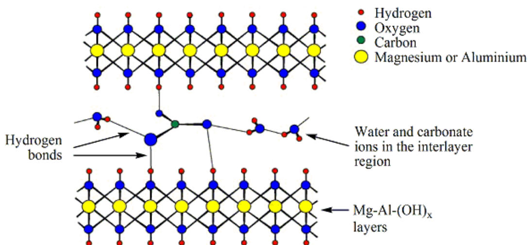
Figure 6. 72 Structure of Mg/Al layered double hydroxide (LDH)
