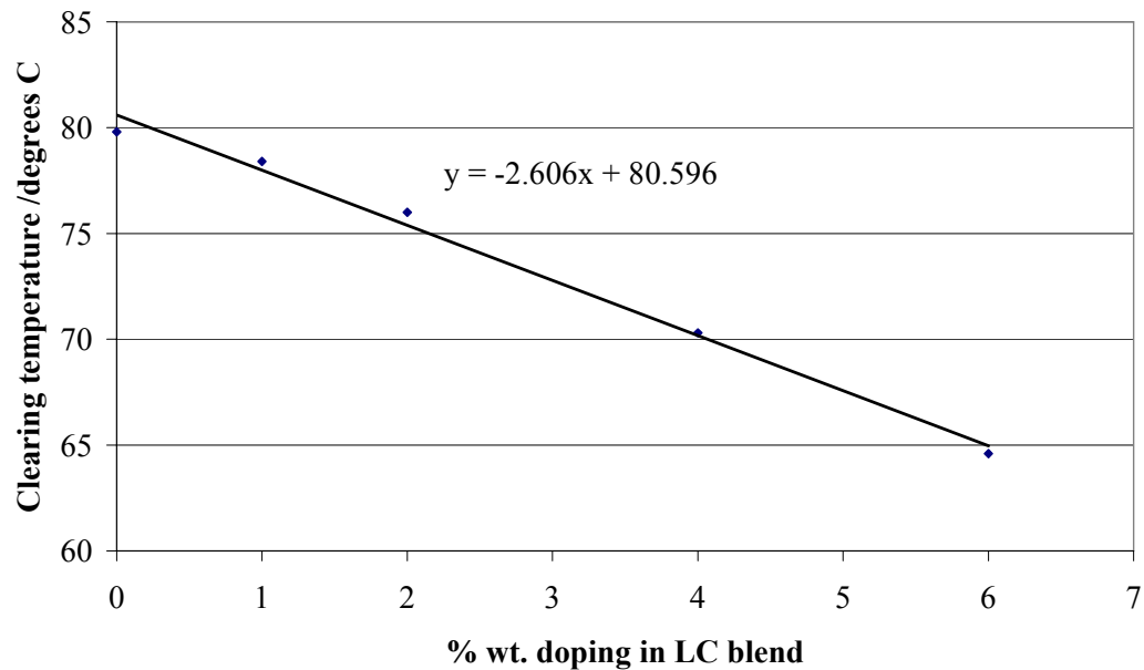
Graph 1. T_{NI} versus percentage doping of a dielectrically negative LC blend with 31 .
