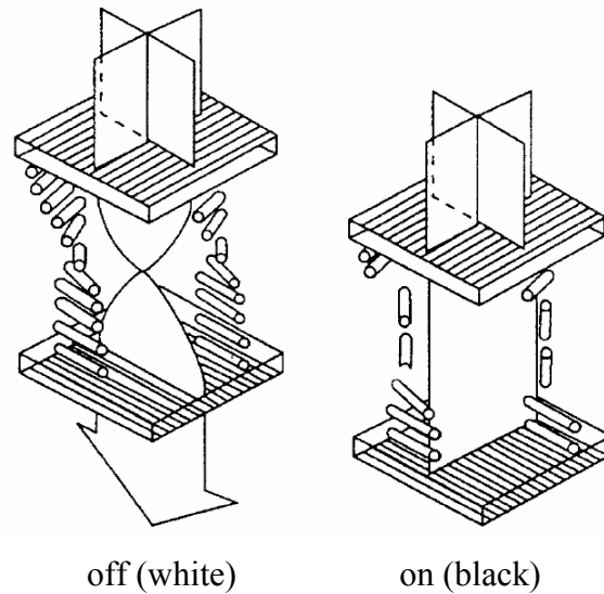
Figure 2. 1 Schematic representation of a TN cell
