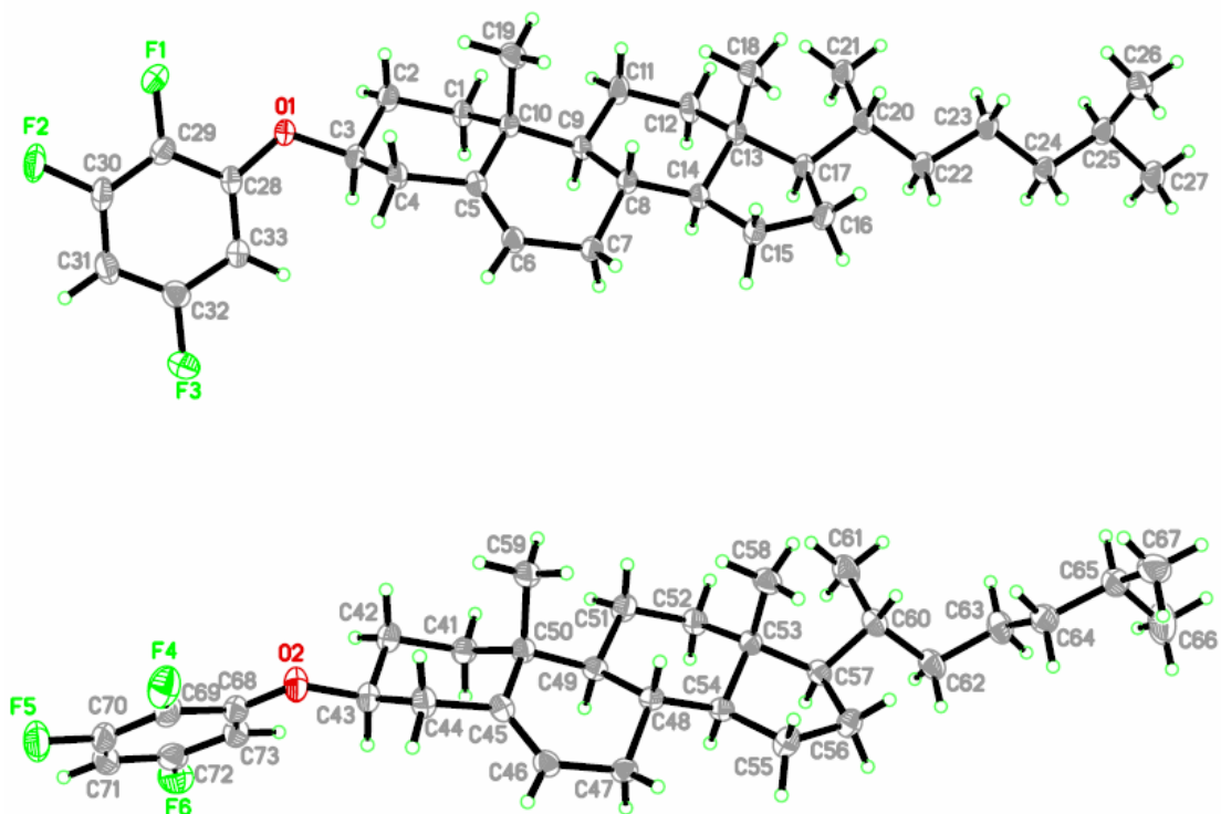
Figure 12. X-ray crystal structure of 3 \beta -(trifluoro-phenoxy)-5-cholestene 52 .
