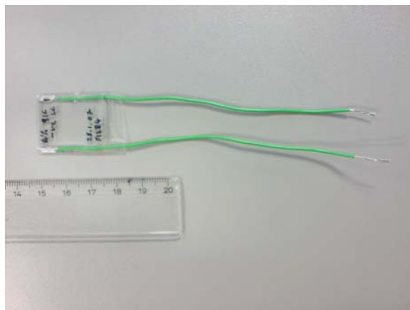
Figure 29. A fully assembled cell filled with fluorinated LC material
