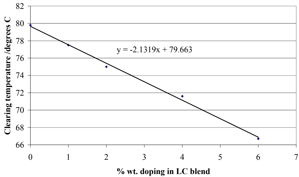
Graph 3. T_{NI} versus percentage doping of a dielectrically negative LC blend with 33 .
