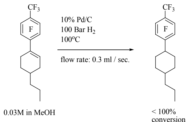
Scheme 34. Attempted reduction of fluorinated alkene 76 in an ‘H-Cube’.
