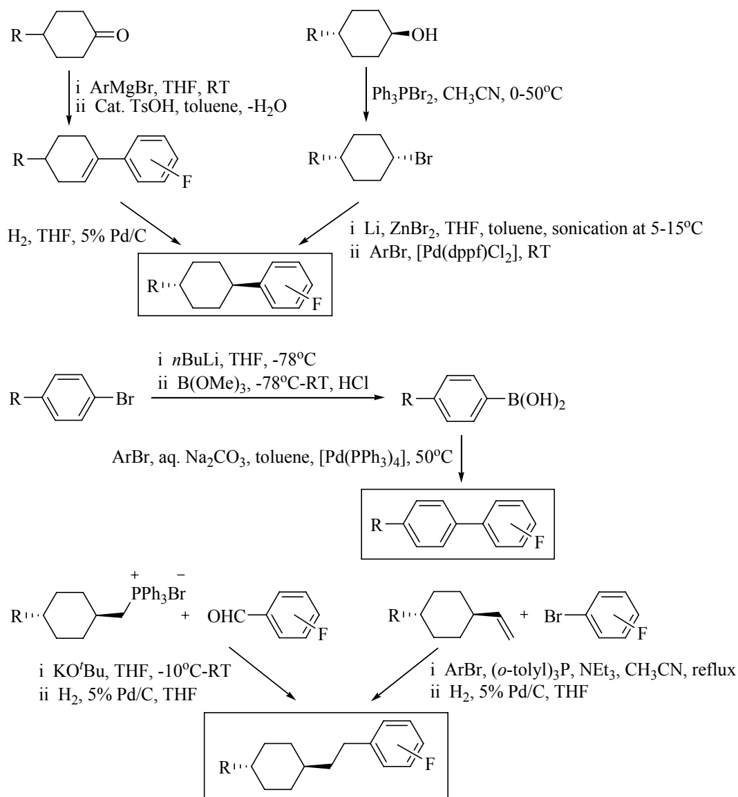
Scheme 1. 1 Typical synthetic routes to nematic LCs.
