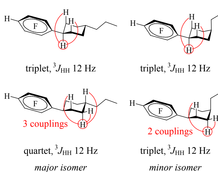
Figure 19. Couplings between protons in major and minor isomers of 86
