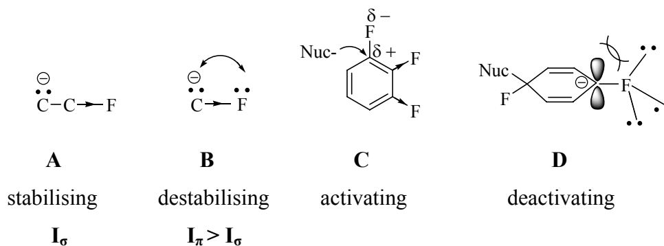
Figure 4. Electronic effects of fluorine atoms
