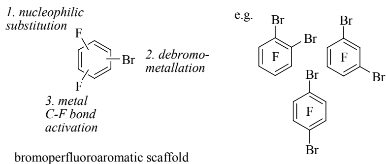
Scheme 21. Methodologies employed for the synthesis of fluorinated materials
