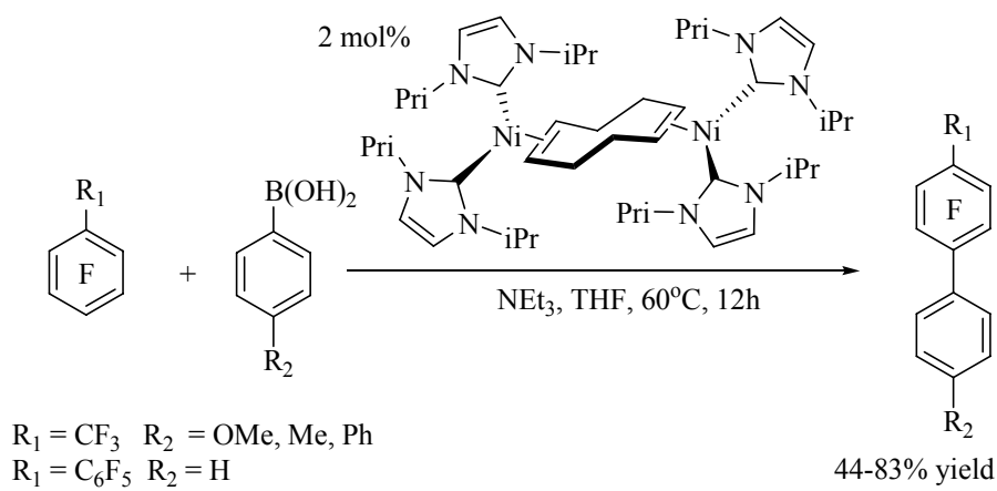
Scheme 20. 90 A cross-coupling reaction using a C-F bond activating N-heterocyclic carbene-stabilized nickel complex
