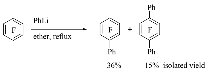
Scheme 36. Synthesis of a fluorobiphenyl via S_NAr of fluorine
