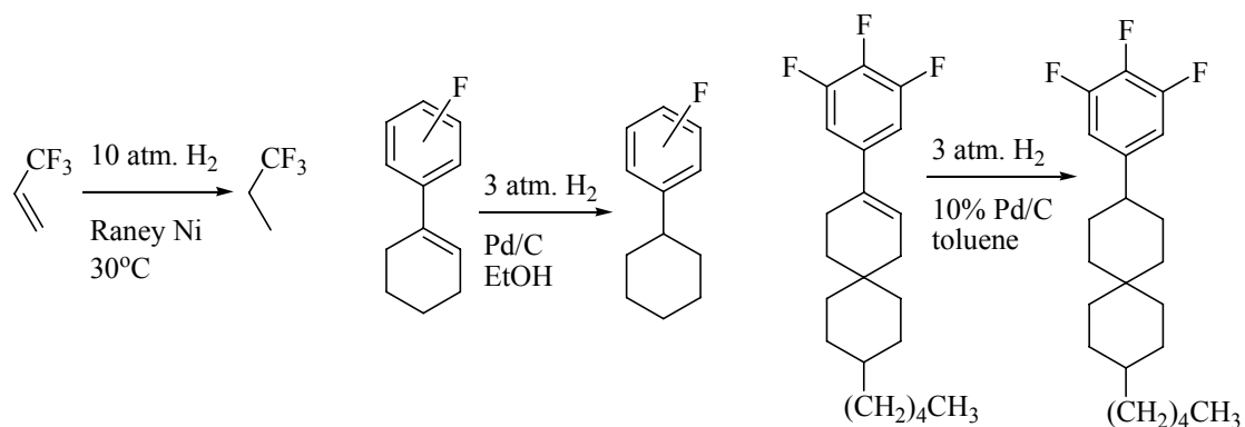
Scheme 31. 102-104 Reductions of unsaturated fluorinated compounds.
