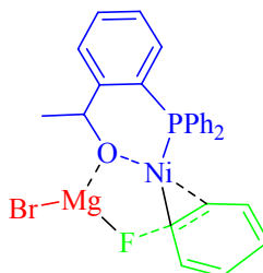
Figure 5. 63 Bimetallic cooperation in the stabilisation of a fluoroarene transition state
