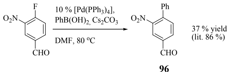
Scheme 39. Suzuki-Miyaura Cross coupling reaction through C–F bond activation
