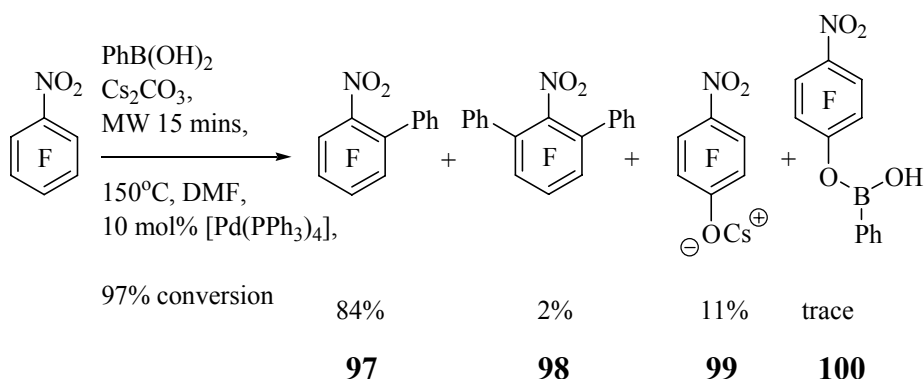
Scheme 40. Attempted coupling of a boronic acid to perfluoronitrobenzene
