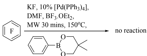
Scheme 47. Attempted C-F bond palladium activation with a Lewis Acid
