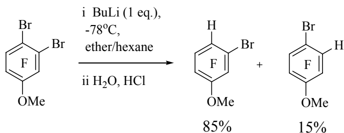
Scheme 30. Selective bromine-lithium exchange
