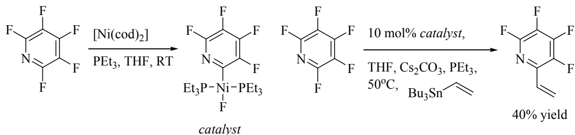
Scheme 18. 86 Coupling of a fluoropyridine to vinyl tin via C–F bond activation
