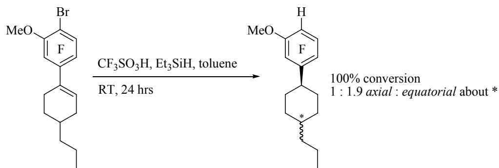
Scheme 33. Reduction of alkene 79 with triflic acid and triethylsilane.
