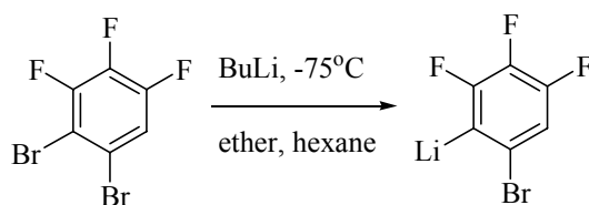
Scheme 9. 49, 52 Br-Li exchange occurring preferentially to H-Li exchange
