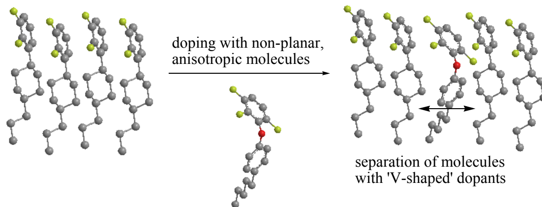
Figure 28. 114 Doping of commercial LC blends with trifluoro(phenoxy)-benzenes
