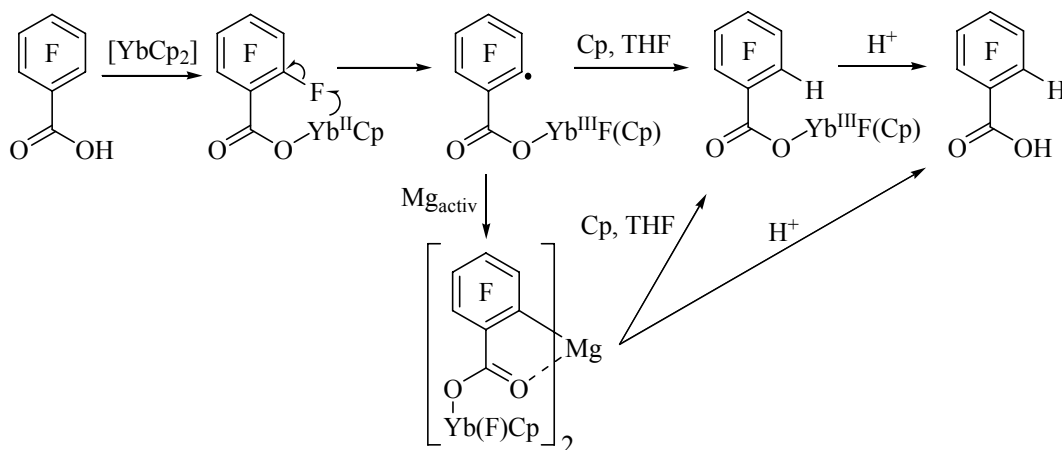
Scheme 16. 83 Selective defluorination of perfluorobenzoic acid
