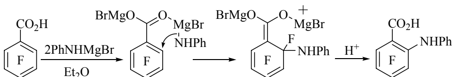
Scheme 6. 9 ortho substitution in pentafluorobenzoic acid
