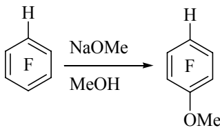
Scheme 4. 11 para substitution in pentafluorobenzene
