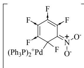
Figure 22. Intermediate Meisenheimer complex formed following attack of palladium on pentafluoronitrobenzene
