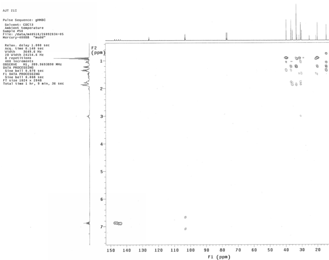
Figure 32. HMBC NMR spectrum
