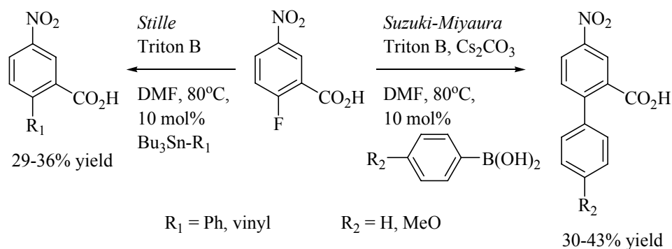
Scheme 15. 71 Stille and Suzuki-Miyaura couplings of 2-fluoro-5-nitrobenzoic acid
