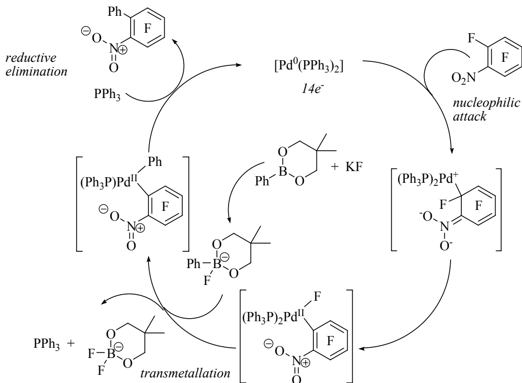
Scheme 43. Mechanism of Suzuki-Miyaura type cross coupling via C-F bond activation
