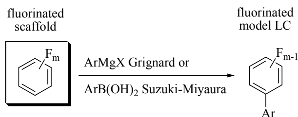
Scheme 24. Synthetic route to fluorinated biphenyl structures via C–F bond activation
