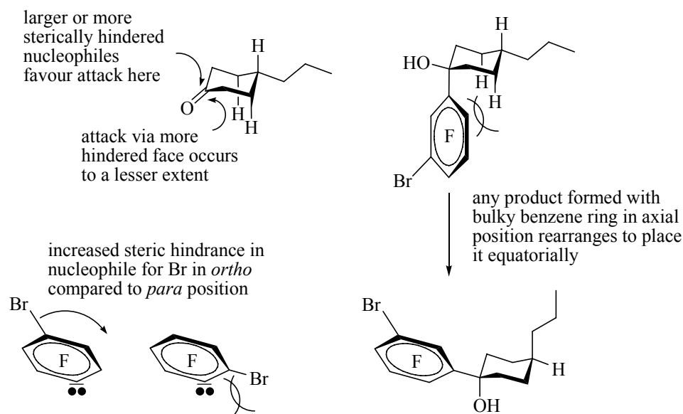
Figure 16. Explanation for the formation of the configurational isomers of 62-64
