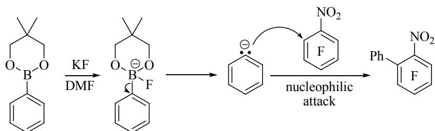
Scheme 46. Possible route to the cross coupled biphenyl product via a non-catalytic mechanism
