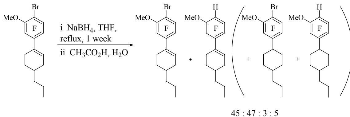
Scheme 32. Attempted reduction of alkene 79 using sodium borohydride.
