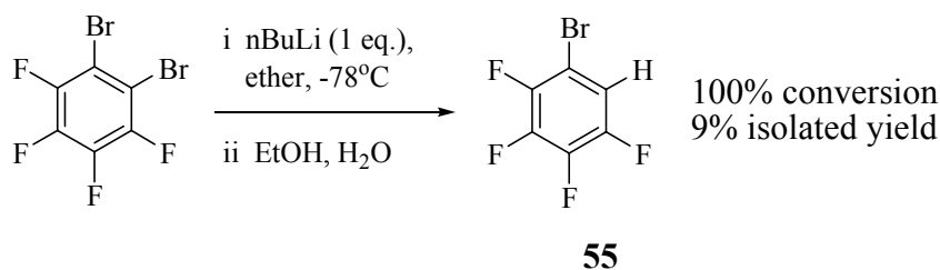
Scheme 29. Protodebromination of 1,2-dibromotetrafluorobenzene
