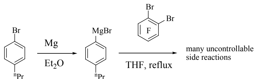
Scheme 26. Grignard reactions do not give the desired biphenyls with dibromotetrafluorobenzene substrates.
