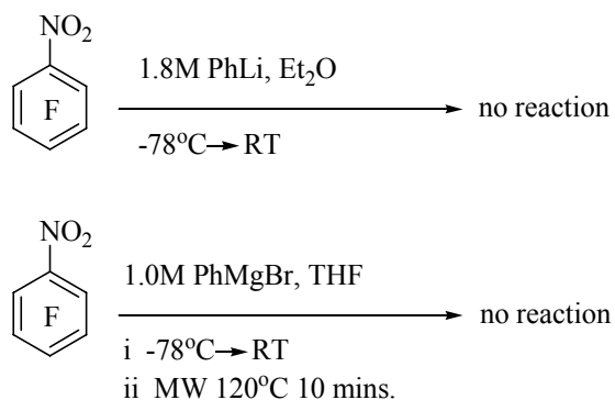
Scheme 38. Attempted synthesis of a fluorinated biphenyl
