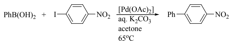
Scheme 12. 56 Metal-catalysed biaryl synthesis
