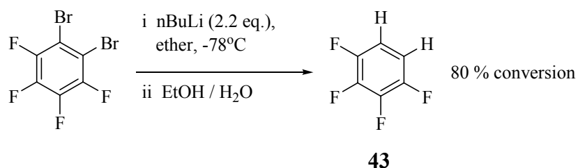
Scheme 28. Removal of two bromine atoms from 1,2-dibromotetrafluorobenzene in a one step procedure
