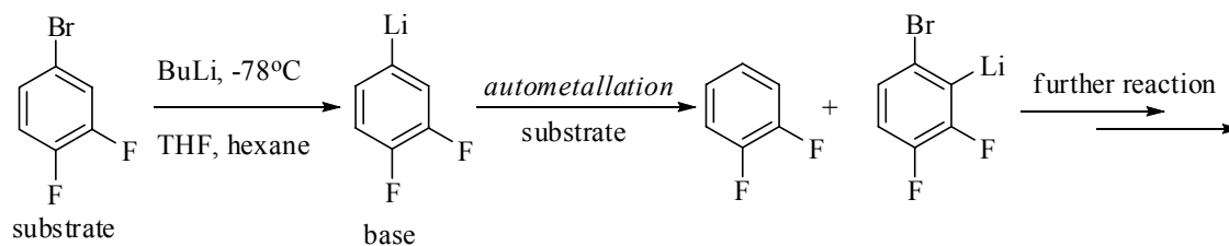
Scheme 8. 51 Autometallation in the lithiation of fluorinated benzenes
