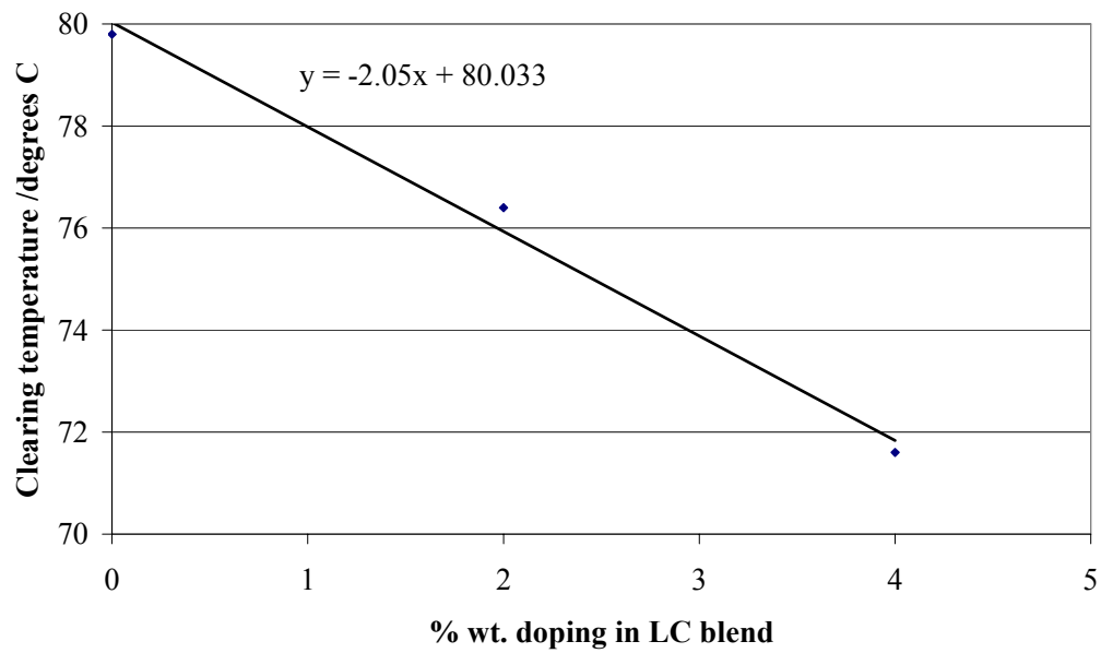
Graph 8. T_{NI} versus percentage doping of a dielectrically negative LC blend with 50 .
