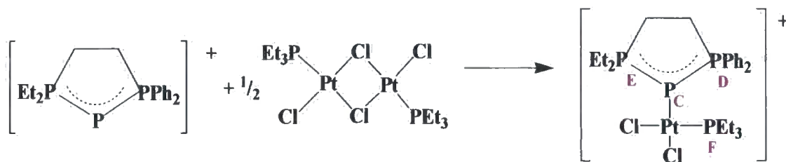
Scheme 1.18: Reaction between the dedppe cyclic triphosphenium ion and trans -[Pt(PEt 3 )Cl(μ-Cl)] 2
