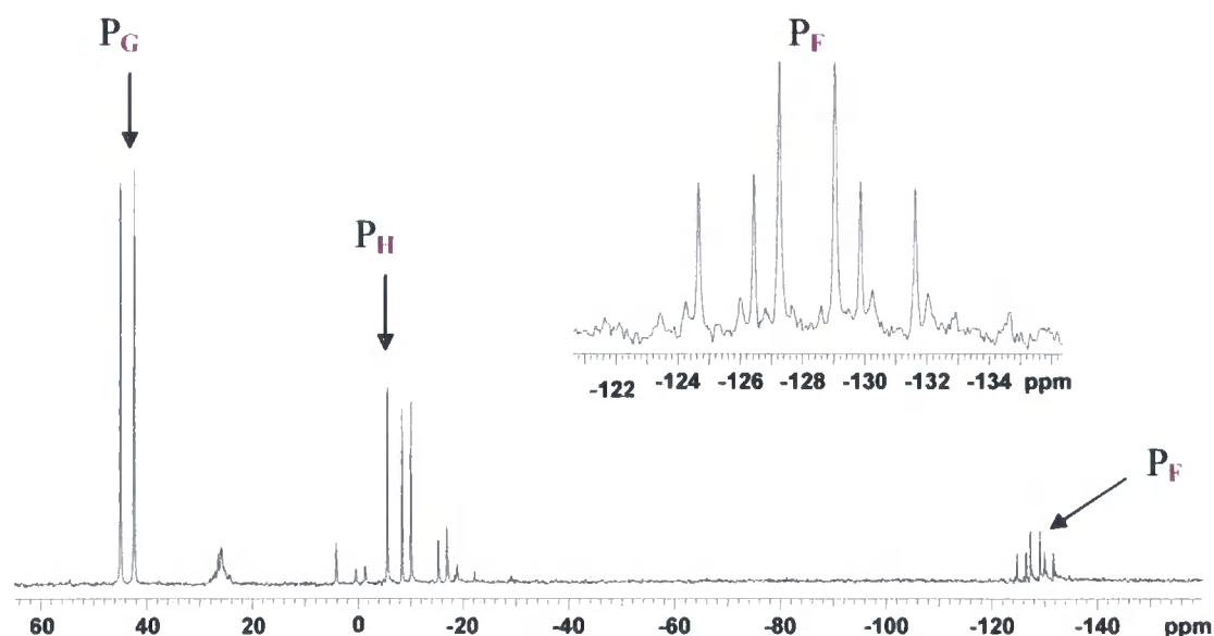
Figure 6.8: ^{31}\text{P} NMR spectrum of the reaction between dcypb cyclic triphosphenium ion and trans -[Pt(PPhMe 2 )Cl( \mu -Cl)] 2 .
