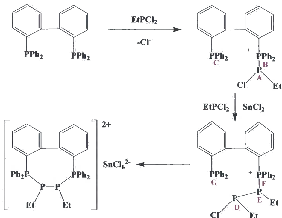
Scheme 1.23: Proposed mechanism for cyclic tetraphosphenium ions derived from biphep
