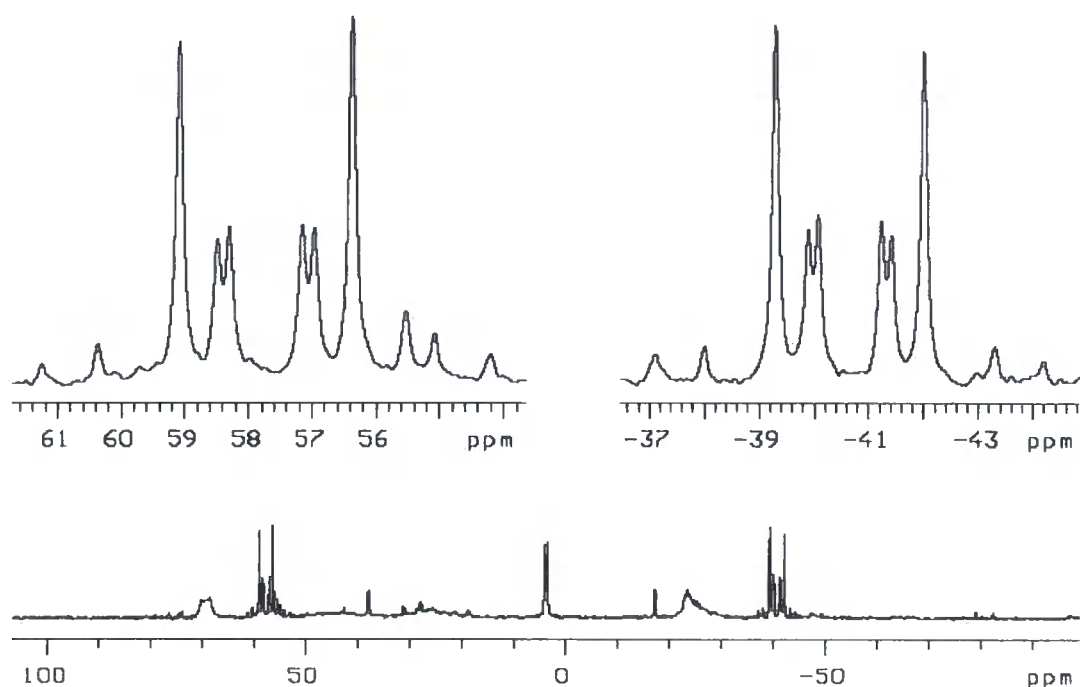
Figure 5.1: ^{31}\text{P}\{^1\text{H}\} NMR spectrum of the reaction mixture in the formation of the dppm ( \text{R}'=\text{Et} ) cyclic tetraphosphenium ion, 50a
