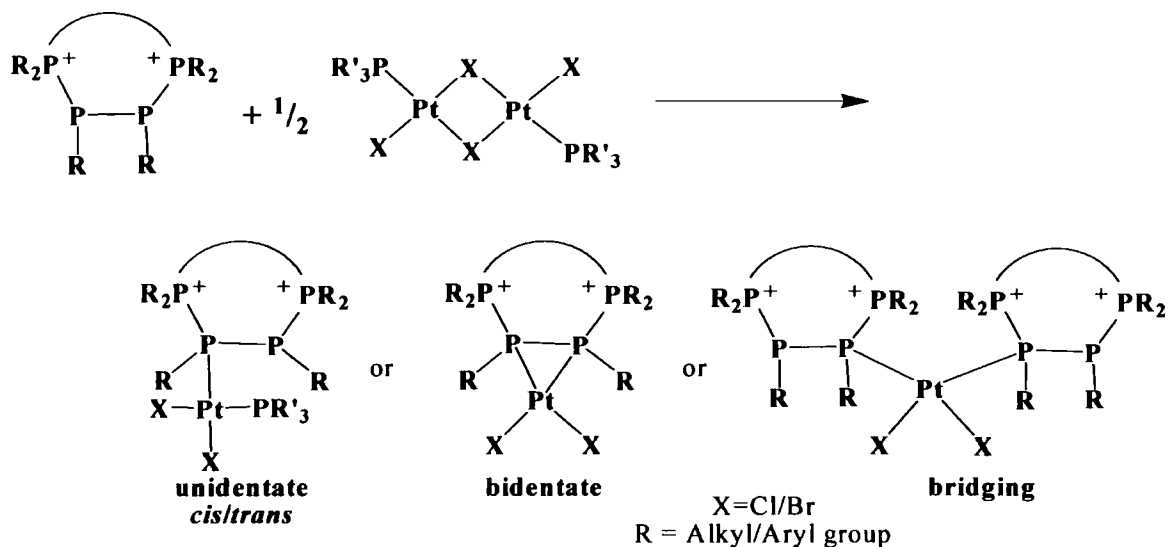
Scheme 7.2: Possible products from the reaction of cyclic tetraphosphenium ions with trans -[Pt(PR 3 )Cl(μ-Cl)] 2
