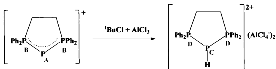
Scheme 1.8: Protonation of the dppe cyclic triphosphenium ion using {}^t\text{BuCl} and \text{AlCl}_3
