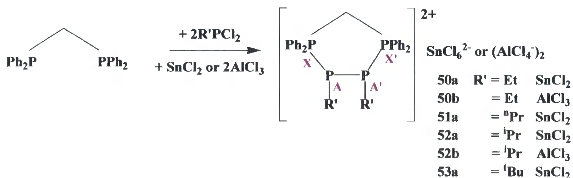
Scheme 5.1: Synthetic route to cyclic tetraphosponium ions derived from dppm
