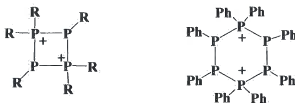
Figure 1.13: Four- 41 and six- 42 membered homocyclic diphosponium cations
