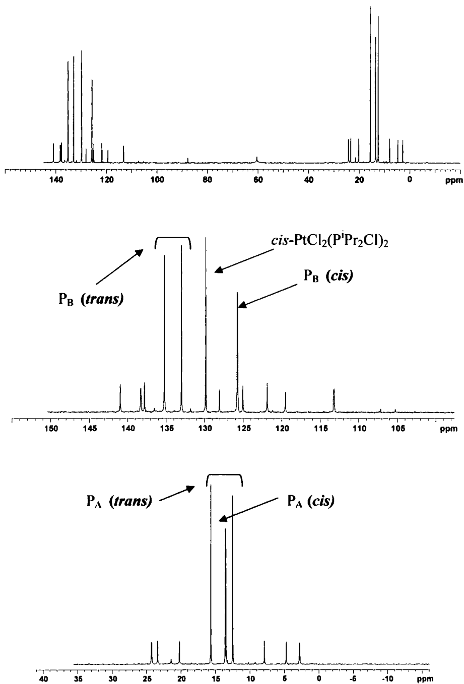
Figure 6.14: Initial ^{31}\text{P}\{^1\text{H}\} NMR spectrum for the reaction between ^1\text{Pr}_2\text{PCl} and \text{trans-}[\text{Pt}(\text{PEt}_3)\text{Cl}(\mu\text{-Cl})_2] showing both cis and trans - \text{PtCl}_2(\text{PEt}_3)(\text{P}^1\text{Pr}_2\text{Cl}) complexes (top: full spectra, middle: expansion of the region between 98 and 165 ppm, bottom: expansion of the region between -16 and 41 ppm)
