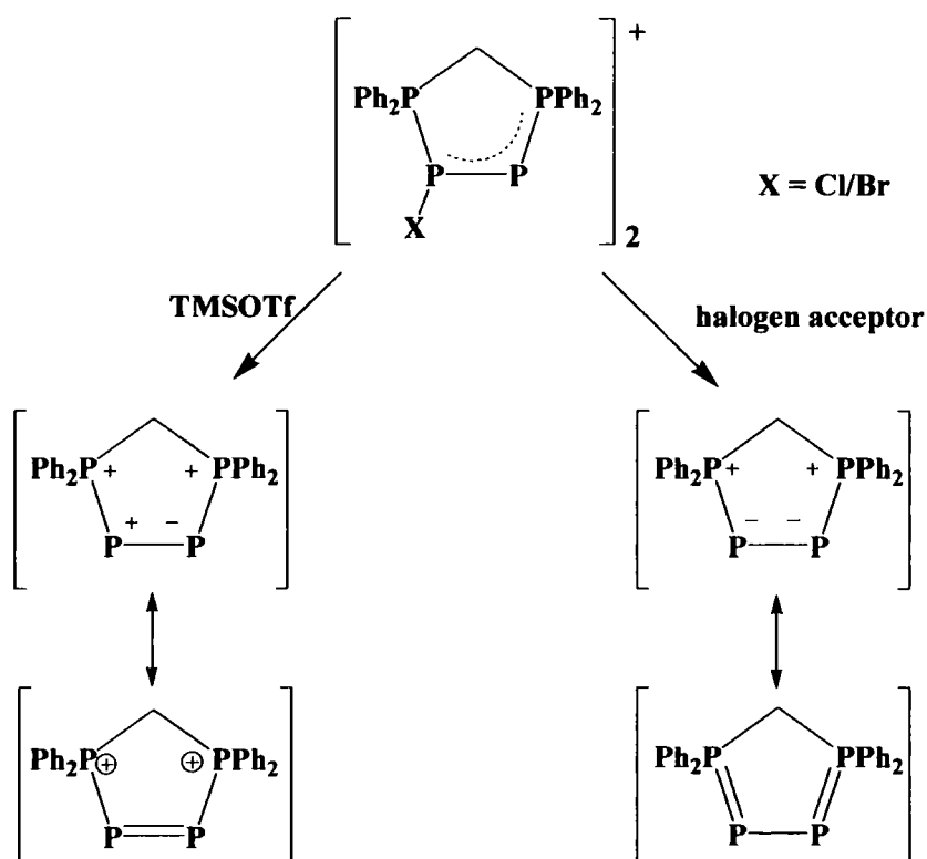
Scheme 7.4: Possible outcomes from the removal of X from a cyclic tetraphosphenium ion
