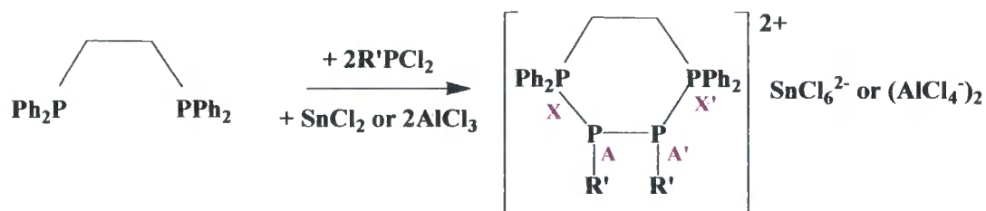
Scheme 5.4: Synthetic route for cyclic tetracosphonium ions derived from dppe
