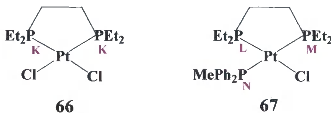
Figure 6.3: Products of the reaction between the 2a and trans -[Pt(PPh 2 Me)Cl( \mu -Cl)] 2
