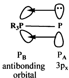
Figure 1.8: Back-bonding interactions between filled 3p_x orbitals on \text{P}_A and empty anti-bonding orbitals on \text{P}_B . 5
