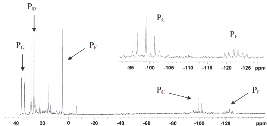
Figure 6.6: ^{31}\text{P} NMR spectrum of the reaction between dippc cyclic triphosphenium ion ( 8b ) and trans -[Pt(PEt 3 )Cl(μ-Cl)] 2
