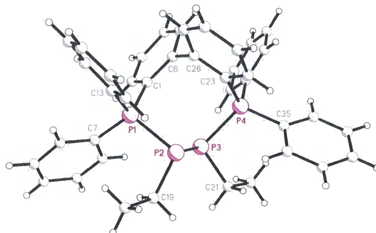
Figure 1.12: Molecular structure of the biphep cyclic tetraphosphenium ion 34
