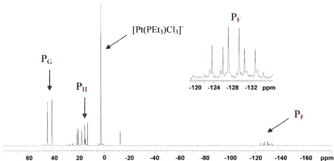
Figure 6.7: 31 P{ 1 H} NMR spectrum of the reaction between dcy pb cyclic triphosphenium ion, 11b , and trans -[Pt(PEt 3 )Cl(μ-Cl)] 2
