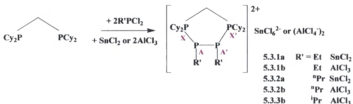
Scheme 5.2: Synthetic route for cyclic tetraphosphenium ions derived from dcypm
