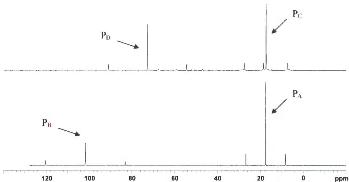
Figure 6.22: ^{31}\text{P}\{^1\text{H}\} NMR data for the reaction between cis -PtCl 2 (PEt 3 )(PCl 3 ) and 2-aminobenzyl alcohol. Bottom: parent complex, top: spectrum after 5 hours of reaction
