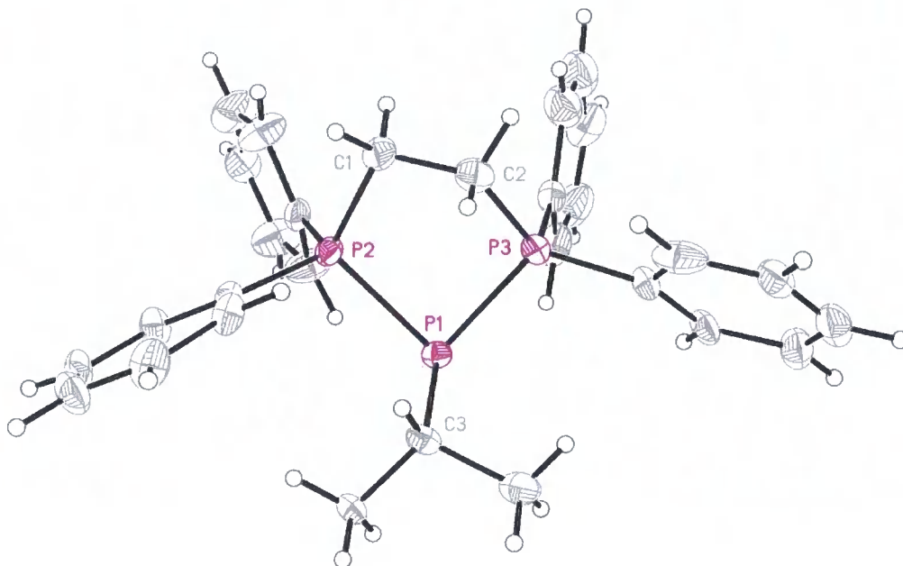
Figure 4.5: The molecular structure of the dication 25b , showing the numbering scheme for the key atoms (the counter-ions have been omitted for clarity). Thermal ellipsoids are drawn at 50 % probability.
