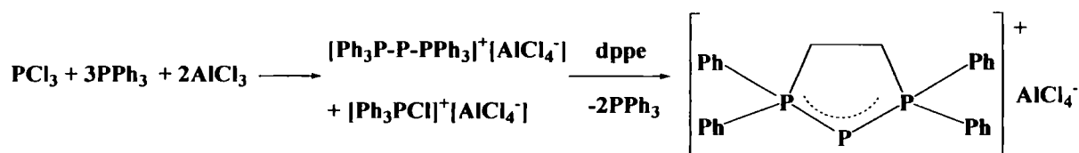
Scheme 1.5: The alternative route to form the 1,1,3,3-tetraphenyl-1λ 5 ,2λ 3 ,3λ 5 -triphosphenyl cation
