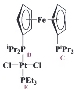
Figure 6.10: Proposed complex 93 formed in the reaction between dippf and trans -[Pt(PEt 3 )Cl(μ-Cl)] 2 .
