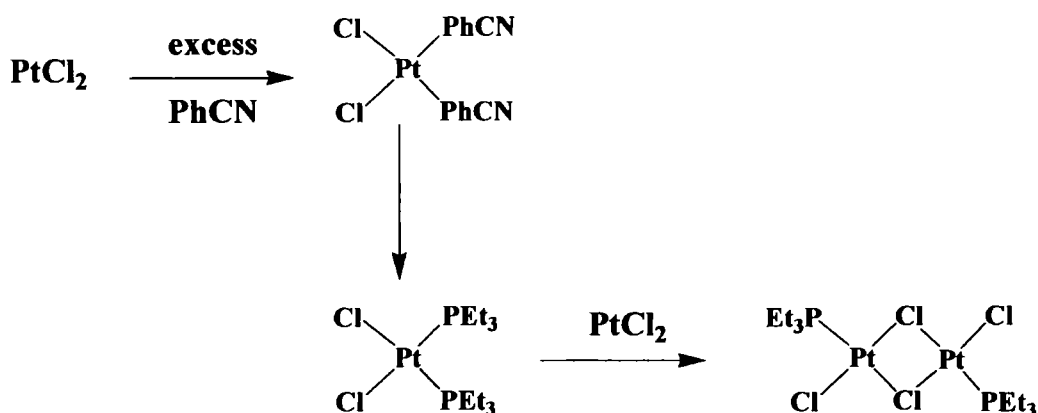
Scheme 6.26: Synthesis of \text{trans}-[\text{Pt}(\text{PEt}_3)\text{Cl}(\mu\text{-Cl})]_2 , a three step reaction 50
