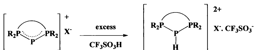
Scheme 1.10: Protonation of cyclic triphosphenium ions using triflic acid
