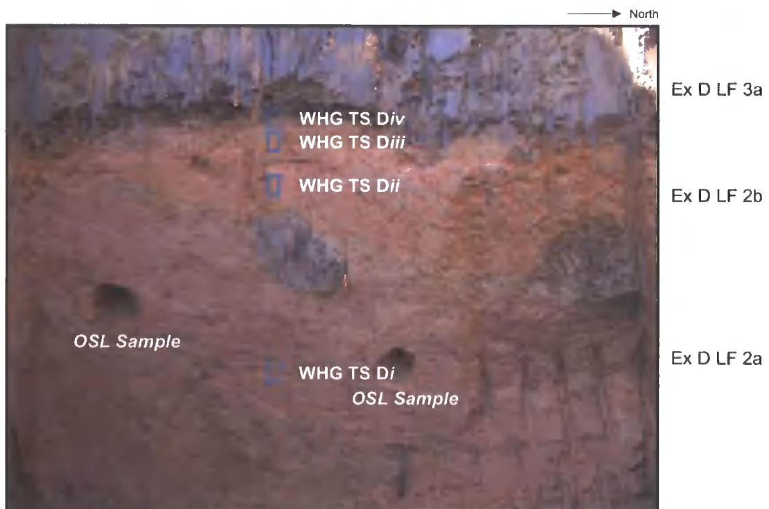
Figure 6.21: Location of thin section samples and OSL samples at Exposure D, Warren House Gill. Geological hammer is 32 cm long. Penknife is 19 cm long when extended.
