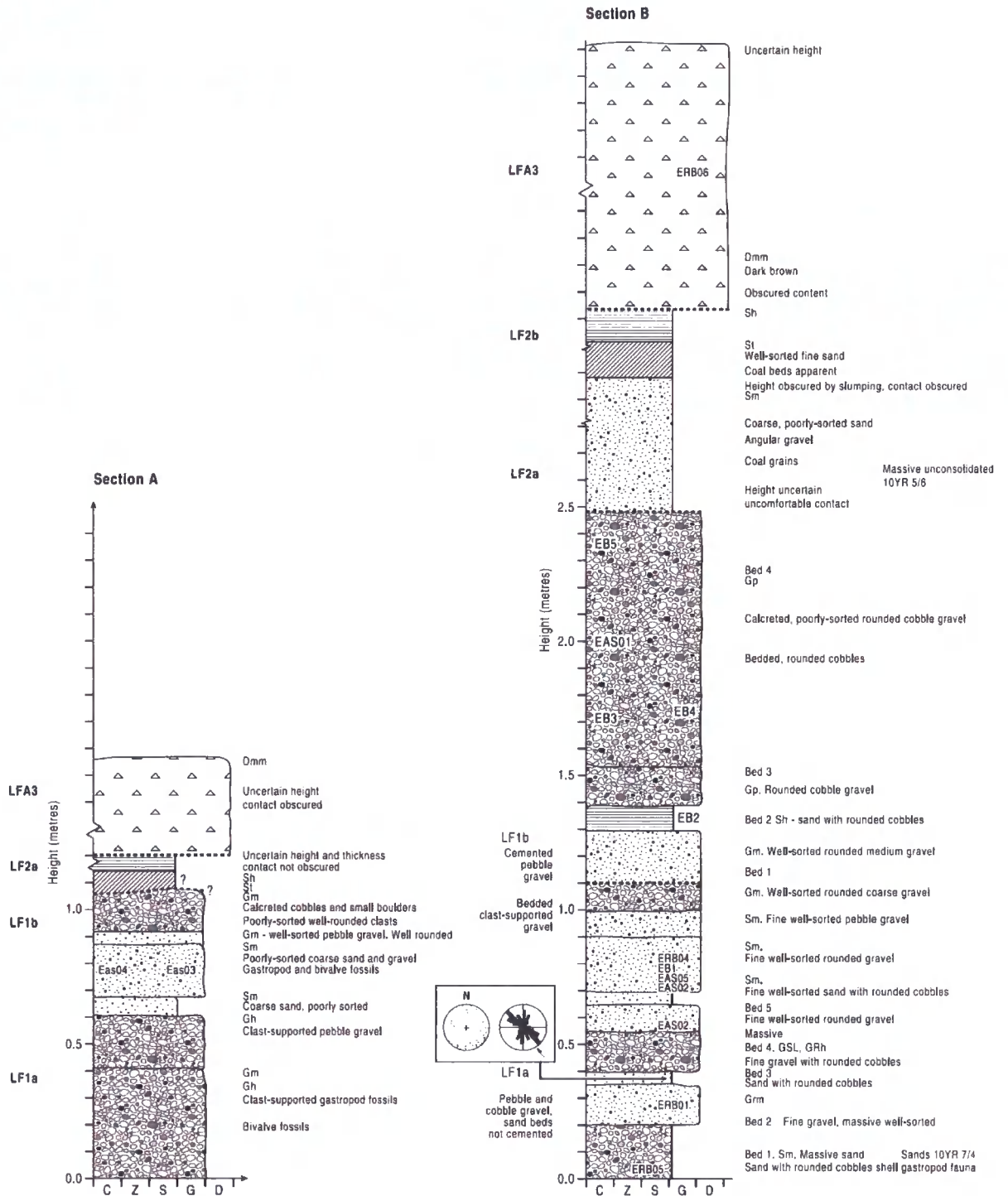
Figure 5.3: Sedimentary logs of Sections A and B, showing LFAs 1 to 3, Shippersea Bay
