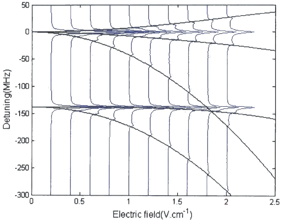
Figure 4.11: Modelling of Stark shifts of 44d states by EIT experiments results with the influence of the oscillating electric field(blue) F_{eff} = (F_p/4)(1 + \sin(\omega t)) corresponding to calculated Stark shifts(black).
