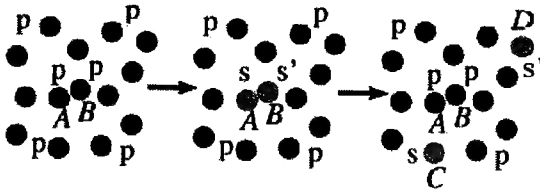
Figure 1.2: A schematic of excitation transfer in process corresponding to energy level in figure 1.1. Two Cs atoms (A and B) at 23p_{3/2} collide to produce 23s_{1/2} and 24s_{1/2} states and eventually transfer these s and s' states to the adjacent atoms (C and D).
