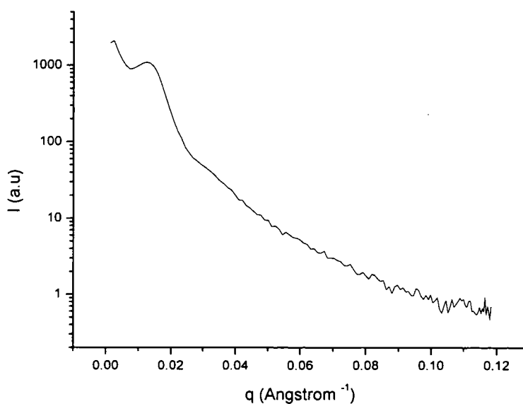
Figure 5.11 SAXS scattering from HyperBlock HBlock 12.
