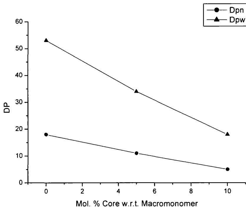
Figure 2.9 Effect of the addition of B_3 core on the extent of Williamson coupling reaction ( Dp_n and Dp_w ) used to prepare HyperMacs from polystyrene AB_2 macromonomer M_n 28000 g\text{mol}^{-1} . (Brominated macromonomer, at room temperature for 24 hours with CS_2CO_3 .)
