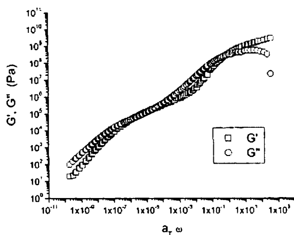
Figure.1.20 Master curve plot of moduli vs. frequency from a 1300 Kgmol -1 dendritically branched polystyrene chains. 90 ( G' represents the storage modulus, G'' the loss modulus.) Reproduced with permission from Macromolecules 2003, 36, 380. Copyright 2003 American Chemical Society.
