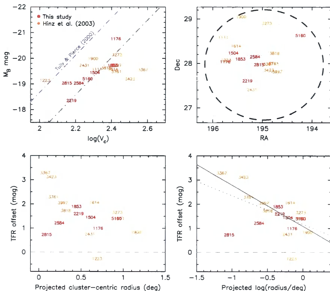
Figure 5.11: Upper-left panel: The Tully-Fisher relation for the Coma S0 galaxies in this study and in Hinze et al. (2003): red and orange GMP ID respectively. For comparison, the spiral TFR from Tully & Pierce (2000, purple dash-dots) is shown. The black dash-dot line indicates the bivariate best fit to the S0s, fixing the slope to the spiral relation. Upper-right panel: The distribution of these S0 galaxies within the Coma cluster core. The contours indicate the local galaxy density, and the dashed circle highlights a cluster-centric radius of 2 Mpc. Lower panels: the luminosity offset from the spiral TFR versus the cluster-centric radius of the galaxy, in linear (left) and logarithmic space (right). The dotted and solid dark grey lines indicate the weighted best fit including and excluding the outlier, GMP2815, respectively.
