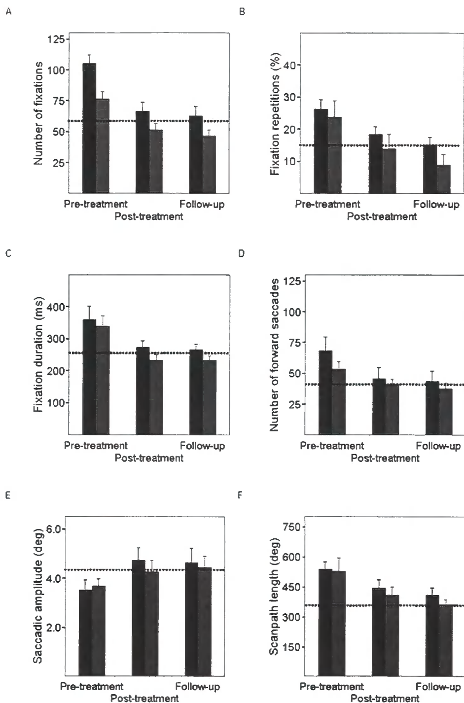
Fig. 2 Mean number of fixations (A), fixation repetitions (%) (B), mean fixation duration (ms) (C), mean number of forward saccades (D), mean saccadic amplitude ( ^{\circ} ) (E) and scanpath length ( ^{\circ} ) (F) before and after treatment and at follow-up for both training groups (text training: black bars, non-text training: grey bars; vertical bars indicate 1 SE). Dotted lines indicate average values for normal, age-matched controls ( n=25 ).
