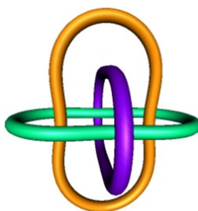
Figure 3.2: Three dimensional representation of the Borromean link.
