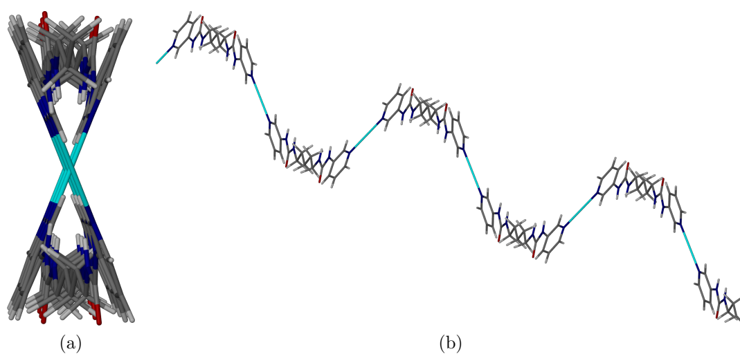
Figure 4.4: The single helix of 2.4 and silver(I) acetate.
