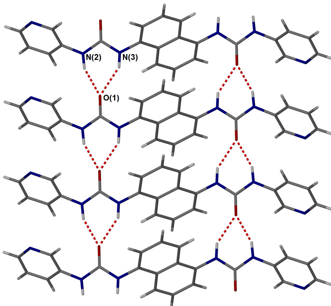
Figure 2.18: The X-ray crystal structure of compound 2.11 . Hydrogen-bond distances N(2)⋯(1) 2.788, N(3)⋯O(1) 2.891 Å.
