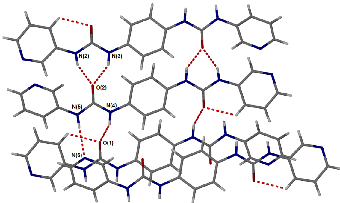
Figure 2.17: The X-ray crystal structure of compound 2.10 . Hydrogen-bond distances \text{N}(2)\cdots\text{O}(2) 2.851, \text{N}(3)\cdots\text{O}(2) 2.925, \text{N}(4)\cdots\text{O}(1) 2.853, \text{N}(5)\cdots\text{N}(6) 3.082, \text{N}(5)\cdots\text{O}(1) 3.219 Å.
