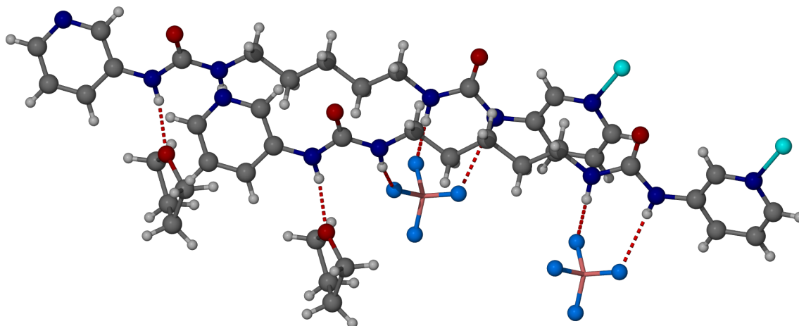
Figure 4.8: Two adjacent bis(pyridylurea) ligands connected via a NH...F interaction to a \text{BF}_4^- anion.
