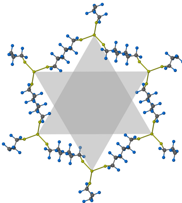
Figure 3.7: Hexagonal Rings from 1,1,2,2,3,3,4,4,5,5,6,6,7,7,8,8-hexadecafluoro-1,8-diodooctane and Iodine.
