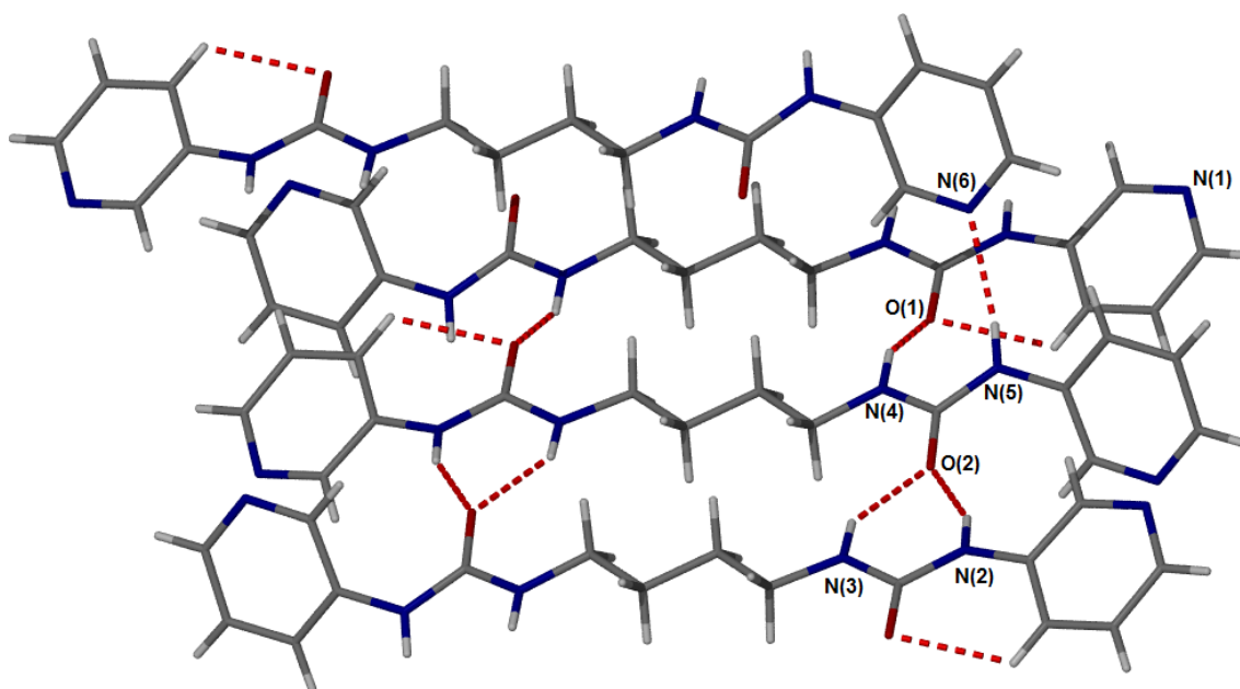
Figure 2.16: The X-ray crystal structure of compound 2.3 . Hydrogen-bond distances N(2) \cdots O(2) 2.880, N(3) \cdots O(2) 2.920, N(4) \cdots O(1) 2.925, N(5) \cdots N(6) 3.024 Å.
