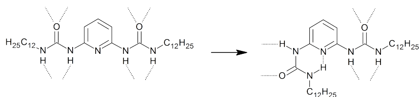
Figure 1.3: Inter- and intramolecular hydrogen-bonding modes of 1.75 .
