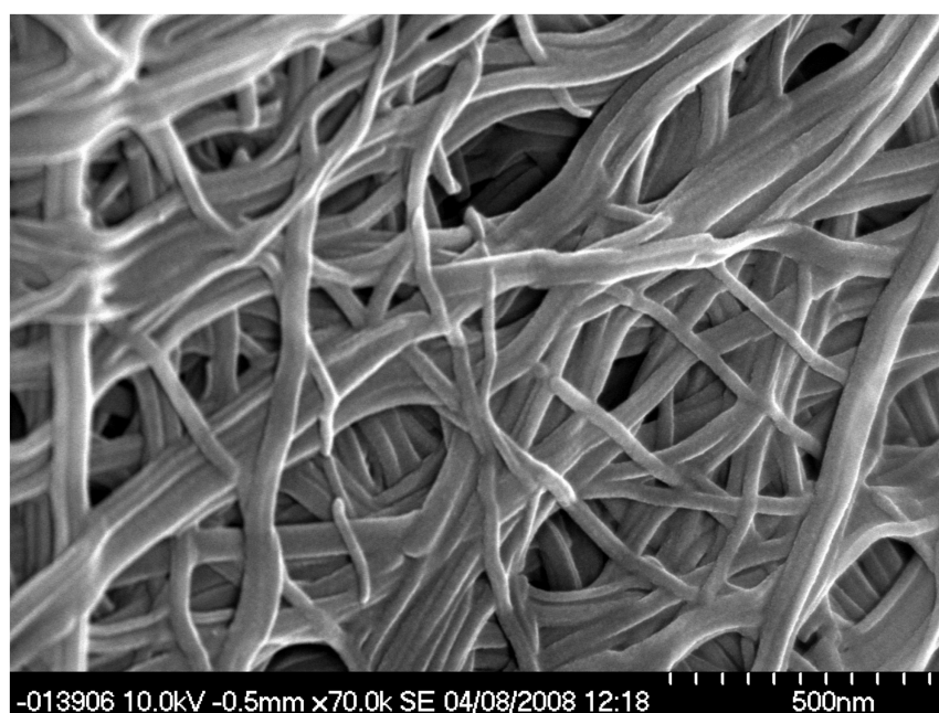
Figure 5.9: SEM micrograph of a partial gel prepared using 2.1 and silver(I) nitrate.
