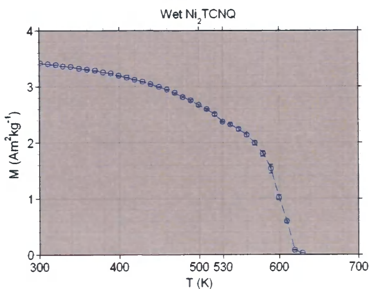
Figure 4.16: M(T) Wet Ni 2 TCNQ sample.
