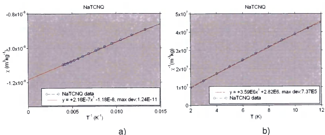
Figure 4.2: a) Susceptibility against inverse temperature for NaTCNQ, intercept is the diamagnetic susceptibility. b) Inverse against temperature for NaTCNQ. The data is then fit to Equation 6 to determine the Curie and Weiss constants.
