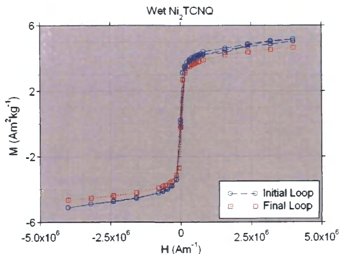
Figure 4.15: M(H) loops for wet Ni 2 TCNQ at 360K. The loops were recorded two weeks apart.
