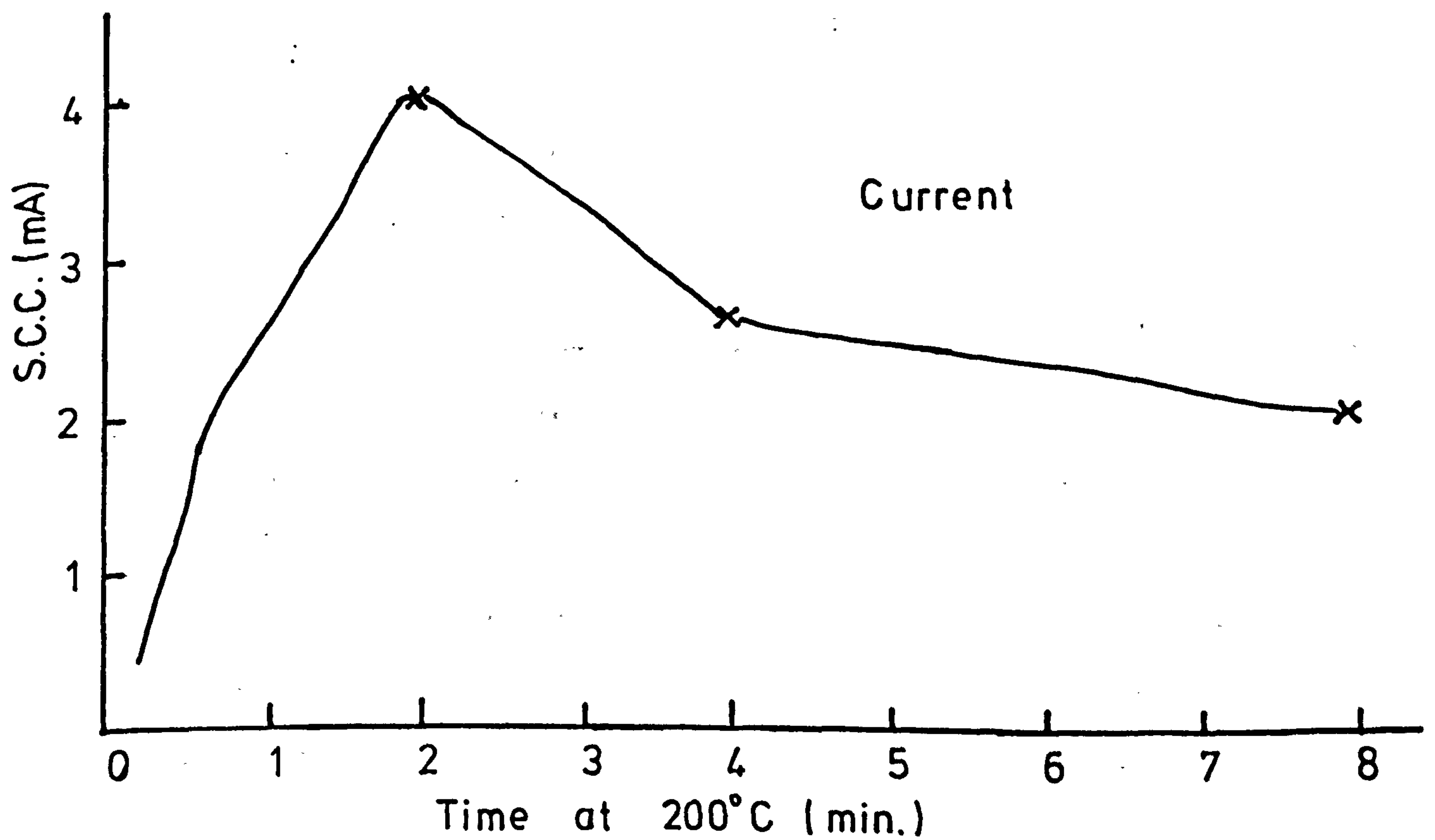
Figure 9.19 Thin Film Cell (film grown in enclosed tube ) Output and Baking Time
