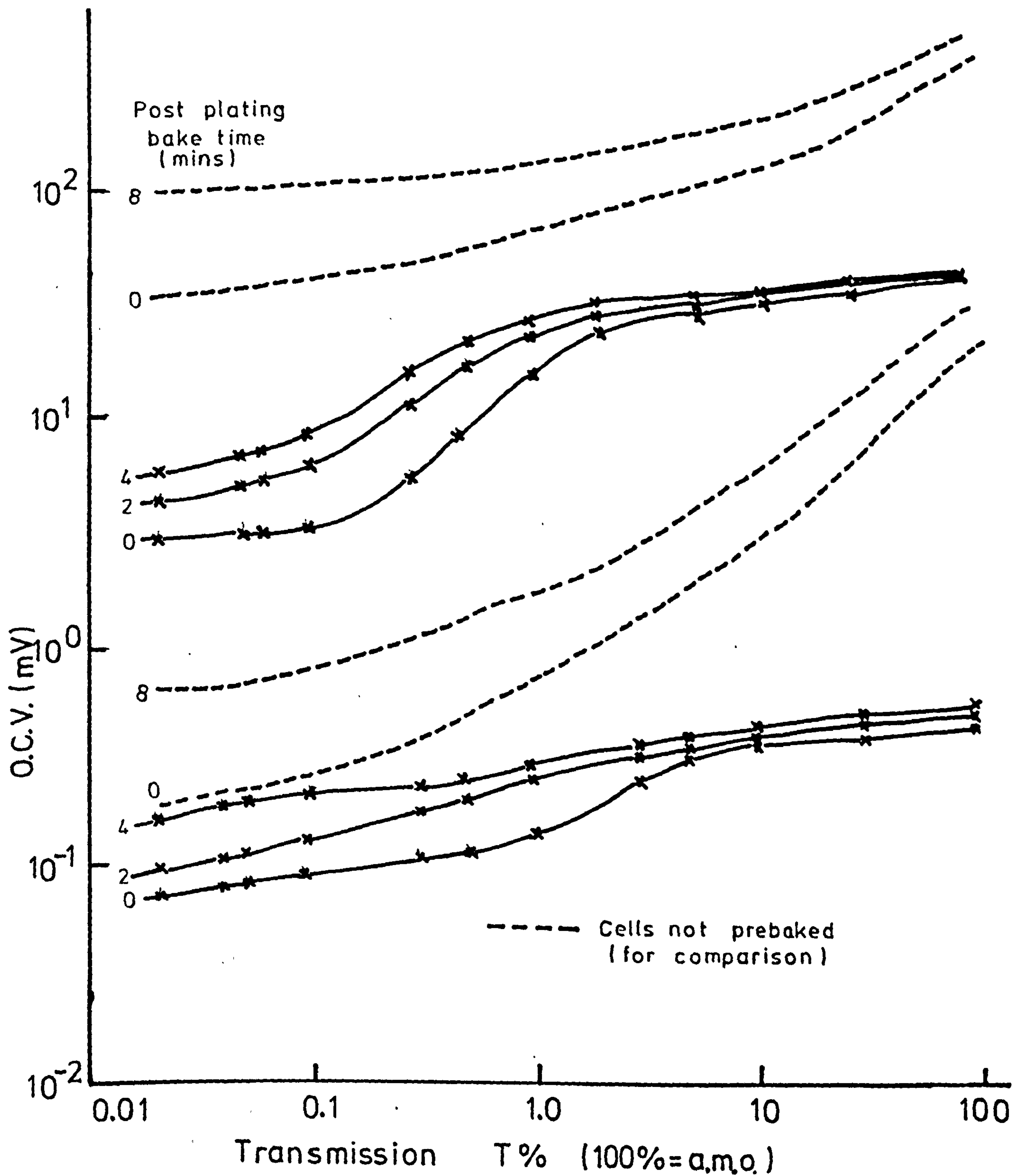
Figure 9.15 OCV Versus Light Intensity for Cells Pre-baked for 2 minutes
