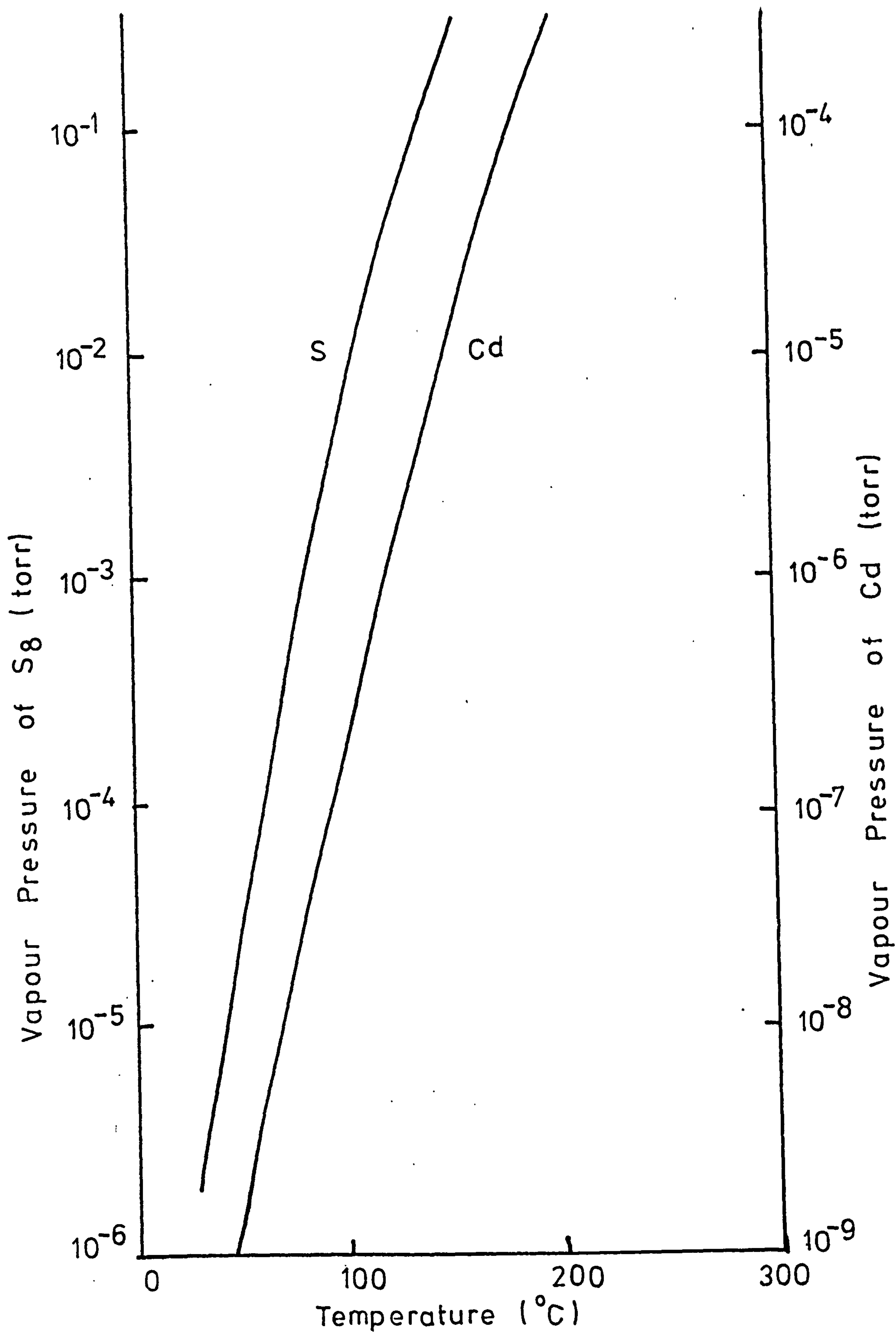
Figure 7.3 S.V.P. of Cd and \text{S}_8
