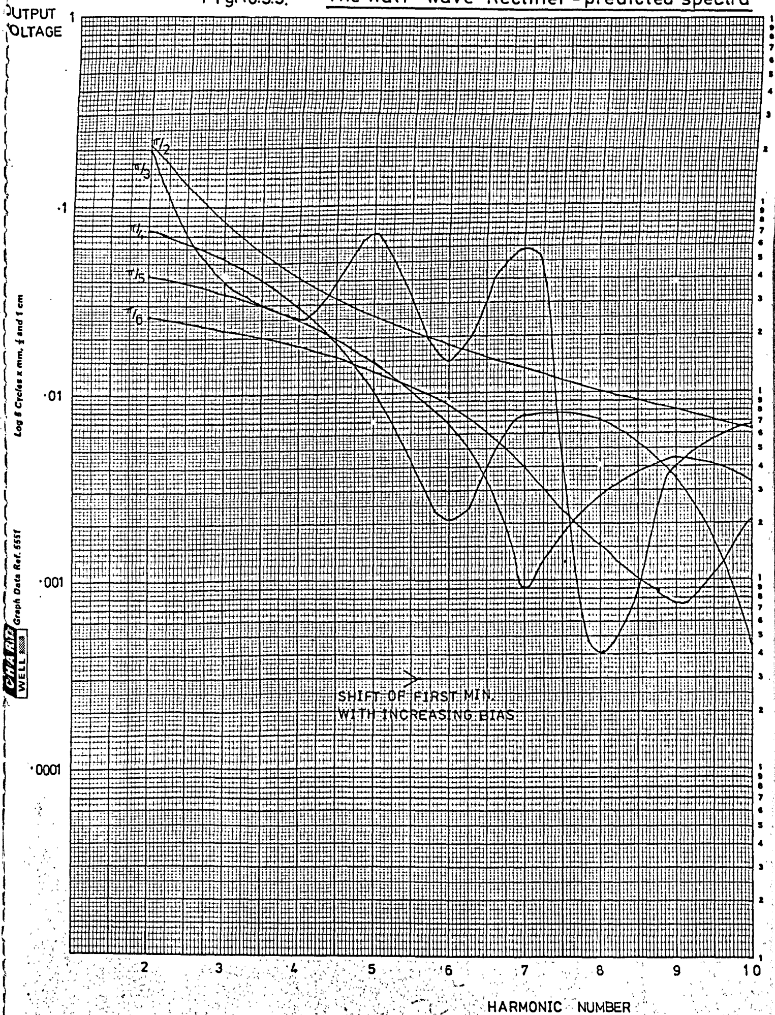
FigA6.35. The half-wave Rectifier - predicted spectra
