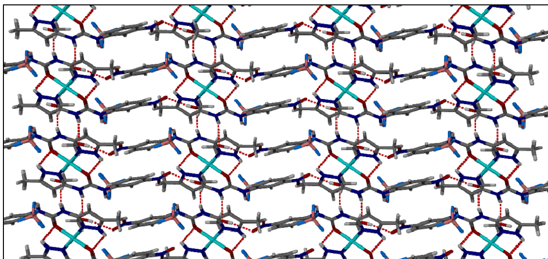
Figure 3.19. Packing of [\text{Cu}(\kappa\text{-N},\text{O-3.10})_2(\text{MeOH})_2](\text{BF}_4)_2 . Selected hydrogen bonds: \text{N3}\cdots\text{O4}^{ii} = 2.968(2) ; \angle \text{N3-H3N}\cdots\text{O4}^{ii} = 155.5^\circ , \text{N3}\cdots\text{F4} = 2.802(2) ; \angle \text{N3-H3N}\cdots\text{F4} = 139.5^\circ and \text{O4}\cdots\text{O3}^{iii} = 2.868(2) ; \angle \text{O4-H4}\cdots\text{O3}^{iii} = 162.8^\circ ( ii = 1+x, y, z and iii = -x, -y, 1-z ).
