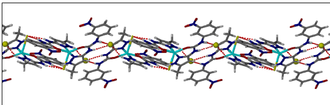
Figure 3.17. Extensive hydrogen bonding of [\text{CuBr}(\kappa\text{-N,O-3.10})_2]\text{Br}\cdot 2\text{H}_2\text{O} . Selected hydrogen bonds: \text{N1}\cdots\text{Br2}^i = 3.370(2) Å; \angle \text{N1-H1}\cdots\text{Br2}^i = 149.6^\circ , \text{N6}\cdots\text{O7W}^{ii} = 2.806(3) Å; \angle \text{N6-H6N}\cdots\text{O7W}^{ii} = 152.2^\circ , \text{N3}\cdots\text{Br1}^{iii} = 3.304(2) Å; \angle \text{N3-H3N}\cdots\text{Br1}^{iii} = 158.7^\circ ; \text{N4}\cdots\text{Br1}^{iii} = 3.371(2) Å; \angle \text{N4-H4N}\cdots\text{Br1}^{iii} = 157.2^\circ , \text{O7W}\cdots\text{O8W}^{iv} = 2.885(4) Å; \angle \text{O7W-H7W}\cdots\text{O8W}^{iv} = 164.9^\circ and \text{O8W}\cdots\text{Br1}^v = 3.293(2) Å; \angle \text{O8W-H8W}\cdots\text{Br1}^v = 162.9^\circ ( i = 1-x, 1-y, -z ; ii = 1-x, \frac{1}{2}+y, \frac{1}{2}-z ; iii = -x, 1-y, -z ; iv = x, \frac{1}{2}-y, z-\frac{1}{2} and v = 1-x, y-\frac{1}{2}, \frac{1}{2}-z ).
