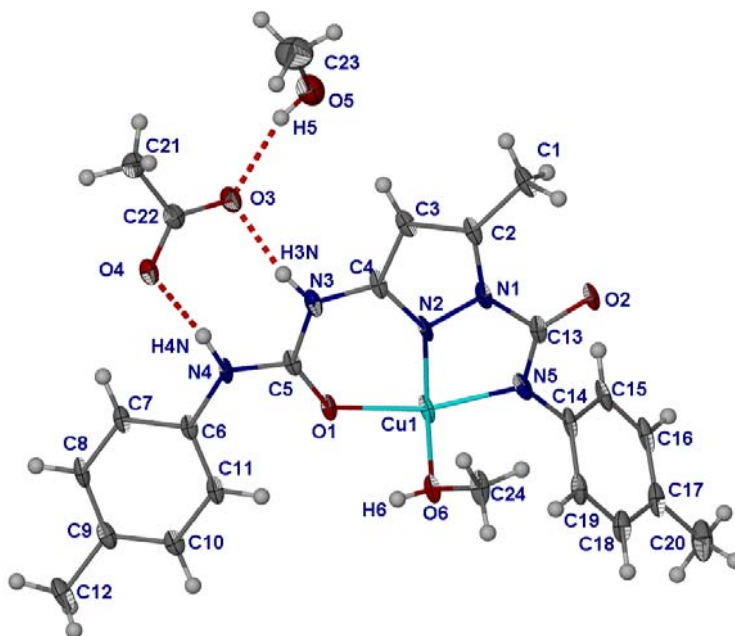
Figure 3.20. ASU of [\{\text{Cu}(\mu\text{-}\kappa\text{-O},\text{O},\text{N},\text{N}\text{-}\mathbf{3.11a})(\text{MeOH})\}_6](\text{MeCO}_2)_6 \cdot 6\text{MeOH} . Atoms are shown as ellipsoids at 30% probability. Selected bond lengths: \text{N5}\cdots\text{Cu1} = 2.001(4) Å, \text{N2}\cdots\text{Cu1} = 1.882(5) Å, \text{O1}\cdots\text{Cu1} = 2.004(3) Å, \text{O6}\cdots\text{Cu1} = 2.216(4) Å and \text{O2}^i\cdots\text{Cu1} = 1.939(3) Å. Selected hydrogen bonds: \text{N3}\cdots\text{O3} = 2.730(6) ; \angle \text{N3-H3N}\cdots\text{O3} = 165.3^\circ and \text{N4}\cdots\text{O4} = 2.765(6) ; \angle \text{N4-H4N}\cdots\text{O4} = 169.9^\circ , \text{O5}\cdots\text{O3} = 2.824(6) ; \angle \text{O5-H5}\cdots\text{O3} = 164.9^\circ and \text{O6}\cdots\text{O4}^{ii} = 2.679(5) ; \angle \text{O6-H6}\cdots\text{O4}^{ii} = 173.4^\circ ( i = 1+y, 1-x+y, -z and ii = \frac{5}{3}-x, \frac{1}{3}-y, \frac{1}{3}-z ).
