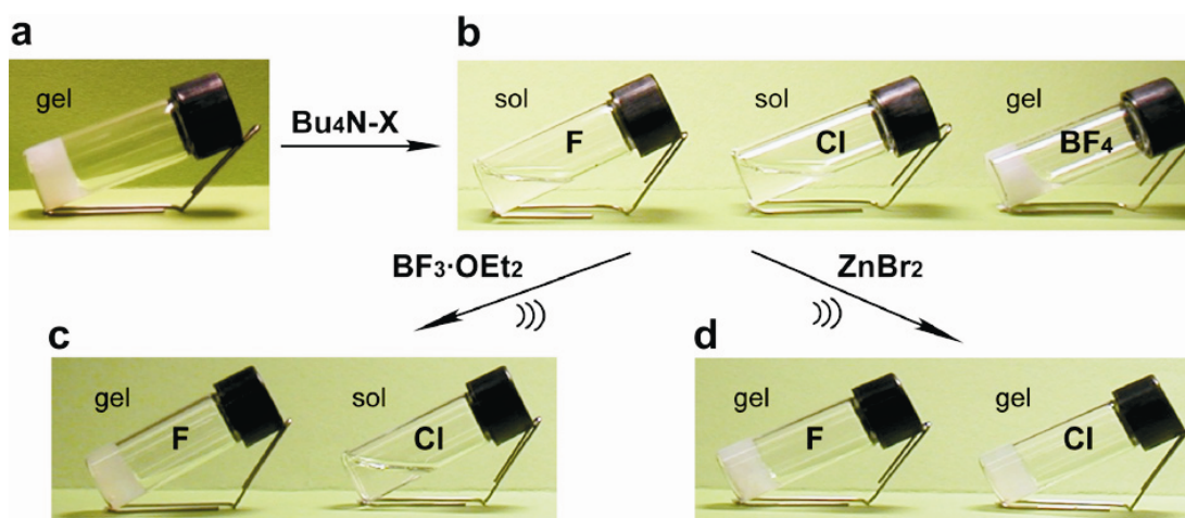
Figure 1.8. The acetone gel of 1.29 , showing the transitions between the gel state and liquid states upon addition of chemical stimuli ( \text{X} = \text{F}^- , \text{Cl}^- or \text{BF}_4^- ). a) Acetone gel of 1.29 (2.0 wt %). b) Acetone gel of 1.29 (2.0 wt %) containing (from left) 1.1 equiv of \text{TBA}^+ \text{F}^- , 1.7 equiv of \text{TBA}^+ \text{Cl}^- , and 10 equiv of \text{TBA}^+ \text{BF}_4^- . c) \text{BF}_3 \cdot \text{OEt}_2 (1.0 equiv for \text{TBA}^+ salt) mixture after sonication of 1.29 and \text{TBA}^+ \text{F}^- (left) or \text{TBA}^+ \text{Cl}^- (right) in acetone. d) \text{ZnBr}_2 (1.0 equiv for \text{TBA}^+ salt) mixture after sonication of 1.29 and \text{TBA}^+ \text{F}^- (left) or \text{TBA}^+ \text{Cl}^- (right) in acetone. (Reproduced with permission from ref. 184 )
