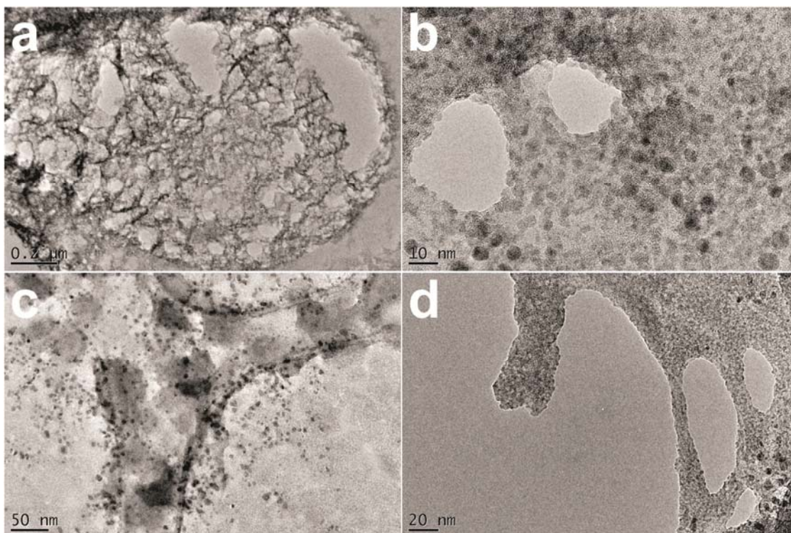
Figure 3.42. TEM images of gels of 3.10 acidified with a,b ) \text{HBF}_4 , c,d ) \text{HPF}_6 .
