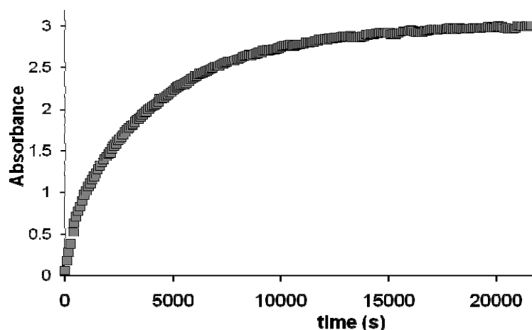
Figure 2.45. IBU release (30 mg in sample gel) over time from a 0.3% gel of 2.1a in EtOH:H 2 O 3:7 into pure water followed using UV spectroscopy.
