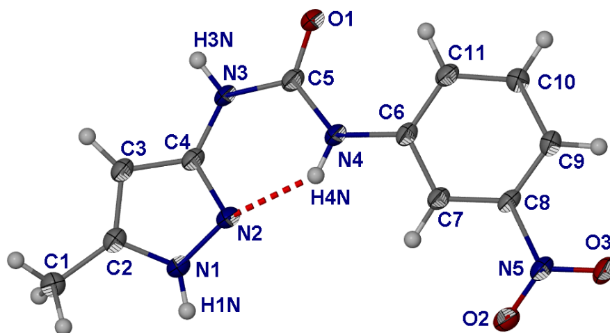
Figure 3.7. Molecular structure of 3.10 . Atoms are shown as ellipsoids at 50% probability. Selected hydrogen bond: N4...N2 = 2.6651(17) Å; \angle N4-H4N...N2 = 139.4°.
