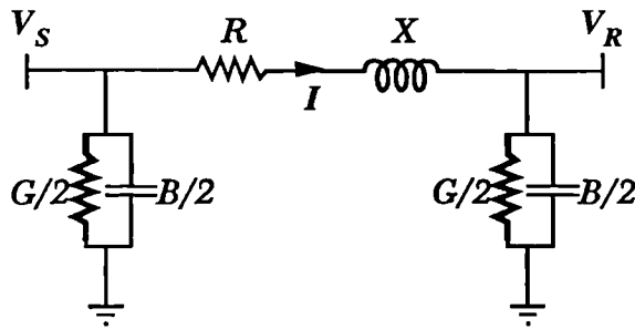
Figure 8.6 \Pi Section Model of a Transmission Line
