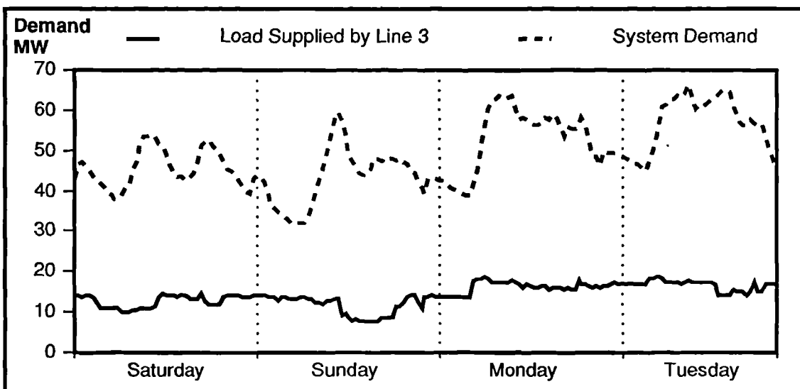
Figure 8.10 Comparison of Load Supplied By Line 3 with System Demand
