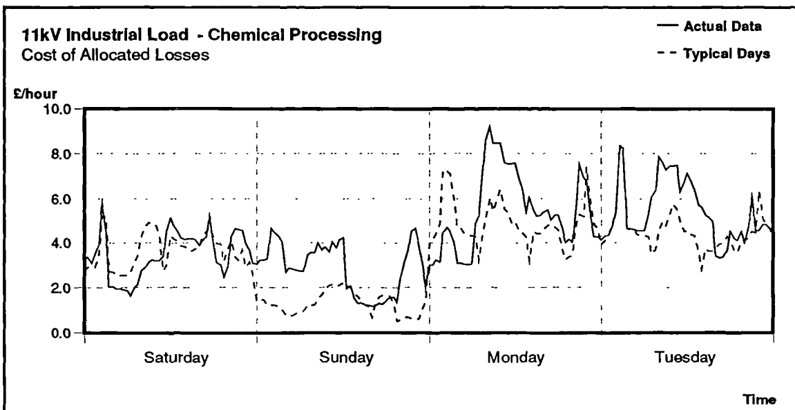
Figure 2.6 Actual Data and Typical Days for 11kV Chemical Processing Plant
