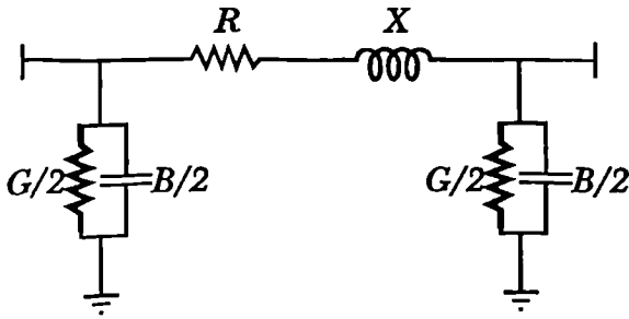
Figure D.1 Transmission Line Model Used in the Load-flow Program
