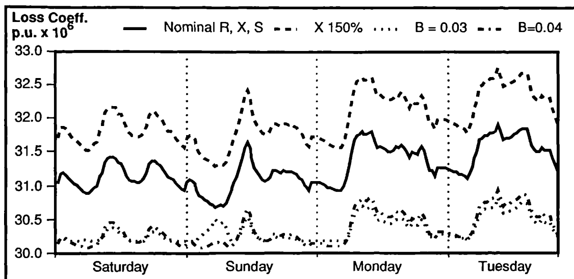
Figure 8.12 Variation In Loss Coefficients with Different Line Parameters
