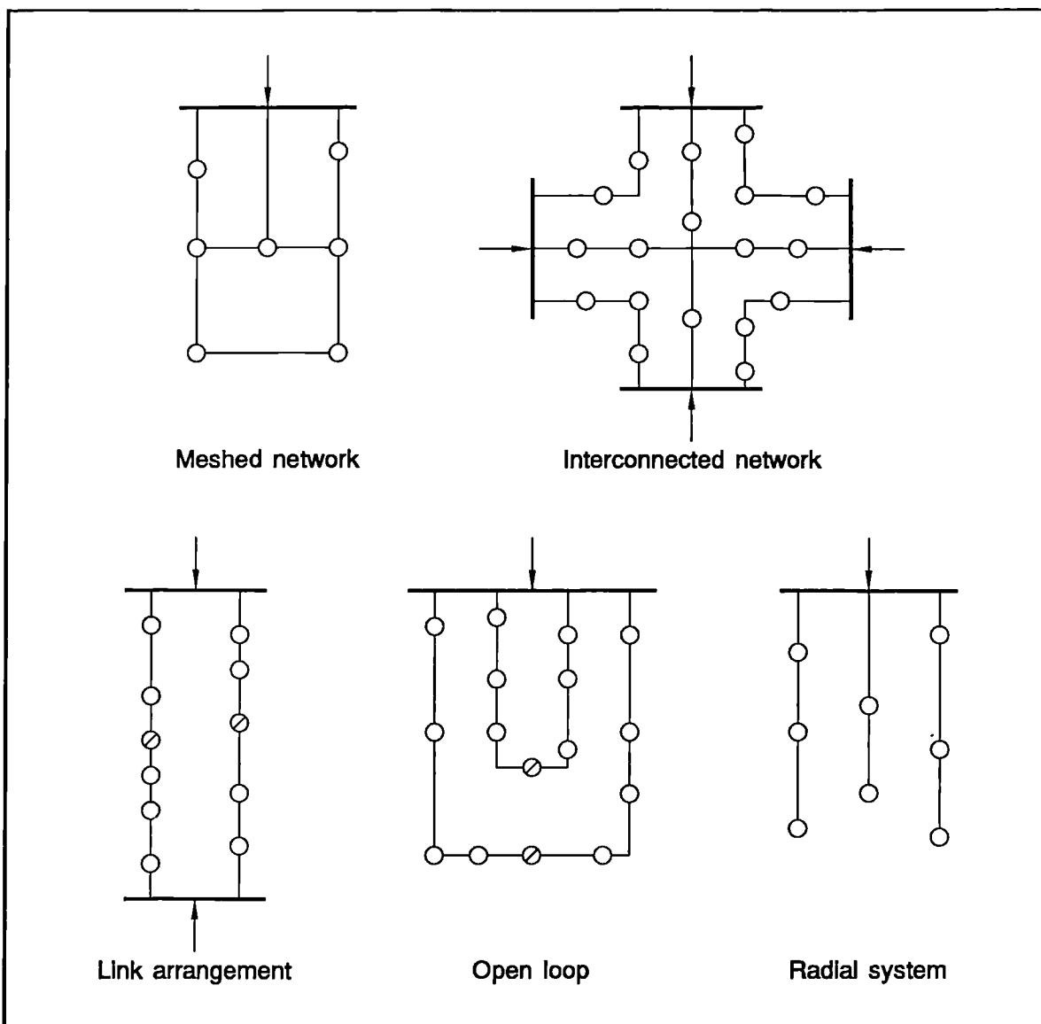
Figure 1.3 Distribution Network Configurations
