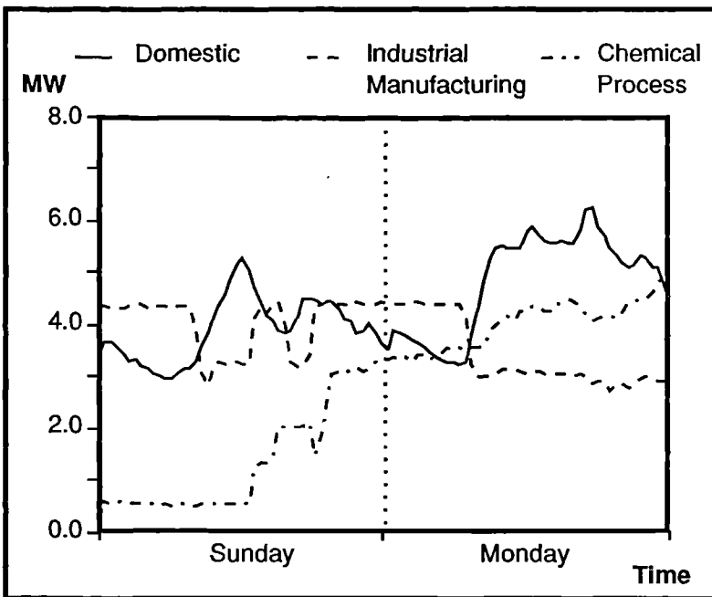
Figure 1.8 Consumer Demand Profiles on Neighbouring 11kV Feeders
