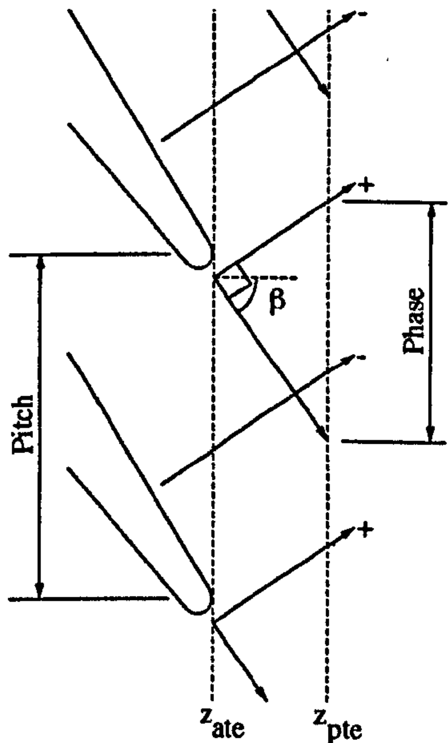
Figure 6.1 Schematic Pressure Field Downstream of a Blade Row.
