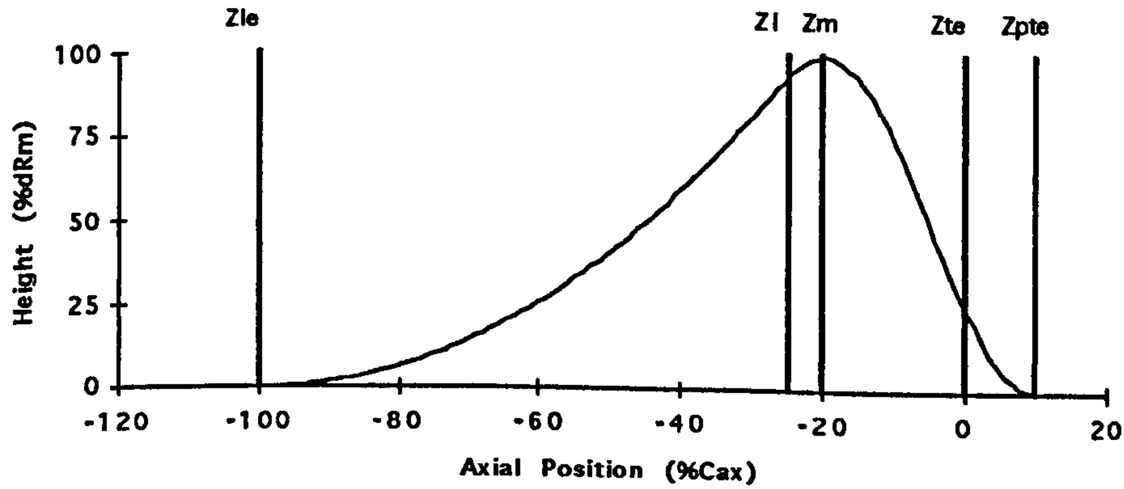
Figure 6.2 Schematic View of the Axial Shape of the Profile.
