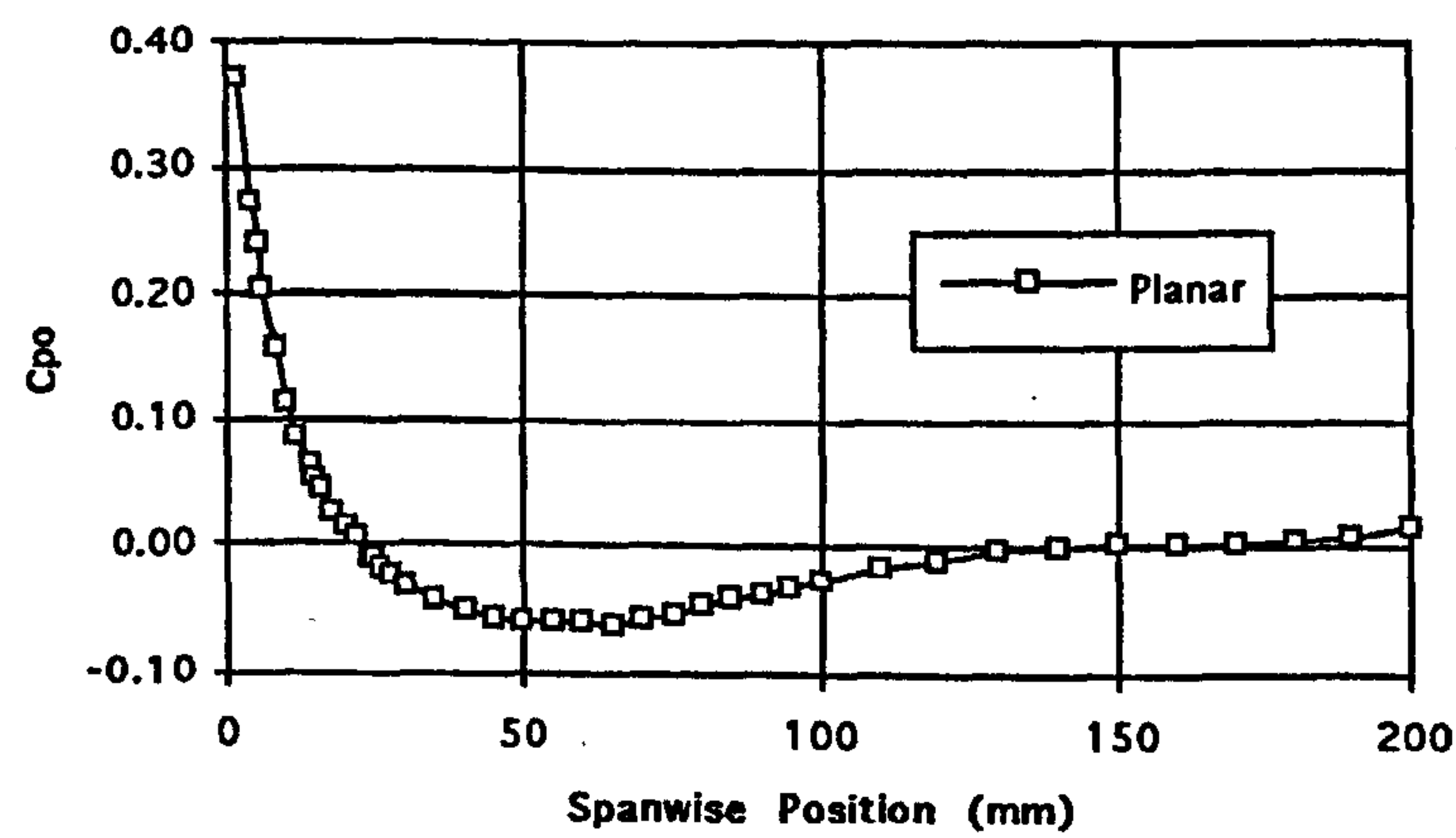
Figure 5.14 Measured Total Pressure Coefficient 100% C_{ax} Upstream.
