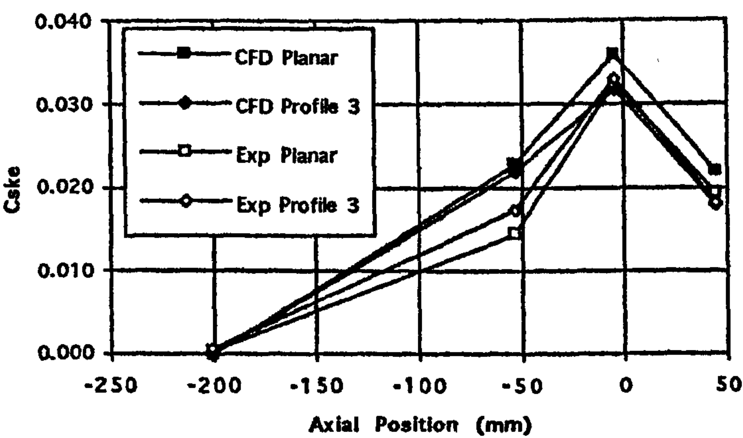
Figure 6.28 Growth of C_{SKE} Through the Cascade.
