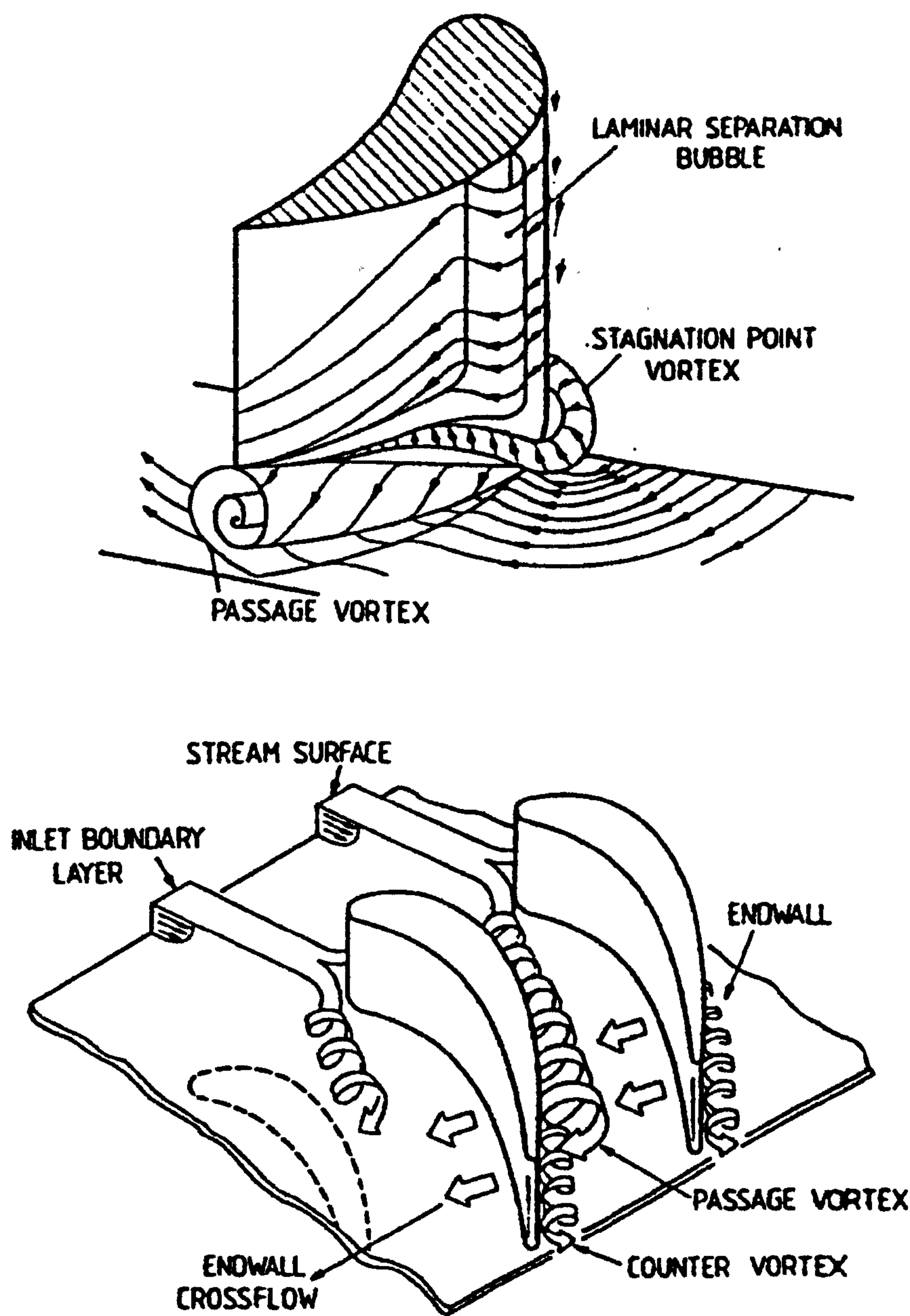
Figure 2.1 General Secondary Flow Structure (after Klein [1966] and Langston [1976])
