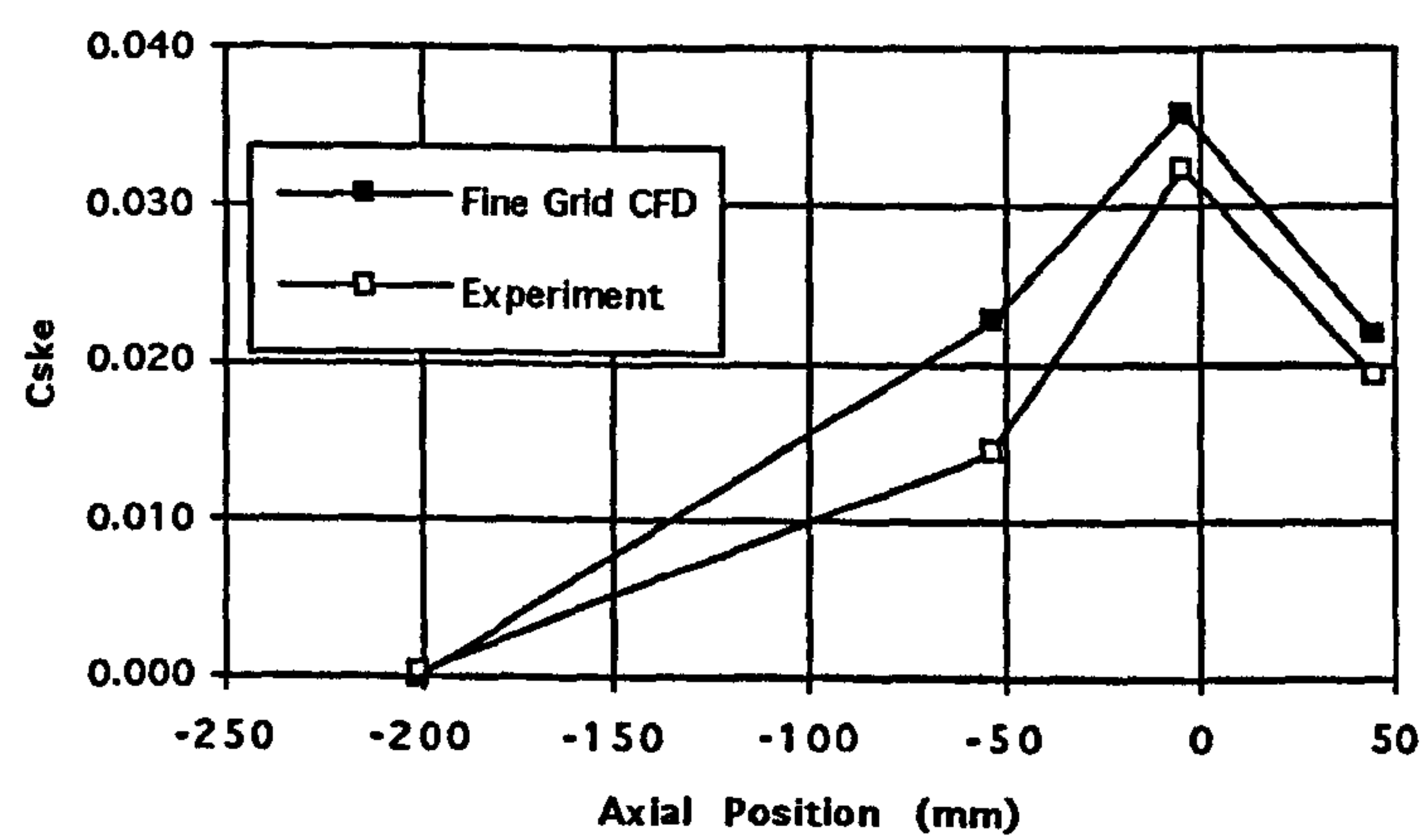
Figure 5.20 Growth of Secondary Kinetic Energy Through the Cascade.
