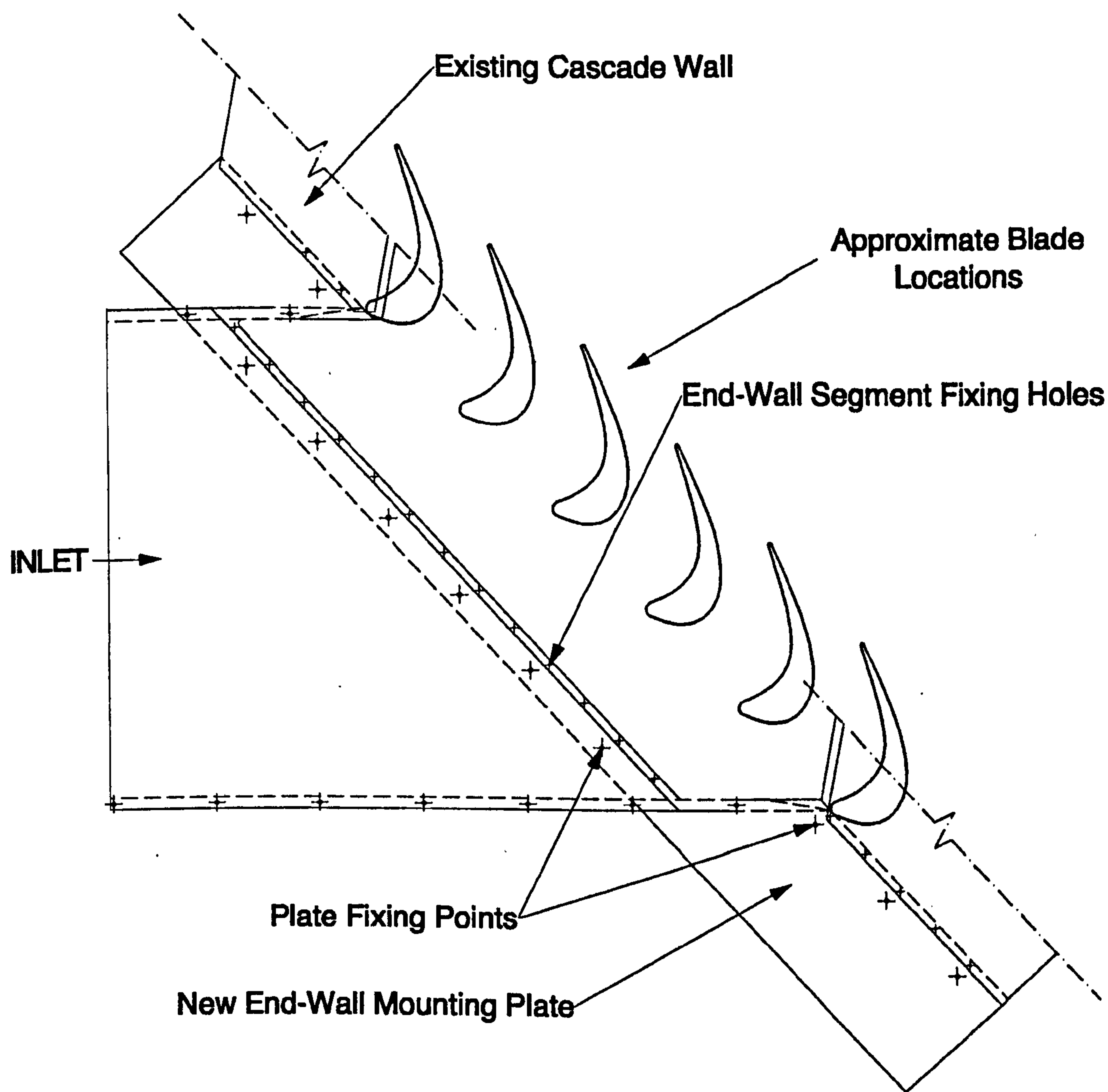
Figure 7.1 Wind Tunnel Modifications to Allow Large End-wall Segments to be Mounted.
