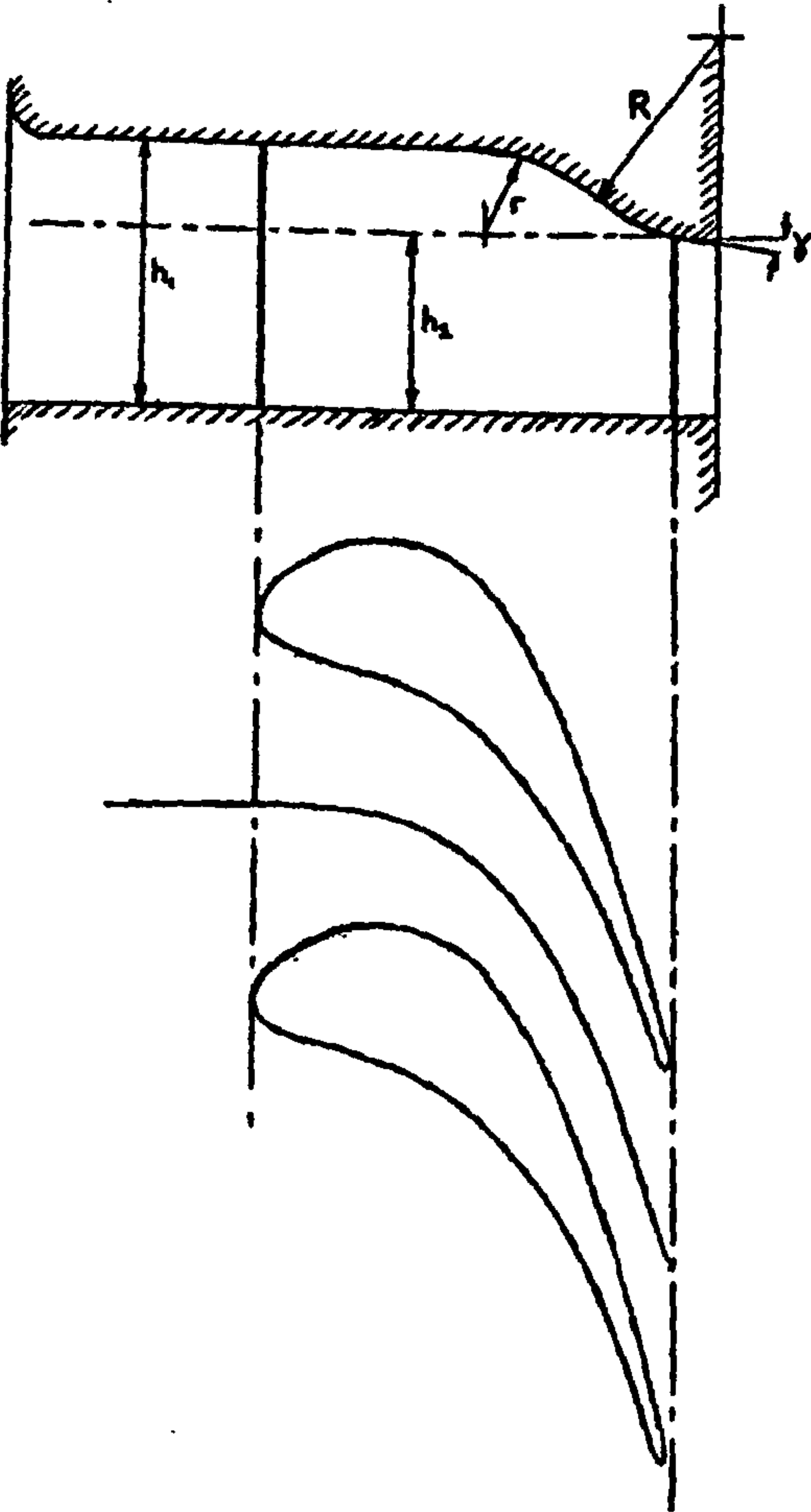
Contraction Shape (after Diech [1960])
