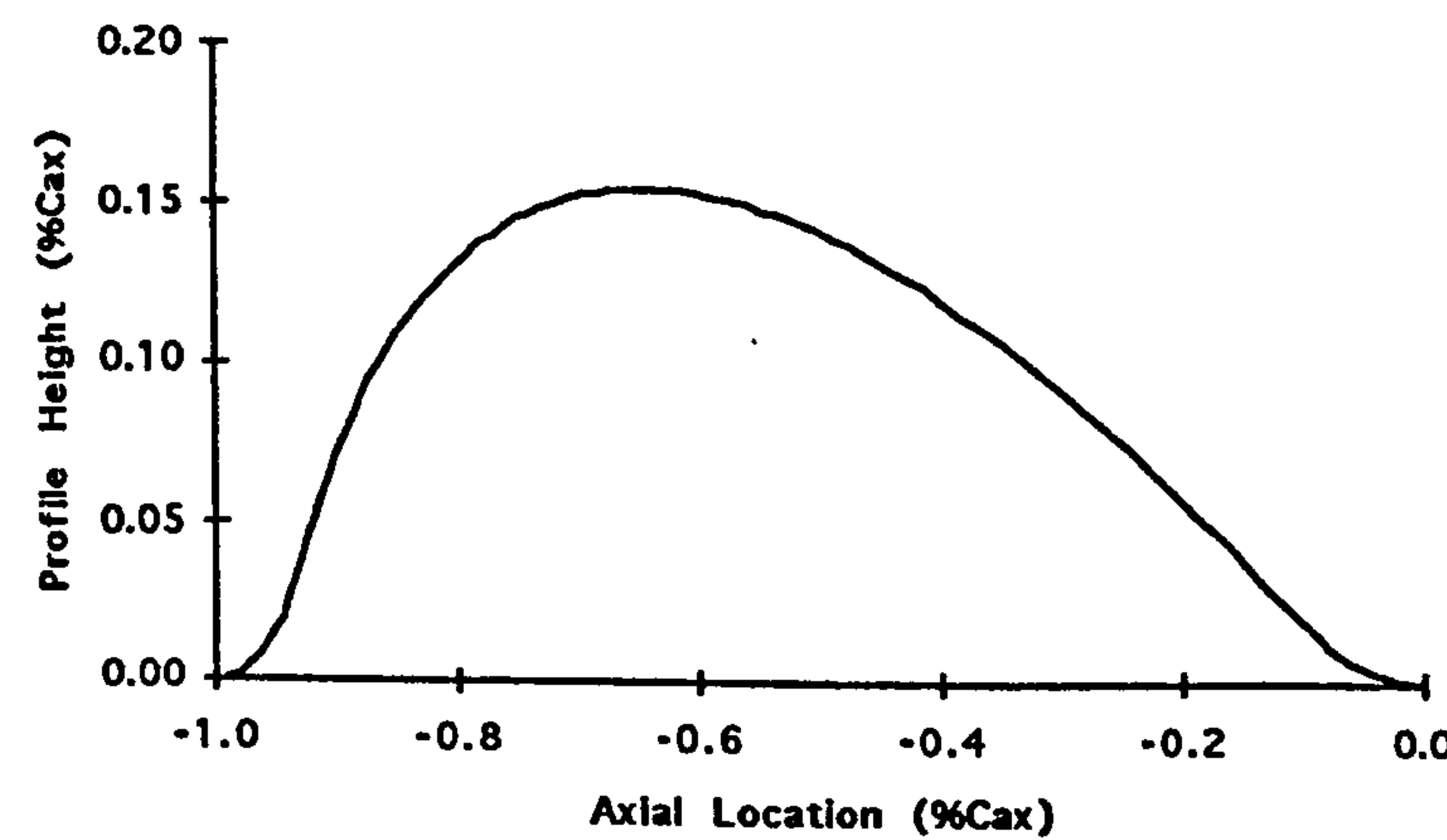
Figure 8.2 Axial Component of Profile AXM2
