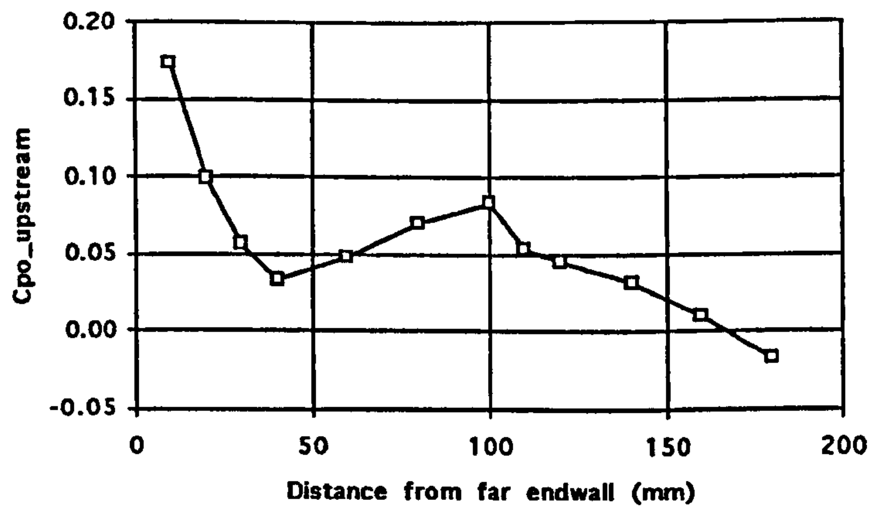
Figure 4.9 Inlet Total Pressure Non-uniformity at the Reference Probe Location.
