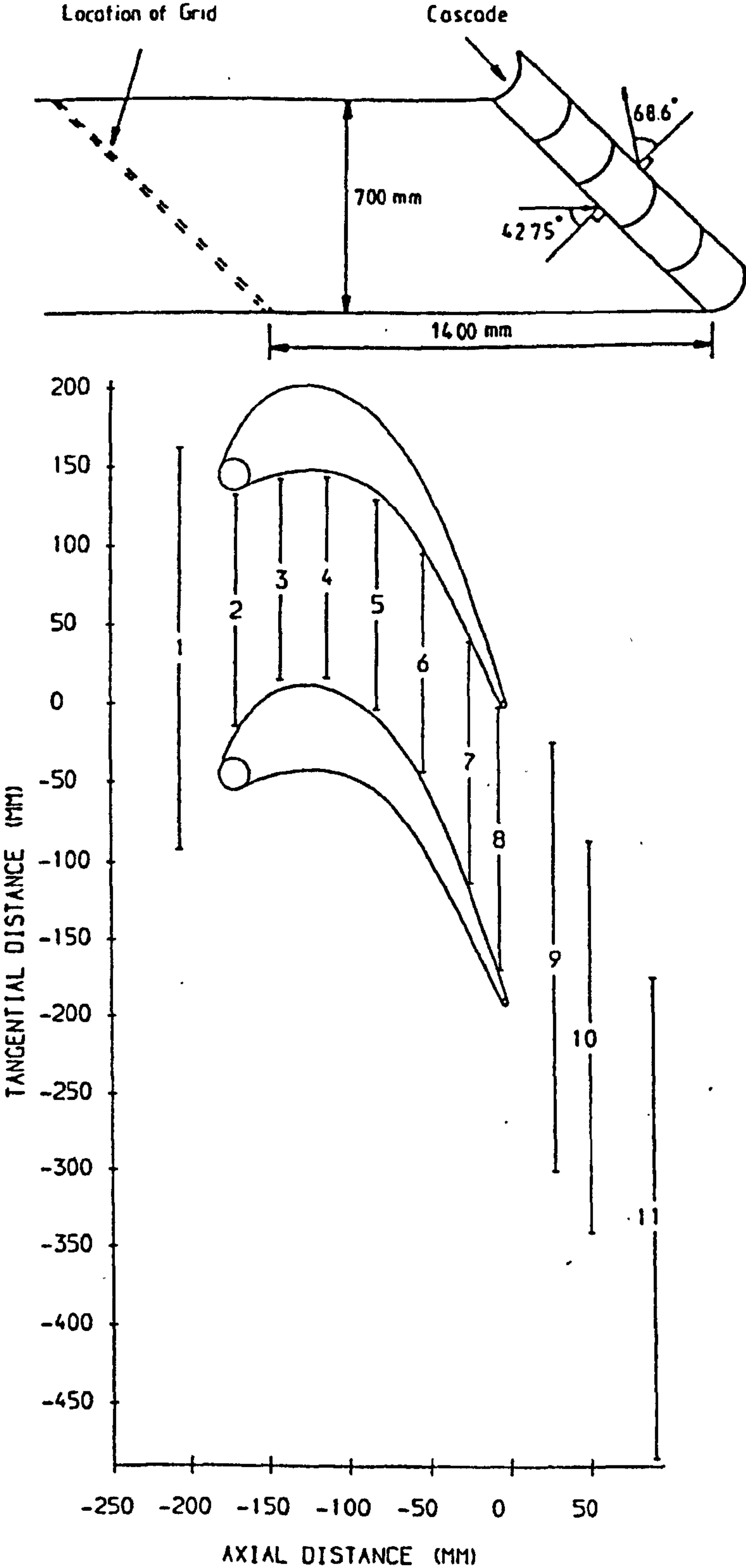
Layout of the Durham Linear Cascade.
