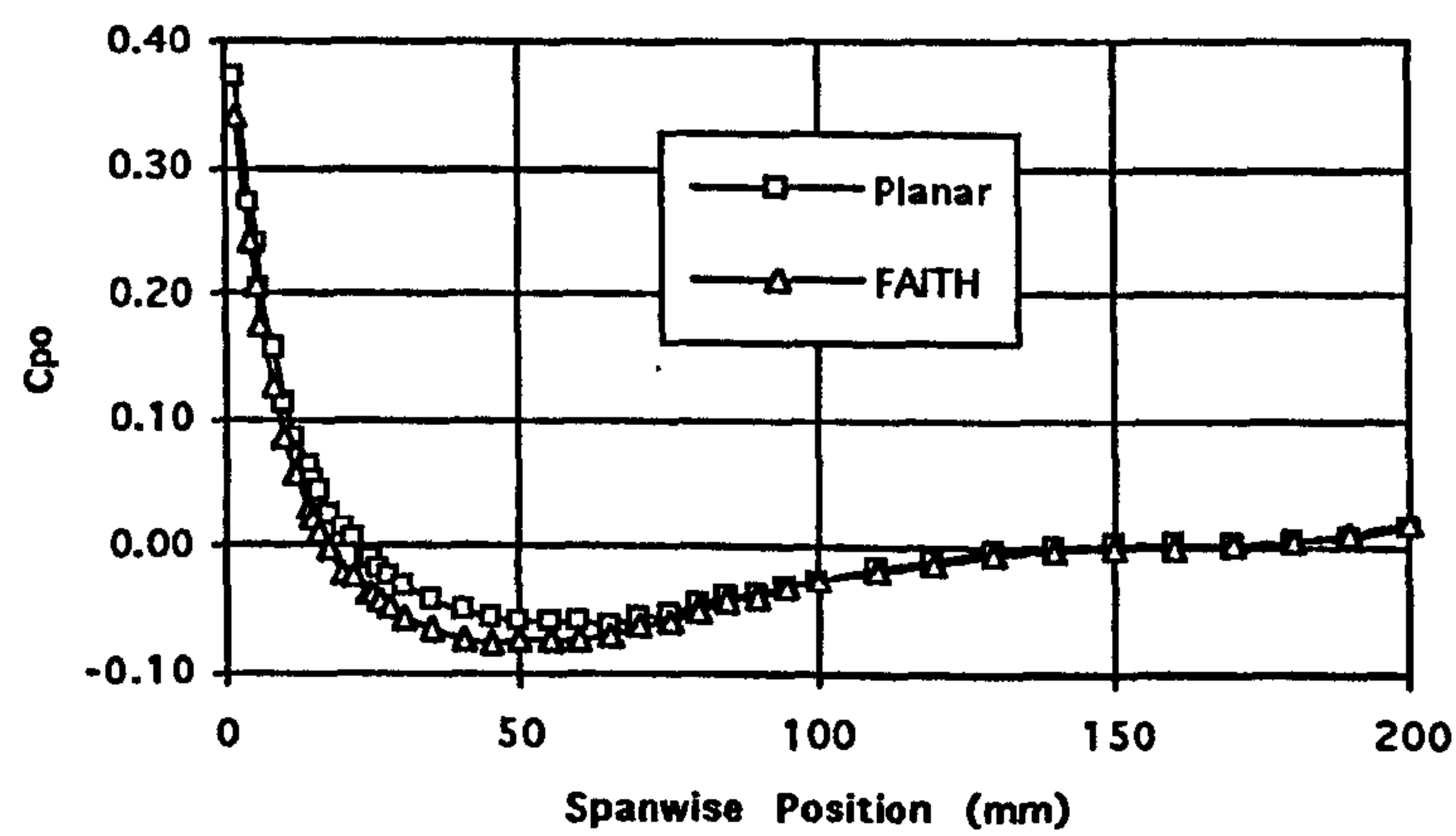
Figure 7.16 Measured Total Pressure Coefficient 100% C_{tx} Upstream.
