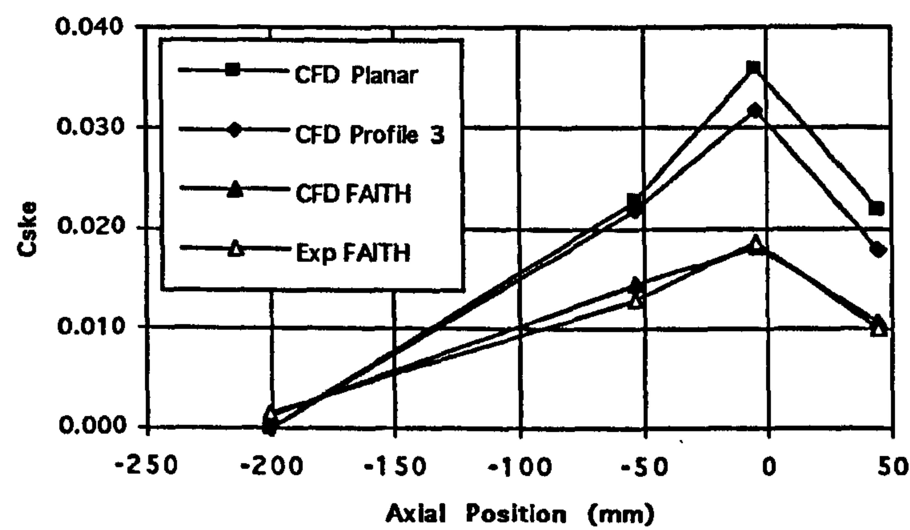
Figure 7.21 Growth of C_{SKE} Through the Cascade.
