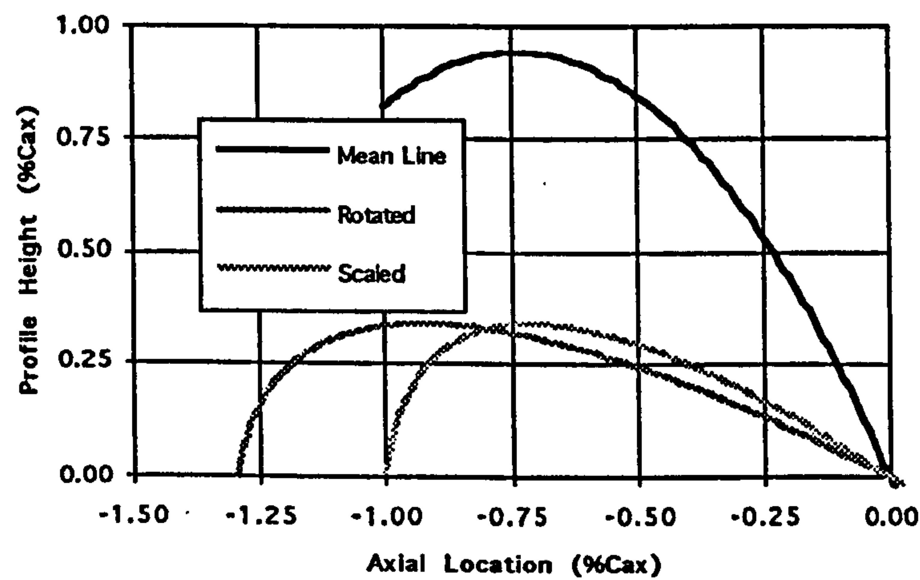
Figure 8.1 Modification of the Blade Mean Line.
