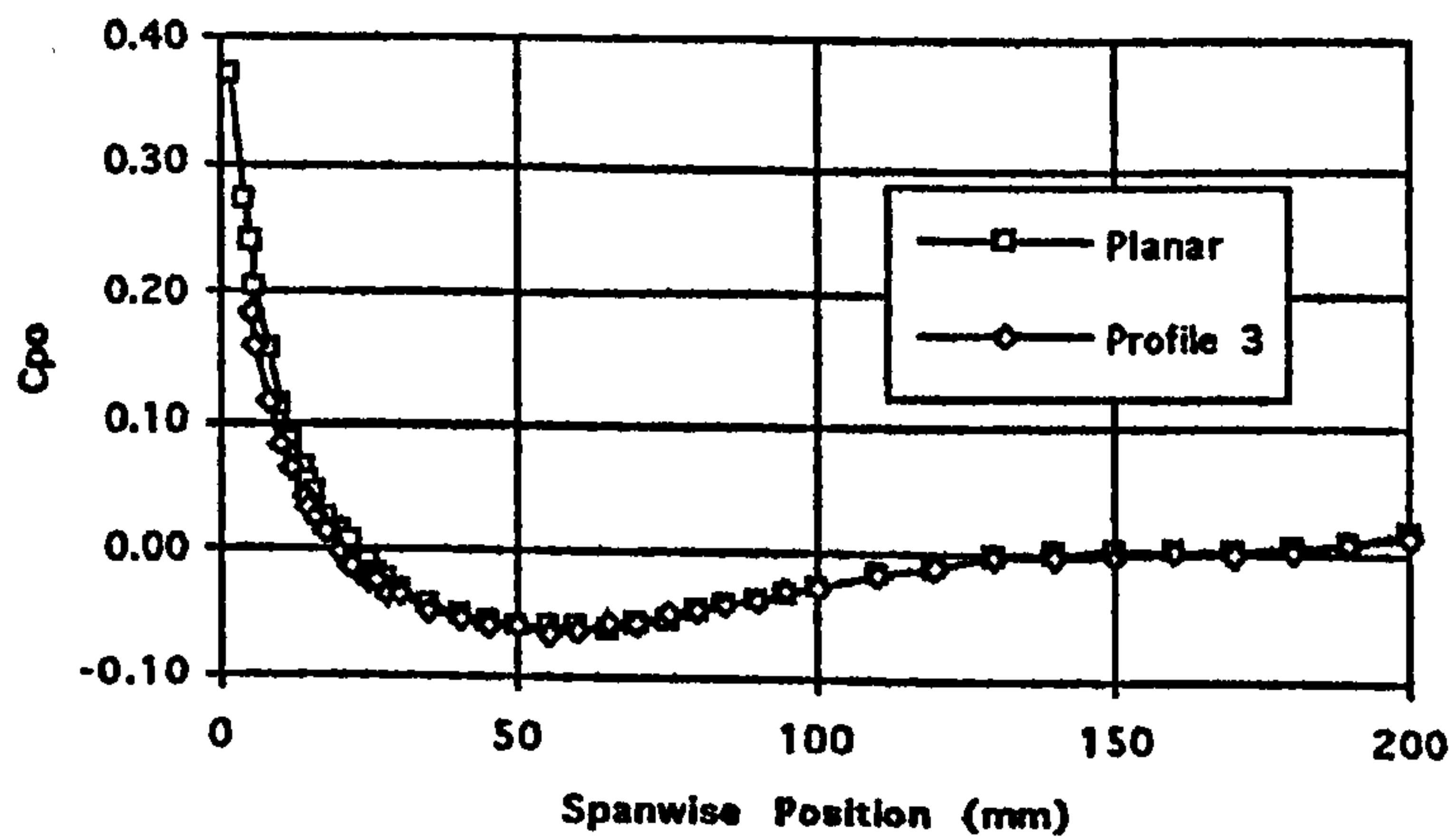
Figure 6.23 Measured Total Pressure Coefficient 100% C_{ax} Upstream.
