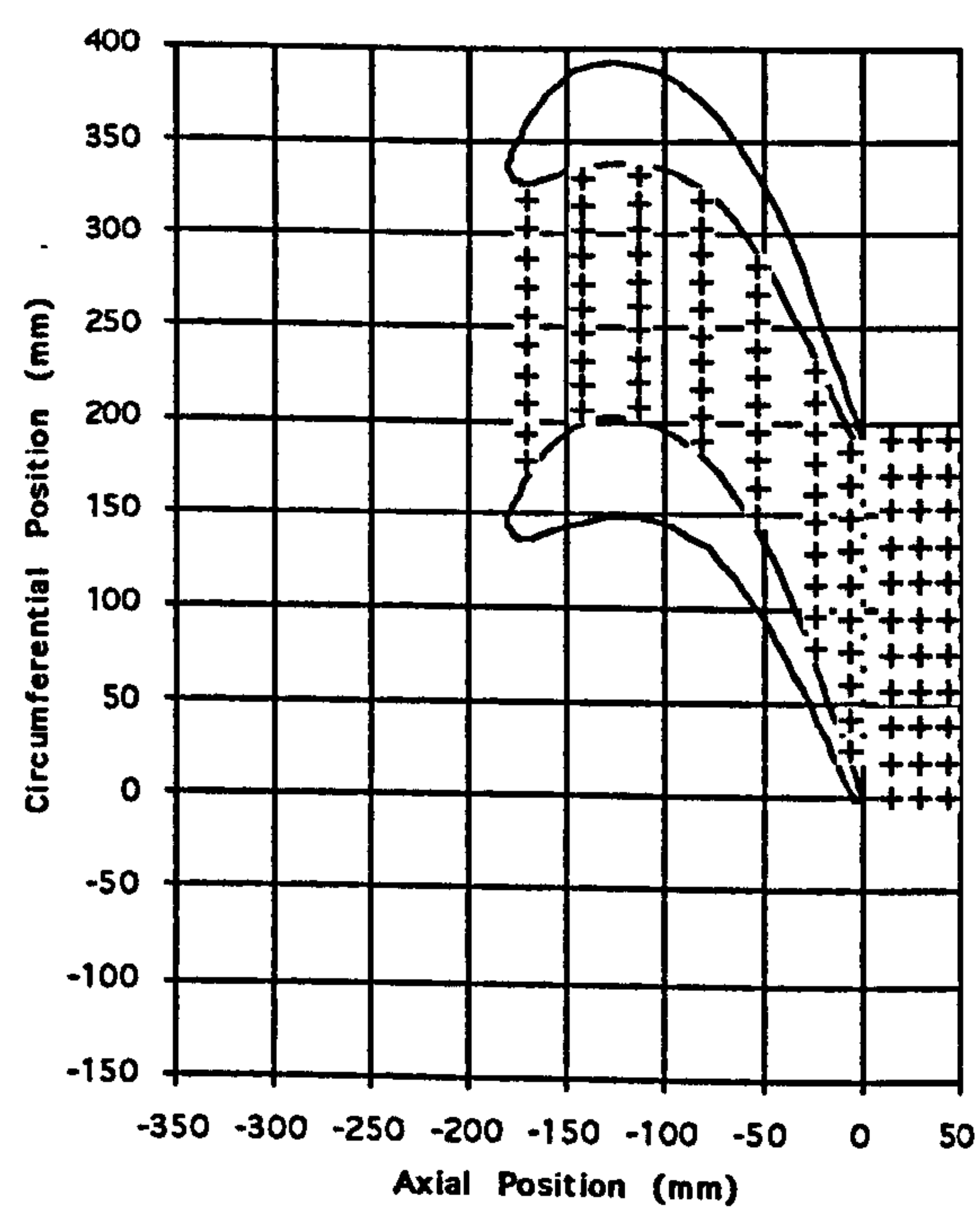
Figure 3.4 End-wall Measurement Locations.
