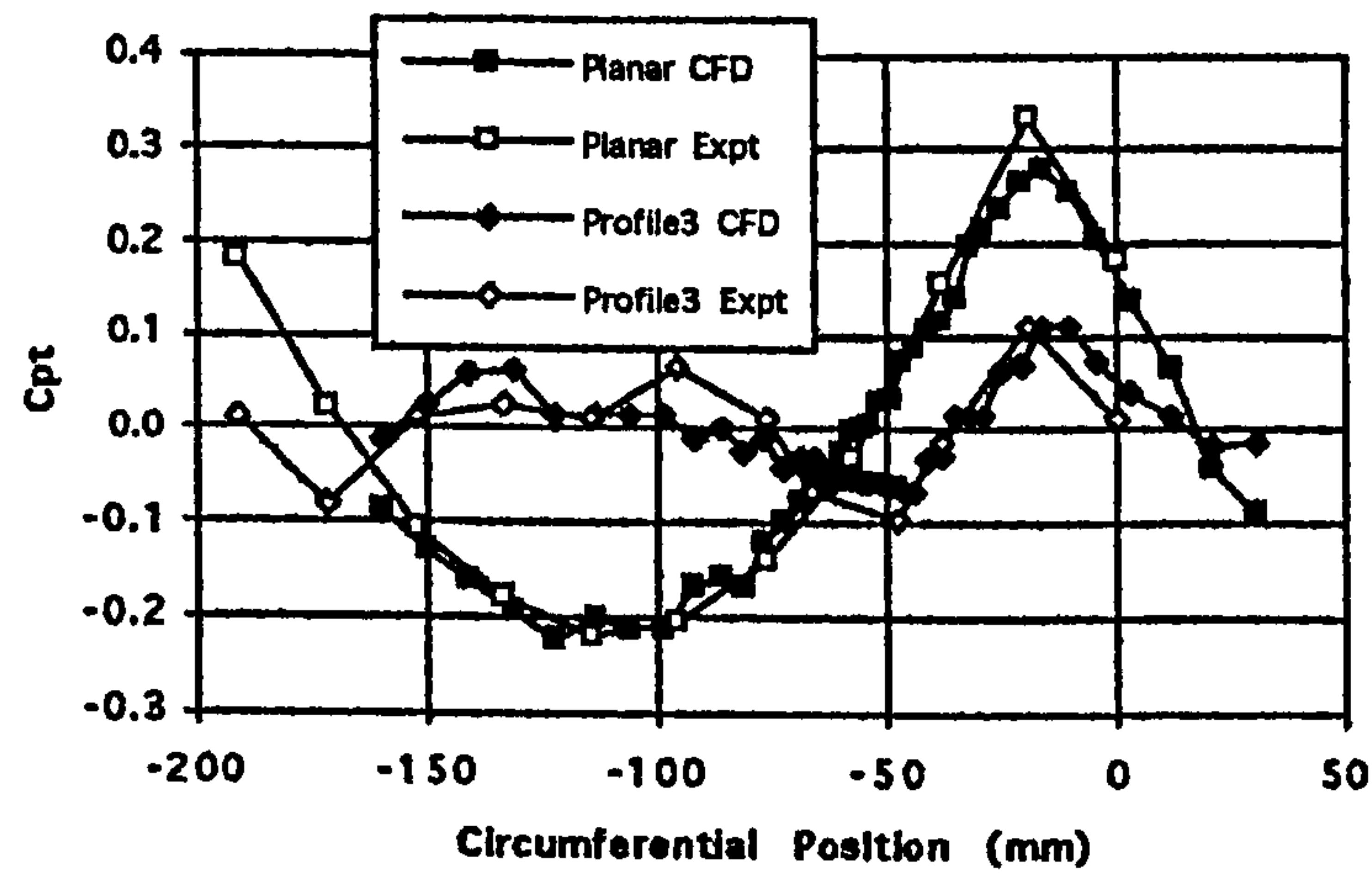
Figure 6.22 Experimental Non-Dimensional Pressures at Platform Trailing Edge (Fine Grid CFD and Planar Wall Data Included for Comparison).
