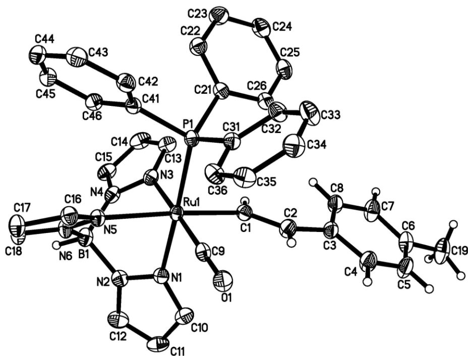
Figure 28 Molecular structure of 23. In this and subsequent Figures, only a selection of the H atoms are shown for clarity.
