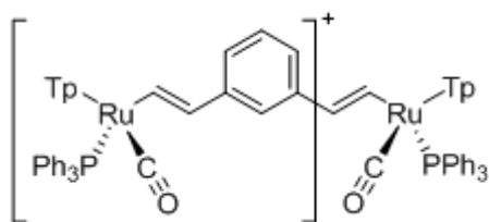
Figure 54 A schematic representation of [36]^{2+} showing an idealised representation of the localised charge distribution.
