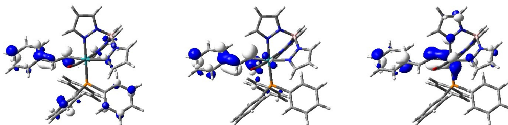
Figure 48 Contour plots of LUMO+4, \alpha -LUSO and \beta -HOSO for \mathbf{23-H}/[\mathbf{23-H}]^+ .
