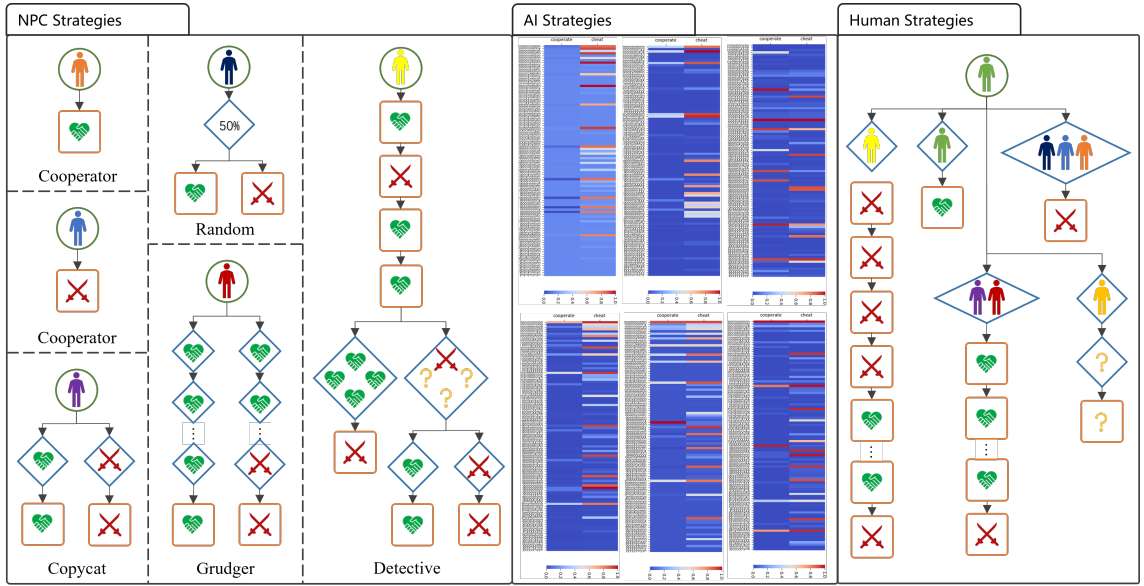
Figure 4.5: visualisation of player decision trees and corresponding strategy distributions. The left panels illustrate how different personality archetypes make sequential decisions, while the right panels depict the distribution of these strategies across multiple training epochs. The heat map illustrates the q-table information and shows how player behaviours evolve.
