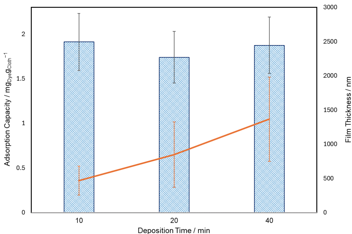
Figure 3-8. Maximum adsorption capacity for a DMAM-phenol derivatised, pulsed plasma poly(4-VBC) coated TPU cloths, following deposition for either 10, 20 or 40 min towards 50 mg L -1 anionic dye AB10B solutions (blue bars). The thickness of the deposited pulsed plasma poly(4-VBC) films (red line) has been overlain.
