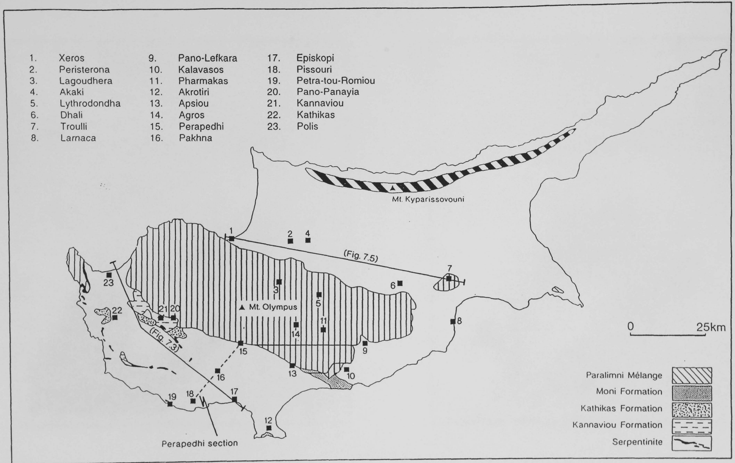
Fig. 7.6. Simplified geological map of Cyprus, displaying the localities of place names employed in Chapter 7, cross-section lines (Figs 7.3,5) and the position of the Perapedhi section (Krashennnikov and Kaleda, 1994).
