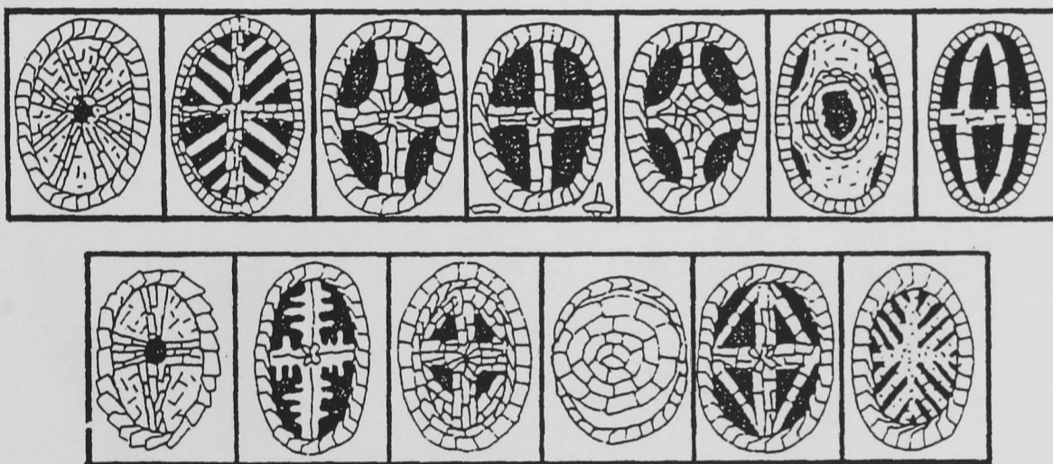
Fig. B.11. Typical Ahmuellerellace structural arrangements (modified from Perch-Nielsen, 1985a).
