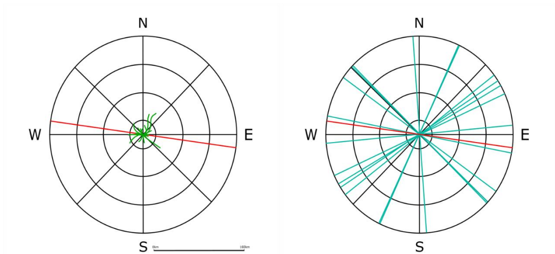
Figure 3.21: Rose diagram showing the orientations of volcanic rift zones (green lines) compared to the overall azimuth of the segment (HAWAII-04) which the volcanoes lie on (red line).
