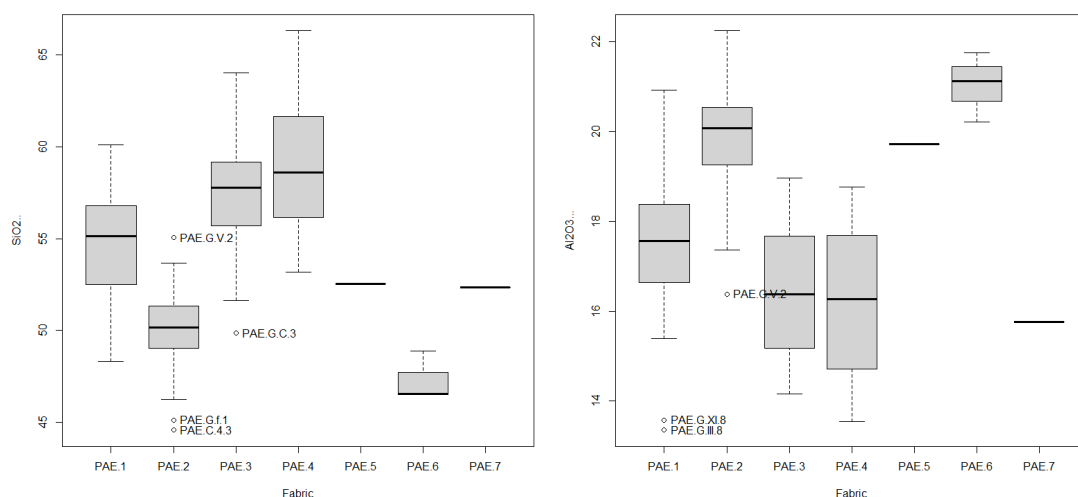
Figure 7.47. Paestum. Univariate plots showing the variations in \text{SiO}_2 and \text{Al}_2\text{O}_3 content (wt%) grouped according to petrographic fabric.
