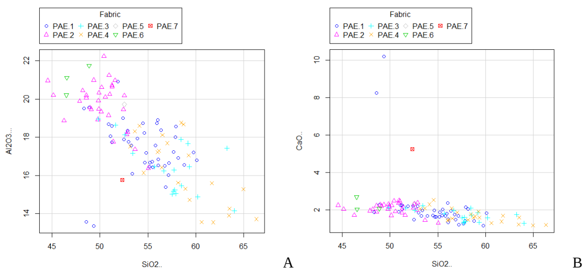
Figure 7.48. Paestum. Binary major oxides (wt%) compositional plots of samples grouped according to petrographic fabric: A. \text{SiO}_2 and \text{Al}_2\text{O}_3 ; B. \text{SiO}_2 and \text{CaO} .
