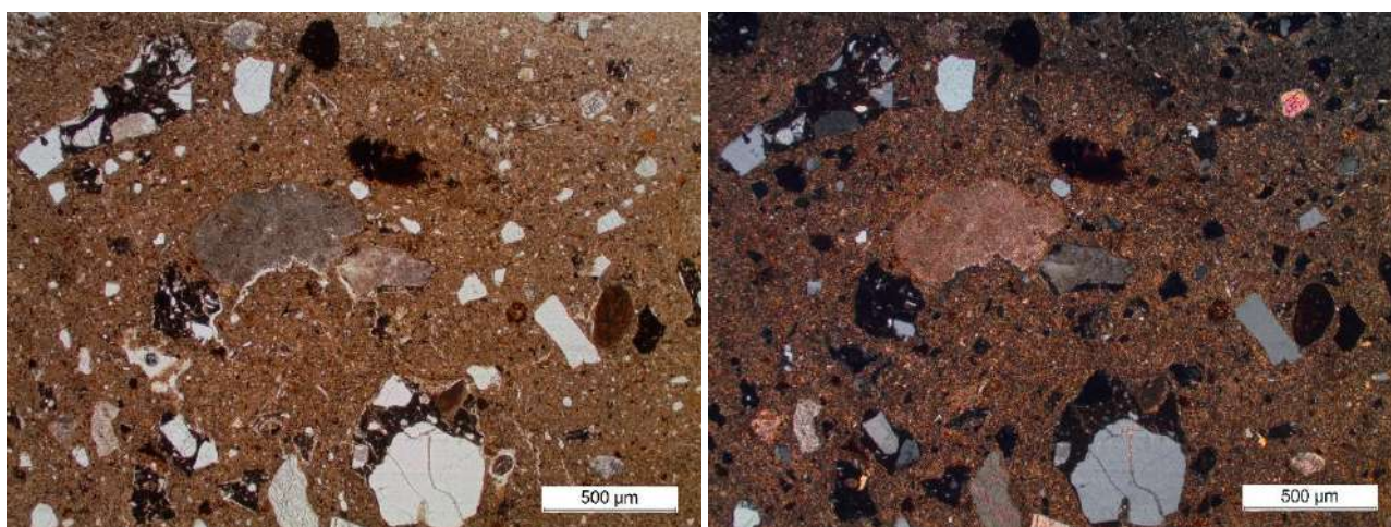
Figure 7.9. Details of the micritic and spathic calcite inclusions detected in sample PAE.A.II.01, petrographic fabric Pae7, carbonatic with grog.
