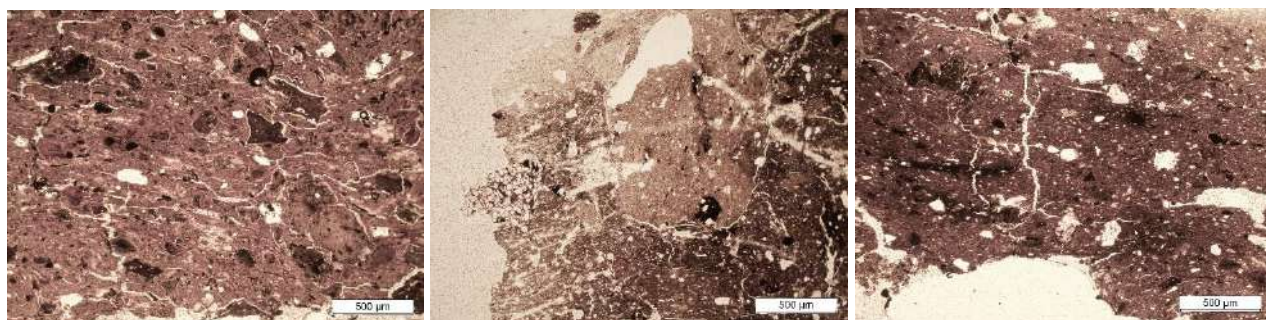
Figure 7.29. Fabric Sal2, microphotographs of the samples with grog/ARF, sedimentary rock fragments and burnt organics (PPL). From left to right samples SAL.C.II.05, SAL.C.II.03, SAL.C.II.01.
