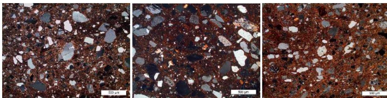
Figure 7.6. XPL thin section photographs of fabric Pae4 subfabrics: left Pae4a (sample PAE.A.III.07); centre Pae4b (sample PAE.A.II.4); right Pae4c (sample PAE.G.IX.1).
