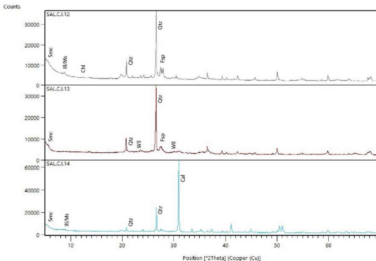
Figure 7.34. Sala Consilina. XRD spectra of samples from fabrics Sal1 (SAL.C.I.12) with presence of chlorite/kaolinite, Sal4 (SAL.C.I.13) and Sal5 (SAL.C.I.14). Ill: illite; Ms: muscovite; Qtz: quartz; Fsp: feldspars; Cal: calcite; Wll: wollastonite.
