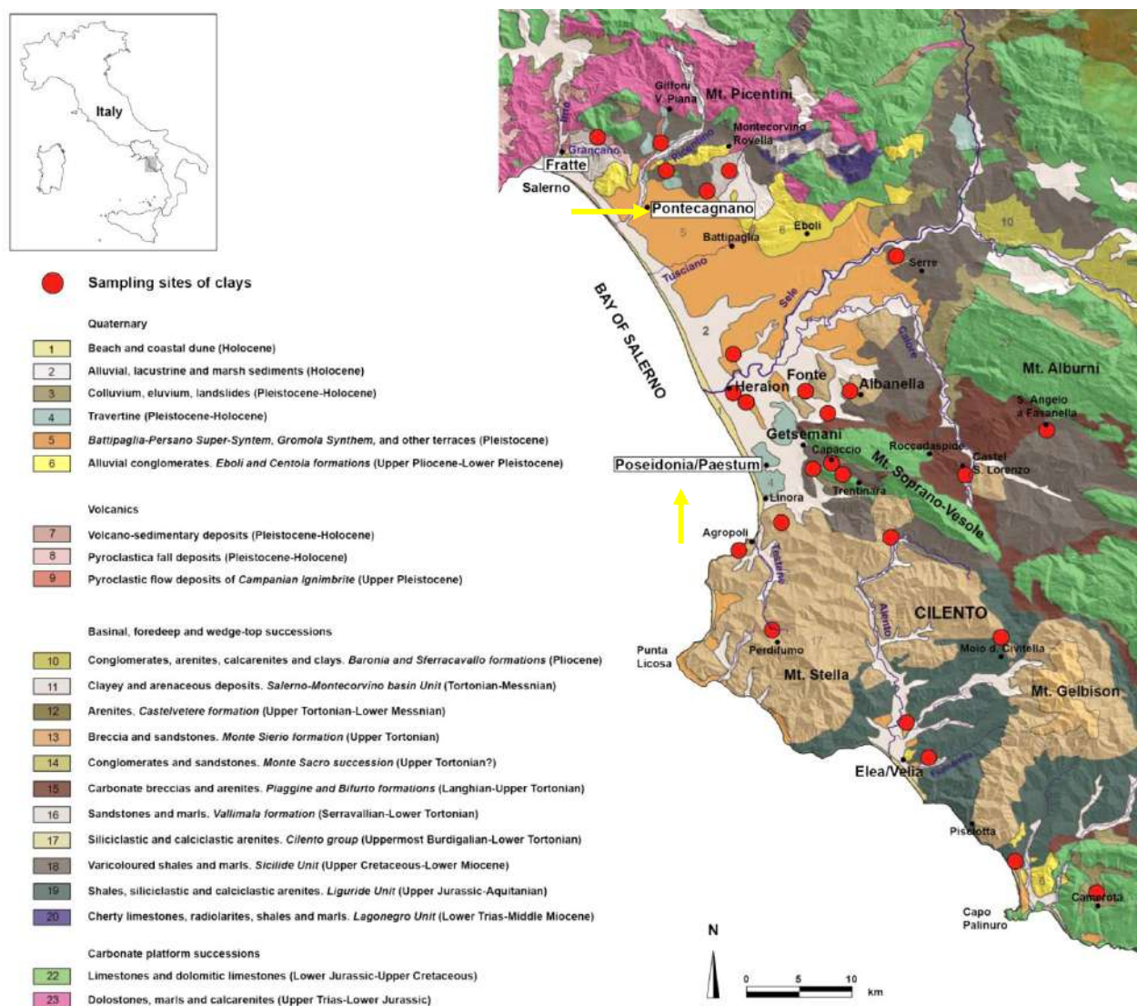
Figure 4.2. Geological map of the Sele River plain and surroundings. The yellow arrows point to the archaeological sites analysed: Pontecagnano and Paestum. The red dots are the clays sampled and reported in De Bonis and Gassner 2018.
