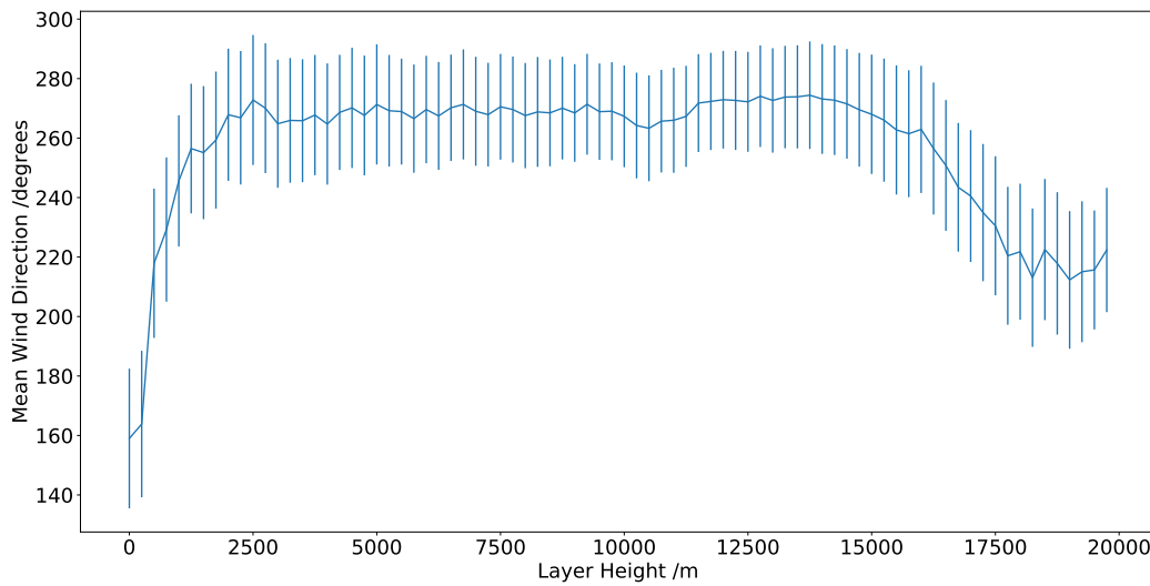
Figure 3.21: Mean wind direction with height of the layers across the available SCIDAR data. Errorbars are the standard deviation of the angular change between layers.
