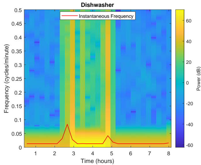
Figure 3.4: Instantaneous frequency estimate of a dishwasher from the UK DALE dataset.
