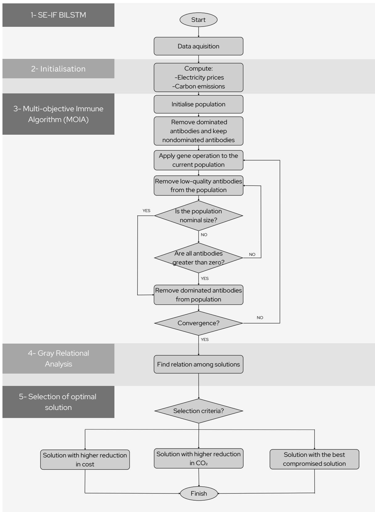
Figure 5.6: Flowchart of the multi-objective problem, including the MOIA.
