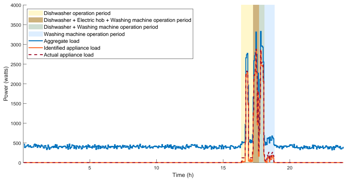
Figure 4.6: Scenario 5 load showing detected appliance load.
