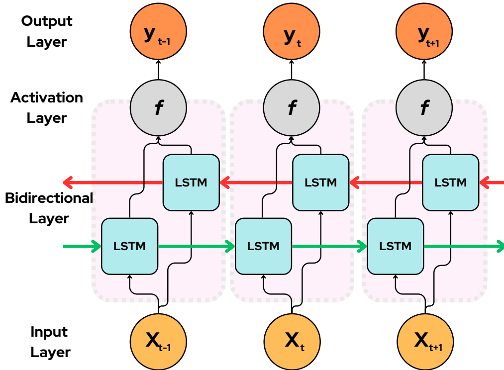
Figure 2.4: Diagram of the layers of a BiLSTM neural network [71].
