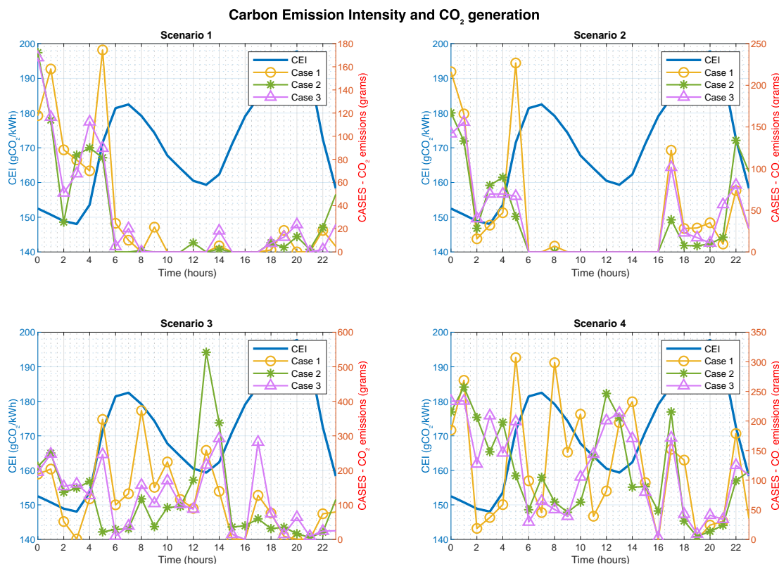
Figure 5.10: CO 2 generation in comparison to the CEI in each scenario for all cases using the MOIA.
