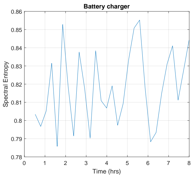
Figure 3.1: Spectral entropy of a battery charger from the UK DALE dataset.
