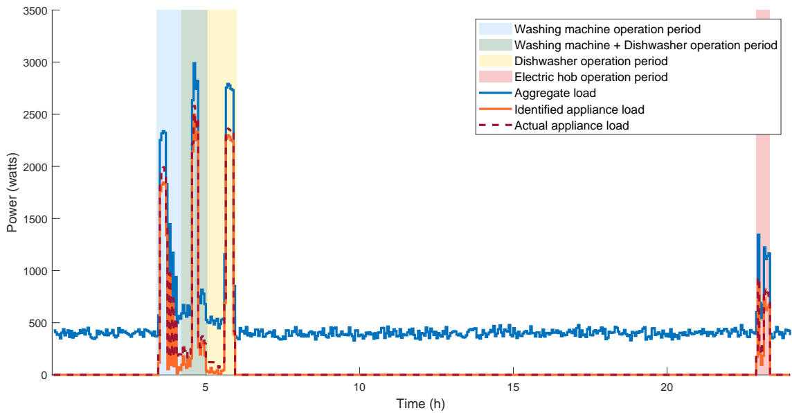
Figure 4.3: Scenario 2 load showing detected appliance load.
