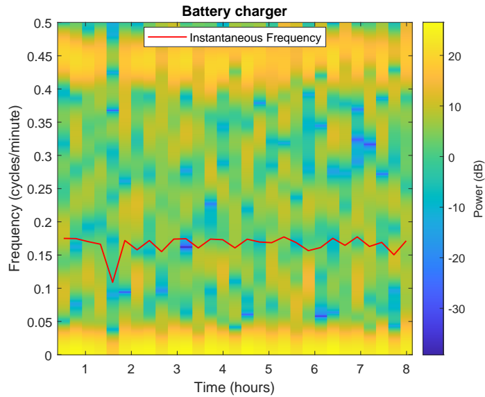
Figure 3.3: Instantaneous frequency estimate of a battery charger from the UK DALE dataset.
