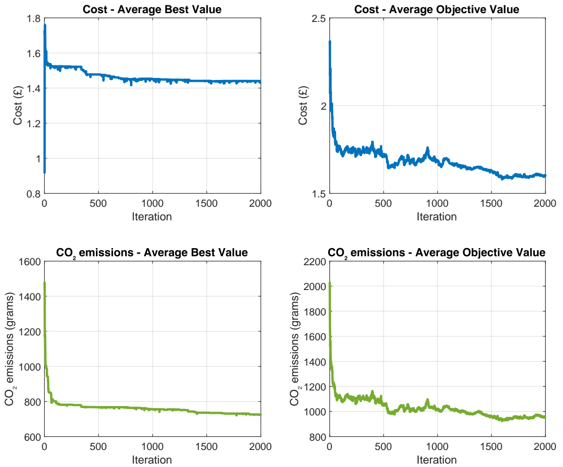
Figure 5.9: Convergence trends of the MOIA algorithm over iterations. The top graphs display the progression of the average best value (ABV) and average objective value (AOV) for Cost, while the bottom graphs show these values for CO 2 emissions.
