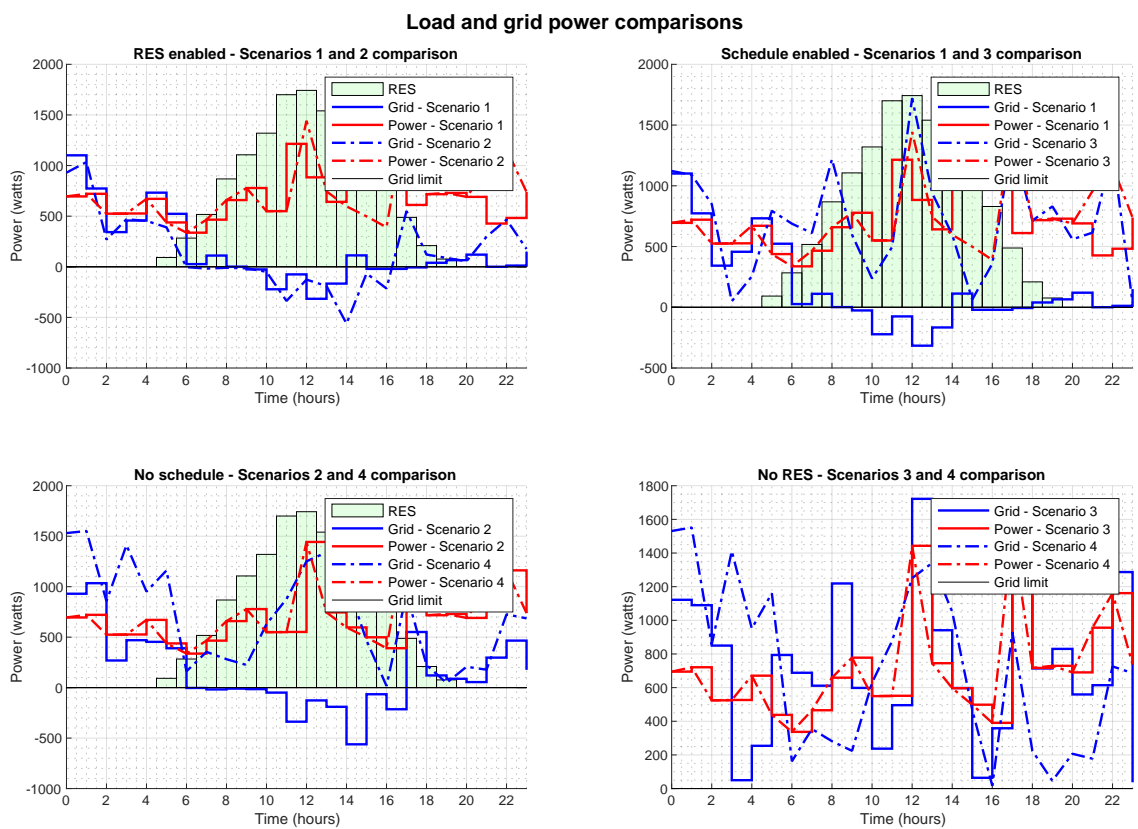
Figure 5.12: Comparison of similar scenarios, regarding their abilities to use RES or scheduling. All scenarios are considering Case 3 using the MOIA.
