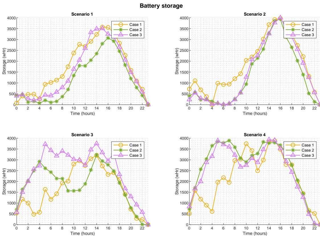
Figure 5.11: Battery storage behaviour in each scenario for all cases using the MOIA.
