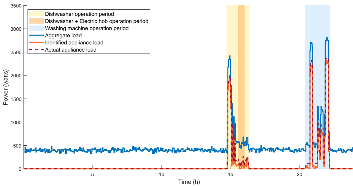
Figure 4.5: Scenario 4 load showing detected appliance load.
