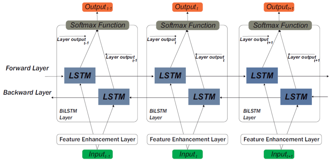
Figure 3.10: Structure of the SE-IF BiLSTM neural network
