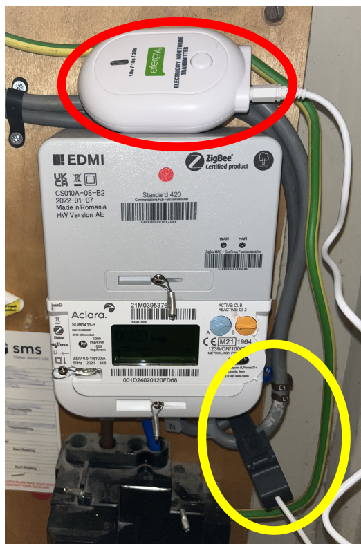
Figure 2.1: An Efergy energy monitor transmitter (red circle) that takes readings with a CT sensor (yellow circle) in an electricity box.
