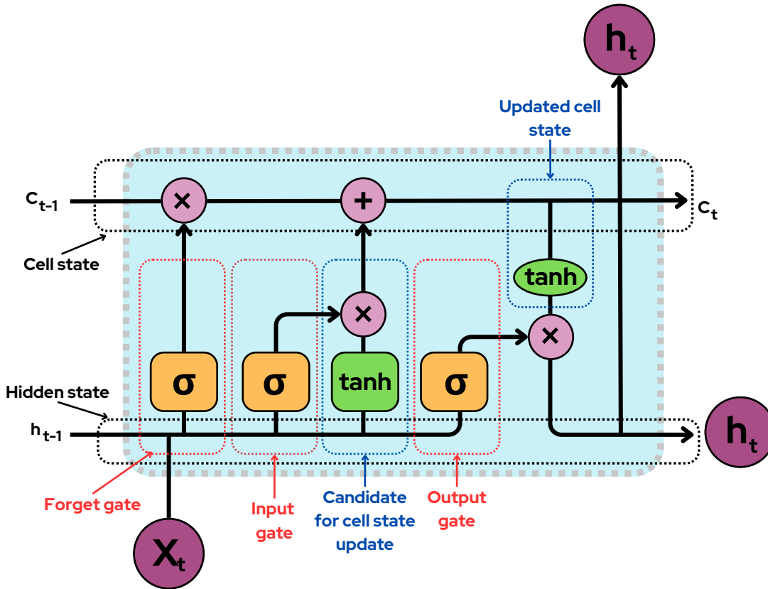
Figure 2.3: Diagram of a LSTM neural network layer [65].
