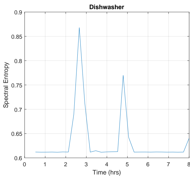
Figure 3.2: Spectral entropy of a dishwasher from the UK DALE dataset.
