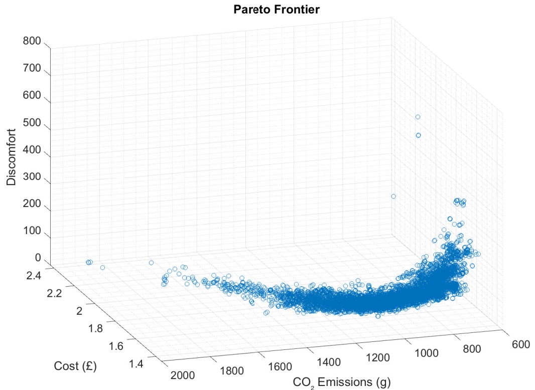
Figure 5.5: Pareto frontier obtained after evaluating the MOP with the MOIA.
