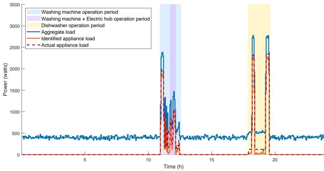
Figure 4.4: Scenario 3 load showing detected appliance load.
