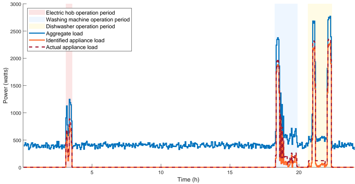
Figure 4.2: Scenario 1 load showing detected appliance load.
