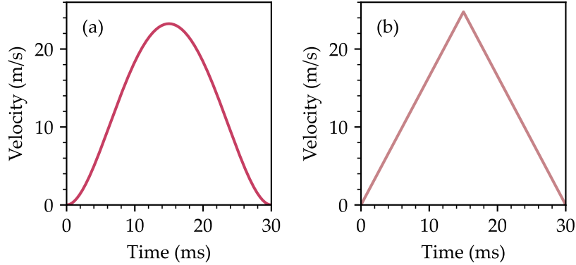
Figure 3.7: Transport velocity trajectories, as defined in Eq. (3.6) and Eq. (3.7) (a) Minimum Jerk Trajectory (b) Linear trajectory.
