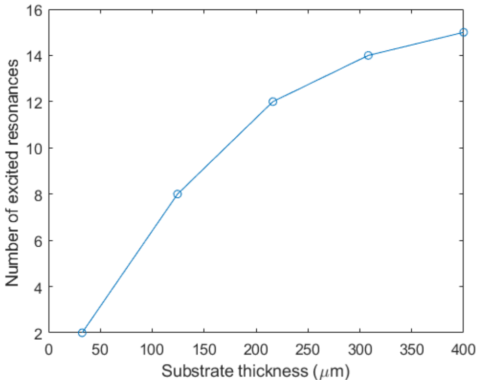
FIGURE 3.29: Increasing number of excited resonances in the 0.3 -2 THz range with increasing substrate thickness
