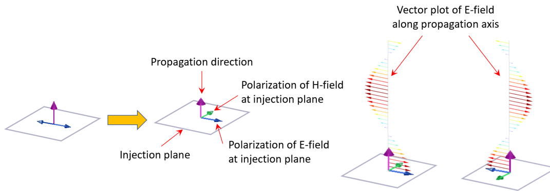
(C) Lumerical source injection notation
