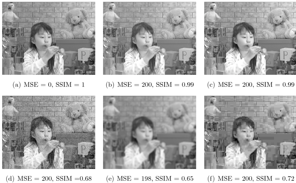
FIGURE 4.8: Comparison between SME and SSIM algorithms with respect to noisy images [95]
